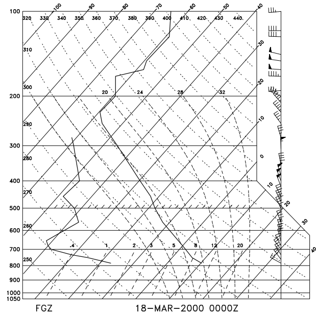
Figure 2: Skew T - \ln p plot from Flagstaff, Arizona (FGZ) taken at 0000 UTC 18 March 2000.
