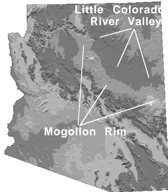
Figure 1: Image showing terrain and elevation over the state of Arizona. The Mogollon Rim and Little Colorado River Valley are noted.
