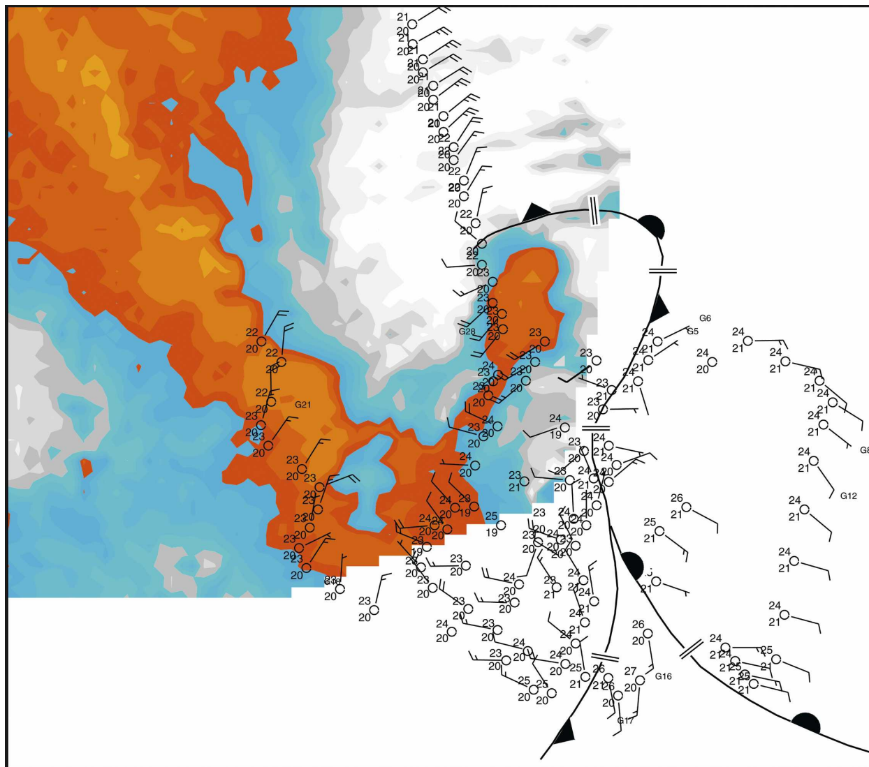
FIG. 10. Base scan reflectivity from the DOW with MM surface observations overlain at 2019 UTC 8 Jun 1995; the MM observations have been selectively thinned for legibility.
