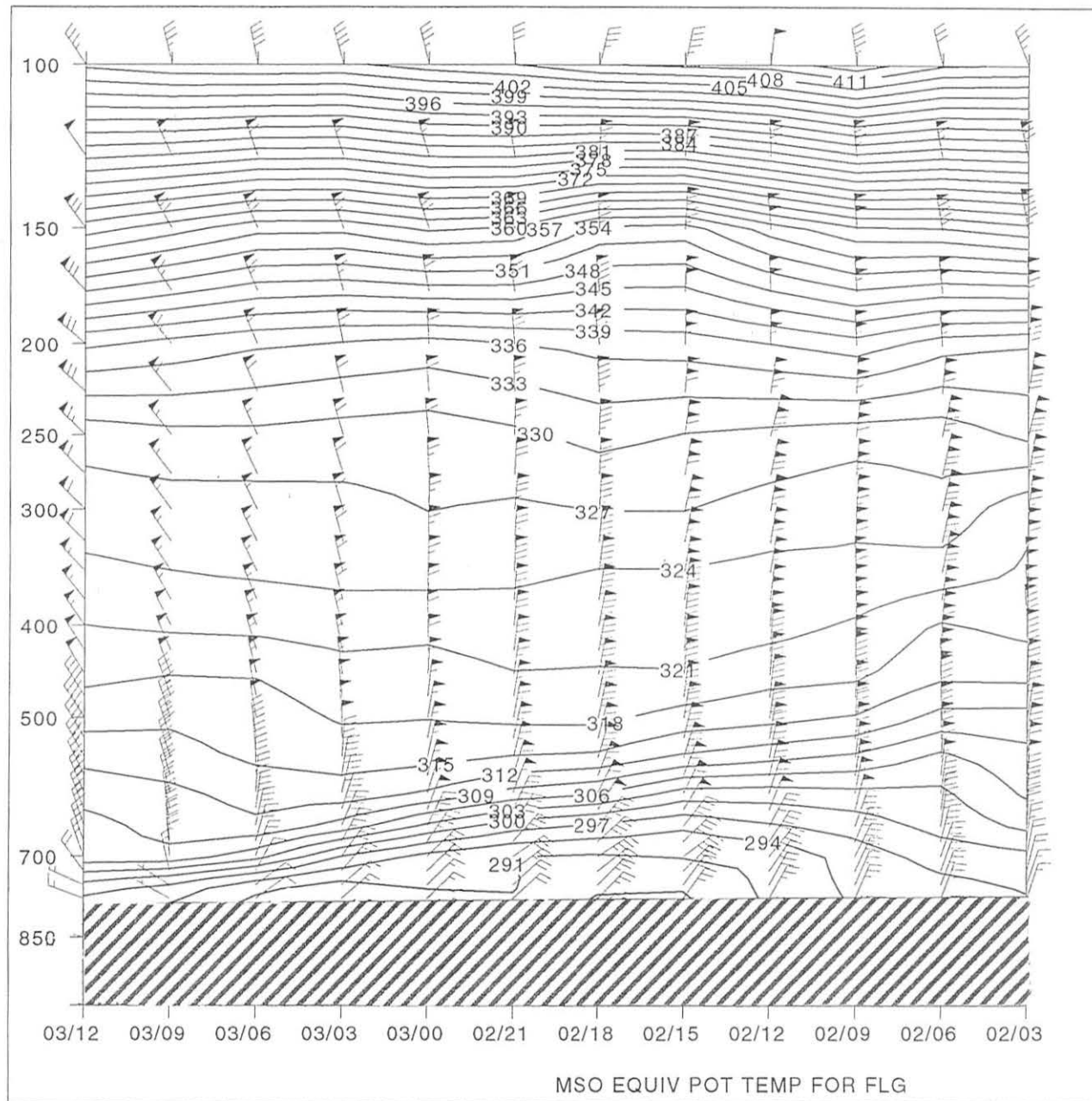
Fig. 6. Meso Eta forecast (from 0300 UTC 1/2/96 run) time-section of equivalent potential temperature ( \theta -e) and winds. Valid times increase from right to left. Area below ground level (approx. 780mb) is hatched. Height of the mountain in question is near 700mb.
