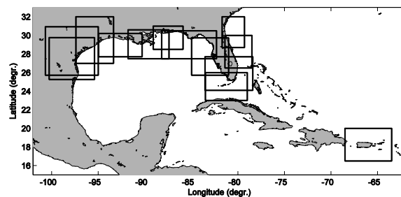
Figure 2. High-resolution NWPS model domains for coastal WFOs in the Western, Alaskan and Pacific Regions (top, WFO Guam not shown), Eastern Region (center) and Southern Region, including Puerto Rico and the Virgin Islands (bottom).
