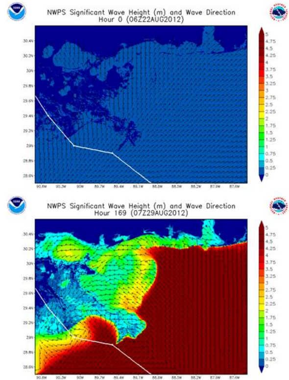
Figure 9. Field output from NWPS displaying the total significant wave height and peak wave direction several days in advance of landfall (top) compared to the total significant wave height and peak wave direction at or around landfall (bottom). Hurricane best track included (white line).
