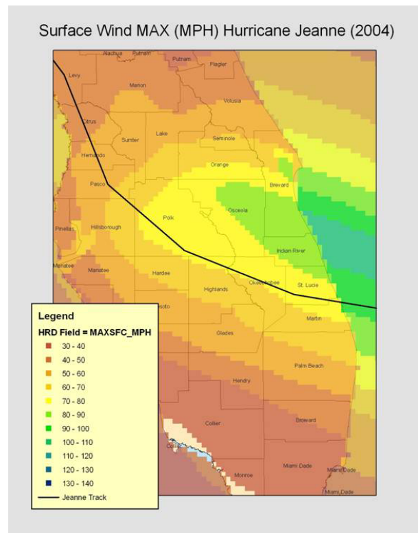
Fig. 12 Same as Fig. 6 except for Hurricane Jeanne. Note the winds of 100-110 mph along the coast north of the hurricane track and within the special tornado warning area.
