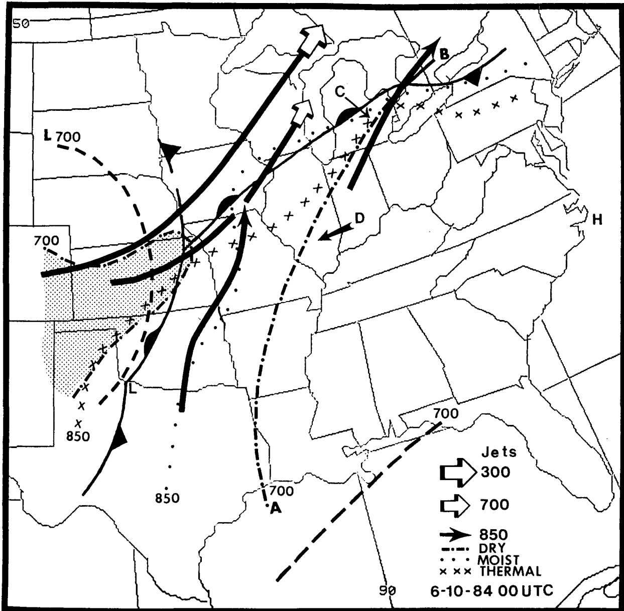
FIG. 10. Composite analysis for 0000 UTC 10 June 1984. Surface fronts and 700-mb troughs shown by conventional notation. Other analyzed features are identified in the legend. The location of the Lake Charles, Louisiana to Buffalo, New York cross section (Figs. 14a & b) coincides with the dashed-dot dry axis from "A" to "B." Arrow over Michigan at "C" points to location of tornado at 1943 UTC, and arrow at "D" indicates location of Salem, Illinois upper-air site (see Fig. 11).
