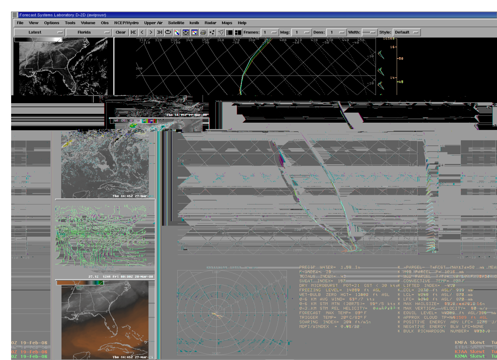
AWIPS display of the KMFL, KTBW, KJAX, and KXMR composite soundings for the NE flow regime.
