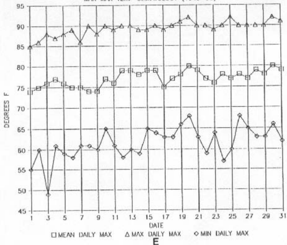
MAR MAX TEMP CLIMATOLOGY (1949-86)
