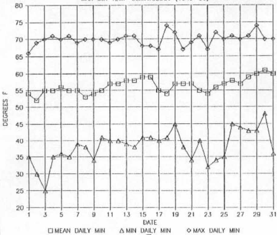
MAR MIN TEMP CLIMATOLOGY (1949-86)
