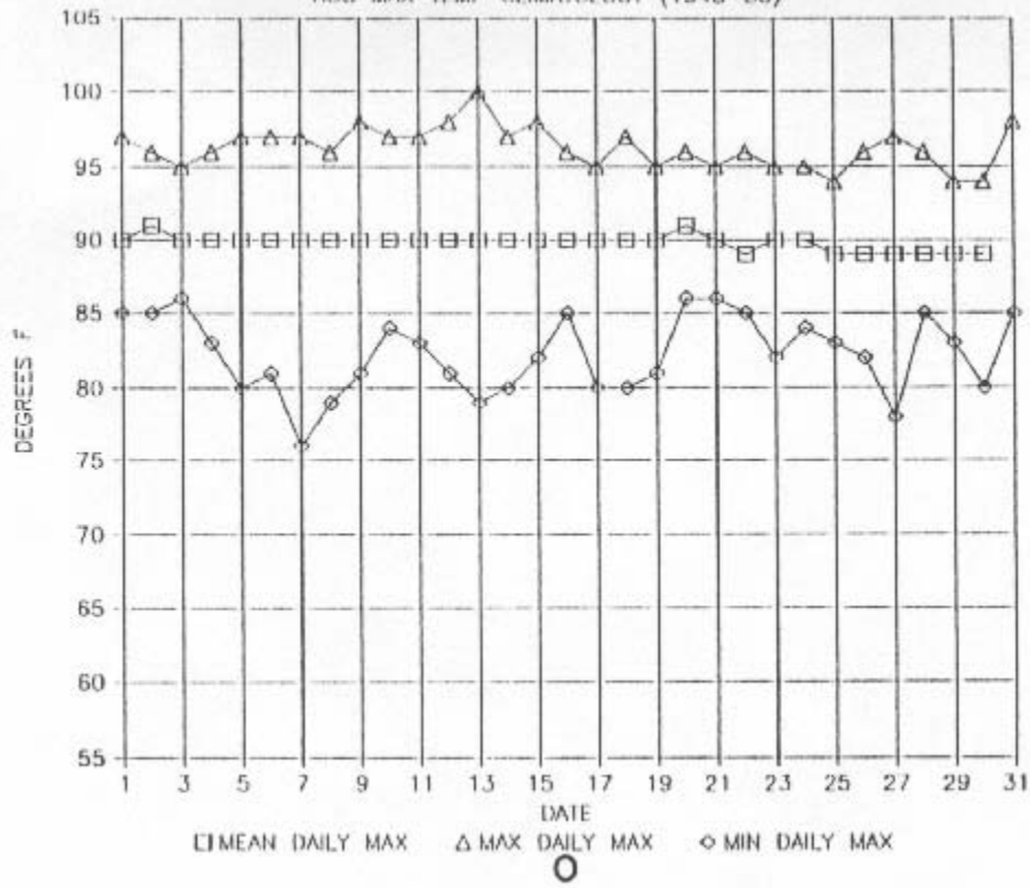
AUG MAX TEMP CLIMATOLOGY (1948-86)
