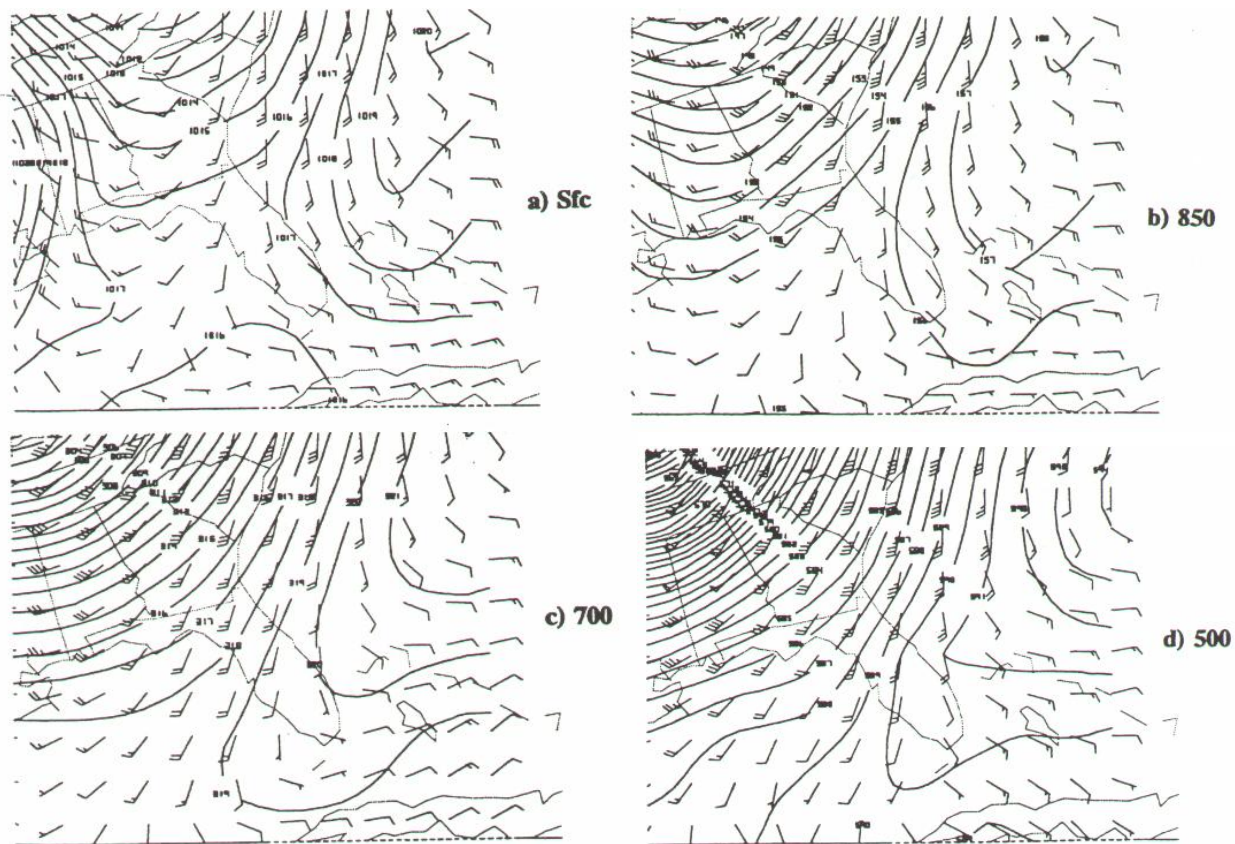
Fig. 15. Same as Fig 3, except for 1200 UTC September 27, 1993.
