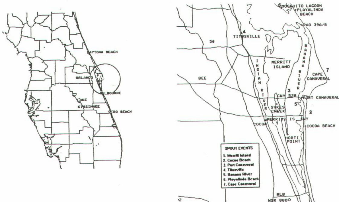
Fig. 2. Cape Canaveral area, showing location of events (1-7) described in text.
