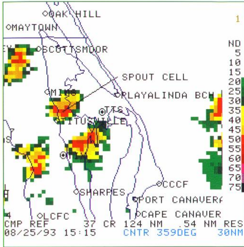
Fig. D. Composite Reflectivity 1515 UTC, August 25, 1993.
