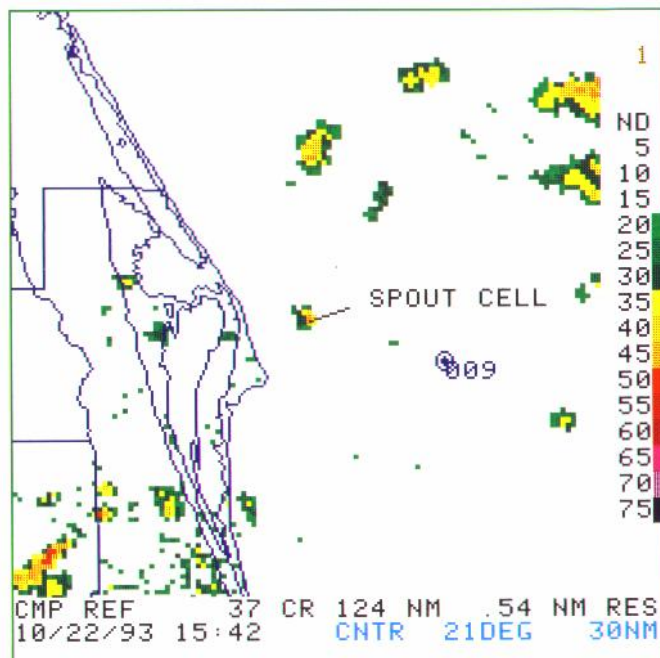
Fig. G1. Composite Reflectivity 1542 UTC, October 22, 1993.
