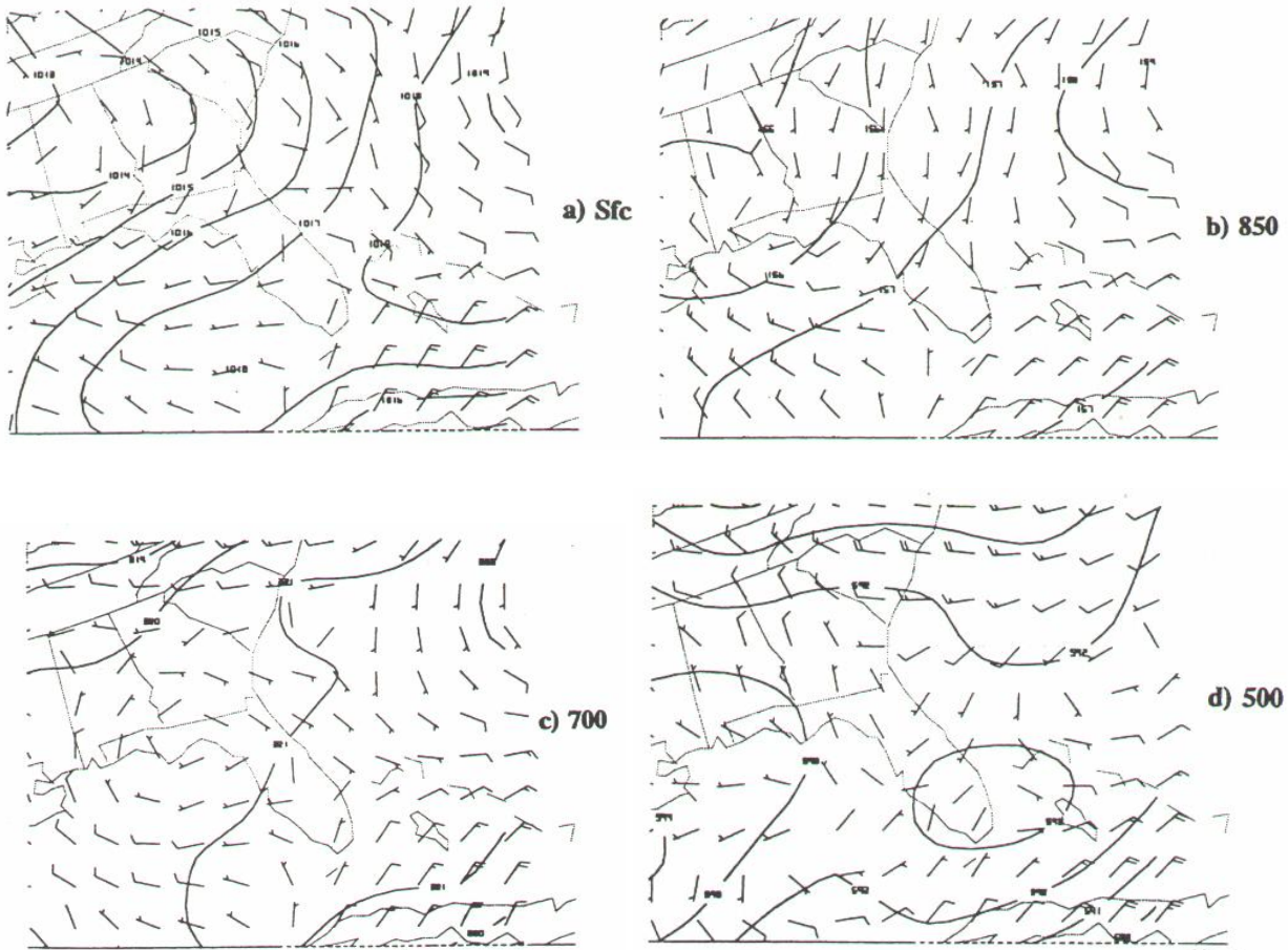
Fig. 6. Same as Fig. 3, except for 0000 UTC July 24, 1993.
