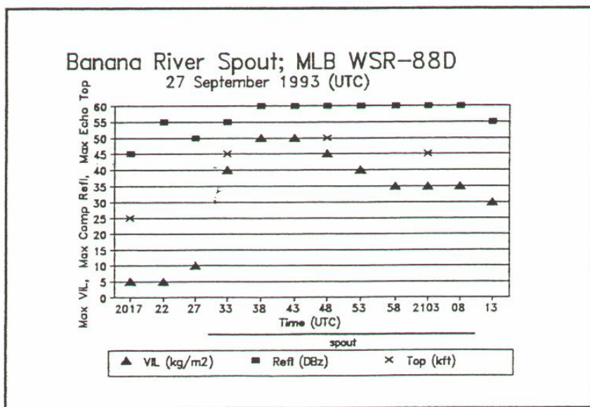
Fig. 17. Radar observed parameters of the spout cell. The estimated time and duration of the spout is indicated with a bold line below the time axis.
