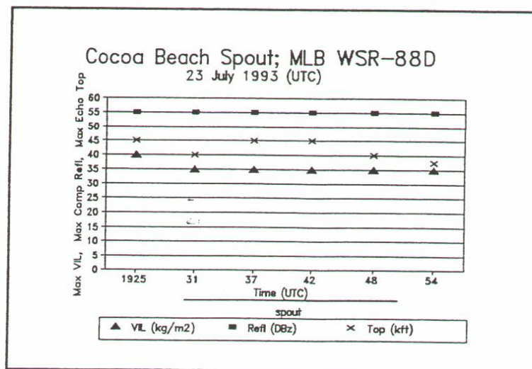
Fig. 8. Radar observed parameters for the spout cell. The estimated time and duration of the spout is indicated with a bold line below the time axis.
