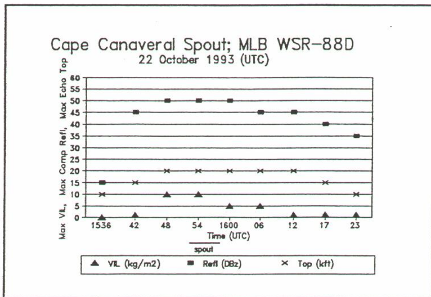
Fig. 23. Radar observed parameters of the spout cell. Bold line at bottom represents the estimated spout duration.
