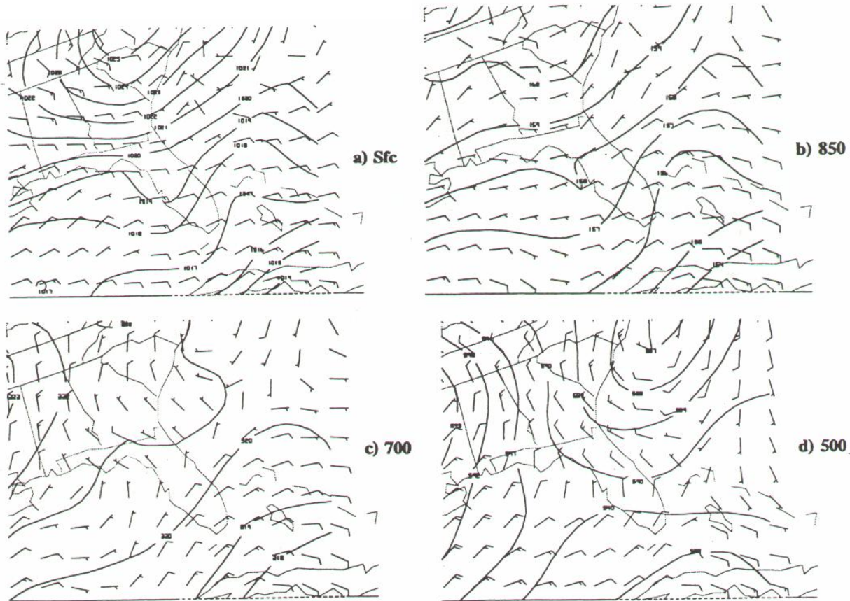
Fig 9. Same as Fig 3, except for 1200 UTC August 10, 1993.
