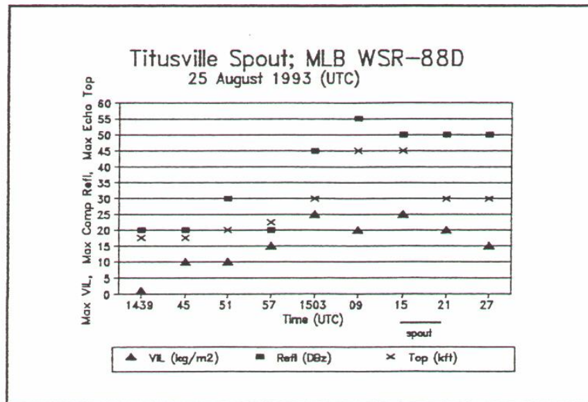
Fig. 14. Radar observed parameters for the spout cell. The estimated time and duration of the spout is indicated with a bold line below the time axis.
