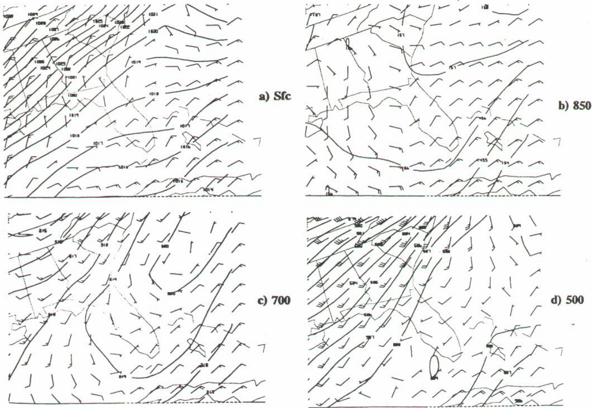
Fig. 21. Same as Fig. 3, except for 1200 UTC October 22, 1993.
