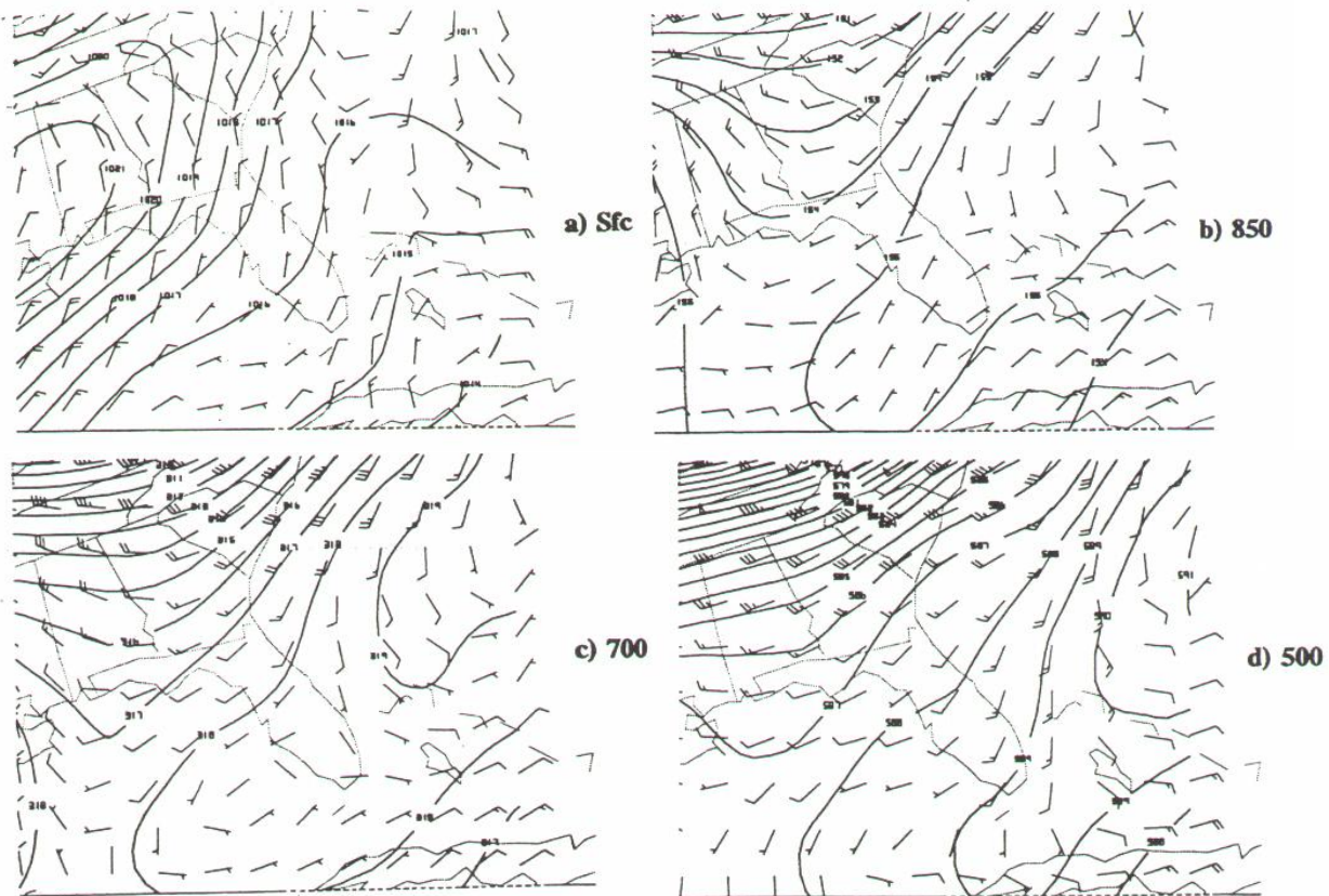
Fig. 18. Same as Fig 3, except for 1200 UTC September 28 1993.
