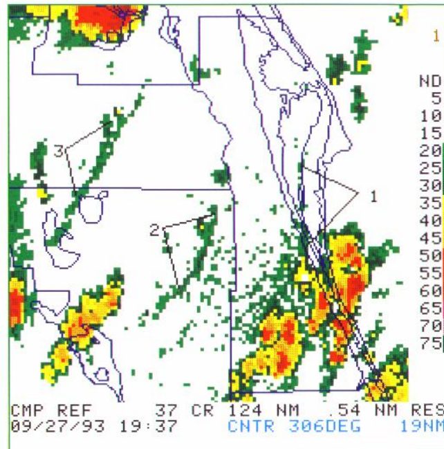
Fig. E. Composite Reflectivity 1937 UTC, September 27, 1993.
