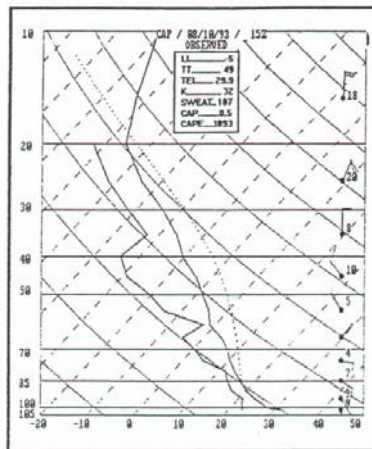
Fig. 10. Cape Canaveral sounding at 1500 UTC August 1993.
