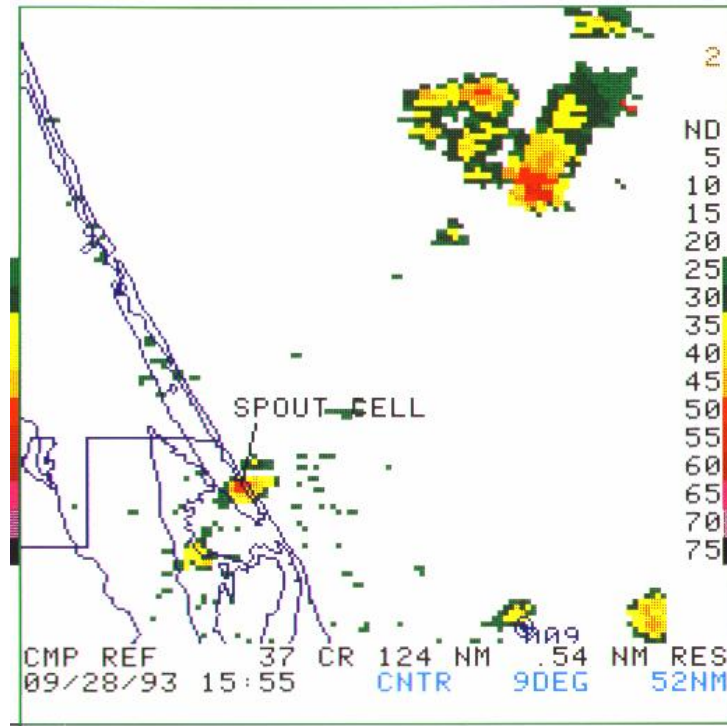
Fig. F2. Composite Reflectivity 1555 UTC, September 28, 1993.
