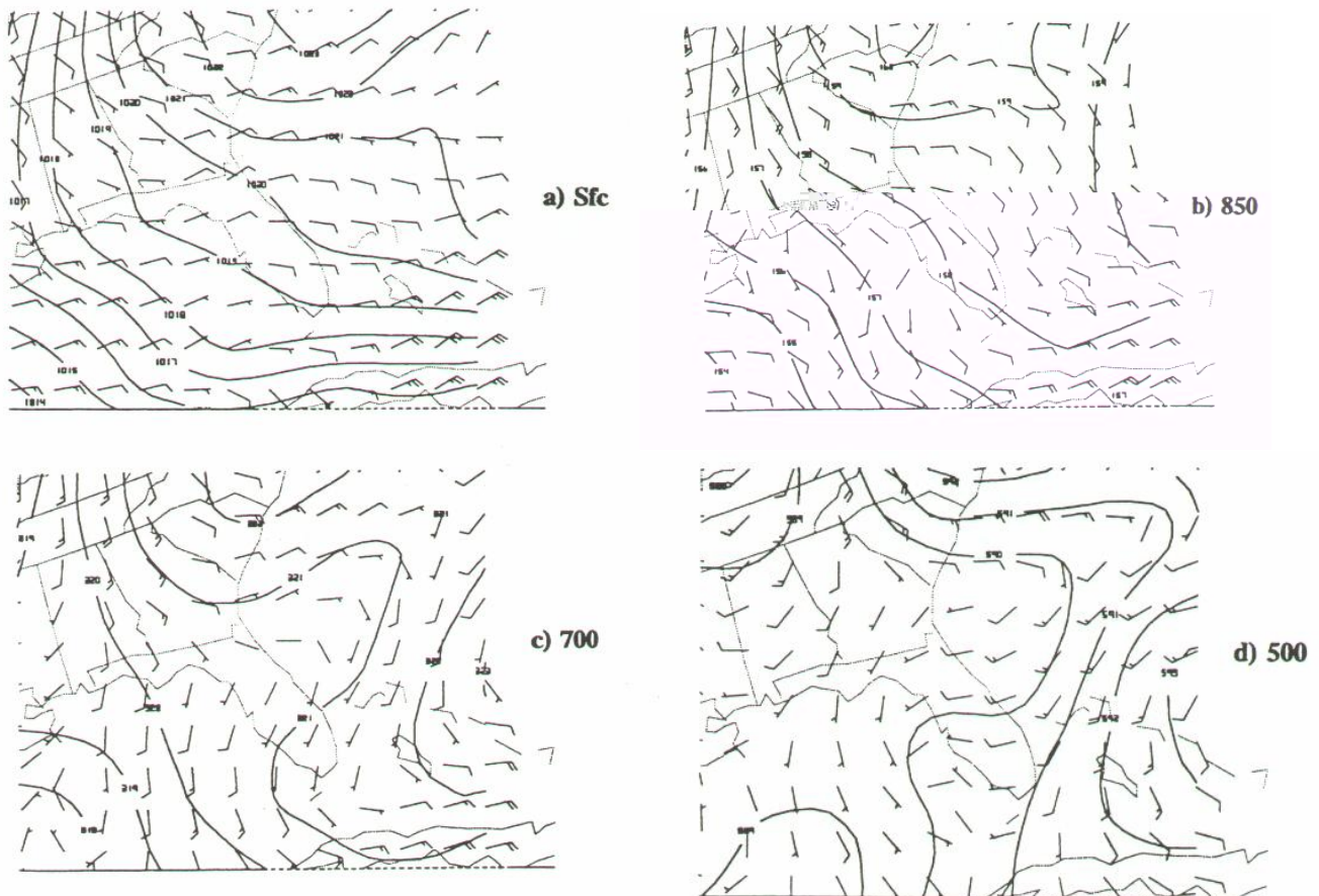
Fig 3. NGM analysis from PC-GRIDDS, 0000 UTC June 25, 1993. a) 1000 mb winds (kt) and MSL pressure (mb); b-d) wind (kt) and heights (dm) for levels indicated.
