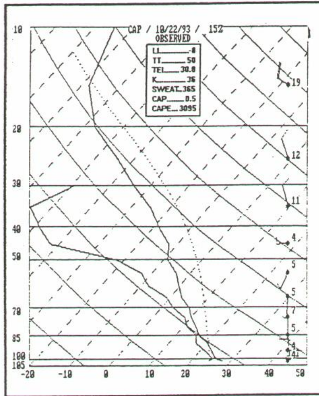
Fig. 22. Cape Canaveral sounding at 1500 UTC October 22, 1993.
