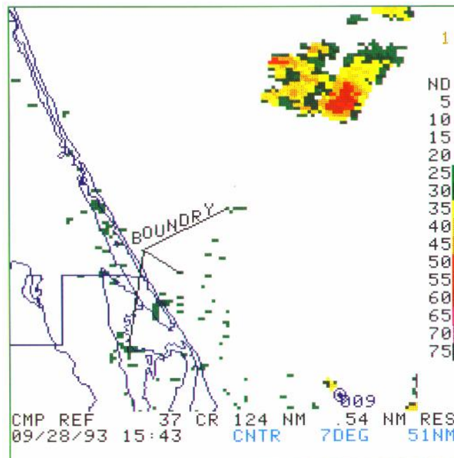
Fig. F1. Composite Reflectivity 1543 UTC, September 28, 1993.
