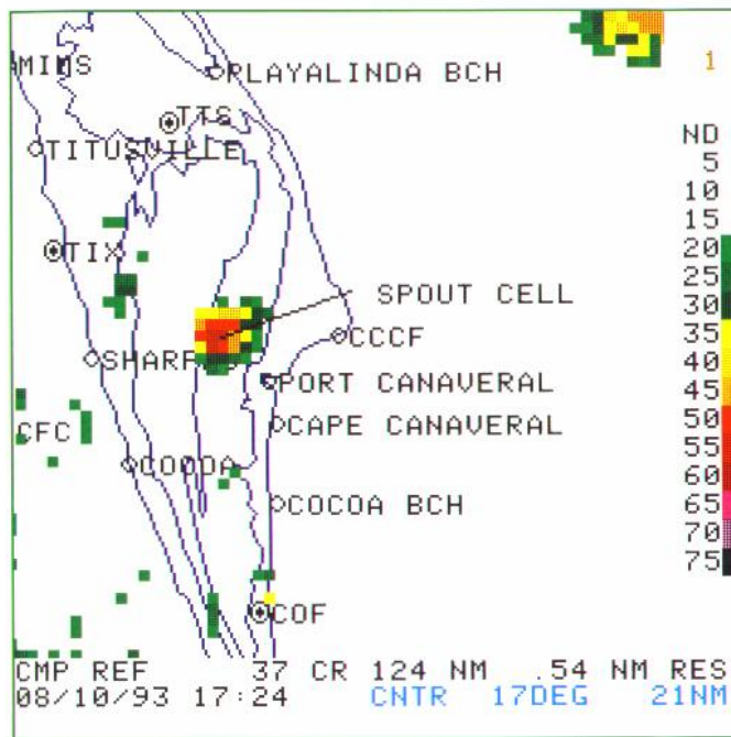
Fig. C. Composite Reflectivity 1724 UTC, August 10, 1993.
