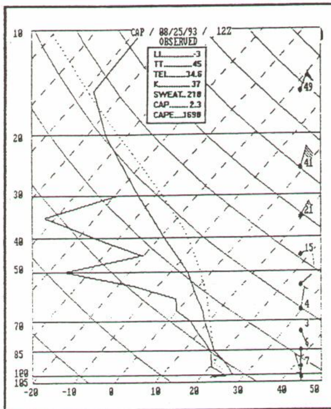
Fig. 13. Cape Canaveral sounding at 1200 UTC August 25, 1993.
