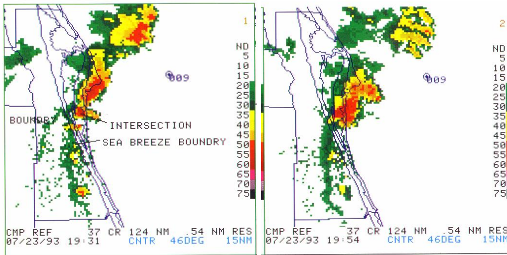
Fig. B. Composite Reflectivity 1931 and 1954 UTC, July 23, 1993.
