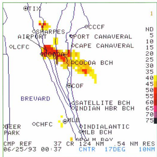
Fig. A. Composite Reflectivity, 0037 UTC, June 25, 1993.
