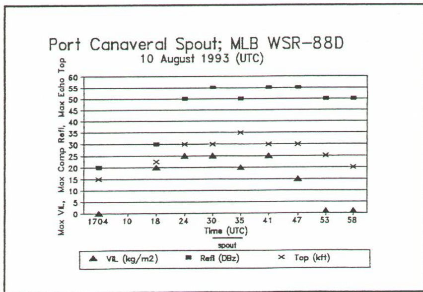
Fig. 11. Radar observed parameters for the spout cell. The estimated time and duration of the spout is indicated with a bold line below the time axis.
