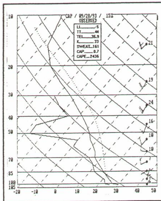
Fig. 19. Cape Canaveral sounding at 1500 UTC September 28, 1993.
