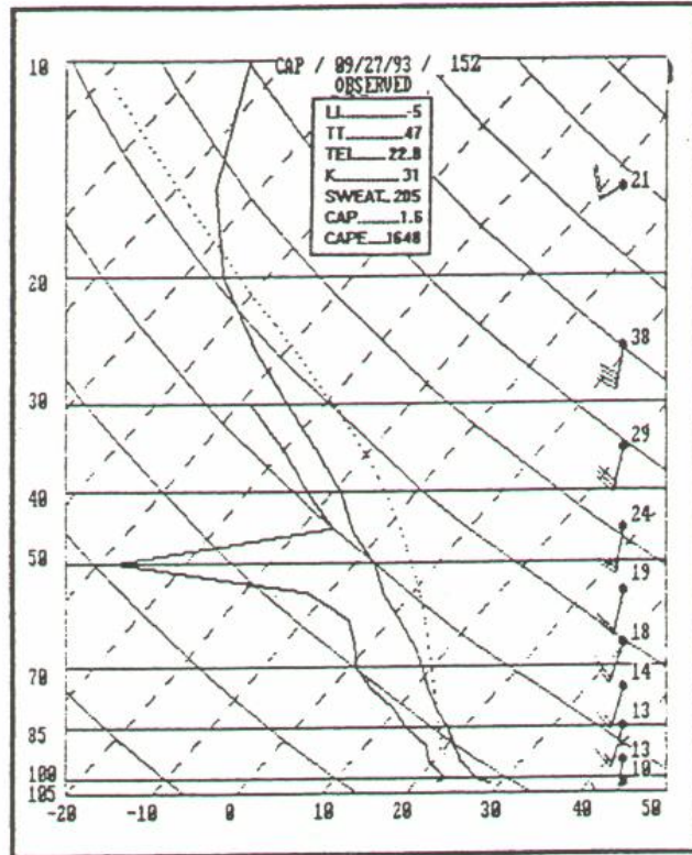
Fig. 16. Cape Canaveral sounding at 1500 UTC September 27, 1993.
