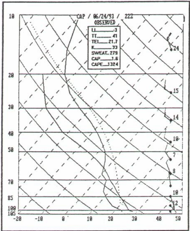
Fig. 4. Cape Canaveral Sounding at 2200 UTC, June 24, 1993.
