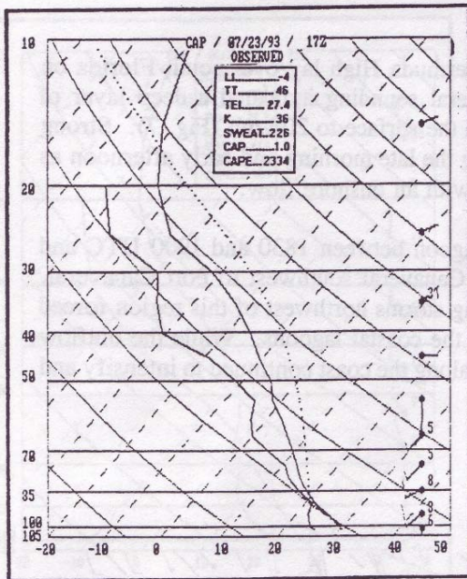
Fig. 7. Cape Canaveral sounding at 1700 UTC July 23, 1993.
