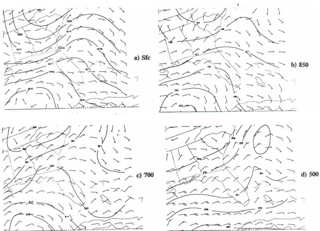
Fig. 12. Same as Fig. 3, except for 1200 UTC August 25, 1993.
