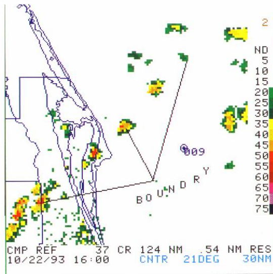
Fig. G1. Composite Reflectivity 1600 UTC, October 22, 1993.
