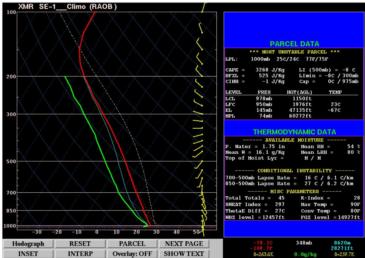
Figure 6. An NSHARP display of the climatological sounding from XMR for the SE-1 flow regime. The temperature profile versus pressure is depicted by the red line, dew point by the green line, and wet-bulb temperature by the blue line. The dashed white line shows the temperature profile of a saturated parcel rising moist adiabatically from 950 mb to 100 mb. The average wind speed and direction profile is shown by the yellow wind barbs on the right-hand-side. The panel on the right-hand-side shows stability parameters and other thermodynamic variables computed from the sounding.
