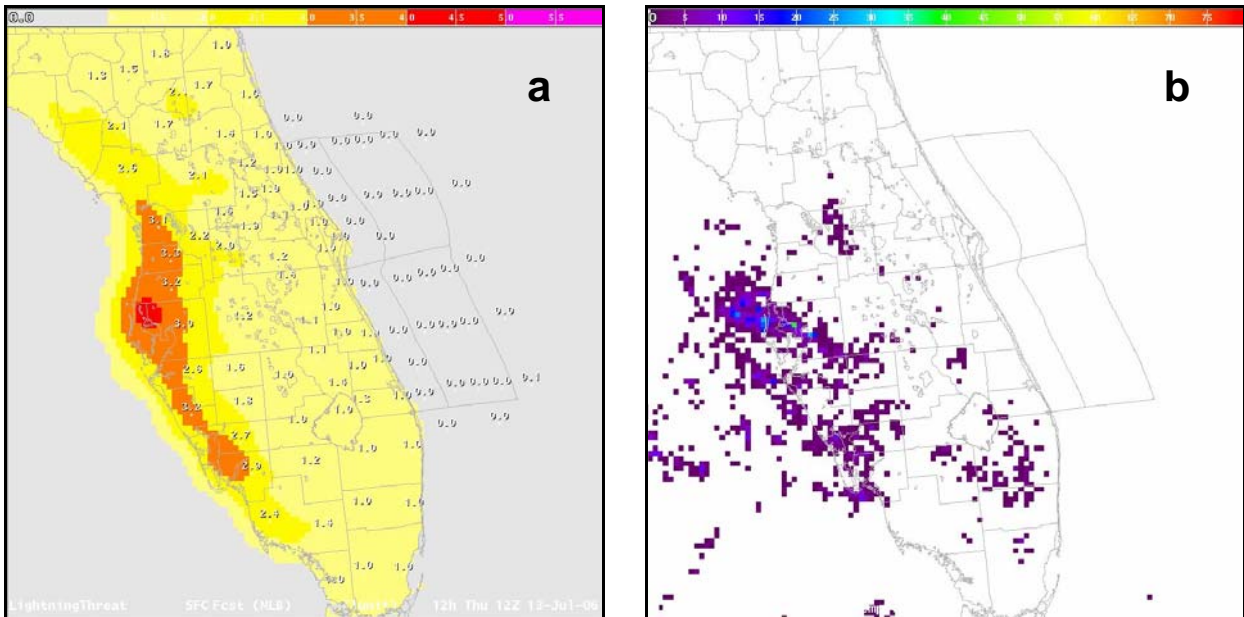
Figure 9. a) The lightning threat index forecast map and b) 5 km gridded lightning density observations from NLDN on 13 July 2006 (# strikes / 5 km 2 / 24 hours).
