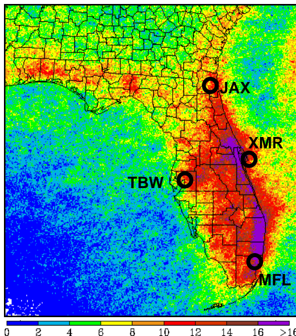
Figure 3. The distribution of daily CG frequencies of occurrence (percent) over Florida for southwest flow in the years 1989-2002 (Stroupe 2003). The locations of the soundings used in this study are indicated by the black circles.
