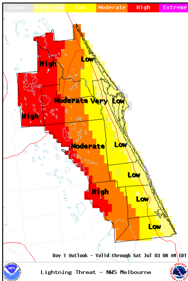
Figure 1. An example of the lightning threat index map issued daily by NWS MLB. The color legend for each threat level is shown at the top of the image.
