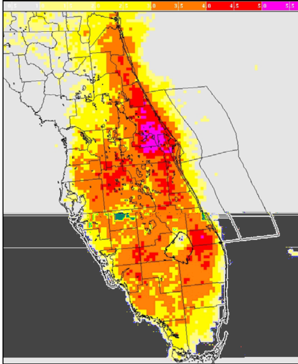
Figure 5. The first-guess lightning threat index map based on the climatological CG density and frequencies in Figure 3.
