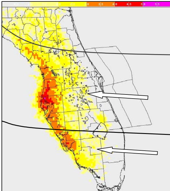
Figure 7. The 1800-2400 UTC climatological lightning probability for the SE-2 flow regime. The scale at the top indicates lower values for grey and light yellow, increasing to the right into the orange, red, and pink. The black lines represent isobars that define the ridge to the north, and the white arrows show the general flow over the peninsula.
