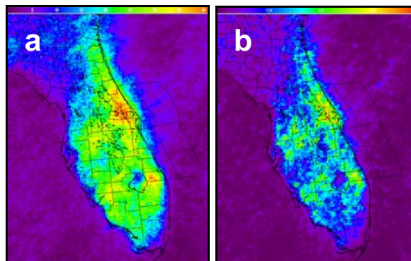
Figure 4. The climatologies of a) CG frequency of occurrence and b) CG density with the ridge axis between Miami and Tampa in the years 1989-2004.
