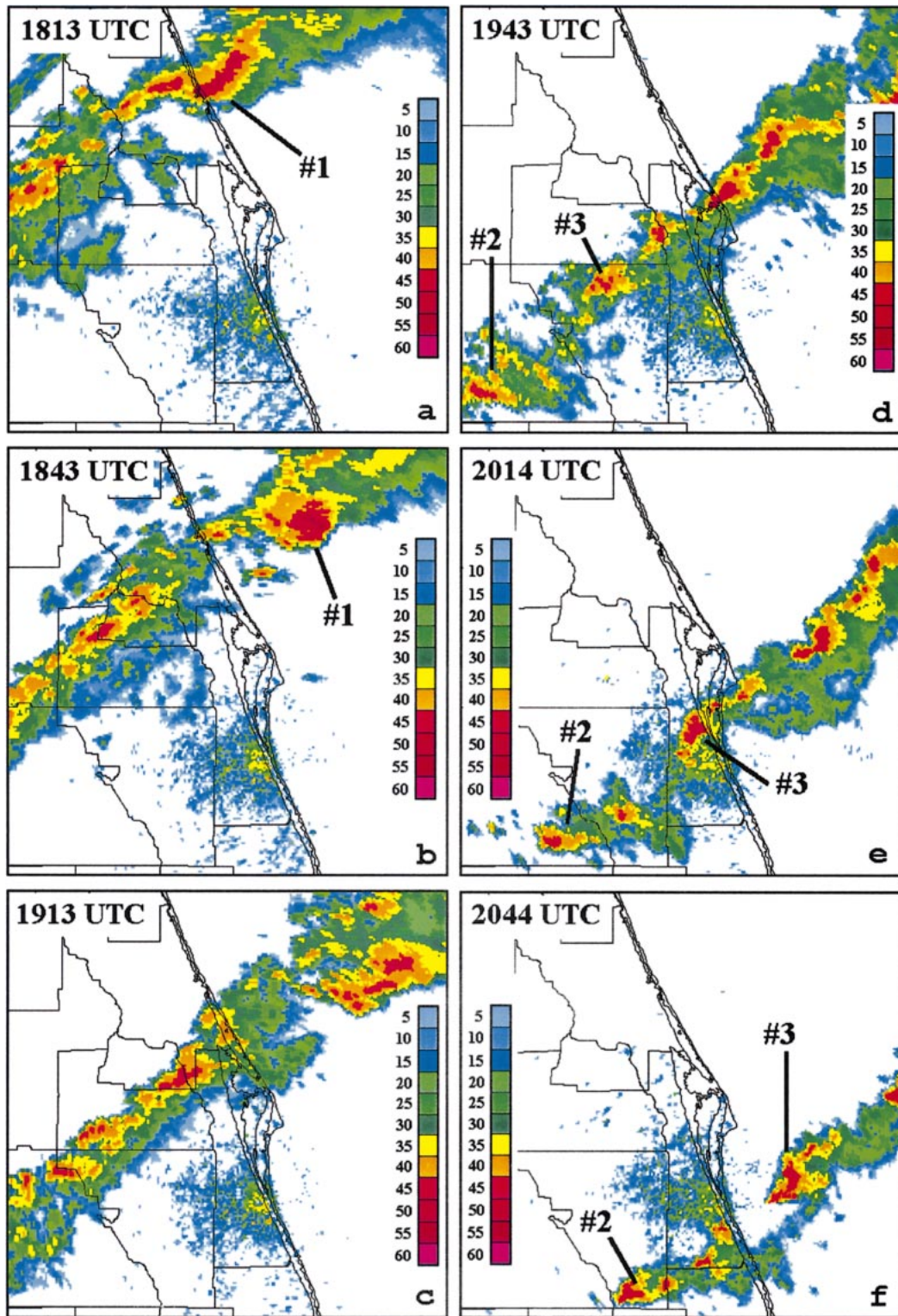
FIG. 7. Base reflectivity images (elevation angle of 0.5^\circ ) from the MLB WSR-88D are shown over east-central Florida from 28 Feb 1999 at the following times: (a) 1813, (b) 1843, (c) 1913, (d) 1943, (e) 2014, and (f) 2044 UTC. Here, #1, #2, and #3 denote three specific cells described in the text.
