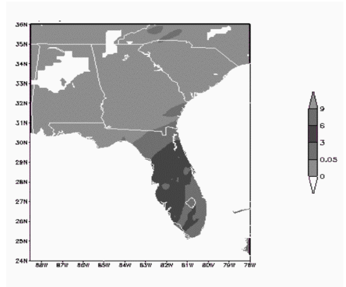
Figure 1. 24-h simulation of accumulated precipitation (convective and non-convective) in inches at 18-km grid beginning 00 UTC 14 September 2001. The initial data for this simulation is the routine FNL available from NCAR.
