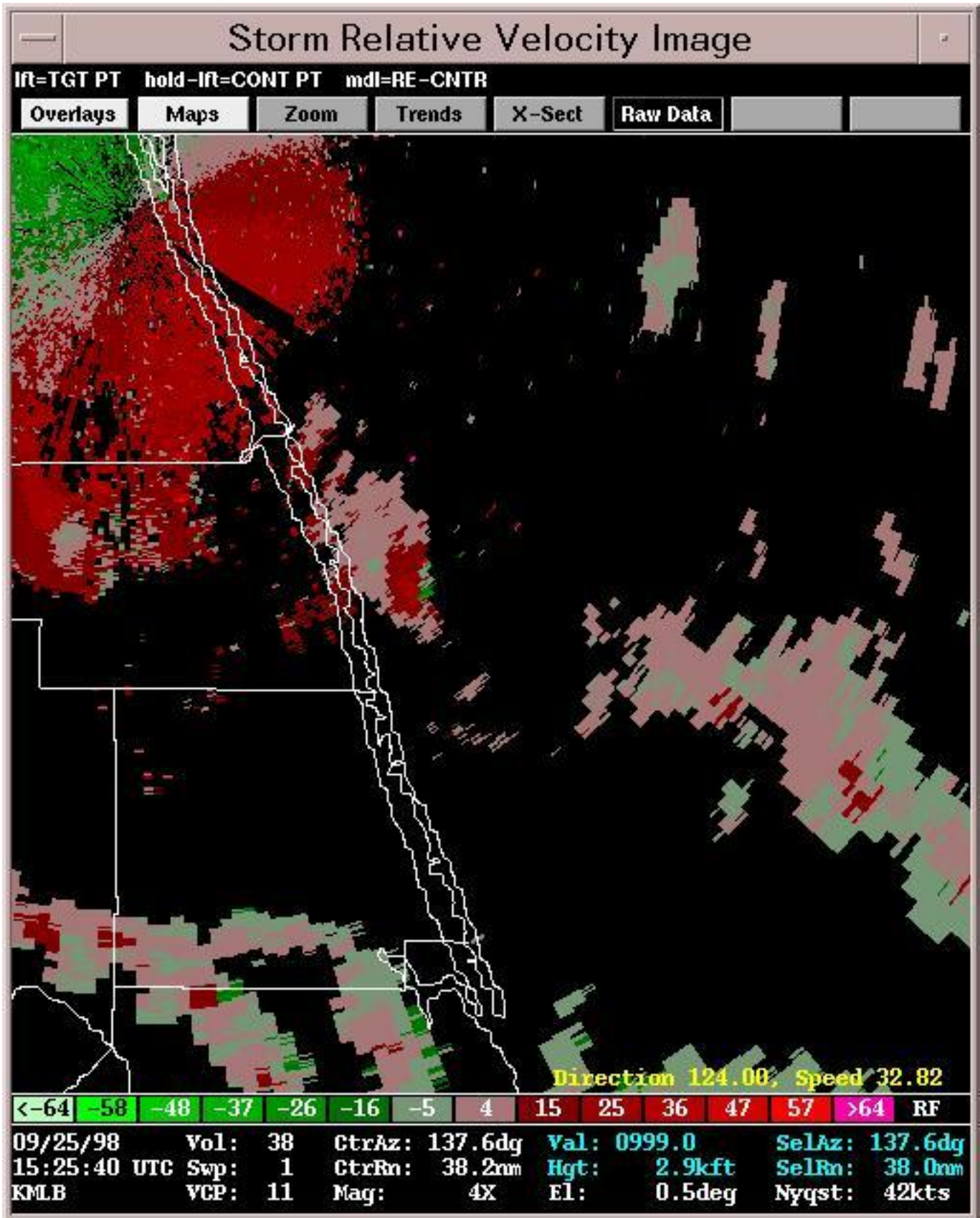
Fig 6b. Storm Relative Velocity image corresponding to Fig. 6a. Note the relatively strong rotation associated with the cell about to move onshore and the weaker circulations with the other cells.
