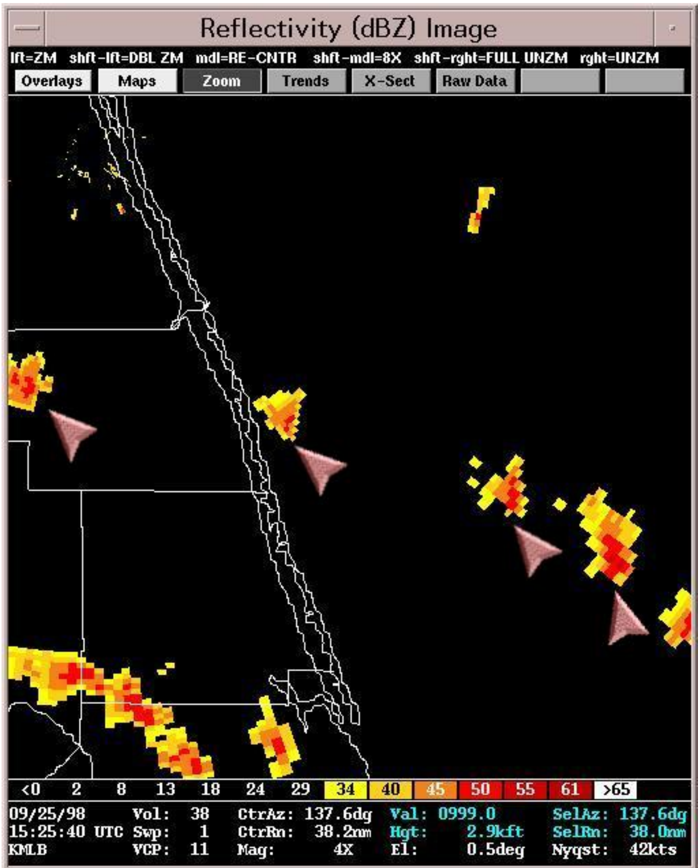
Fig. 6a. Base Reflectivity at 1525 UTC 25 September 1998 indicating scattered heavy showers within a outer rainband associated with TC Georges. The indicated cells exhibited rotation. The cell approaching the coast produced an F0 tornado 30 minutes later (see photograph taken by NWS meteorologist).
