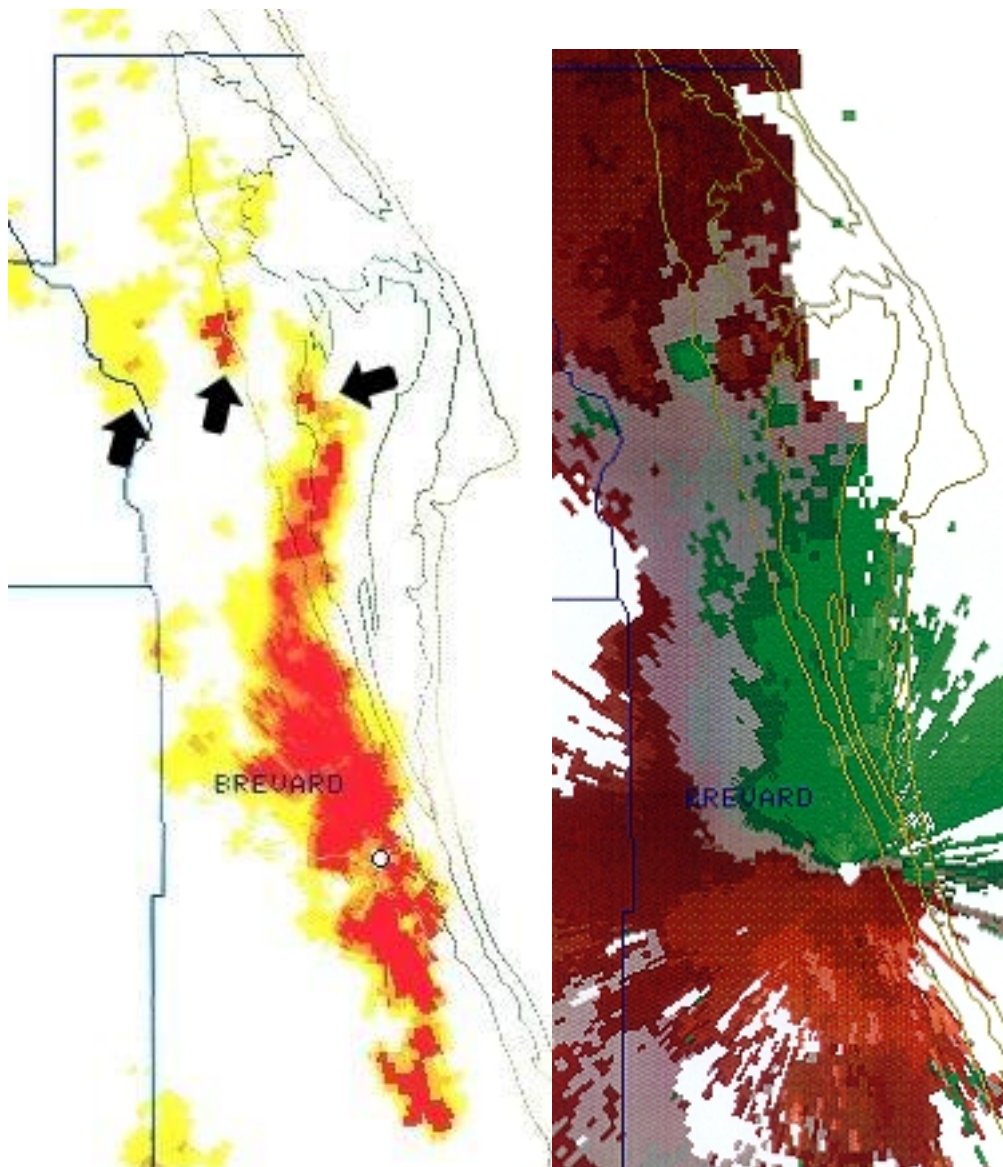
Fig. 3a (left) Boundary on extreme eastern periphery of TC Erin wind field at 1836 UTC 2 August 1995. Meso circulations developed within the stationary band and lifted north, then northwestward through the band. Note the three cells which correlated with persistent rotation. The central one produced several weak tornadoes. Fig. 3b (right) provides a Storm Relative Velocity view of the mesocyclones.
