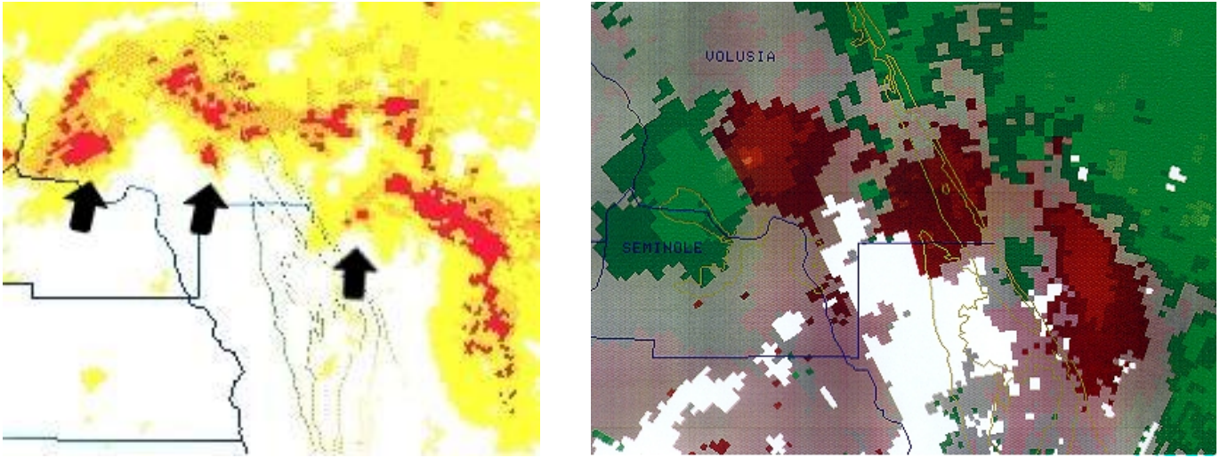
Fig. 1a (left). Dominant rainband (LEWP configuration) associated with TC Gordon at 0900 UTC 16 November 1994. Unobstructed inflow and persistent rotation occurred with each of the cells shown. The westernmost cell produced a brief F0 tornado. Fig. 1b (right). Storm Relative Velocity image corresponding to Fig. 1a. Note the large overall size of the mesocyclones.
