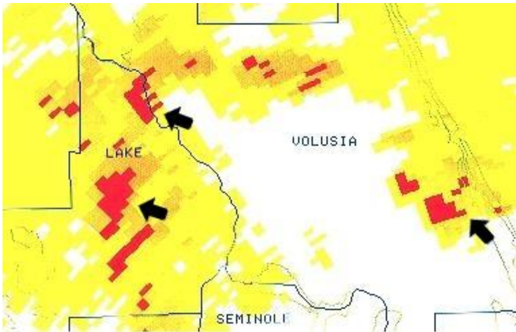
Fig. 5a. Areas of enhanced reflectivity associated with strong low-level mesoscale circulations during TC Josephine at 2117 UTC 7 October 1996. Although all three features began as isolated cells, the two western cells eventually became embedded within surrounding areas of rainfall. At the same time of this image, all three mesocyclones were producing tornadoes. Brief F0 touchdowns occurred in association with the inland cells, while the easternmost cell produced a long-track F2 tornado.
