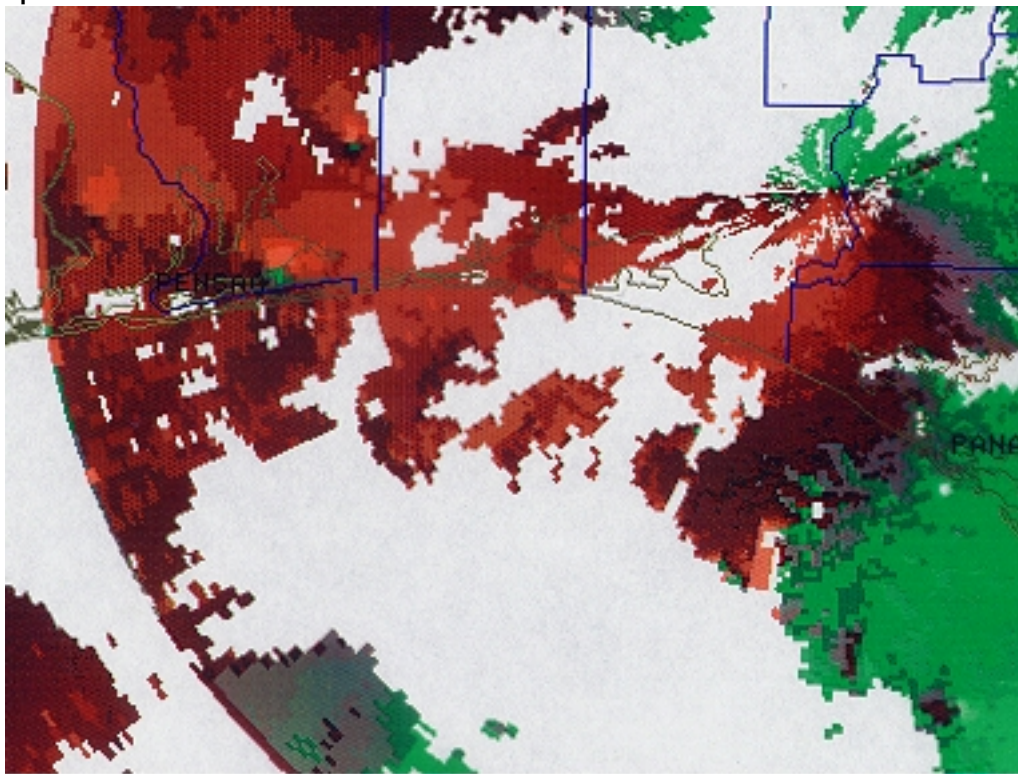
Fig. 4b. Storm Relative Velocity image corresponding to Fig. 4a.
