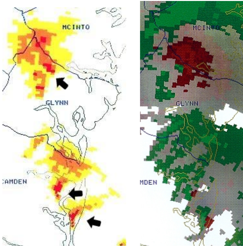
Fig. 2a (left). Isolated high reflectivity cells associated with TC Allison at 0957 UTC 5 June 1995. Classic (mini) hook echoes and persistent rotation occurred with each of the cells shown. The northernmost cell produced a series of tornadoes and the central one produced at least one. Fig. 2b (right). Storm Relative Velocity image corresponding to Fig. 2a.
