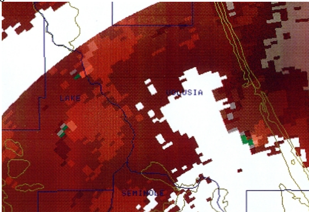
Fig. 5b. Storm Relative Velocity image corresponding to Fig. 5a.
