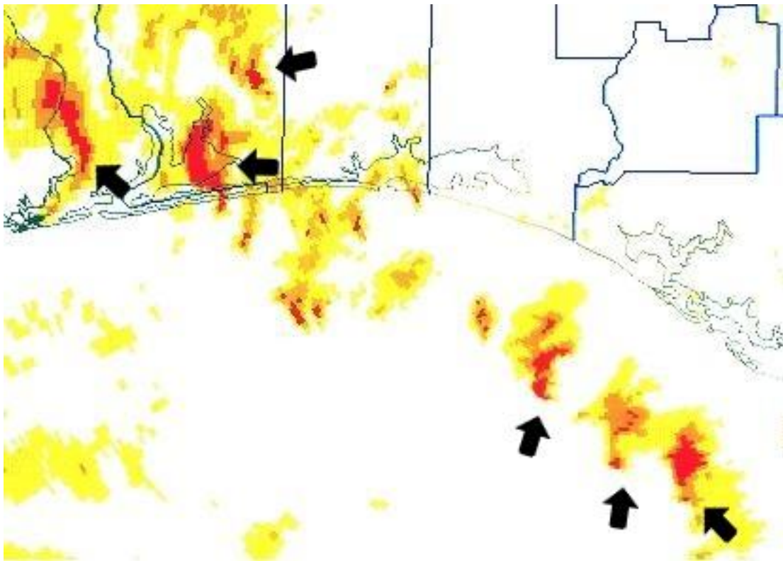
Fig. 4a. Numerous high reflectivity isolated cells associated with TC Opal at 1548 UTC 4 October 1995. Classic hook echoes and strong, persistent rotation occurred with each of the cells shown. Many of the circulations lasted for more than 2 h and exhibited rotational velocities above 17 m/s averaged over the lifetime of the cell. Depths were much greater than typical TC mini-supercells.
