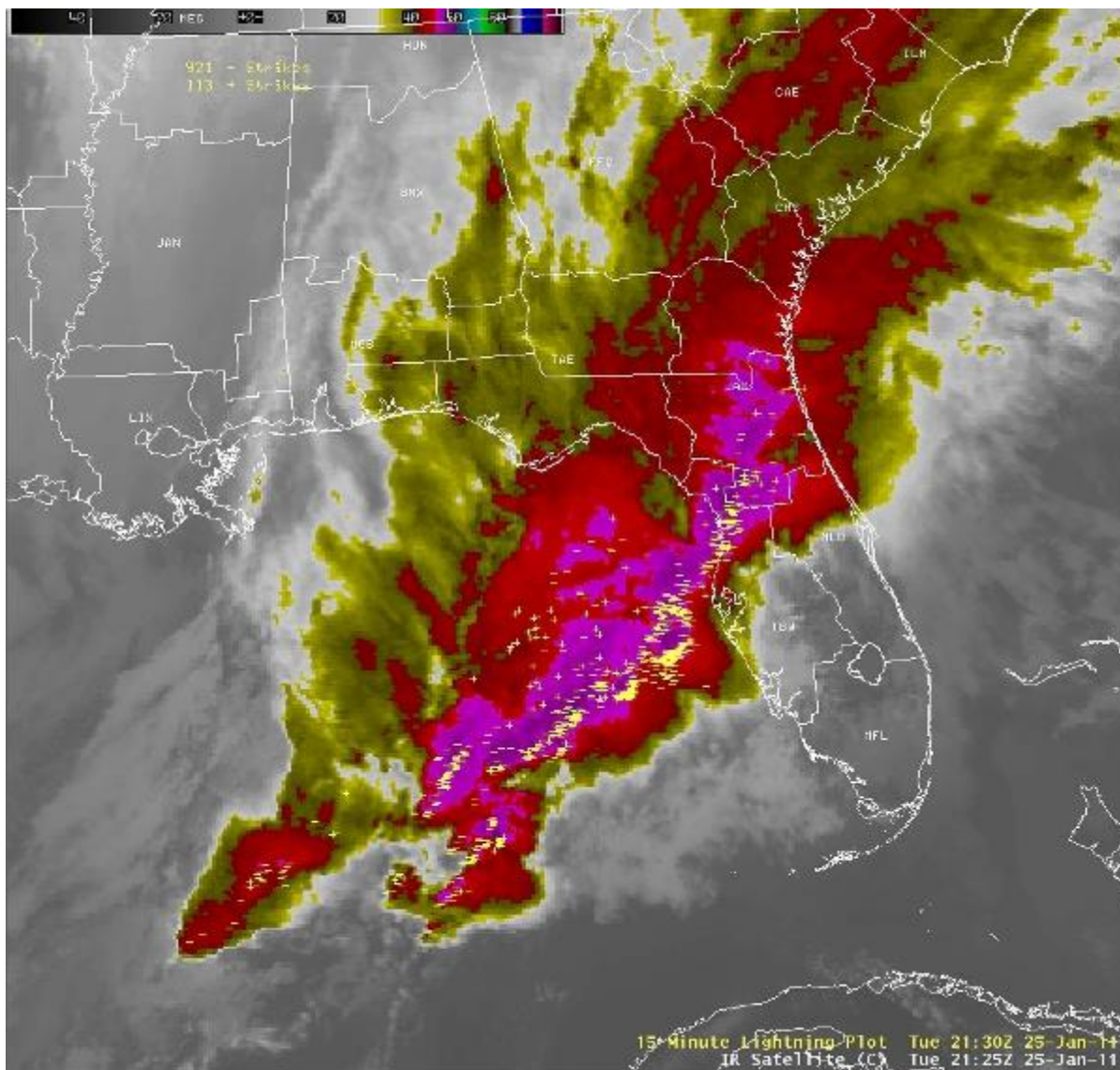
IR Satellite Imagery at 425 PM EST on January 25, 2011.
