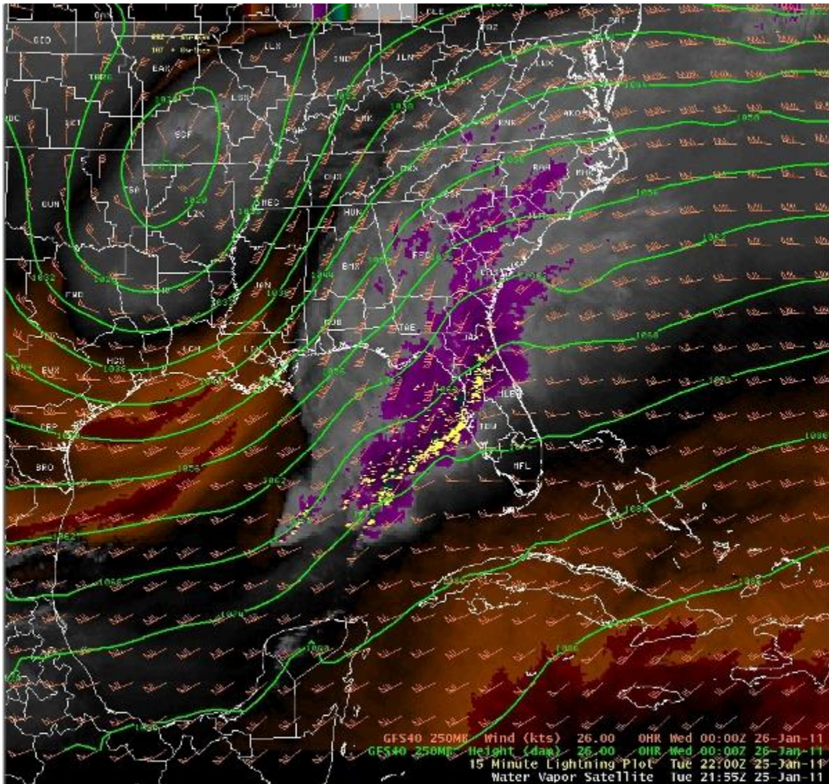
Water Vapor Imagery and upper level winds at 455 PM EST January 25 2011.
