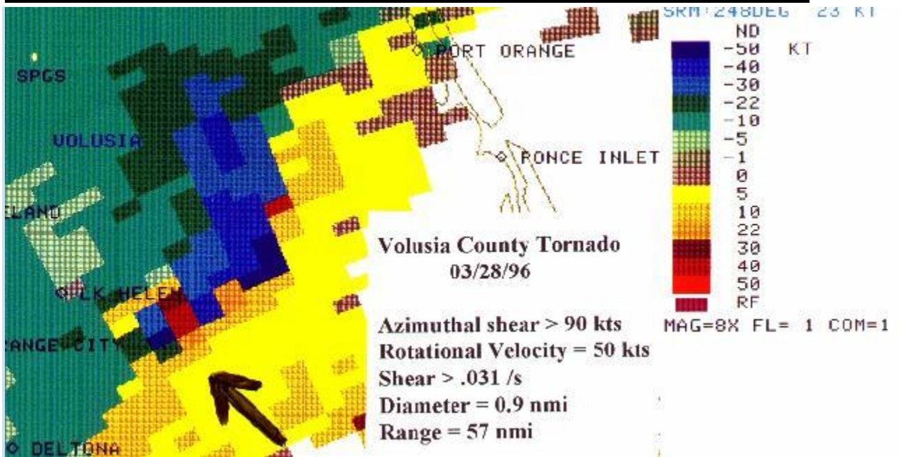
Storm relative velocity display of mesocyclone over southern Volusia County. Arrow points to area of potential tornado.(srm/.5 deg/2132z)
