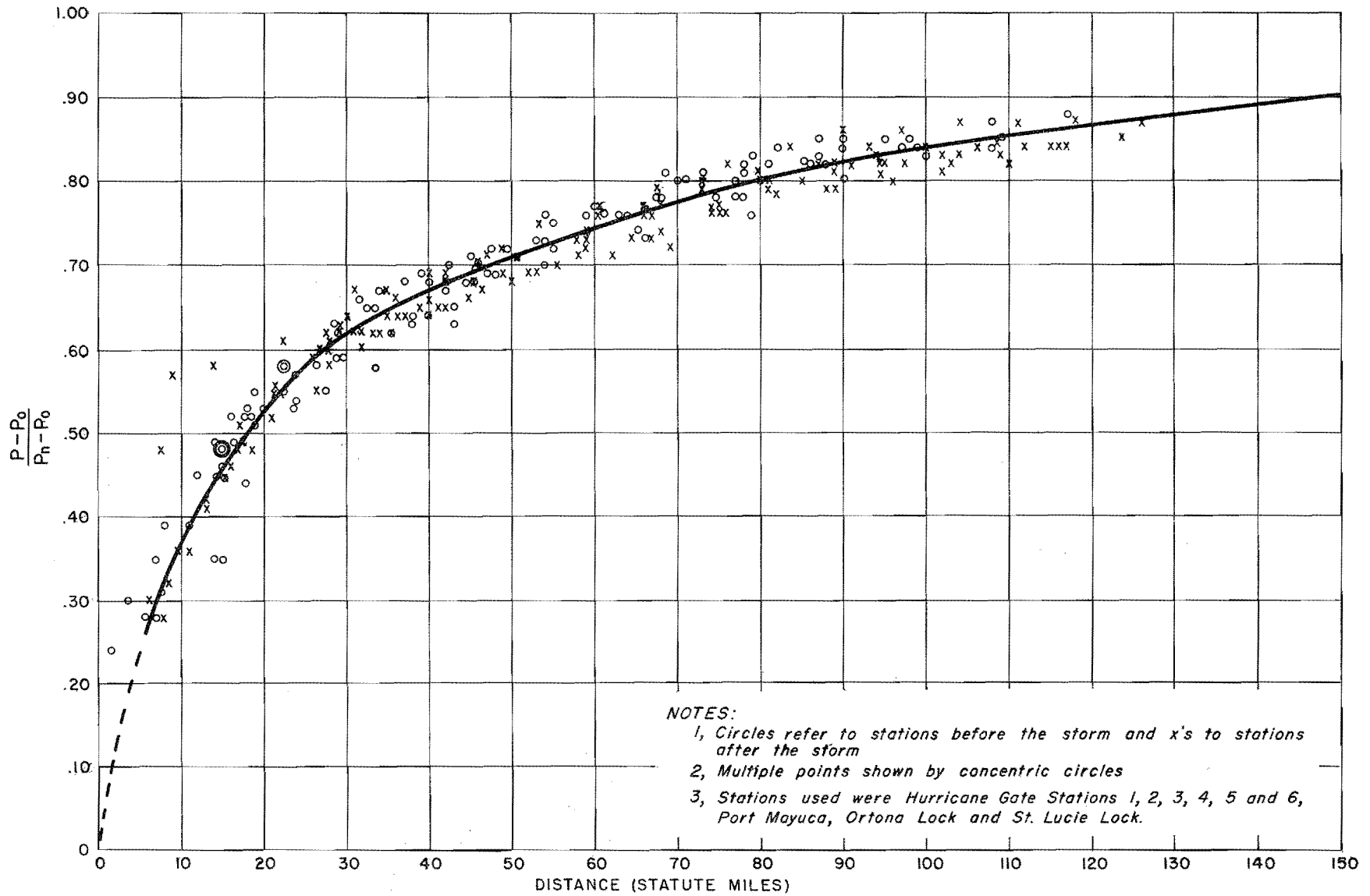
PARAMETRIC PRESSURE PROFILE, STORM OF OCTOBER 17-18, 1950
