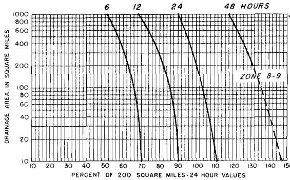
FIGURE 6 SEASONAL VARIATION DEPTH-AREA-DURATION RELATIONSHIPS Percentage to be applied to 200 square miles 24 hour probable maximum precipitation values for: FEBRUARY
