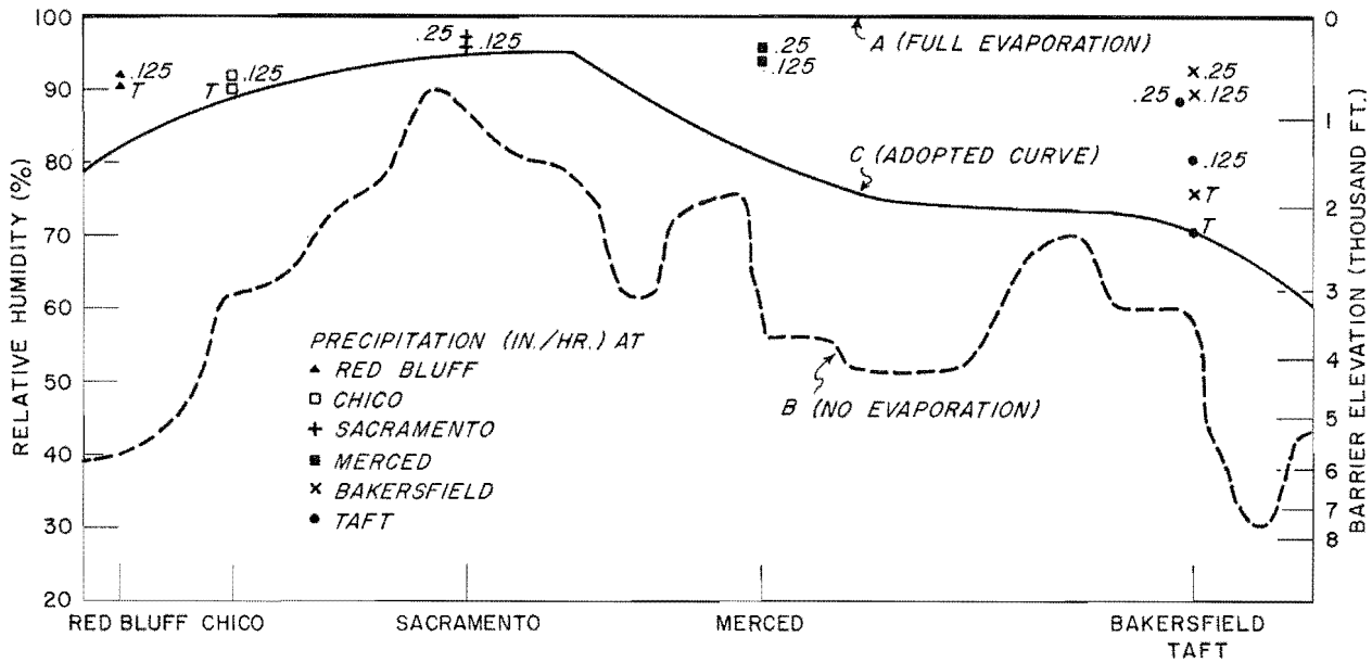
FIG. 5-8. CENTRAL VALLEY DEGREE-OF-SATURATION FOR PMP CONDITIONS
