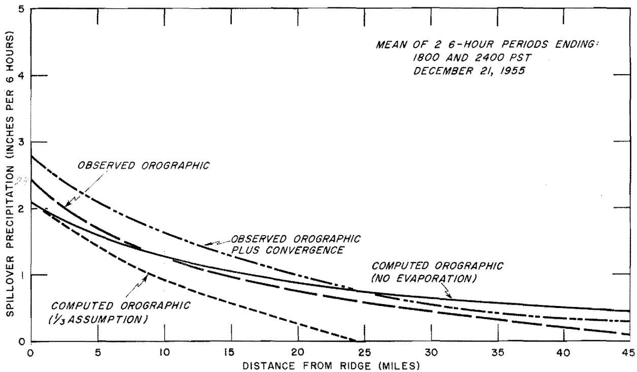
FIG. 6-4. SPILLOVER COMPARISON - COASTAL (See figure 5-15)
