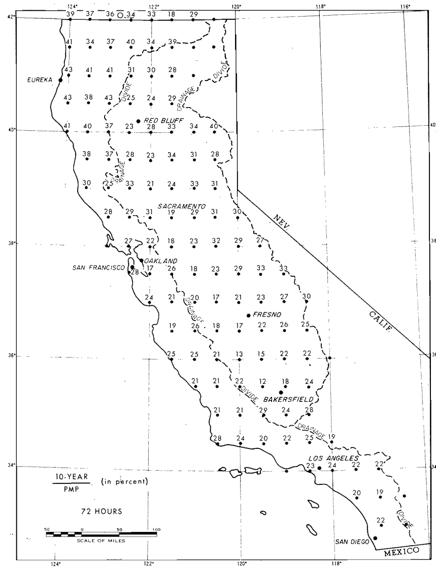
FIG. 8-11. RATIO OF 10-YEAR 72-HOUR PRECIPITATION TO 10-SQUARE-MILE 72-HOUR PMP
