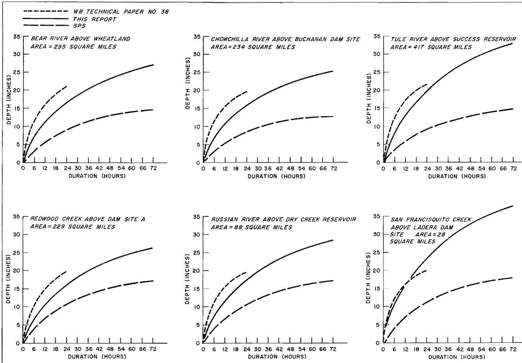
FIG. 8-12. COMPARISON OF PMP FROM W. B. TECHNICAL PAPER NO. 38 WITH PMP FROM THIS REPORT AND STANDARD PROJECT STORM (SPS), FOR SELECTED BASINS
