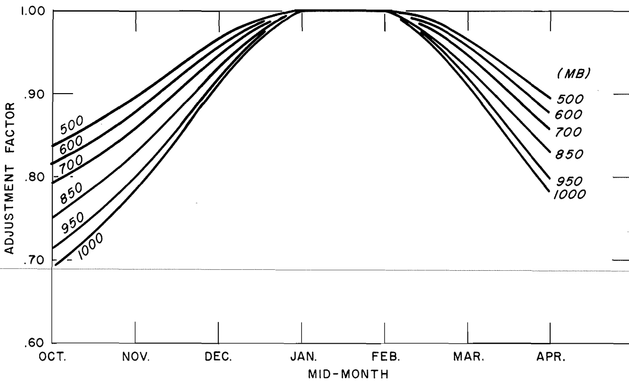
FIG. 5-37. SEASONAL VARIATION OF MAXIMUM WINDS
