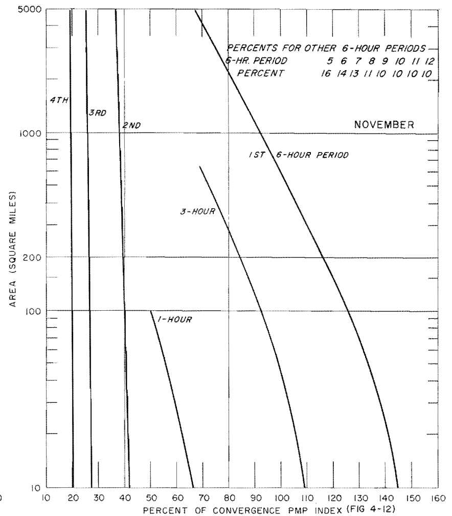
FIG. 4-13a. VARIATION OF CONVERGENCE PMP WITH BASIN SIZE AND DURATION
