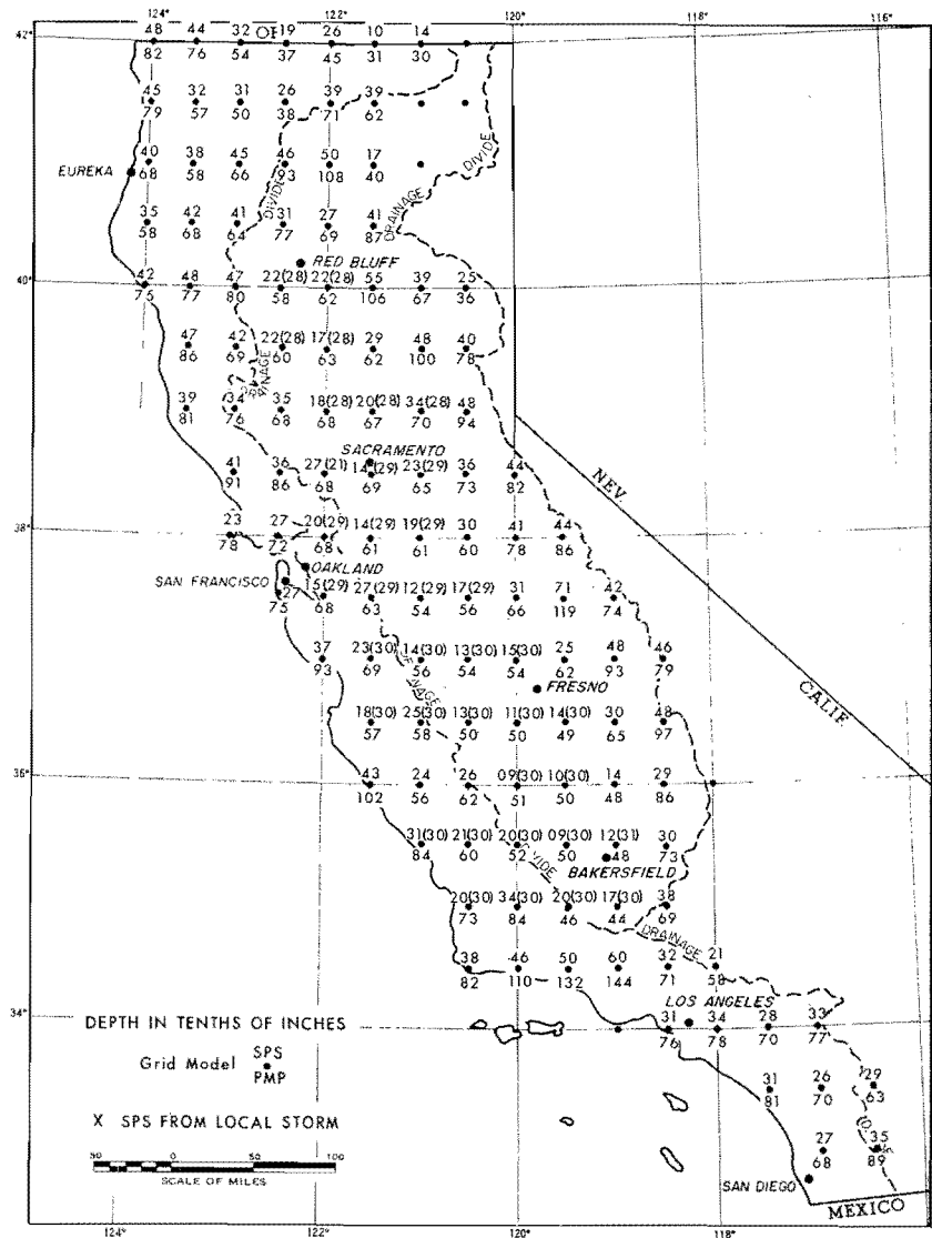
FIG. 8-6. COMPARISON OF SPS AND PMP FOR 6 HOURS AND 200 SQUARE MILES
