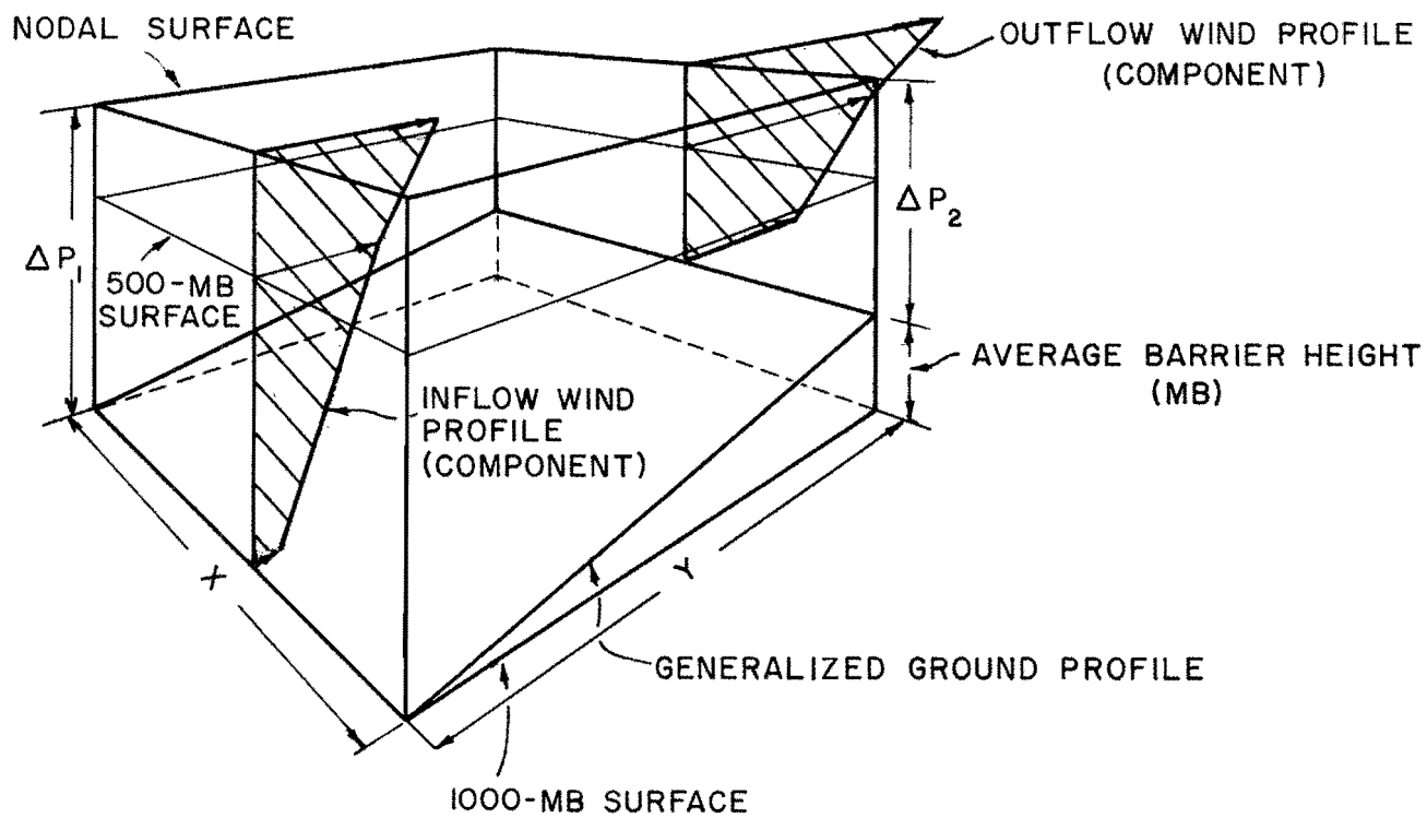
FIG. 5-1. SCHEMATIC INFLOW AND OUTFLOW WIND PROFILES OVER MOUNTAIN BARRIER
