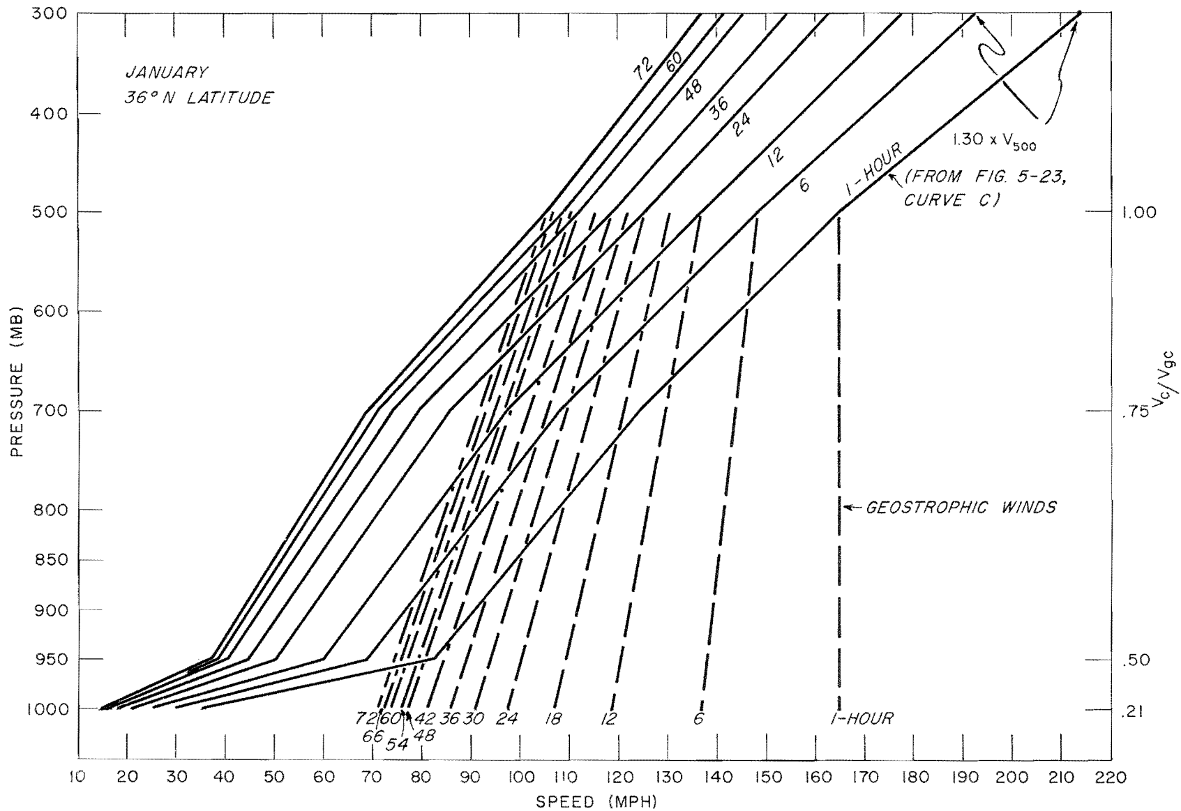
FIG. 5-26. ADOPTED MAXIMUM WINDS NORMAL TO COAST RANGE
