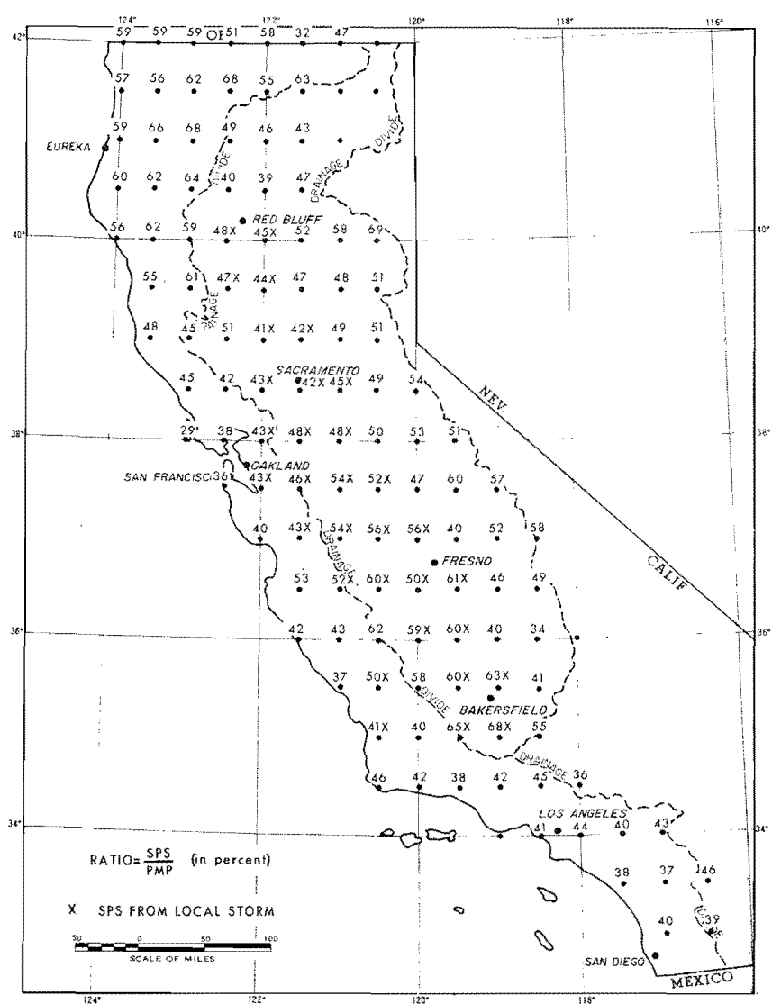
FIG. 8-6. COMPARISON OF SPS AND PMP FOR 6 HOURS AND 200 SQUARE MILES
