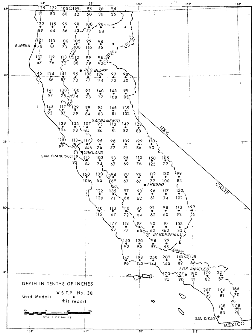
FIG. 8-14. COMPARISON OF PMP FROM W. B. TECHNICAL PAPER NO. 38 WITH THIS REPORT FOR 6 HOURS AND 10 SQUARE MILES
