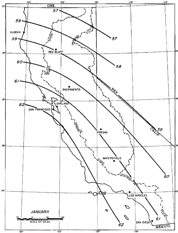
FIG. 4-5a. ENVELOPING 12-HOUR PERSISTING 1000-MB DEW POINT MAPS (°F)
