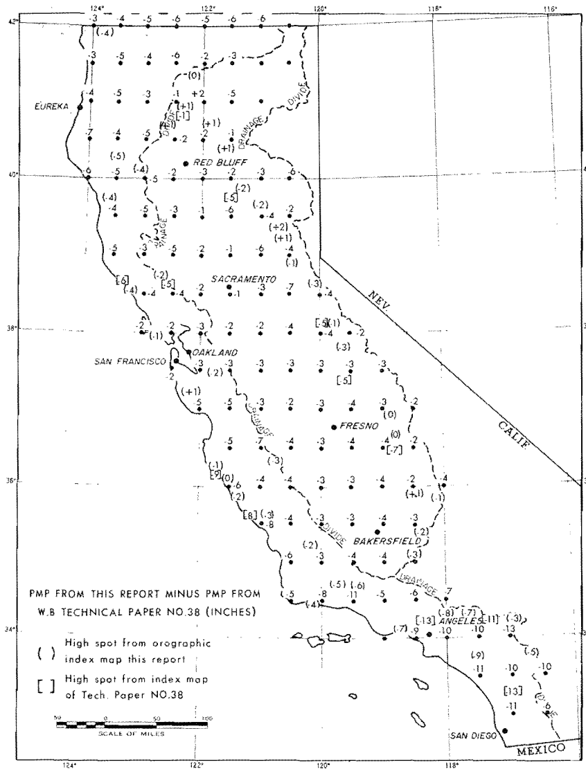
FIG. 8-14. COMPARISON OF PMP FROM W. B. TECHNICAL PAPER NO. 38 WITH THIS REPORT FOR 6 HOURS AND 10 SQUARE MILES
