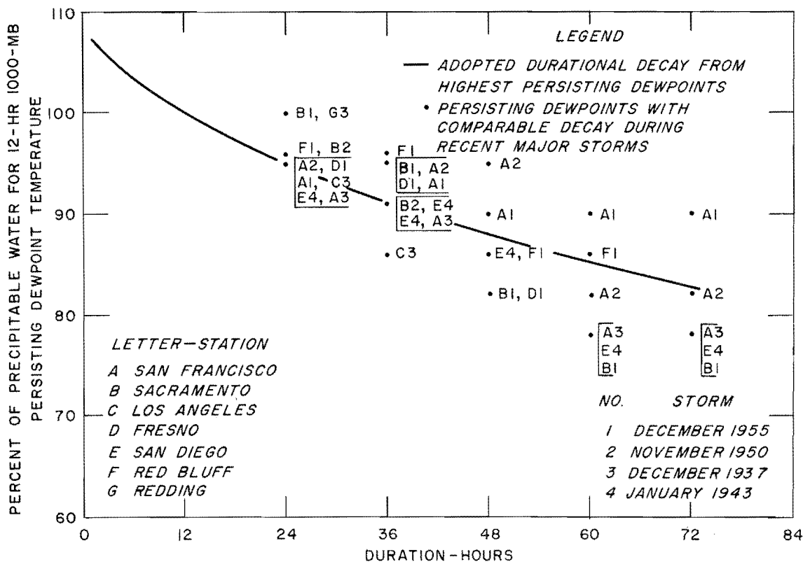
FIG. 4-4. COMPARISON OF OBSERVED AND ADOPTED MOISTURE DECAYS
