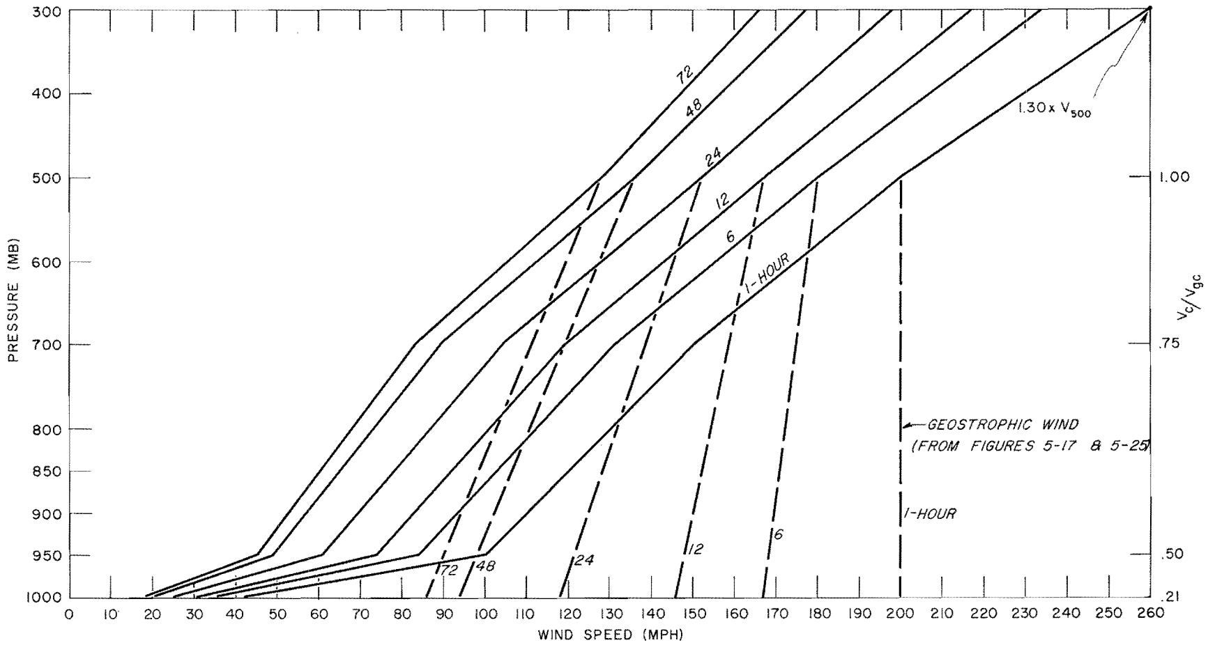
FIG. 5-19. GEOSTROPHICALLY-DERIVED MAXIMUM WINDS, COASTAL
