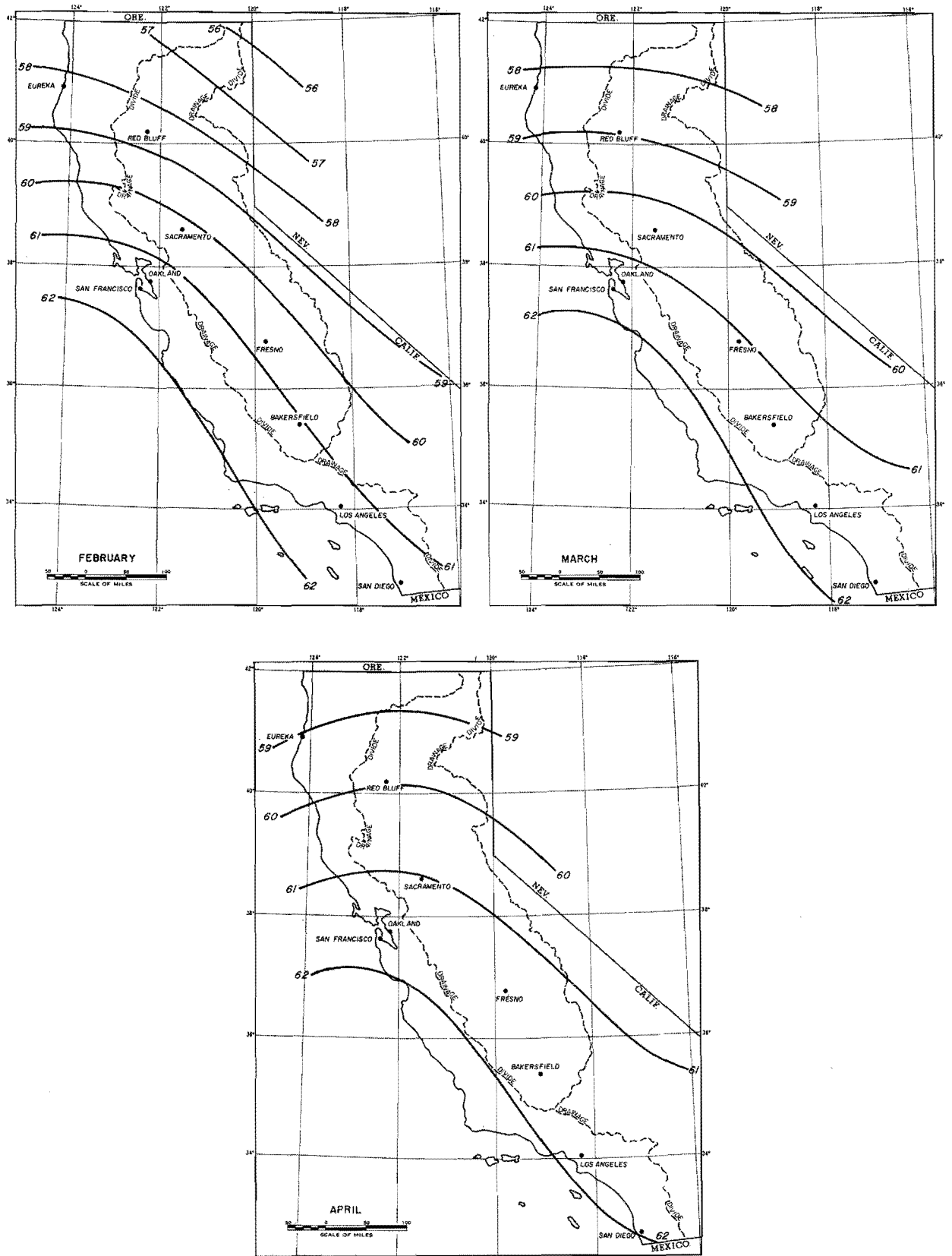
FIG. 4-5b. ENVELOPING 12-HOUR PERSISTING 1000-MB DEW POINT MAPS (°F) (CONT'D)
