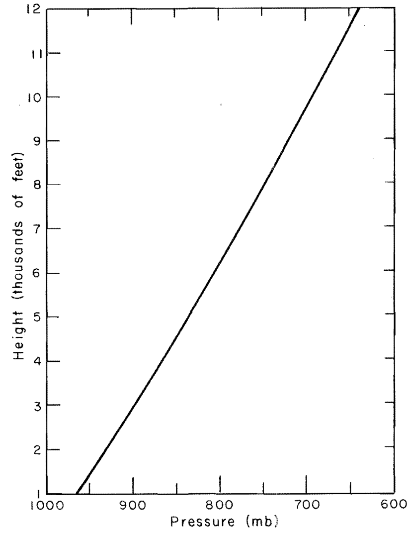
FIG. 10-4. PRESSURE-HEIGHT RELATION
