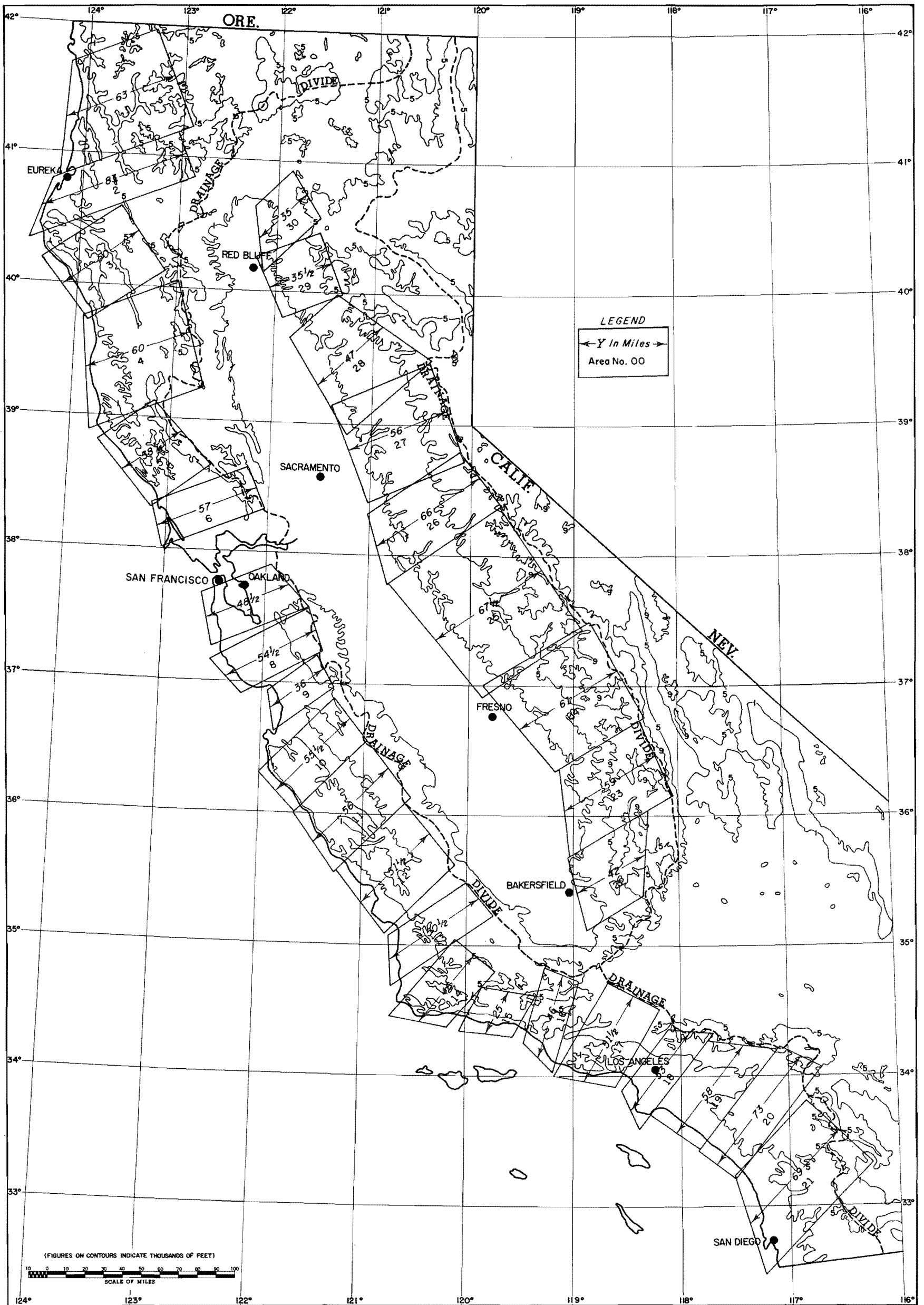
FIG. 5-30. OROGRAPHIC PMP COMPUTATION AREAS
