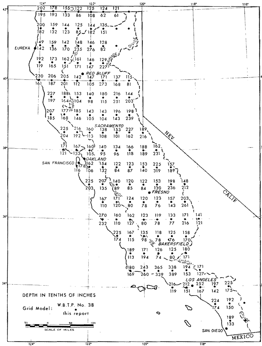
FIG. 8-13. COMPARISON OF PMP FROM W.B. TECHNICAL PAPER NO. 38 WITH THIS REPORT FOR 24 HOURS AND 200 SQUARE MILES
