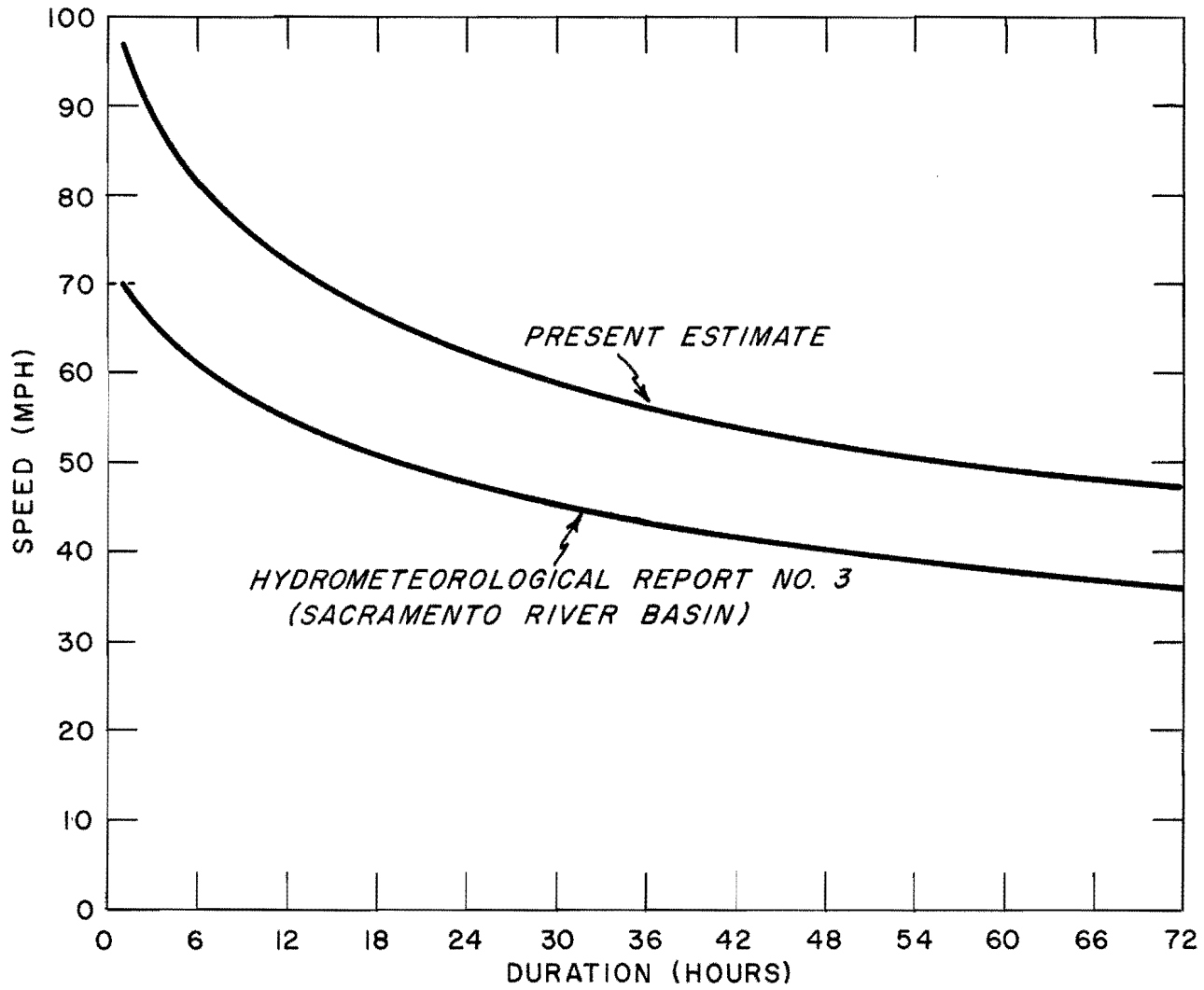
5-28. MAXIMUM 4000-FOOT WINDSPEED COMPARISON, COASTAL
