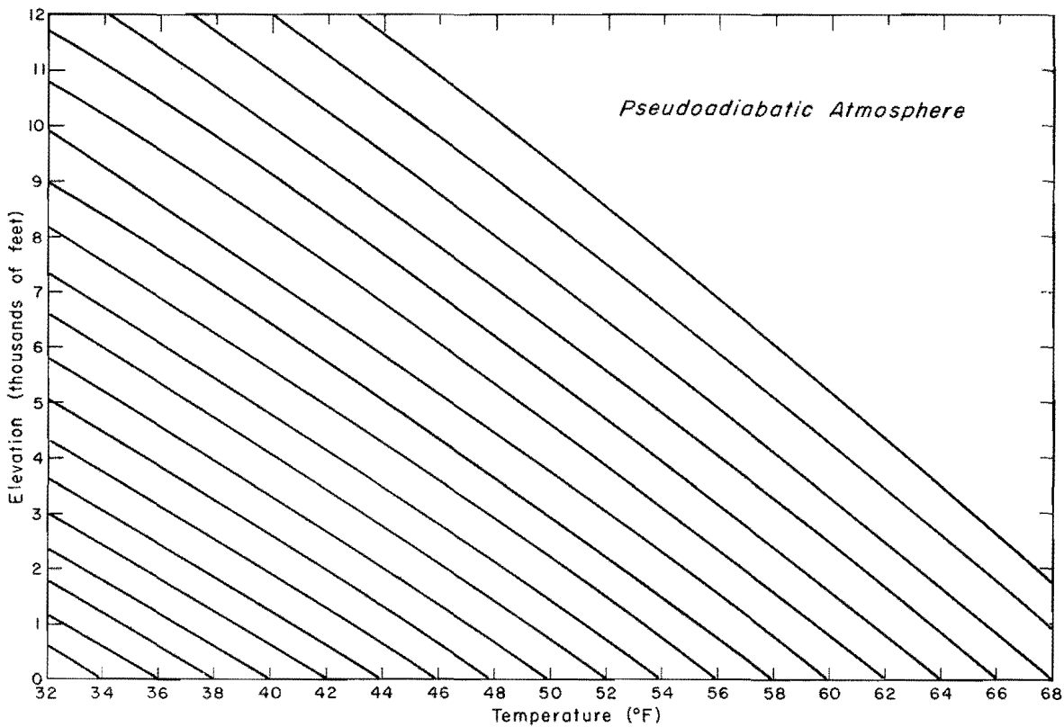
FIG. 10-2. DECREASE OF TEMPERATURE WITH ELEVATION
