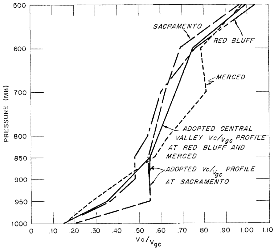
FIG. 5-4. CENTRAL VALLEY V_c/V_{gc} PROFILES
