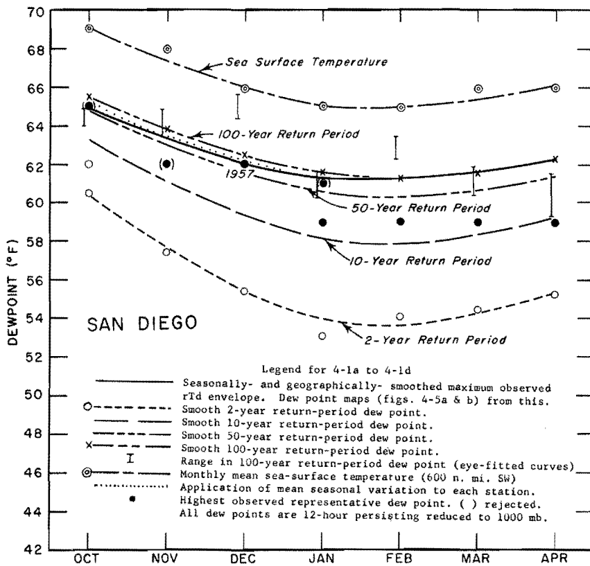
FIG. 4-1a. SEASONAL ENVELOPE OF MAXIMUM OBSERVED DEW POINTS
