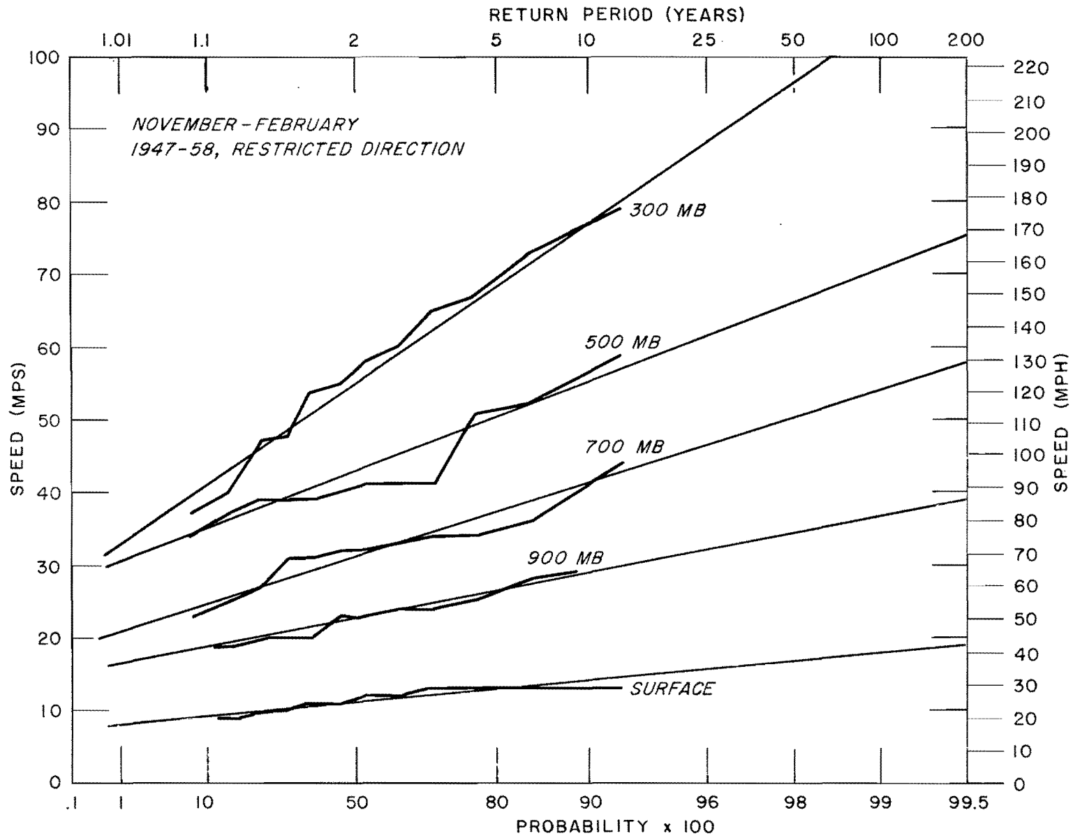
FIG. 5-20. MAXIMUM WINDS ALOFT, OAKLAND, CALIFORNIA
