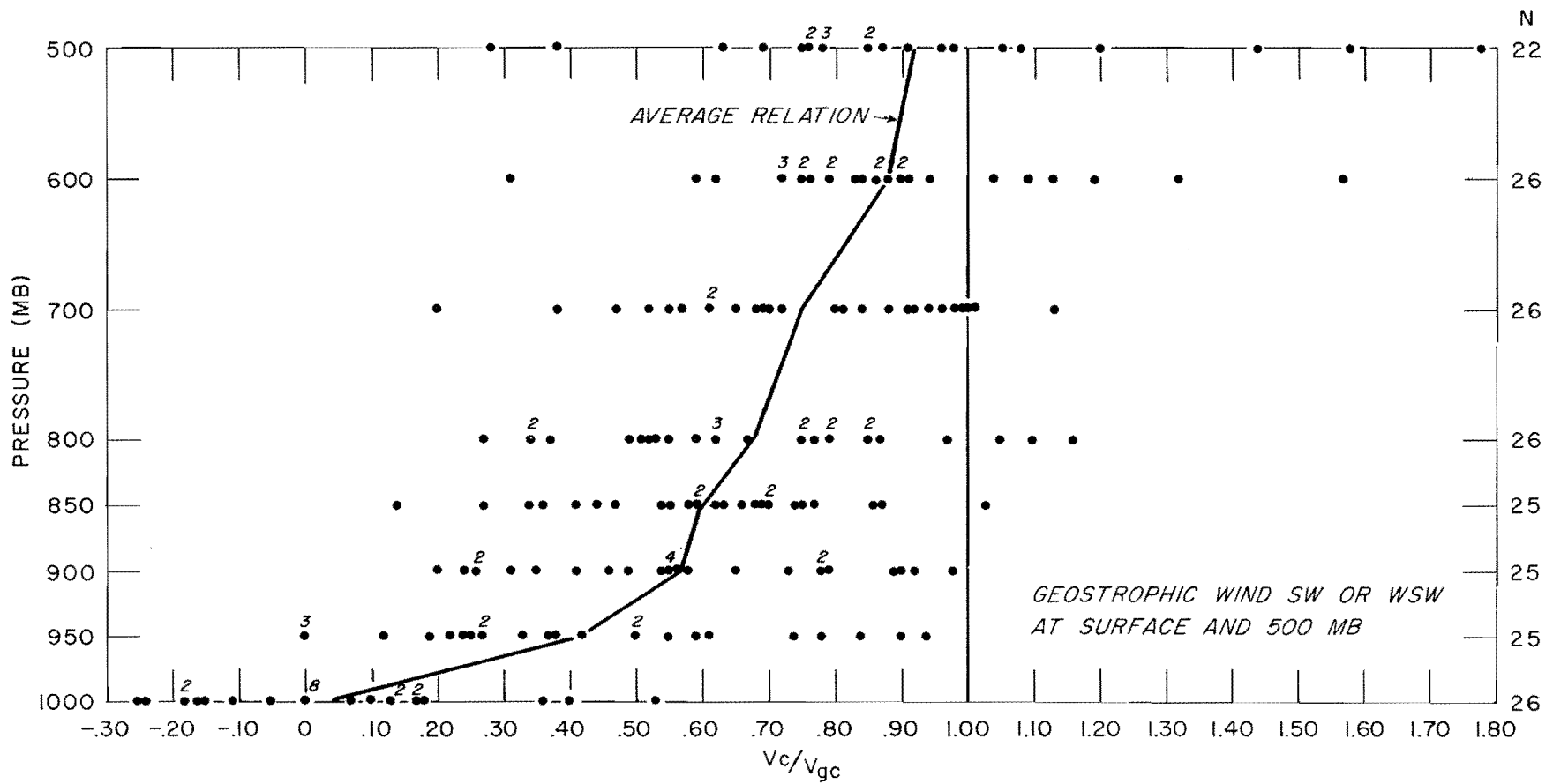
FIG. 5-2. AVERAGE RATIO OF OBSERVED, V_c , TO GEOSTROPHIC WIND COMPONENT, V_{gc} , OAKLAND, CALIFORNIA
