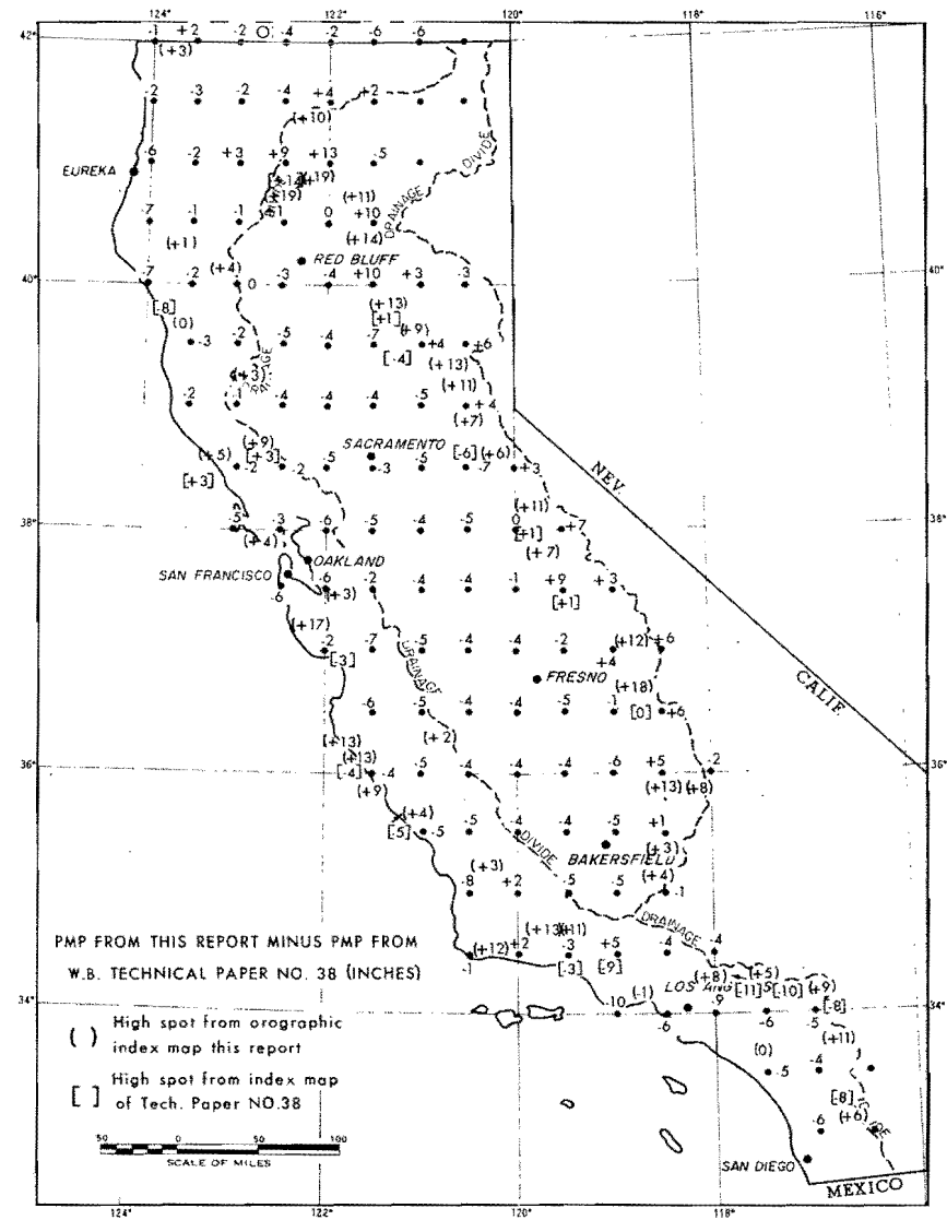
FIG. 8-13. COMPARISON OF PMP FROM W.B. TECHNICAL PAPER NO. 38 WITH THIS REPORT FOR 24 HOURS AND 200 SQUARE MILES
