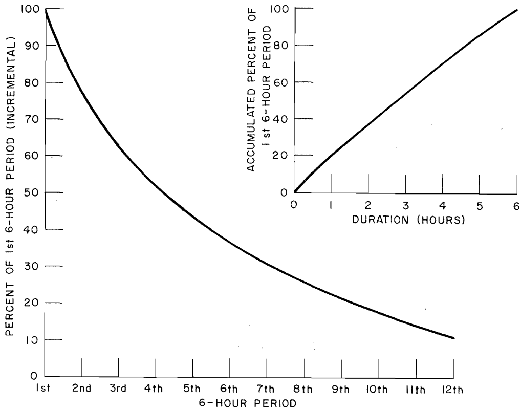
FIG. 5-36. VARIATION OF OROGRAPHIC PMP WITH DURATION
