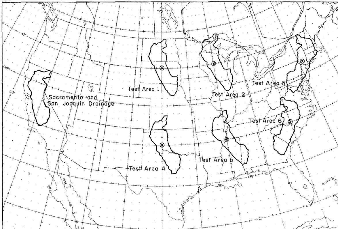
FIG. 8-1. TEST AREAS FOR COMPARISON OF STORM VALUES WITH PMP
