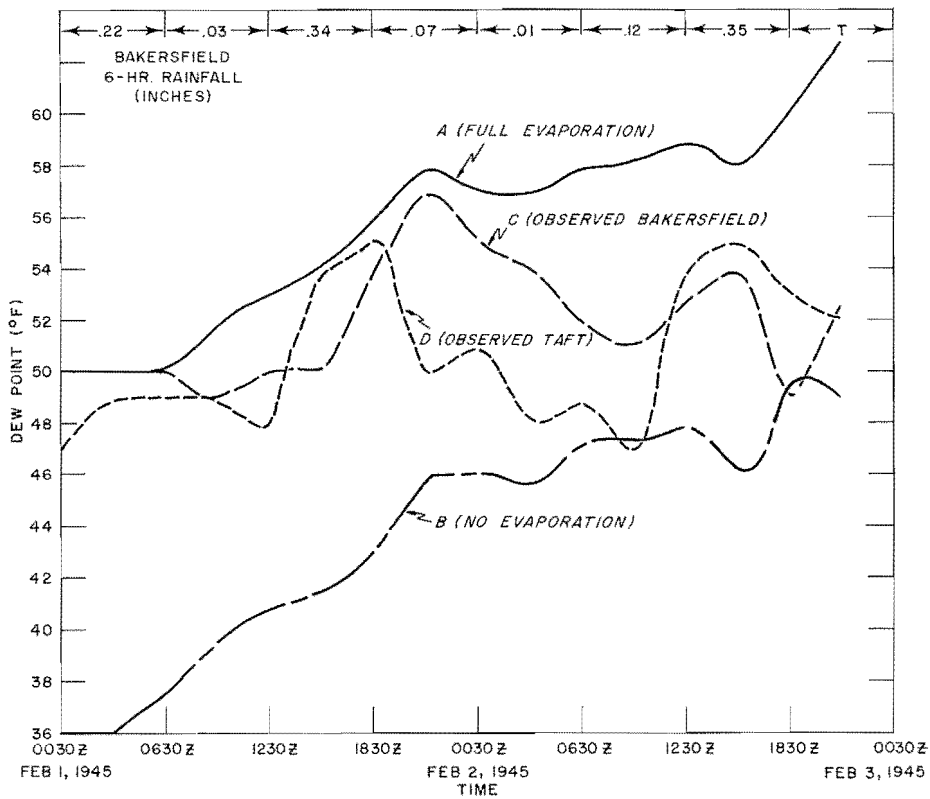
FIG. 5-9. SAN JOAQUIN VALLEY DEW-POINT VARIATIONS
