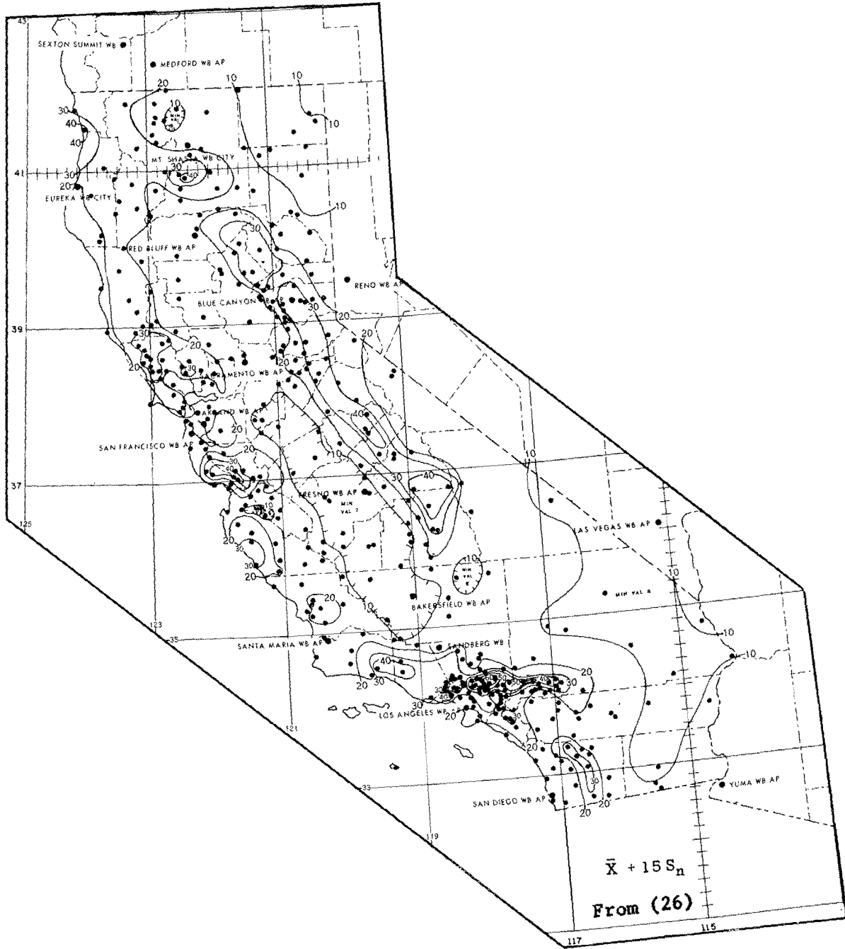
FIG. 8-3. STATISTICAL PMP FOR 24 HOURS AT A POINT, CALIFORNIA
