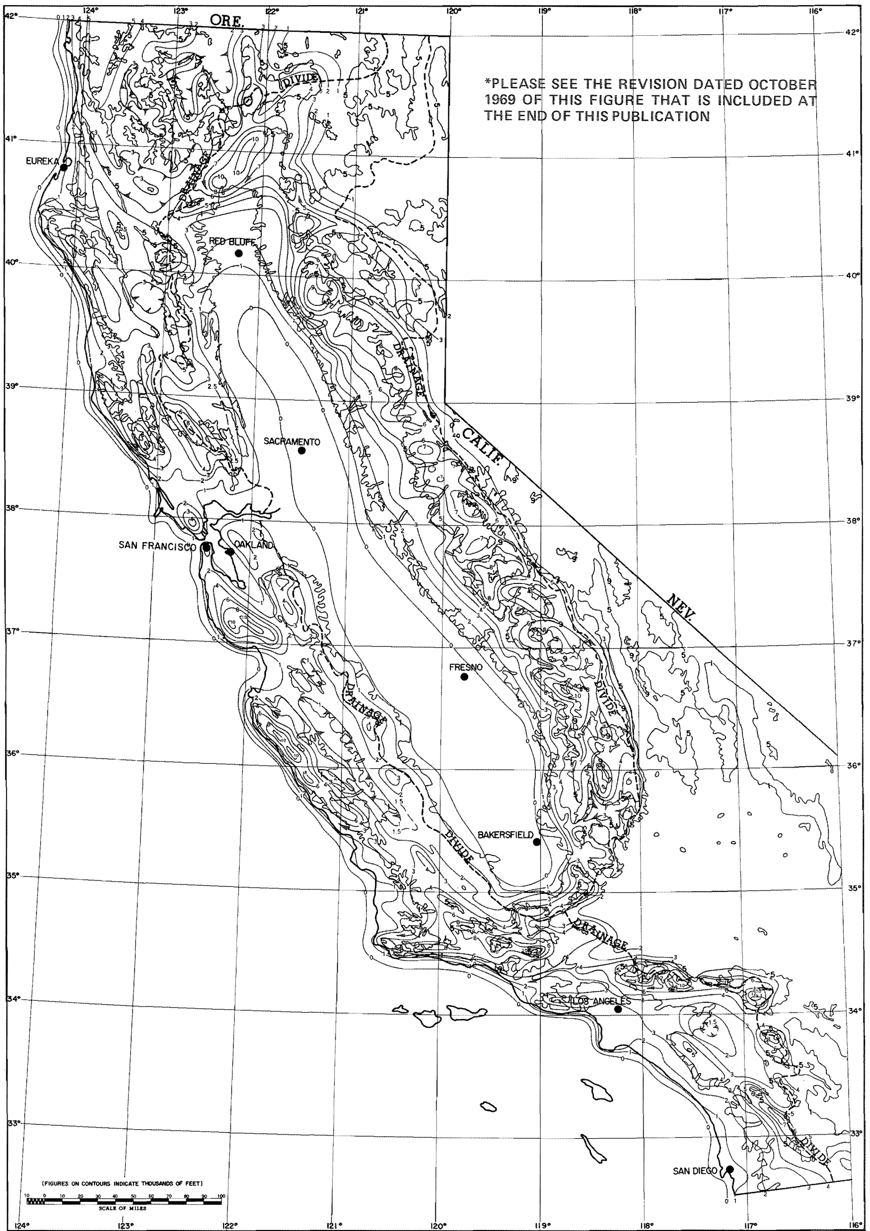
FIG. 5-35. OROGRAPHIC PMP INDEX. 6-HR JANUARY (inches)
