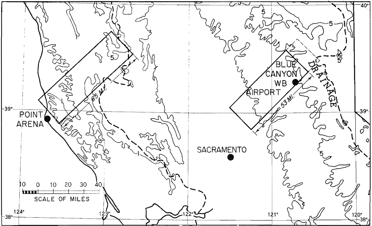
FIG. 5-15. PRECIPITATION-DISTRIBUTION TEST AREAS
