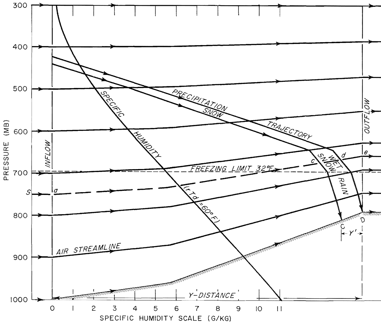
FIG. 5-11. SCHEMATIC DIAGRAM OF OROGRAPHIC MODEL
