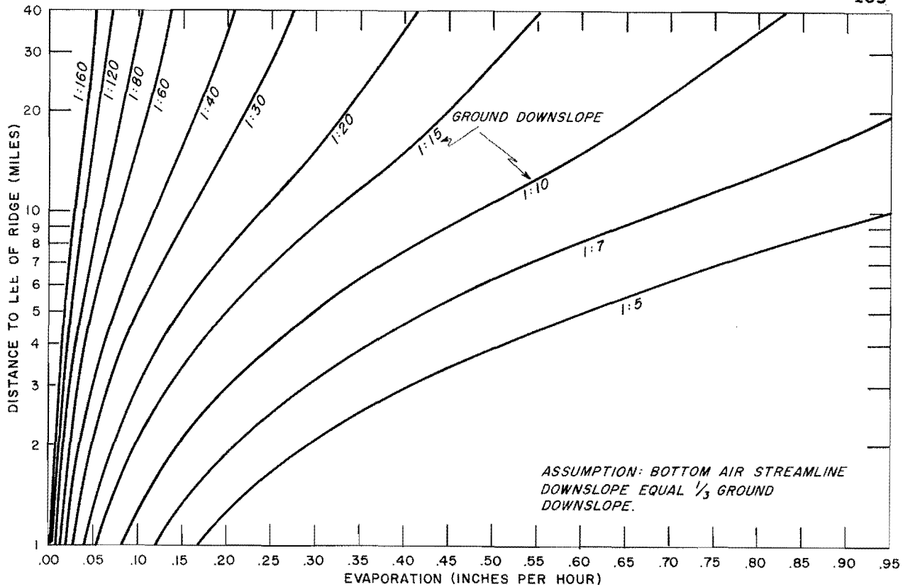
FIG. 6-3. LEEWARD EVAPORATION
