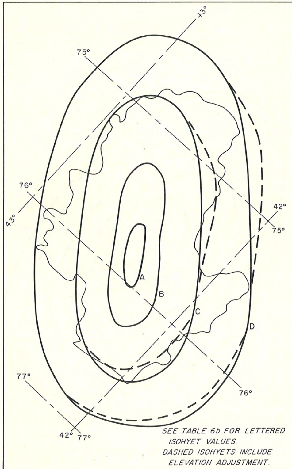
Fig. 13b. Pattern storm for Susquehanna River at Waverly, N. Y.
