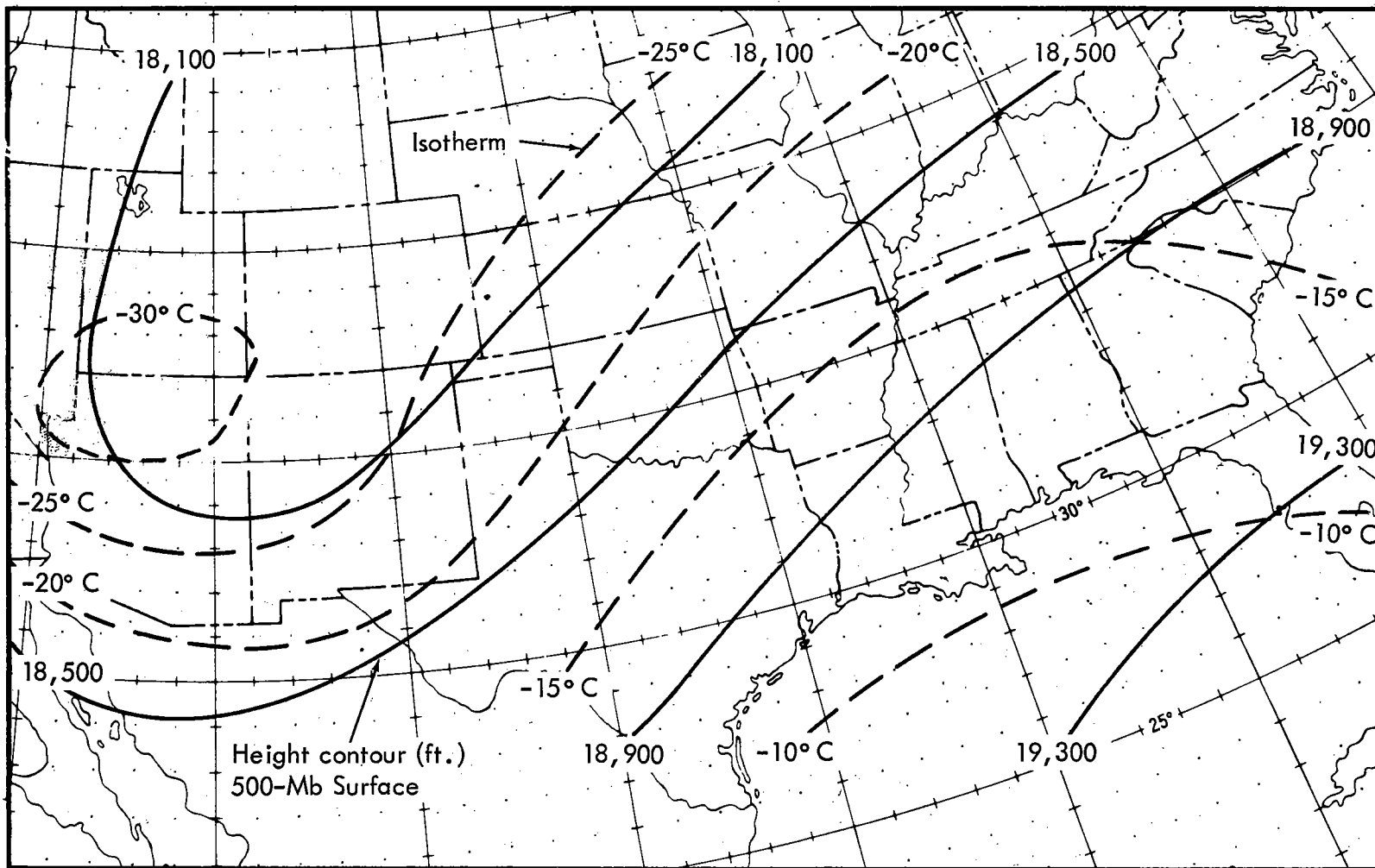
Figure 3-12. Mean 500-mb flow for March 4-5, 1963
