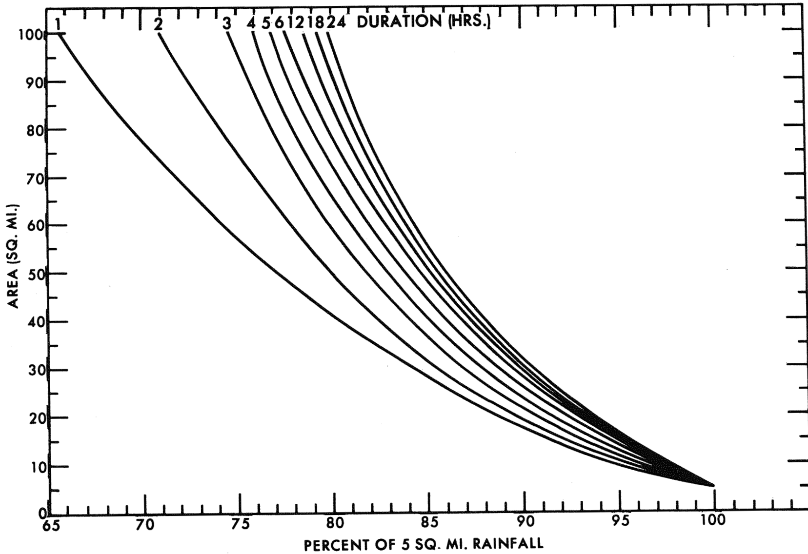
Figure 2-23. Depth-area relations for small basin estimates
