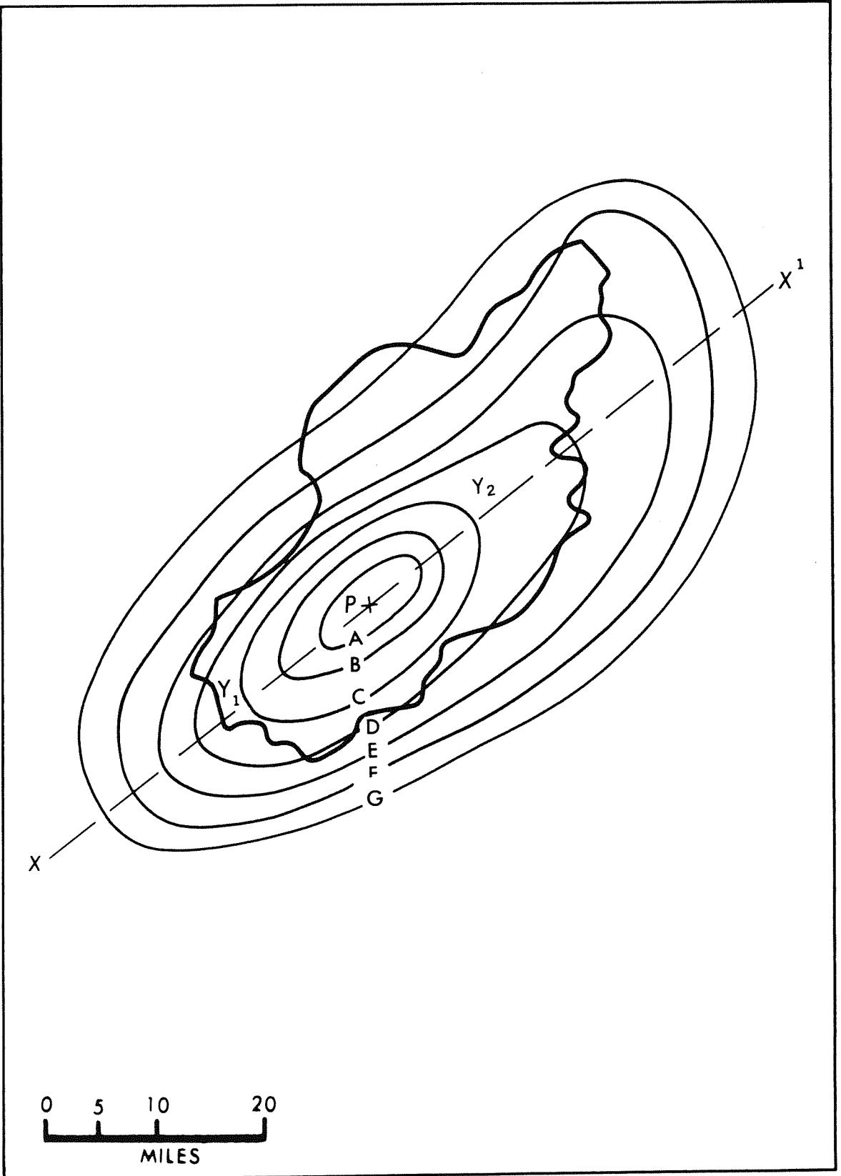
Figure 4-12. Isohyetal pattern for subbasin 12, French Broad River
