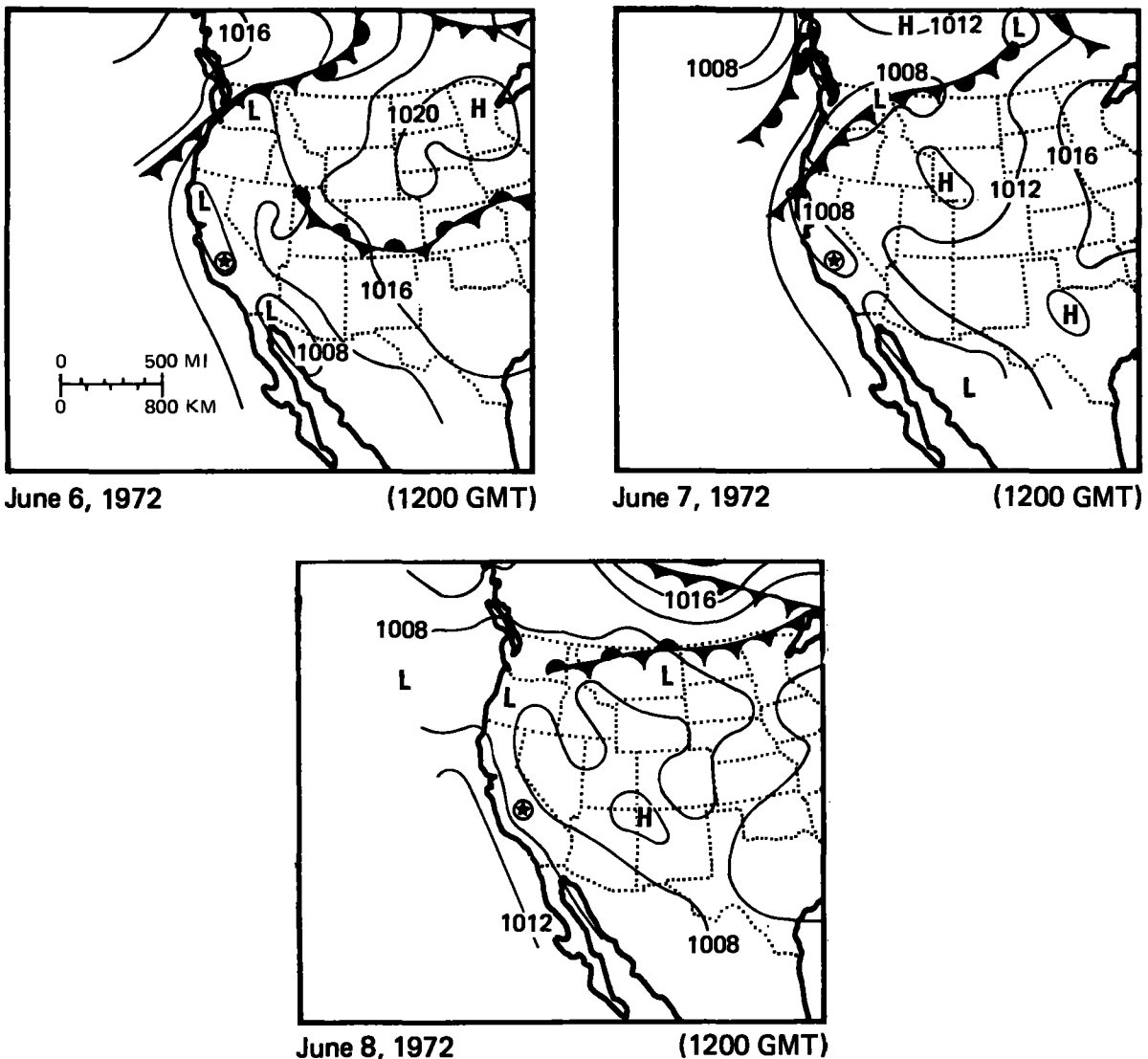
Figure 3.16.--Surface weather maps for June 6-8, 1972.
