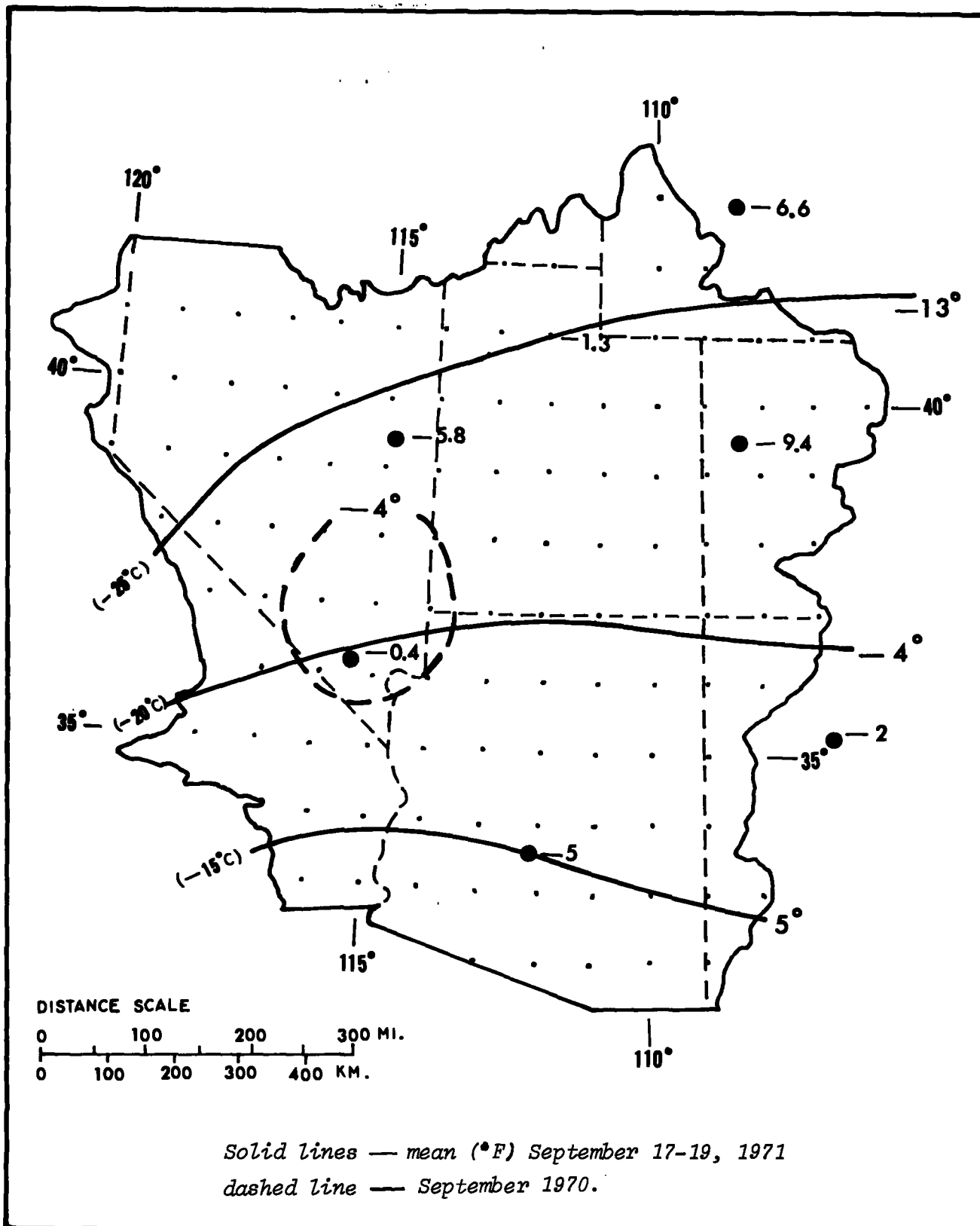
Figure 2.8.--Record 500-mb low temperatures for September.
