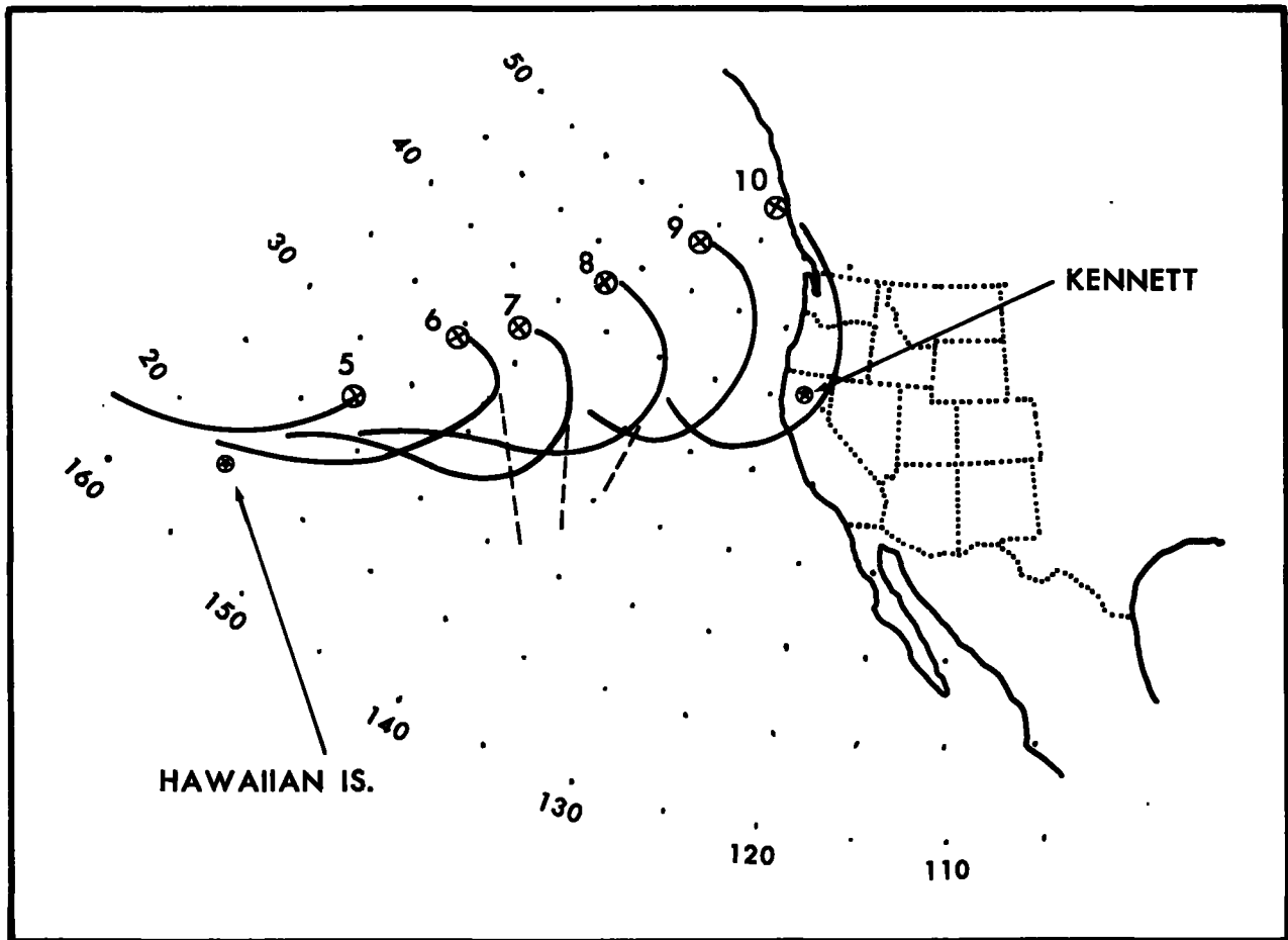
Figure 3.33.--Storm track for May 5-10, 1915.
