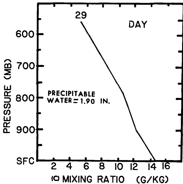
Figure 2.11.--Vertical profiles of mixing ratios on August 27-29, 1951 at Phoenix, Ariz. Metric units are customarily used to describe mixing ratio.
