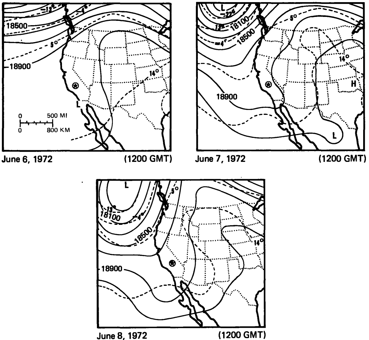
Figure 3.17.--500-mb charts for June 6-7, 1972.
