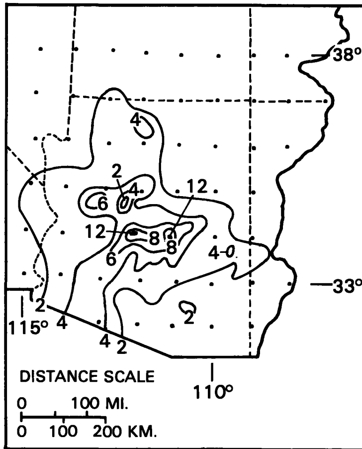
Figure 2.13.--Generalized isohyetal map for storm of August 26-30, 1951.
