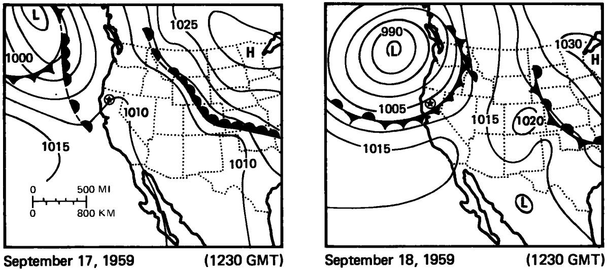
Figure 3.42.--Surface weather maps for September 17-18, 1959.
