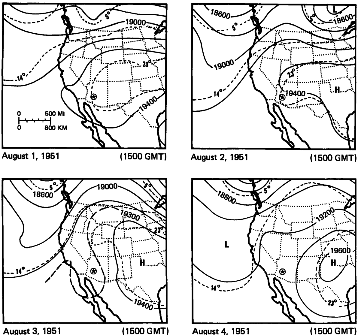
Figure 4.4.--500-mb charts for August 1-4, 1951.
