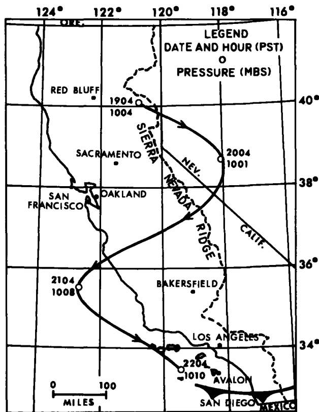
Figure 3.38.--Storm track for storm that produced heavy rain October 21, 1941 at Avalon, Calif.
