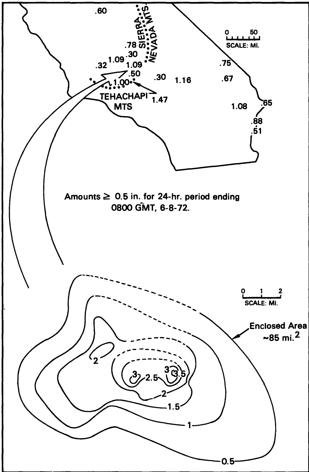
Figure 3.15.--Isohyetal analysis for storm of June 7, 1972.
