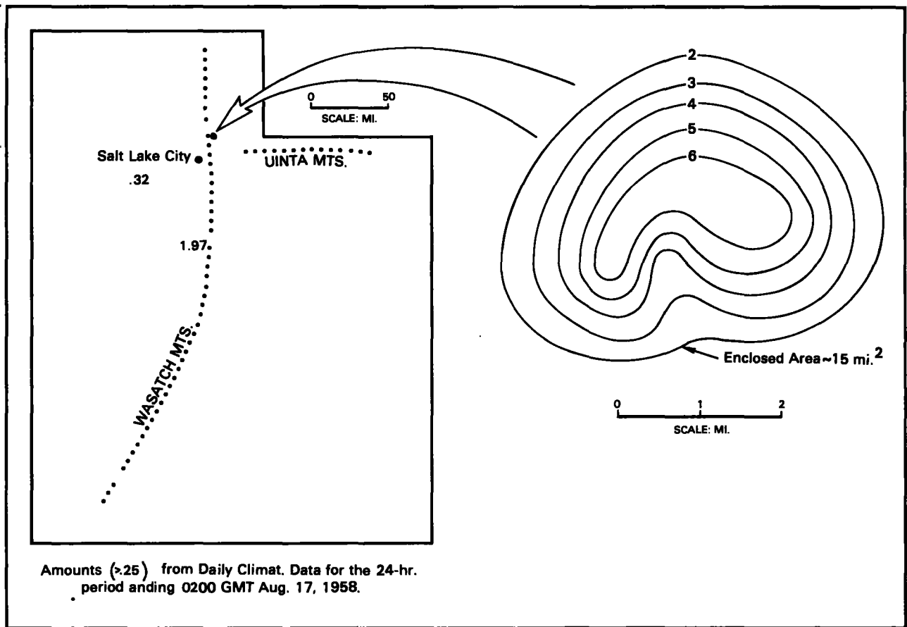
Figure 3.25.--General location map and isohyetal pattern for storm of August 16, 1958 at Morgan, Utah.
