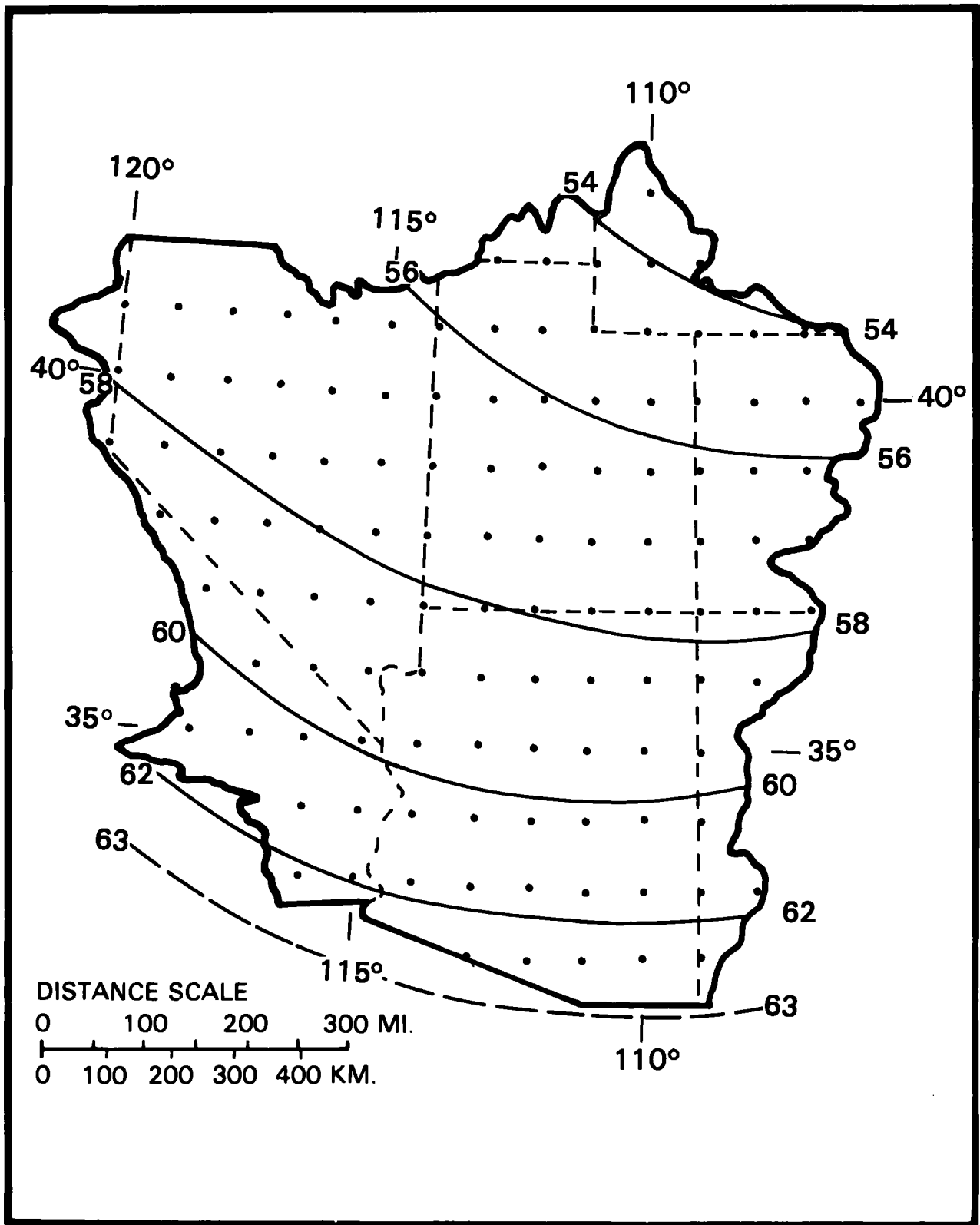
Figure 4.14.--1000-mb 12-hr persisting dew point for mid-February.
