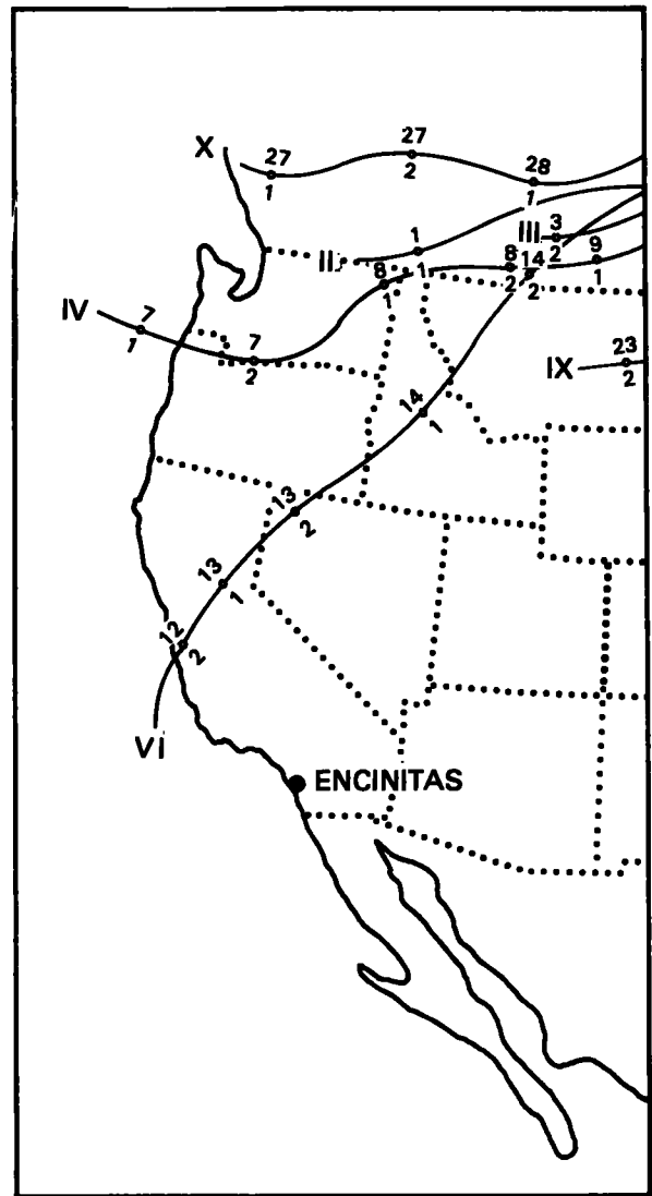
Figure 3.30.--Storm tracks for October 1889.
