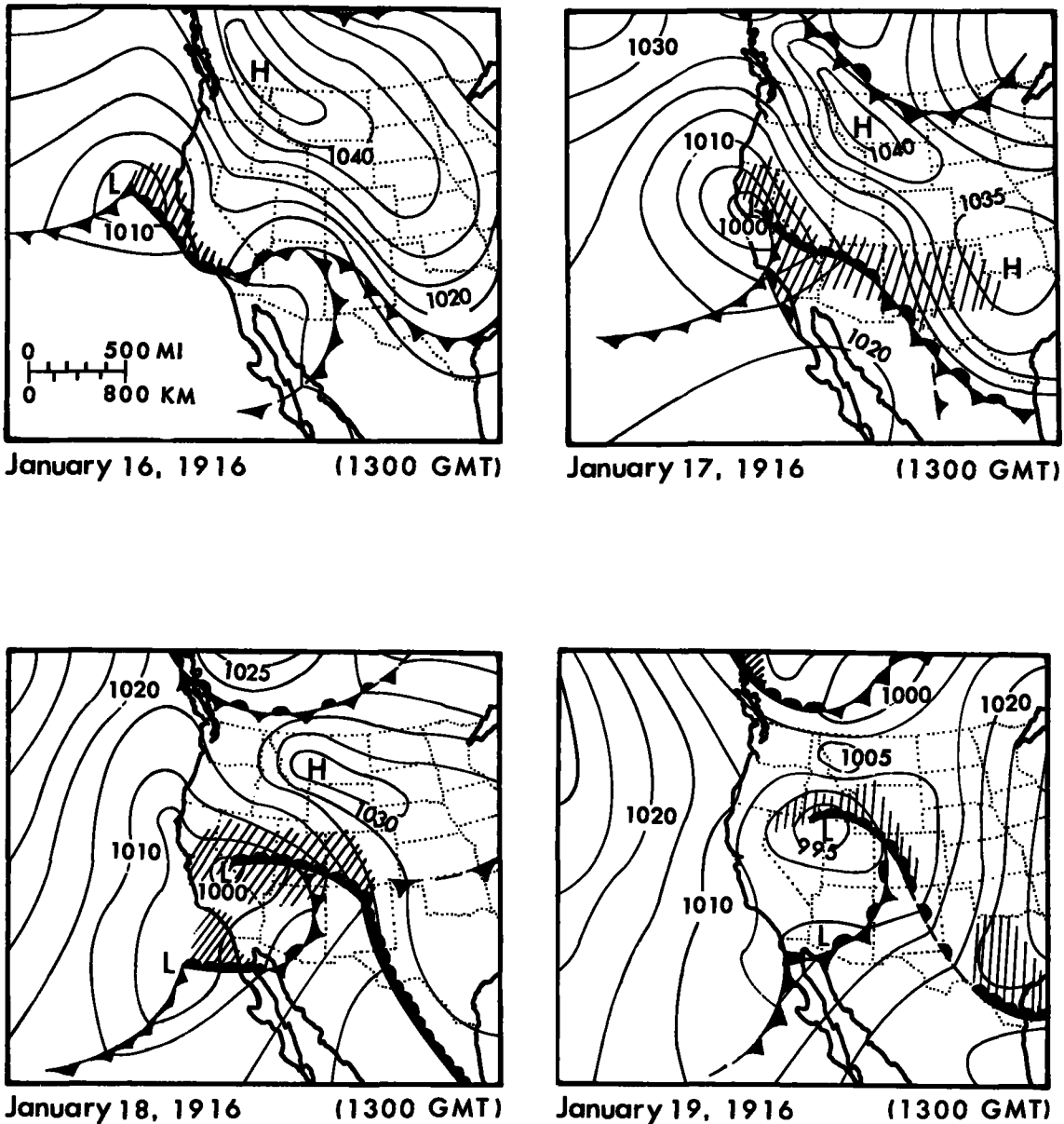
Figure 2.29.--Surface weather maps for January 16-19, 1916.
