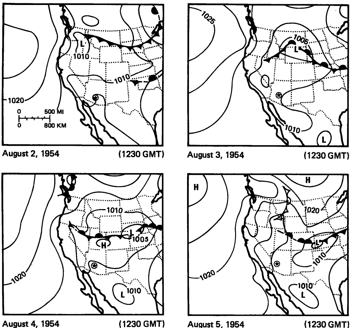
Figure 4.5.--Surface weather maps for August 2-5, 1954.
