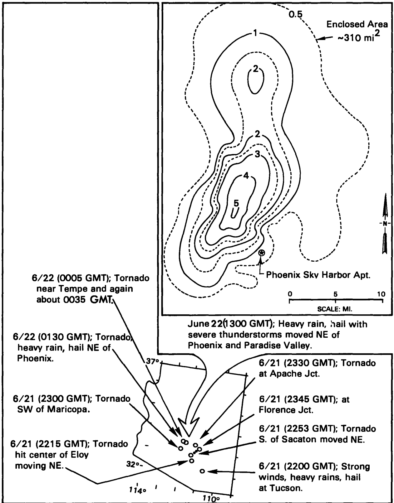
Figure 3.5.--Isohyetal analysis for storm of June 22, 1972.
