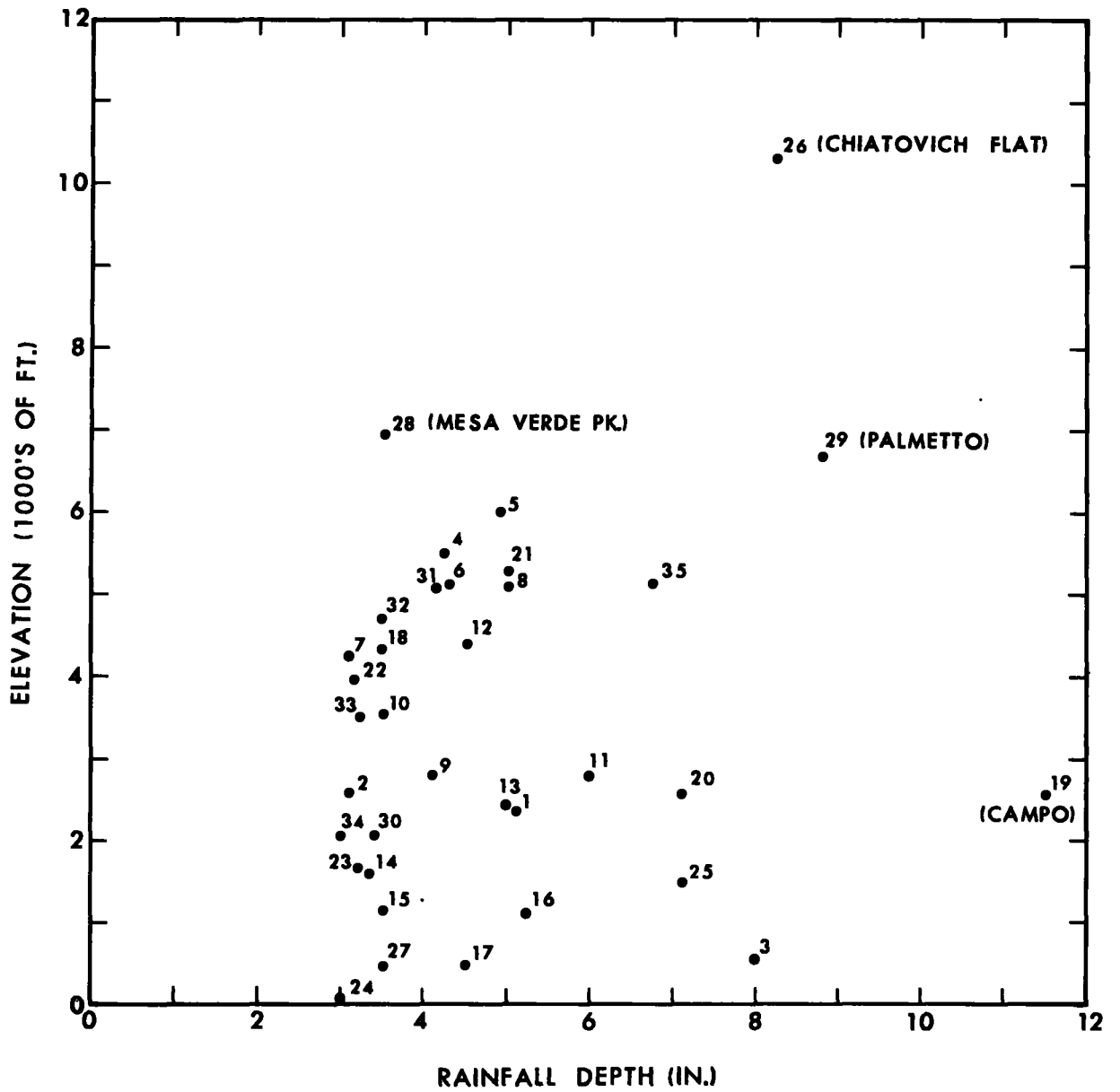
Figure 3.2.--Point rainfall extremes for local storms vs. elevation at which the data were observed. Refer to table 3.1 for storm identification.
