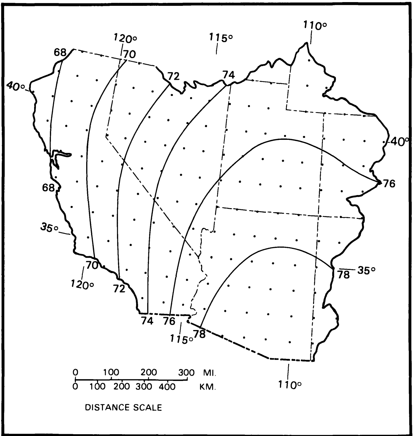
Figure 4.24.--1000-mb 12-hr persisting local storm dew point for mid-August.
