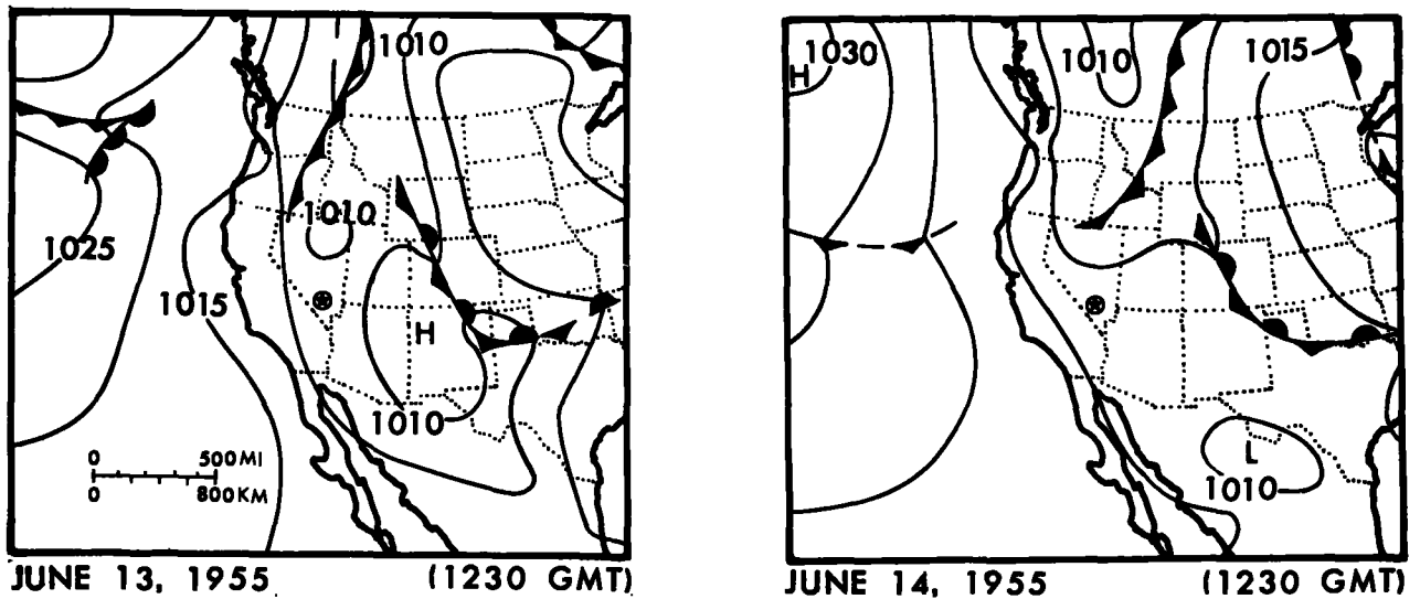
Figure 3.21. Surface weather maps for June 13-14, 1955.
