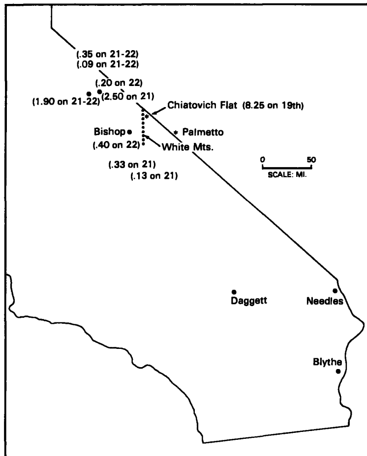
Figure 3.14.--Schematic diagram showing location of rainfall at Chiatovich Flat in relation to White Mountains. Data for other nearby stations are also shown.
