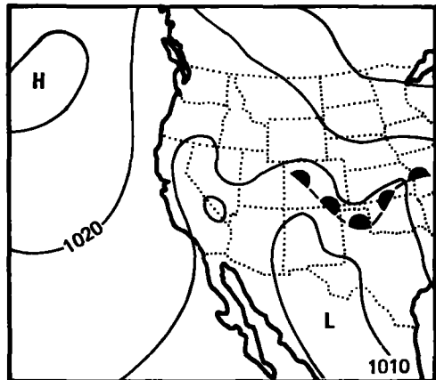
Figure 2.35a.--Surface weather maps for May 31 to June 5, 1943.
