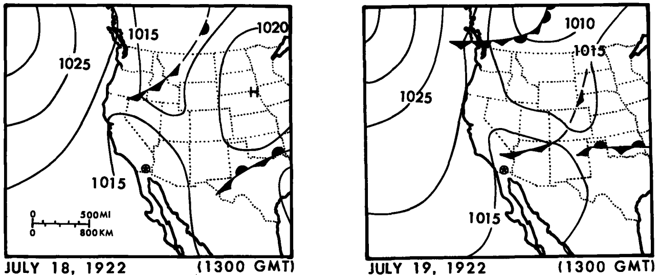
Figure 3.10.--Surface weather maps for July 18-19, 1922.
