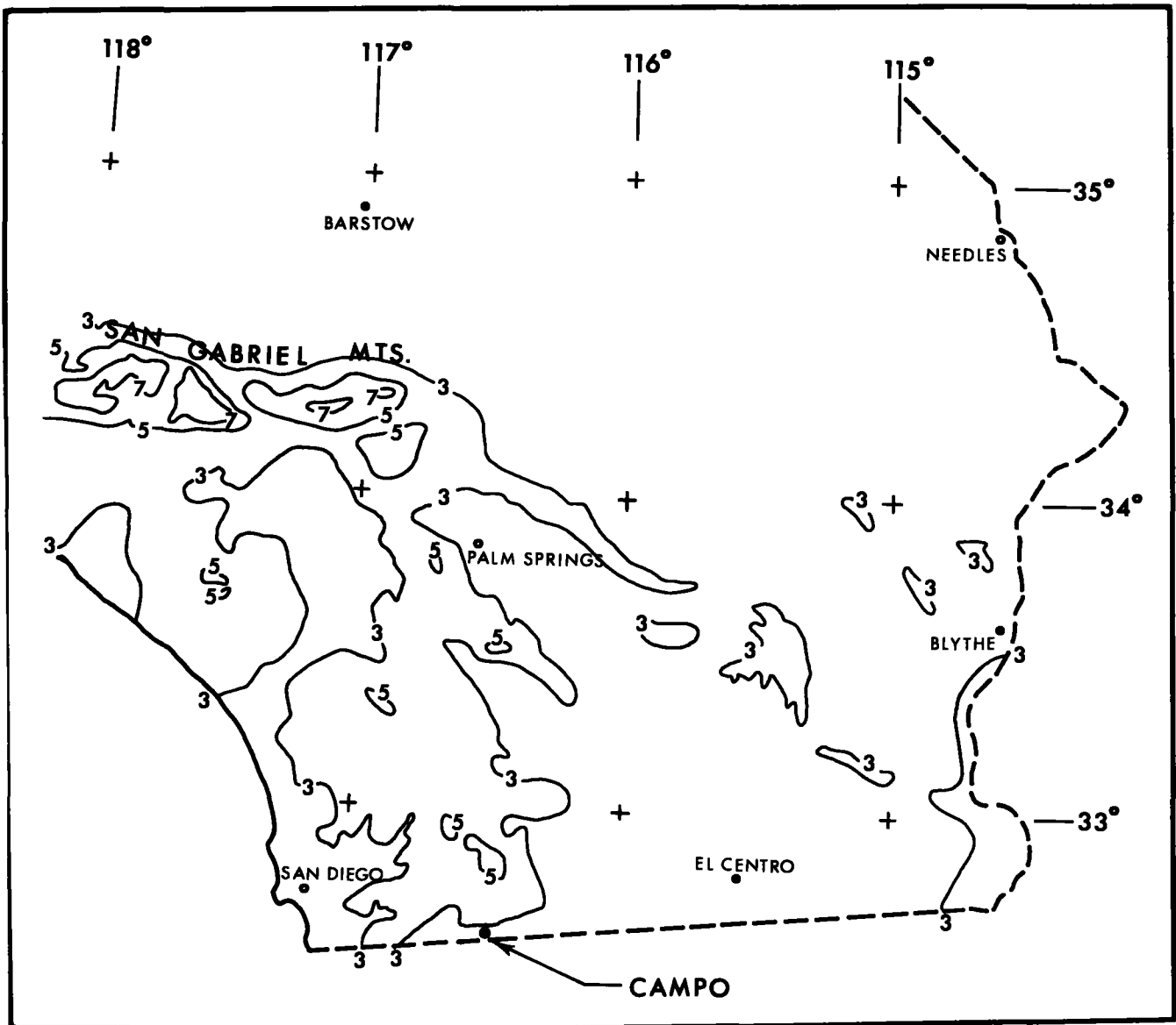
Figure 3.11.--100-yr 6-hr rainfall for southern portion of southern California.
