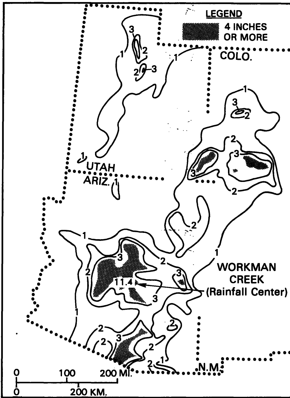
Figure 2.3.--Generalized isohyetal pattern for tropical storm (Norma), September 4-7, 1970,
