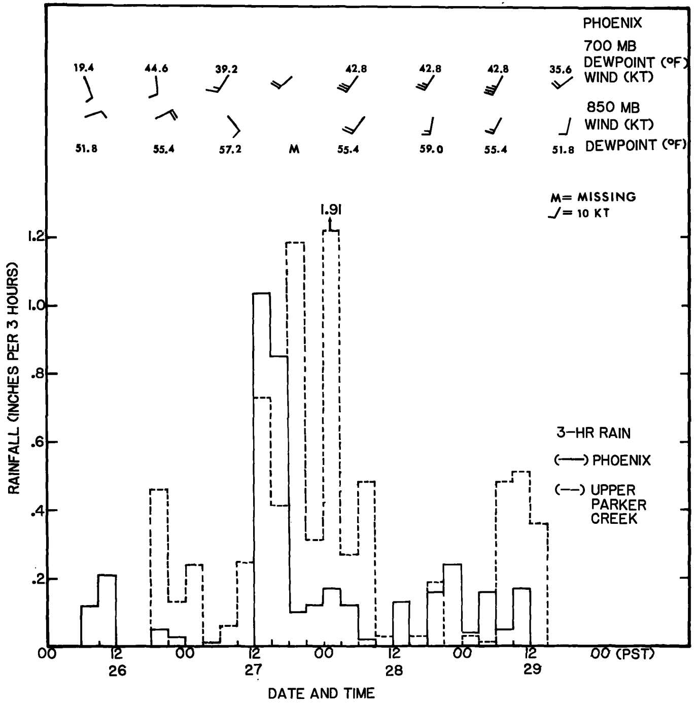
Figure 2.12.--Comparison of dew points and winds at Phoenix, Ariz. with 3-hr precipitation increments at Phoenix and Upper Parker Creek, Ariz., August 20-29, 1951.
