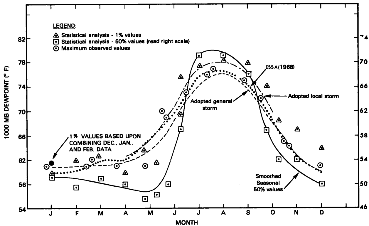
Figure 4.10.--Seasonal plot of dew point values for Salt Lake City, Utah.
