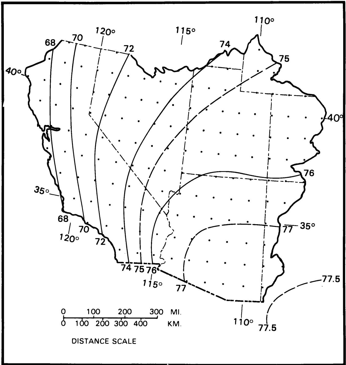
Figure 4.22.--1000-mb 12-hr persisting local storm dew point for mid-July.
