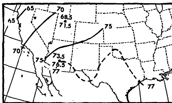
C--ANALYSIS OF ONE PERCENT LEVEL OF PRECIPITABLE WATER EXPRESSED AS 1000-MB DEW POINTS (°F)
