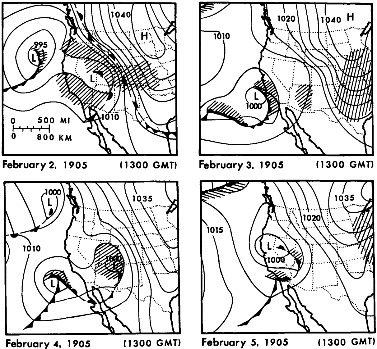
Figure 2.39.--Surface weather maps for February 2-5, 1905.
