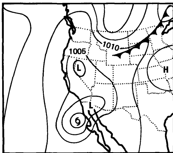
Figure 2.17.--Surface weather maps for October 4-6, 1925 and schematic diagram showing estimated upper level trough positions.
