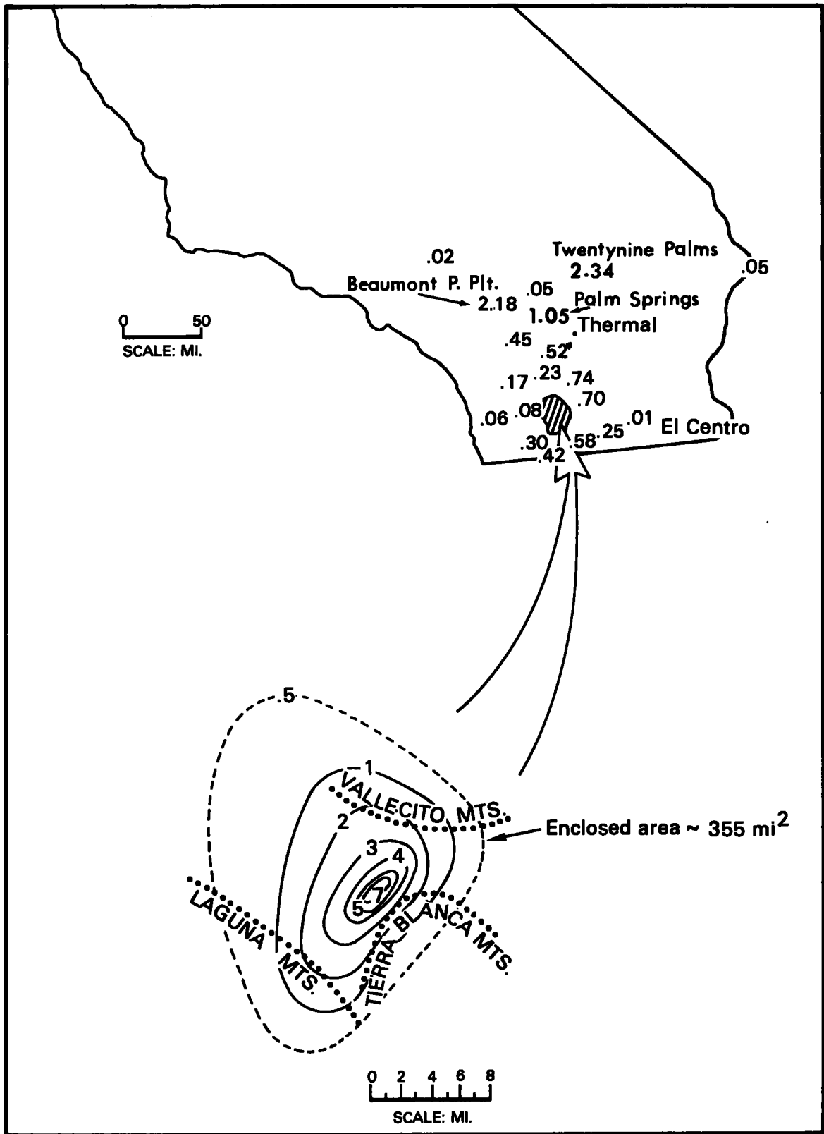
Figure 3.12.--Isohyetal map for storm at Vallecito, Calif. on July 18, 1955. Rainfall data are shown for other stations in southern California.
