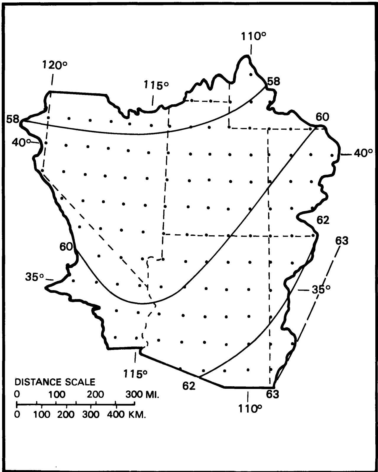
Figure 4.17.--1000-mb 12-hr persisting general storm dew point for mid-April.
