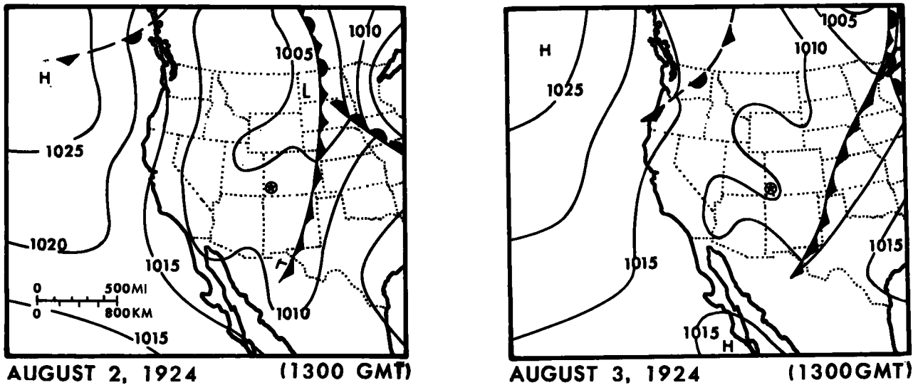
Figure 3.18.--Surface weather maps for August 2-3, 1924.
