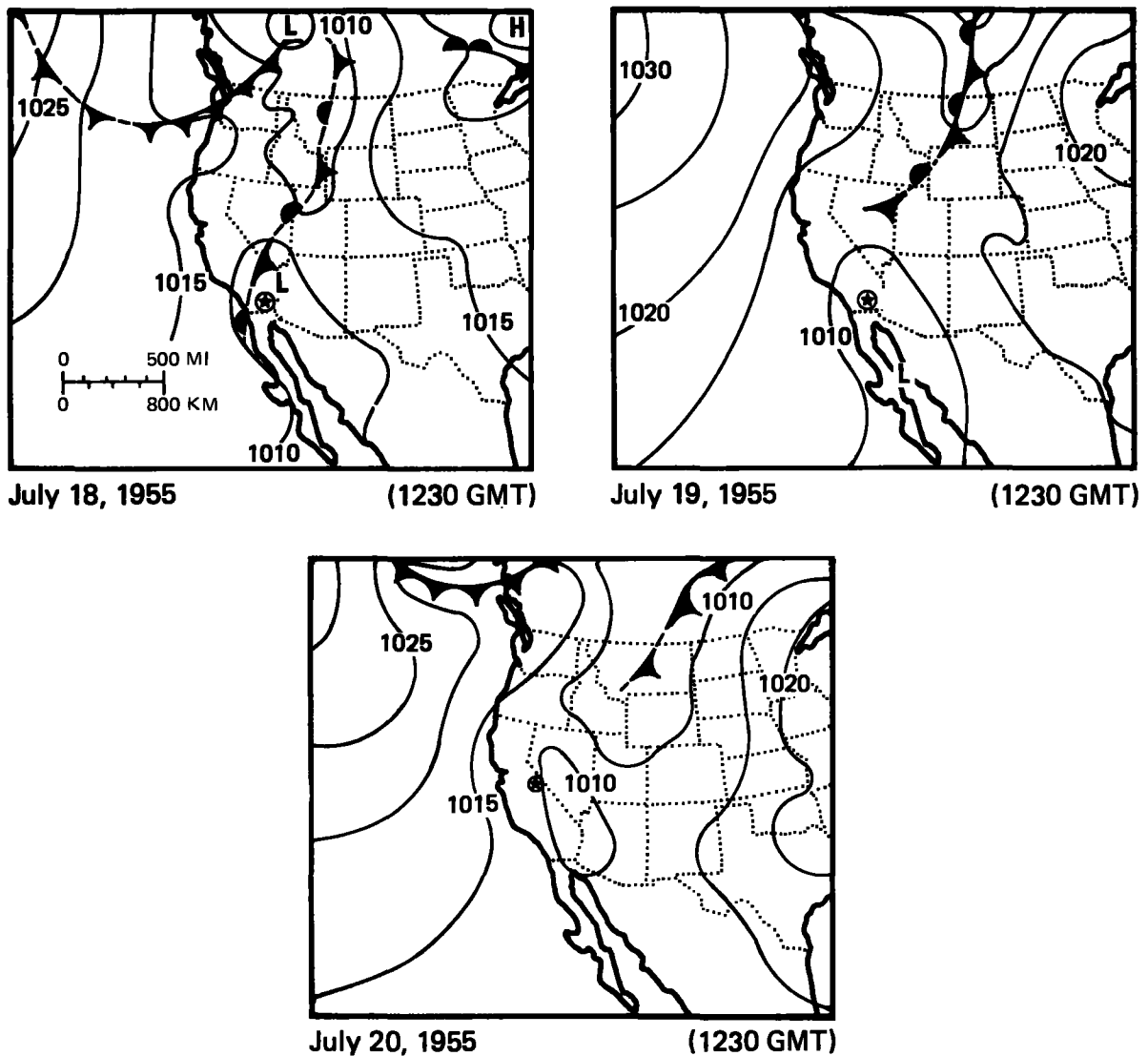
Figure 3.13.--Surface weather maps for July 18-20, 1955.
