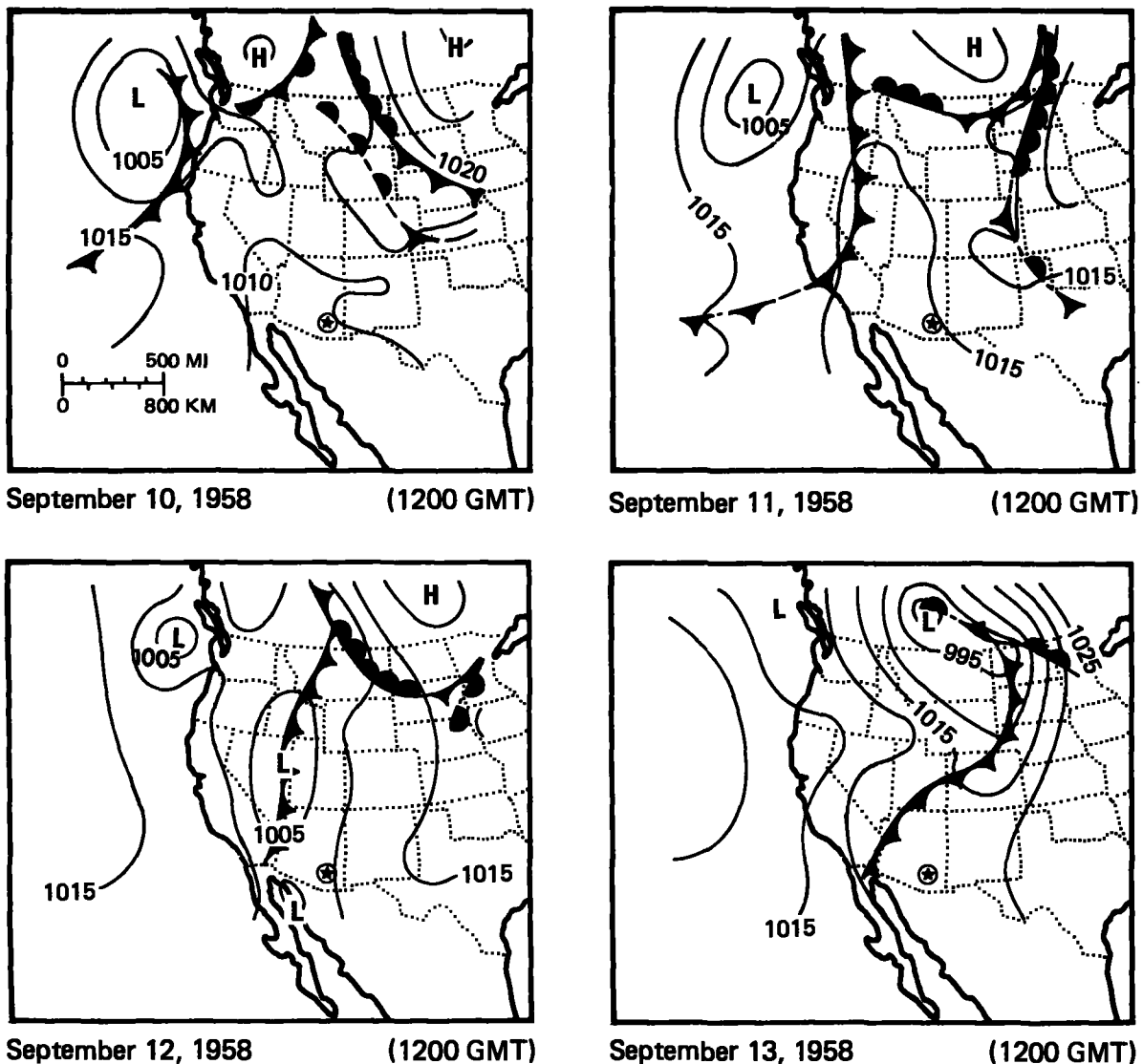
Figure 4.7.--Surface weather maps for September 10-13, 1958.
