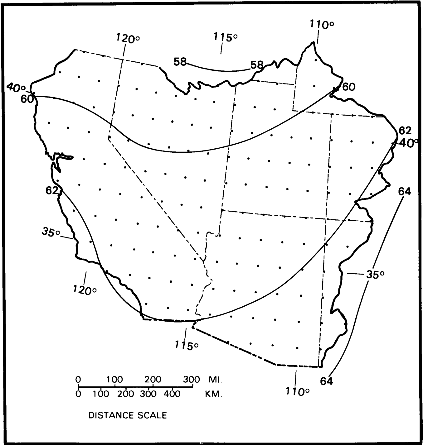
Figure 4-16.--1000-mb 12-hr persisting local storm dew point for mid April.
