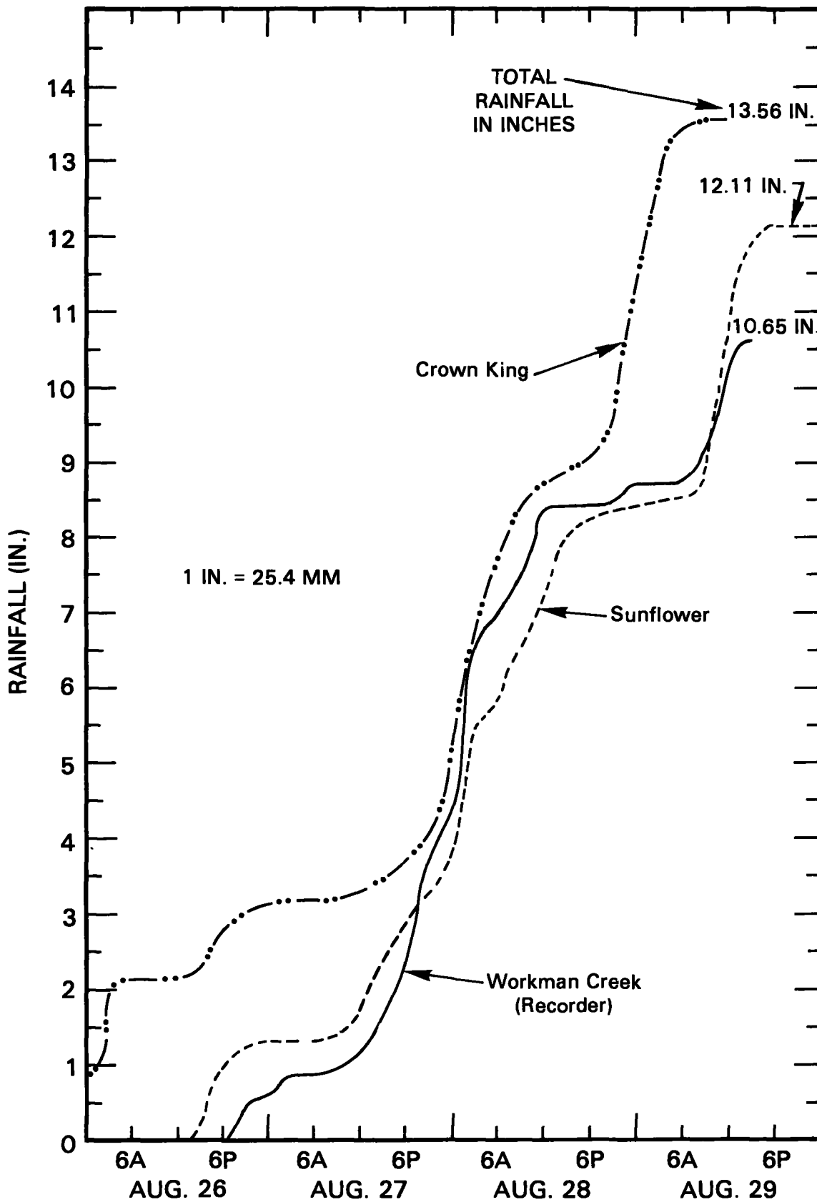
Figure 2.14.--Mass curves of rainfall at selected stations for storm of August 26-30, 1951.
