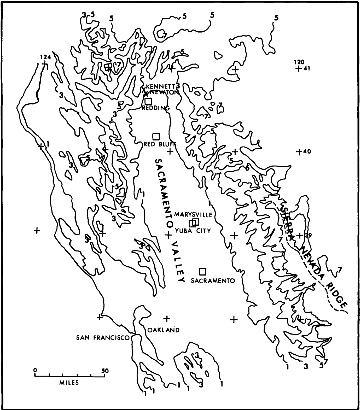
Figure 3.31.--Generalized contours for the Central Valley and surrounding mountains for north central California.
