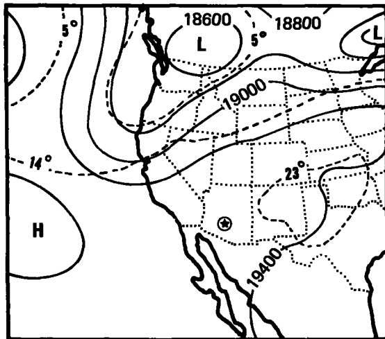
Figure 4.6.--500-mb charts for August 2-5, 1954.
