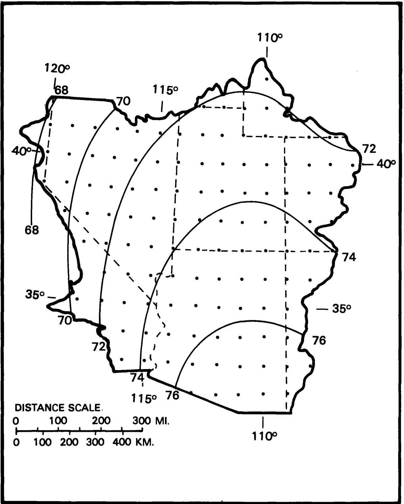
Figure 4.25.--1000-mb 12-hr persisting general storm dew point for mid-August.
