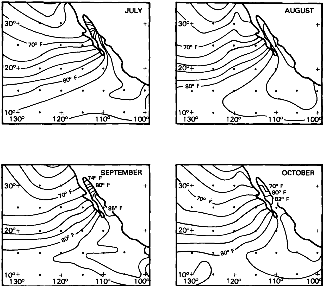
Figure 2.45.--Mean sea-surface temperature charts for the tropical Pacific for July, August, September and October (Lavolette and Seim 1969).
