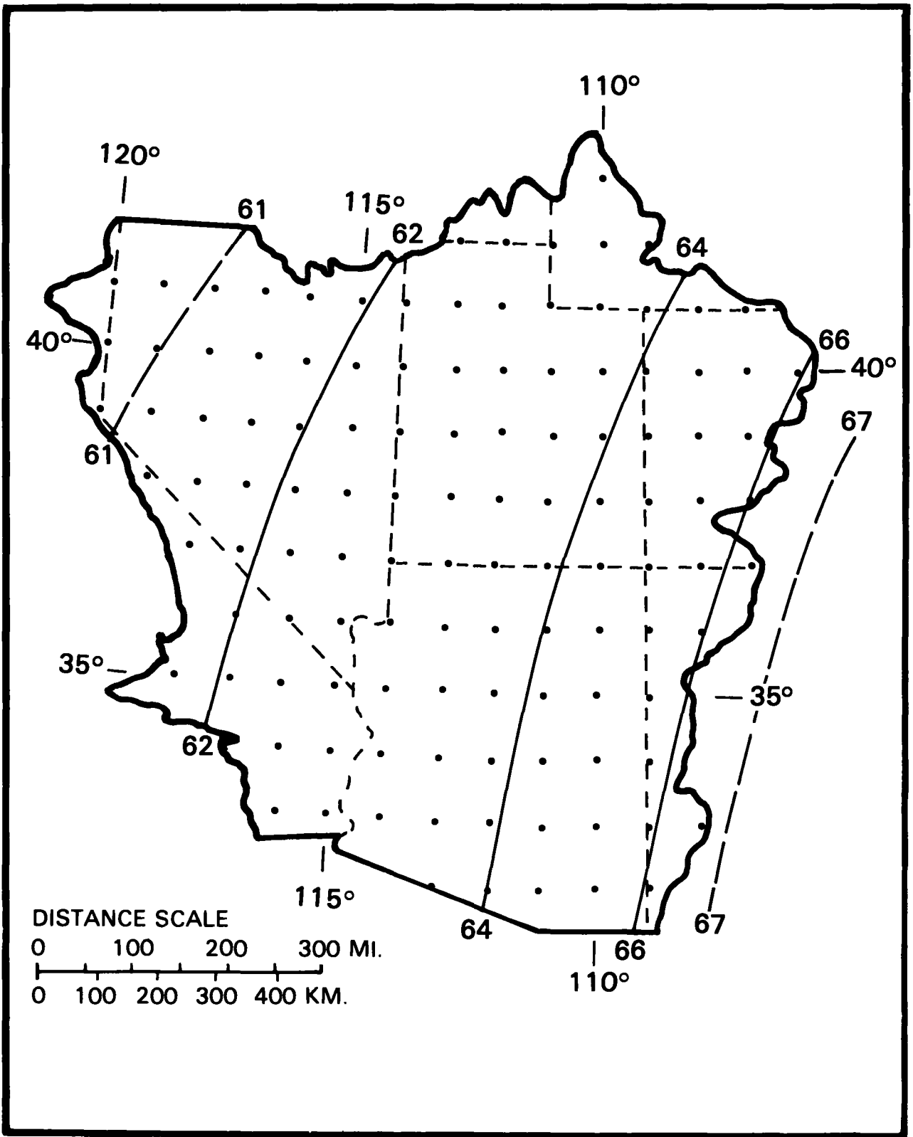
Figure 4.19.--1000-mb 12-hr persisting general storm dew point for mid-May.
