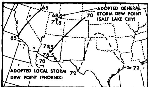
A--ANALYSIS OF MAXIMUM OBSERVED PRECIPITABLE WATER EXPRESSED AS 1000-MB DEW POINTS (°F)
