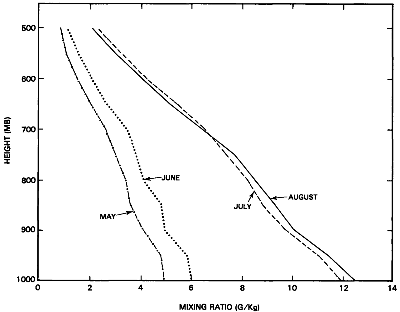
Figure 4.2.--Mean monthly mixing ratio for May, June, July and August at Phoenix, Ariz.
