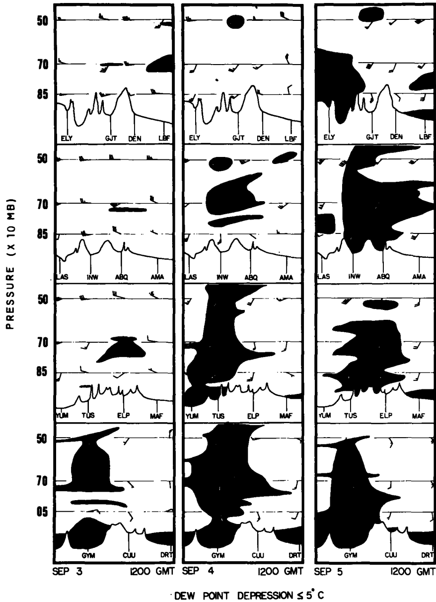
Figure 2.6.--Vertical distribution of moisture over Southwest during the period September 2-7, 1970, from May (1971)
