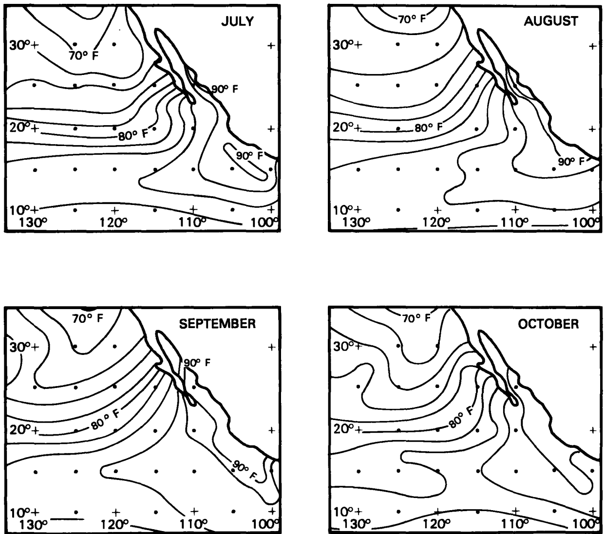
Figure 2.46.--Maximum sea-surface temperature charts for the tropical Pacific for July, August, September and October (Lavolette and Seim 1969).
