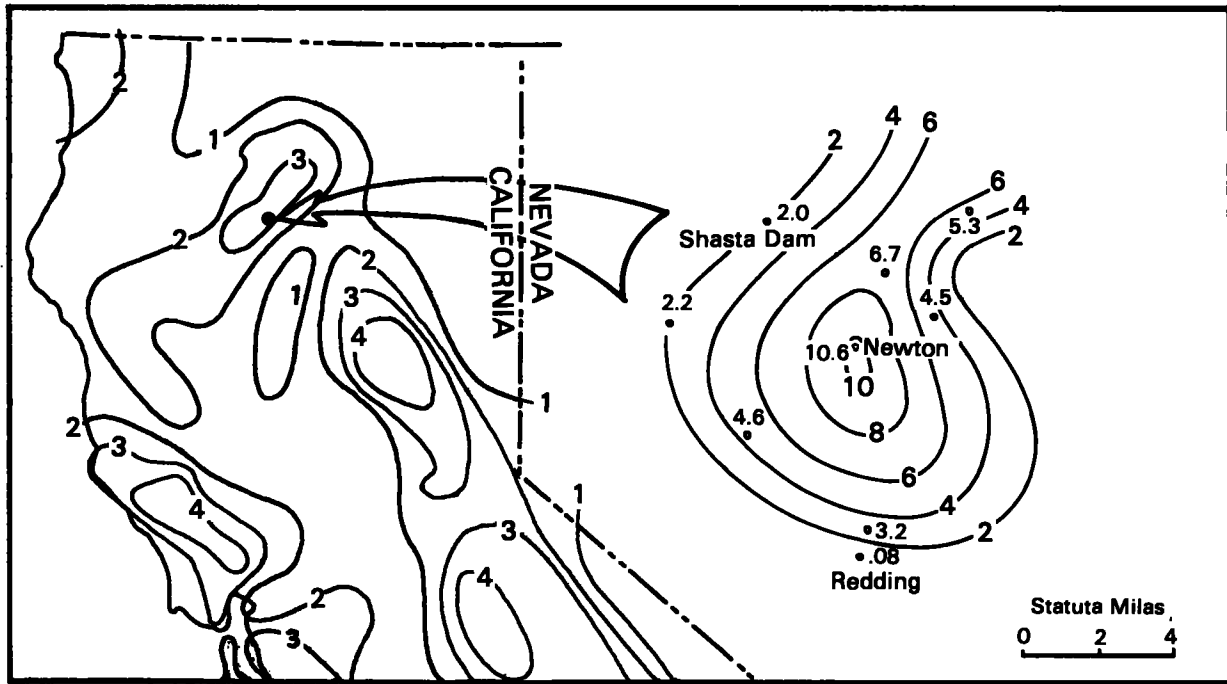
Figure 3.41.--Isohyetal pattern for storm of September 17-18, 1959.
