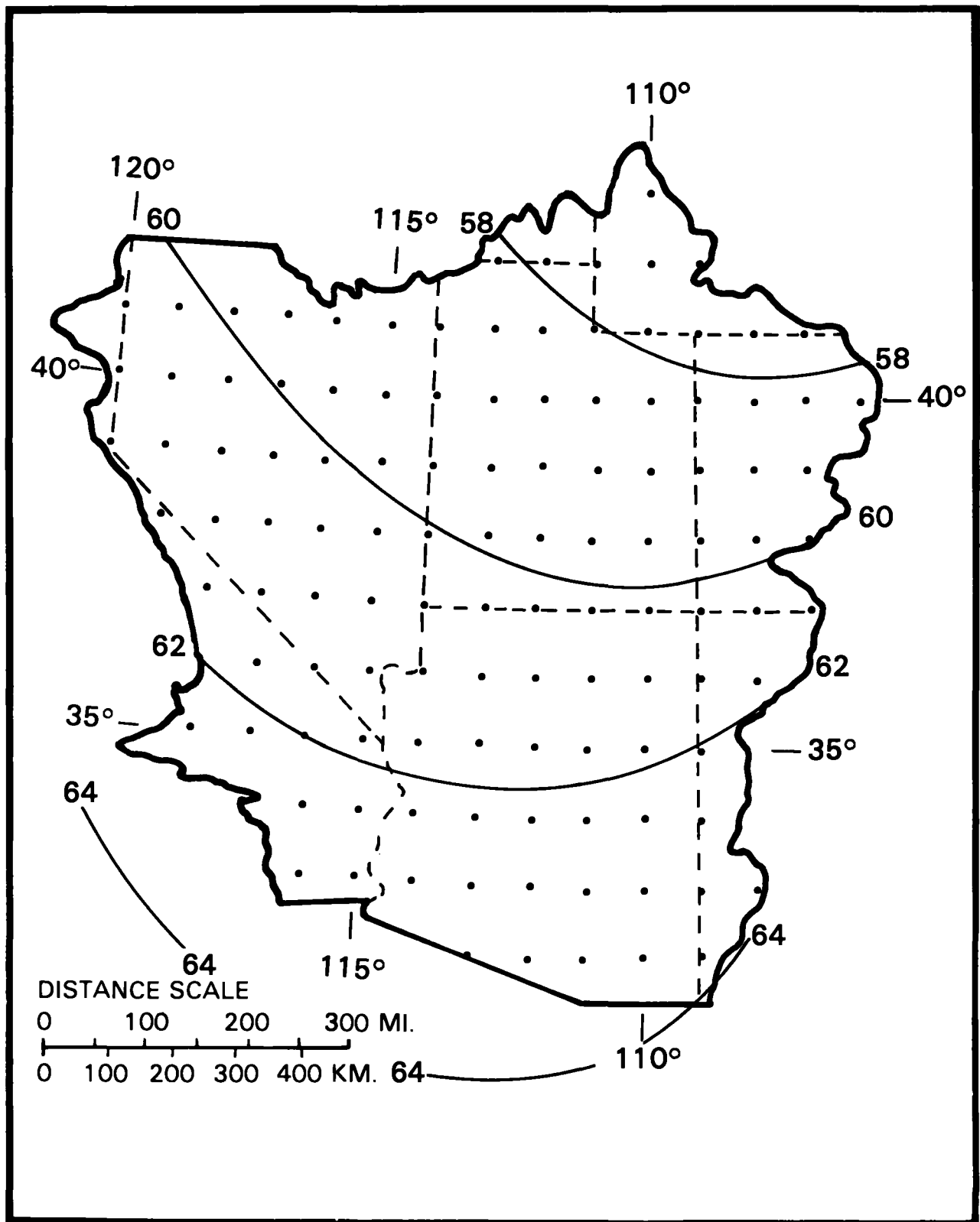
Figure 4.30.--1000-mb 12-hr persisting general dew point for mid-November.
