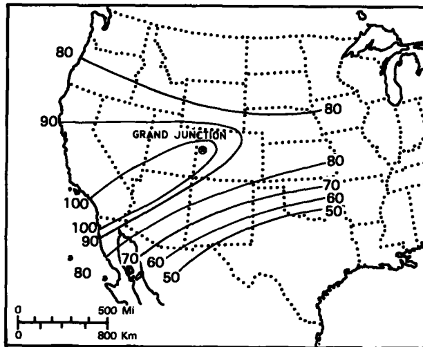
Figure 4.1.--Percentage of months at stations in Southwest with precipitable water values larger than monthly means concurrent with similar months at Grand Junction.
