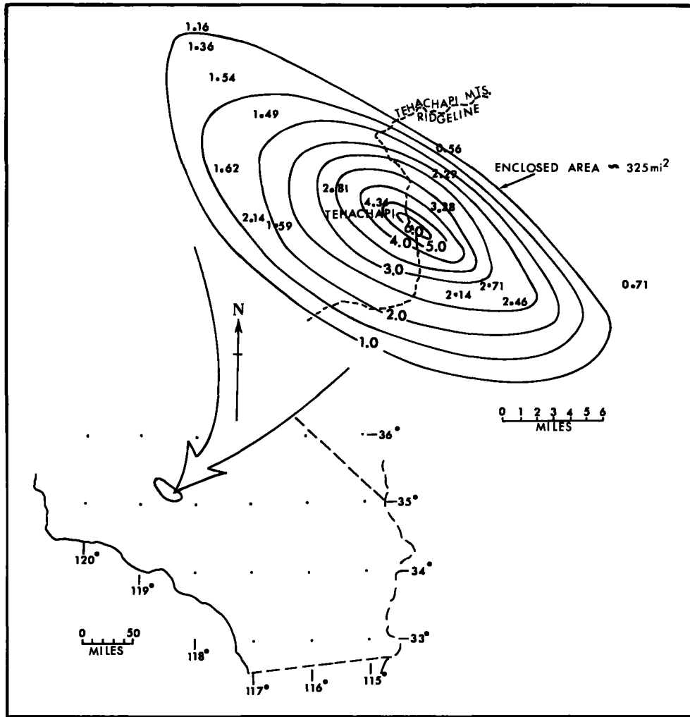
Figure 3.34.--Isohyetal map for storm of September 30, 1932.
