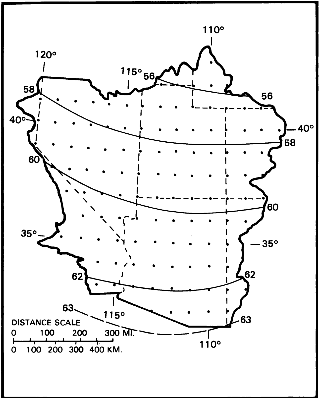
Figure 4.15.--1000-mb 12-hr persisting dew point for mid-March.
