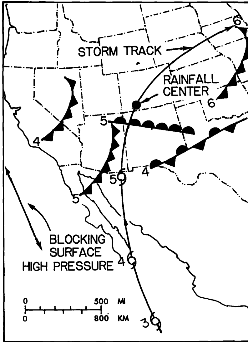
Figure 2.19.--Storm track and significant weather features for storm of October 4-6, 1911.
