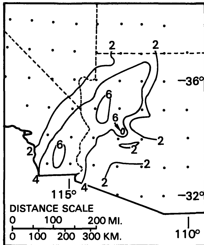
Figure 2.16.--Generalized isohyetal map for storm of September 4-7, 1939.
