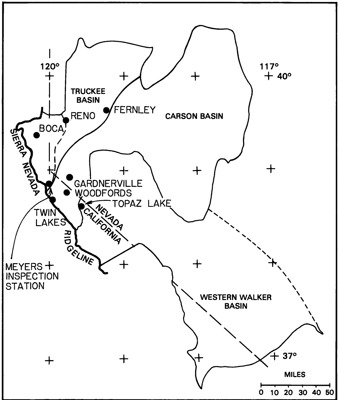
Figure 2.42.--Location map for Truckee, Carson and Walker River drainages.
