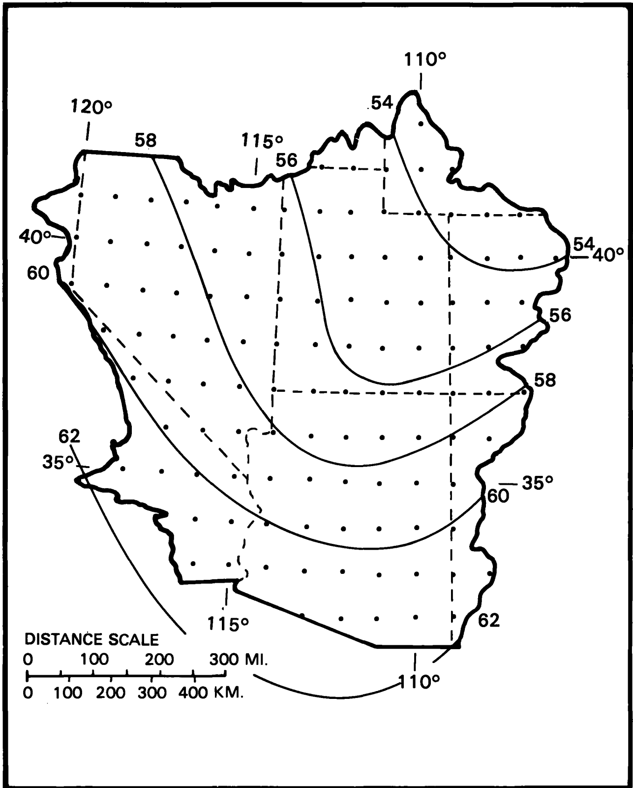
Figure 4.31.--1000-mb 12-hr persisting dew point for mid December.
