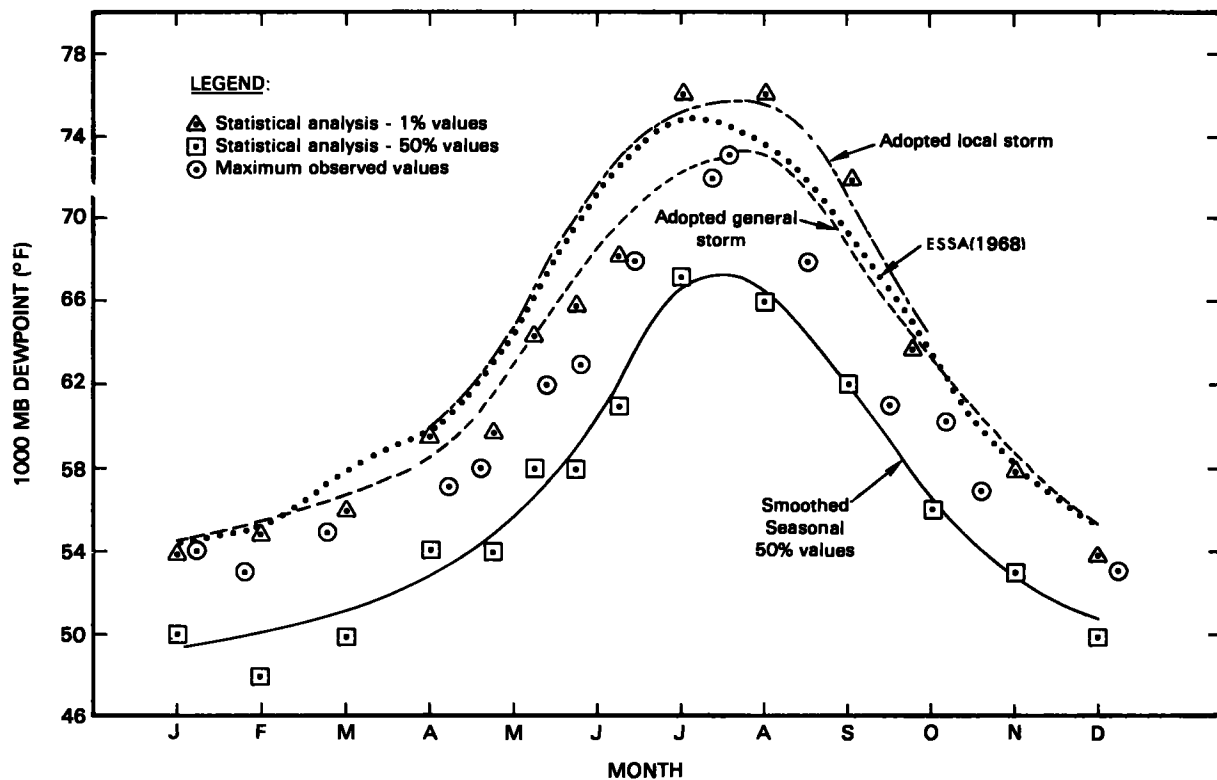
Figure 4.9.--Seasonal plot of dew point values for Phoenix, Ariz.
