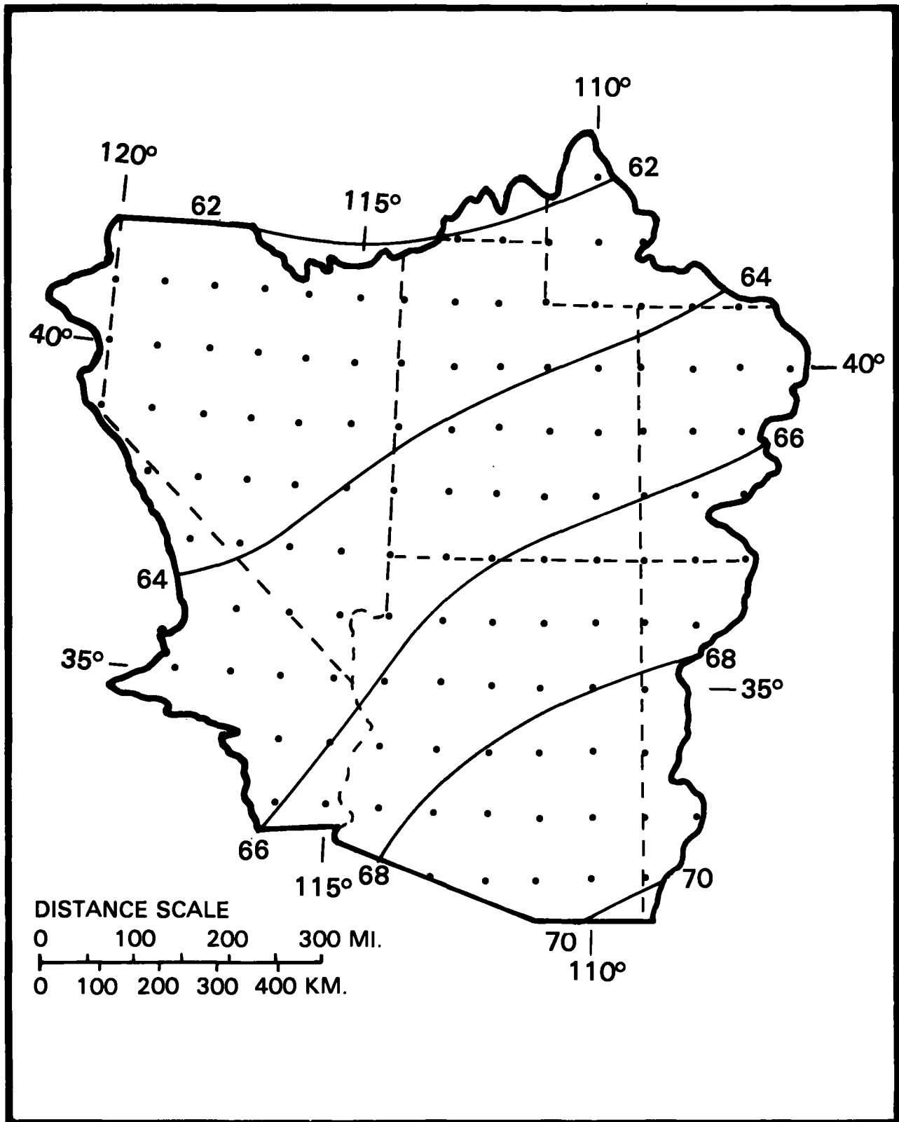
Figure 4.29.--1000-mb 12-hr persisting general storm dew point for mid-October.
