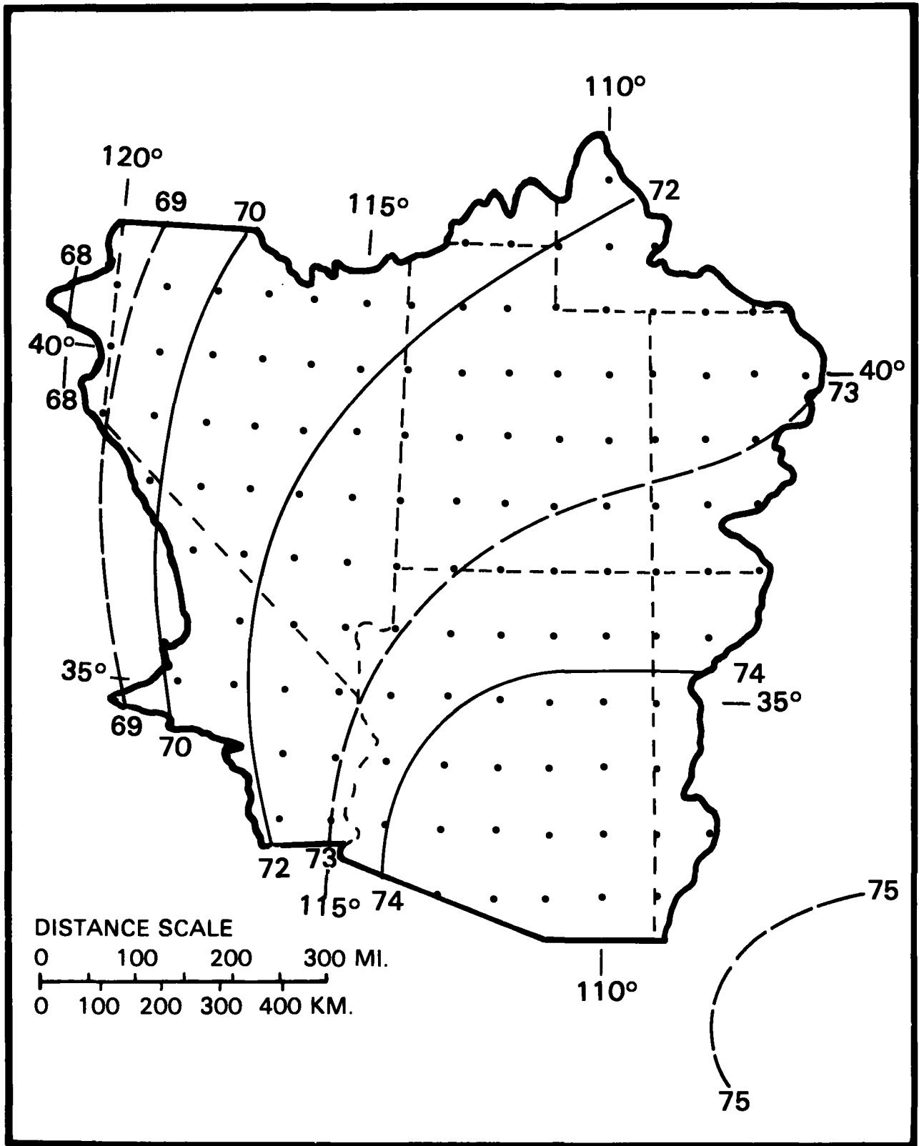
Figure 4.23.--1000-mb 12-hr persisting general storm dew point for mid-July.
