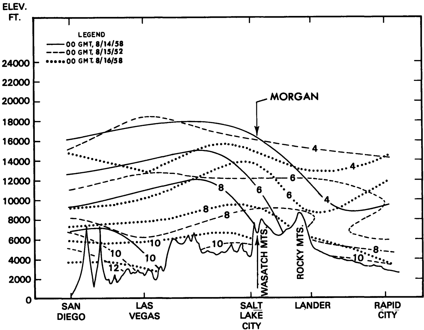
Figure 3.28.--Temporal variations of moisture (8 gm/kg) along vertical cross section along a line from San Diego, California to Rapid City, S.D.
