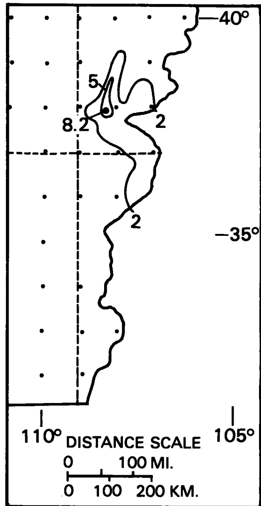
Figure 2.21.--Generalized isohyetal map for storm of October 4-5, 1911.
