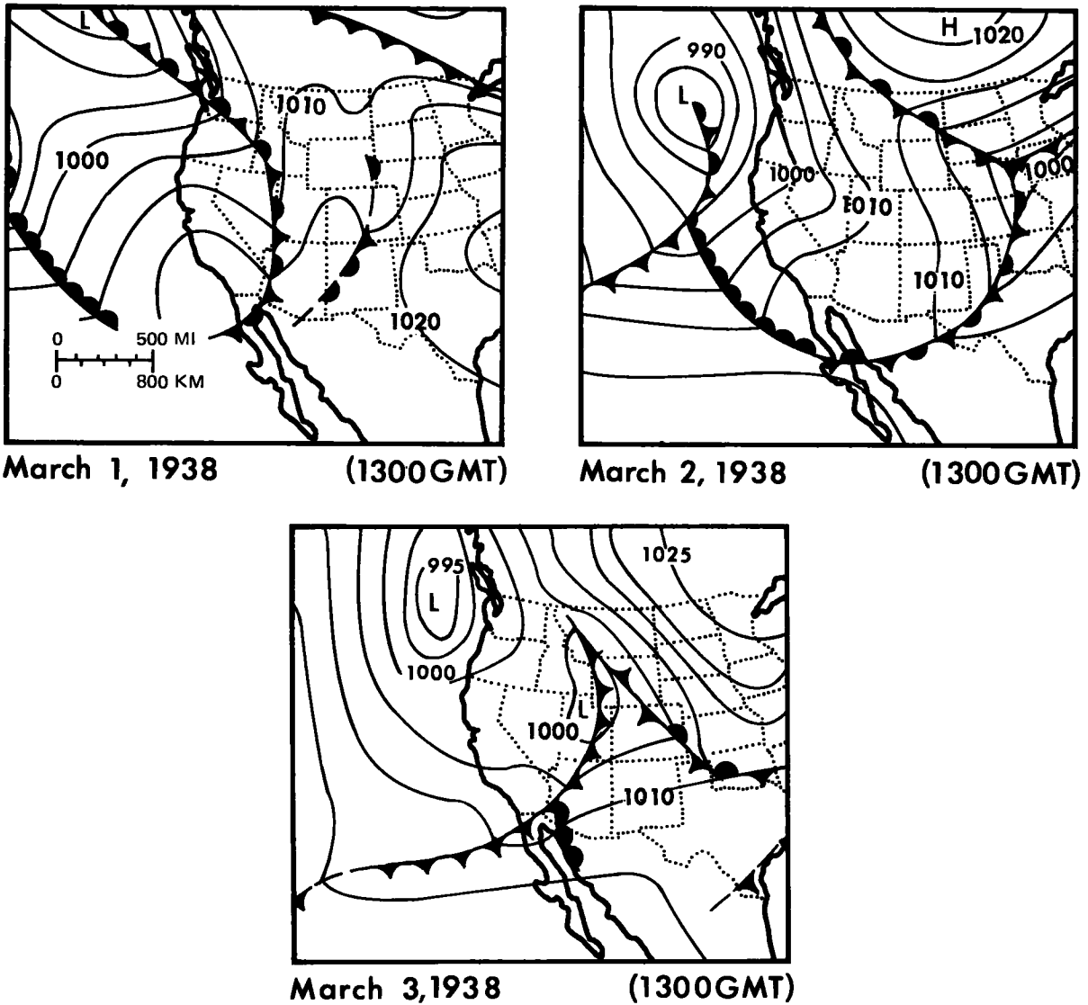
Figure 2.41.--Surface weather maps for March 1-3, 1938.
