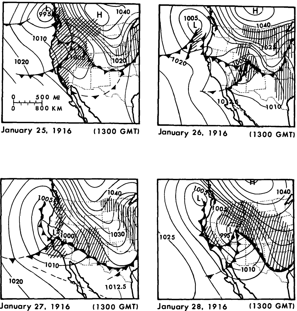
Figure 2.30.--Surface weather maps for January 25-28, 1916.
