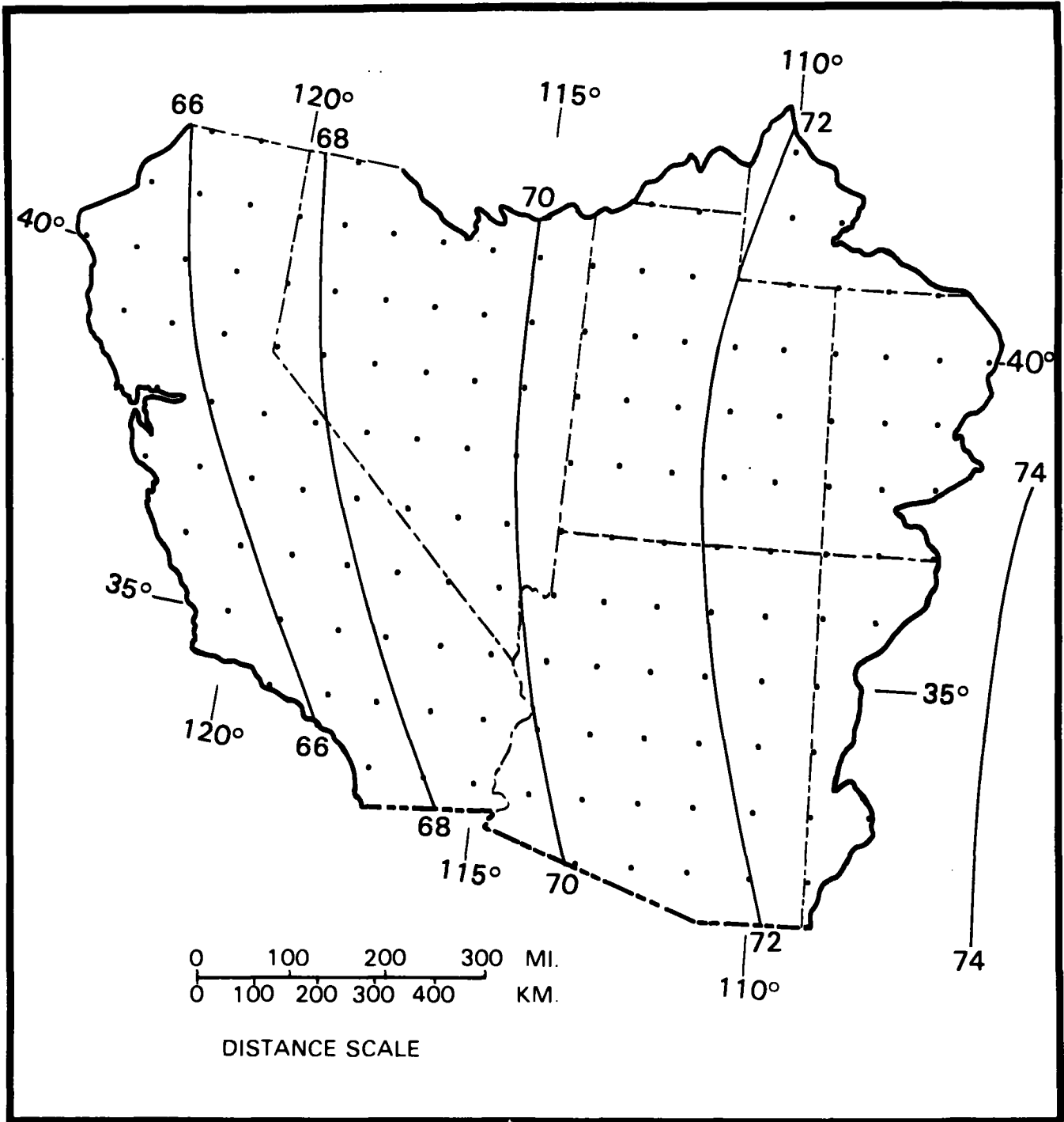
Figure 4.20.--1000-mb 12-hr persisting local storm dew point for mid-June.
