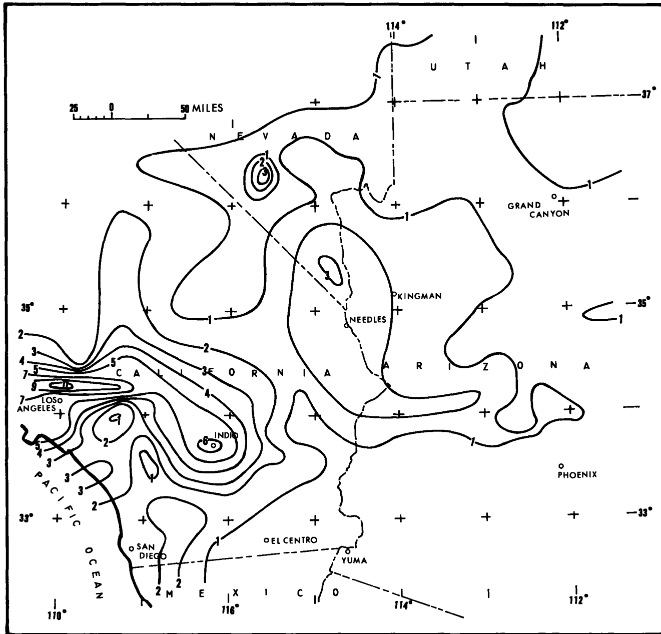
Figure 2.22 Generalized isohyetal map for storm of September 13-15, 1939.
