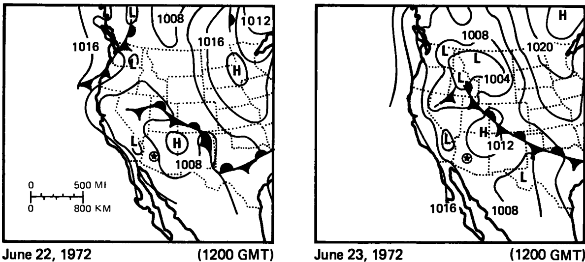
Figure 3.6.--Surface weather maps for June 22 and 23, 1972.
