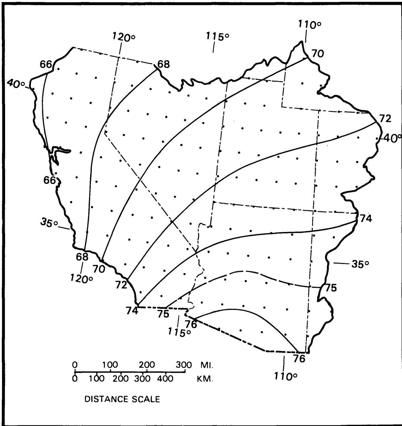
Figure 4.26.--1000-mb 12-hr persisting local-storm dew point for mid-September.
