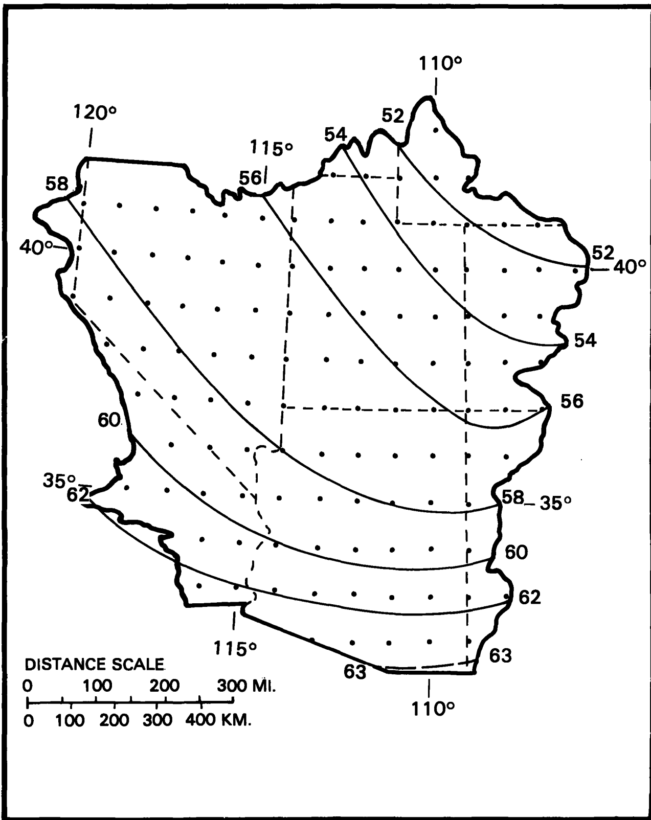
Figure 4.13.--1000-mb 12-hr persisting dew point for mid-January.
