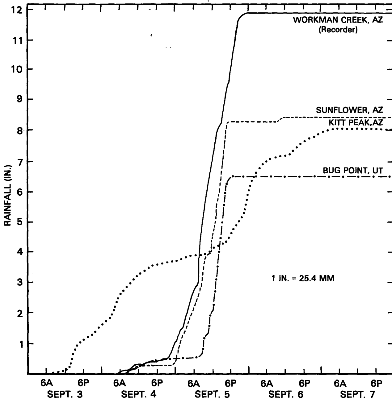
Figure 2.7.--Mass curves of rainfall at selected stations for storm of September 2-7, 1970.
