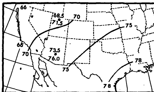
B--MAXIMUM PERSISTING 12-HR 1000-MB DEW POINTS (°F) AFTER ENVIRONMENTAL DATA SERVICE (1968)
