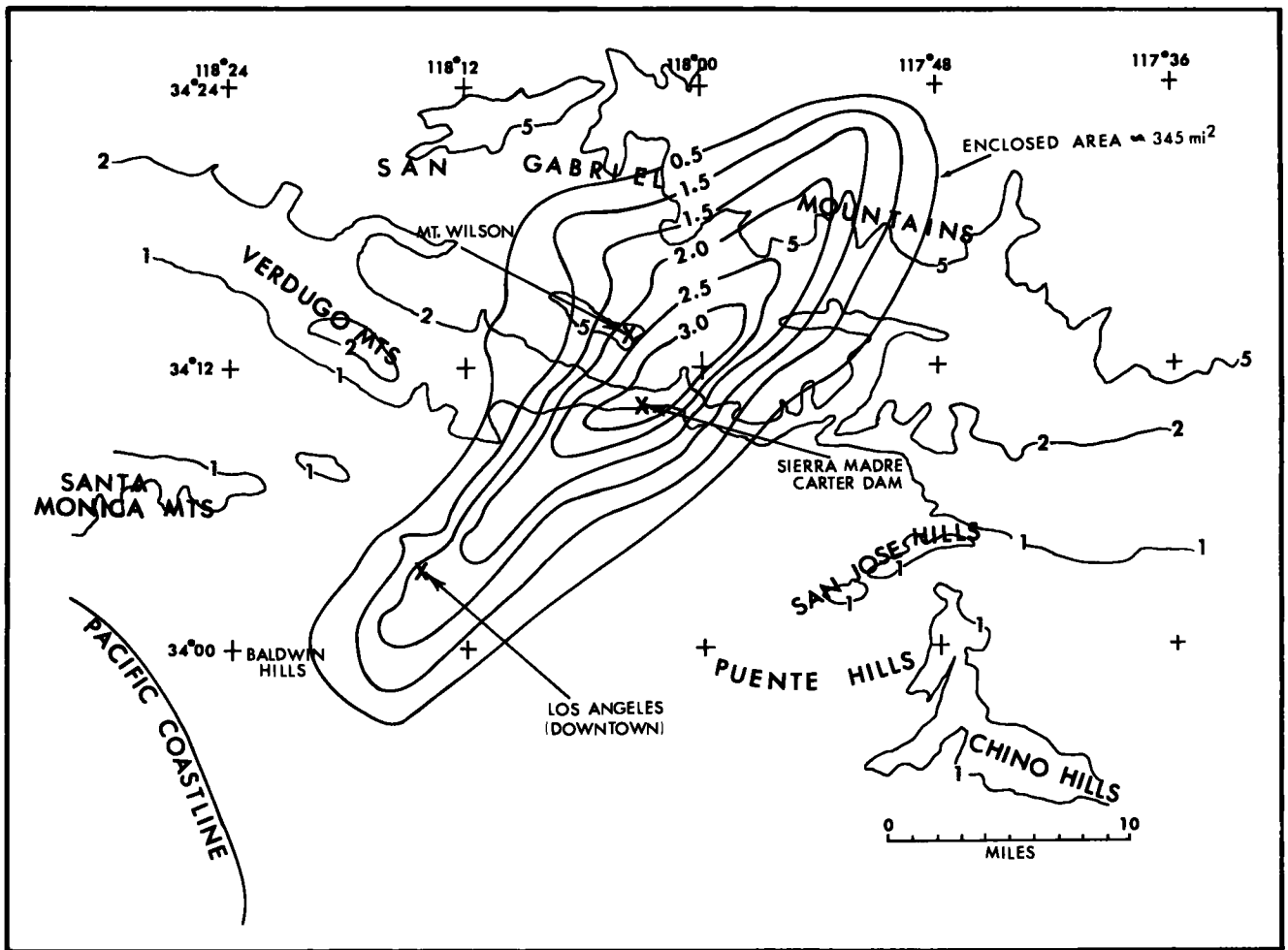
Figure 3.39.--Isohyetal map for storm of March 3, 1943.
