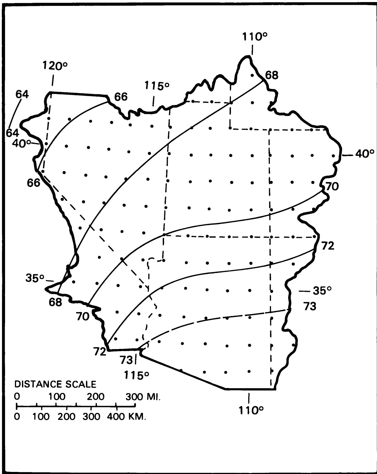
Figure 4.27.--1000-mb 12-hr persisting general storm dew point for mid-September.
