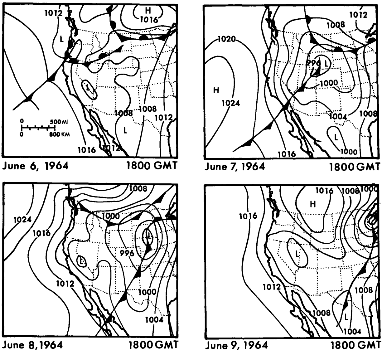
Figure 2.43.--Surface weather maps for June 6-9, 1964.
