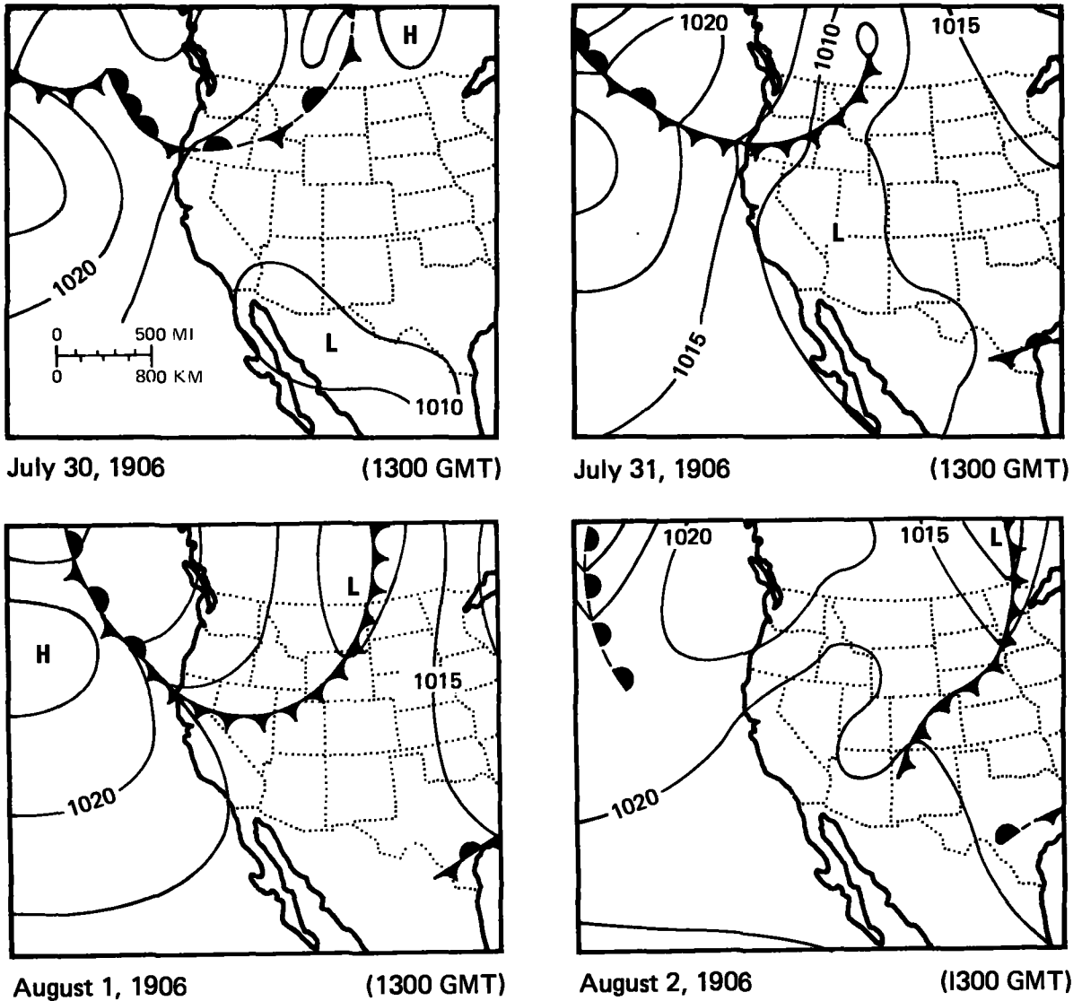
Figure 2.23.--Surface weather maps for July 30 to August 2, 1906.
