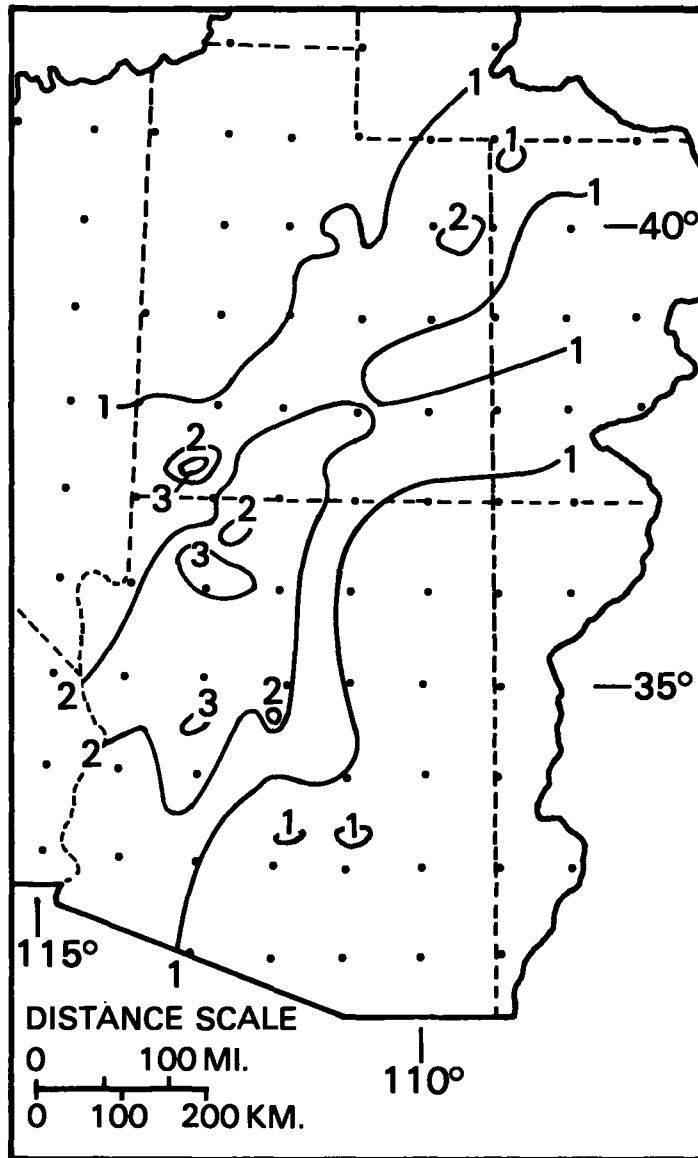
Figure 2.18.--Generalized isohyetal map for the storm of October 4-5, 1925.
