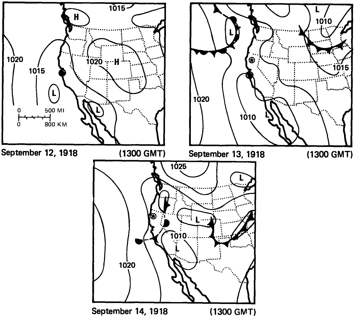
Figure 3.29.--Surface weather maps for September 12-14, 1918.
