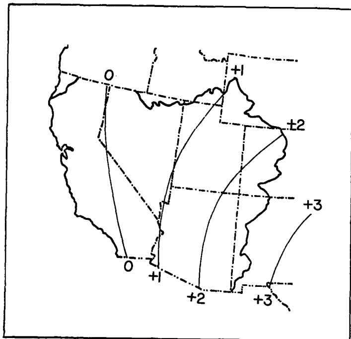
Figure 4.11.--Correction to maximum observed precipitable water to match values determined using 1000-mb 12-hr persisting dew point assuming saturated pseudo-adiabatic conditions.
