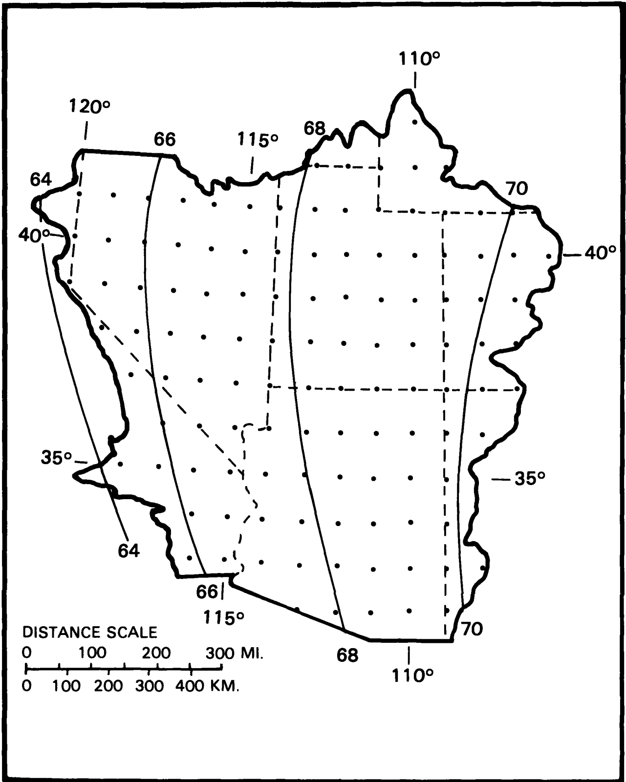
Figure 4.21.--1000-mb 12-hr persisting general storm dew point for mid-June.
