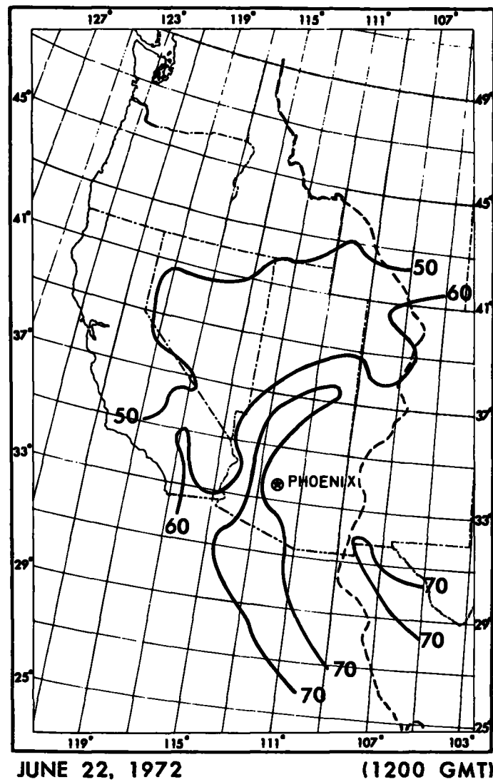
Figure 3.7.--Isodrosotherm analysis depicting moisture movement prior to storm of June 22, 1972.
