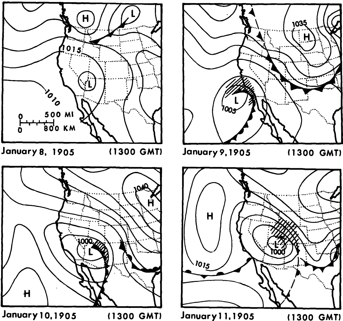
Figure 2.36.--Surface weather maps for January 8-11, 1905.
