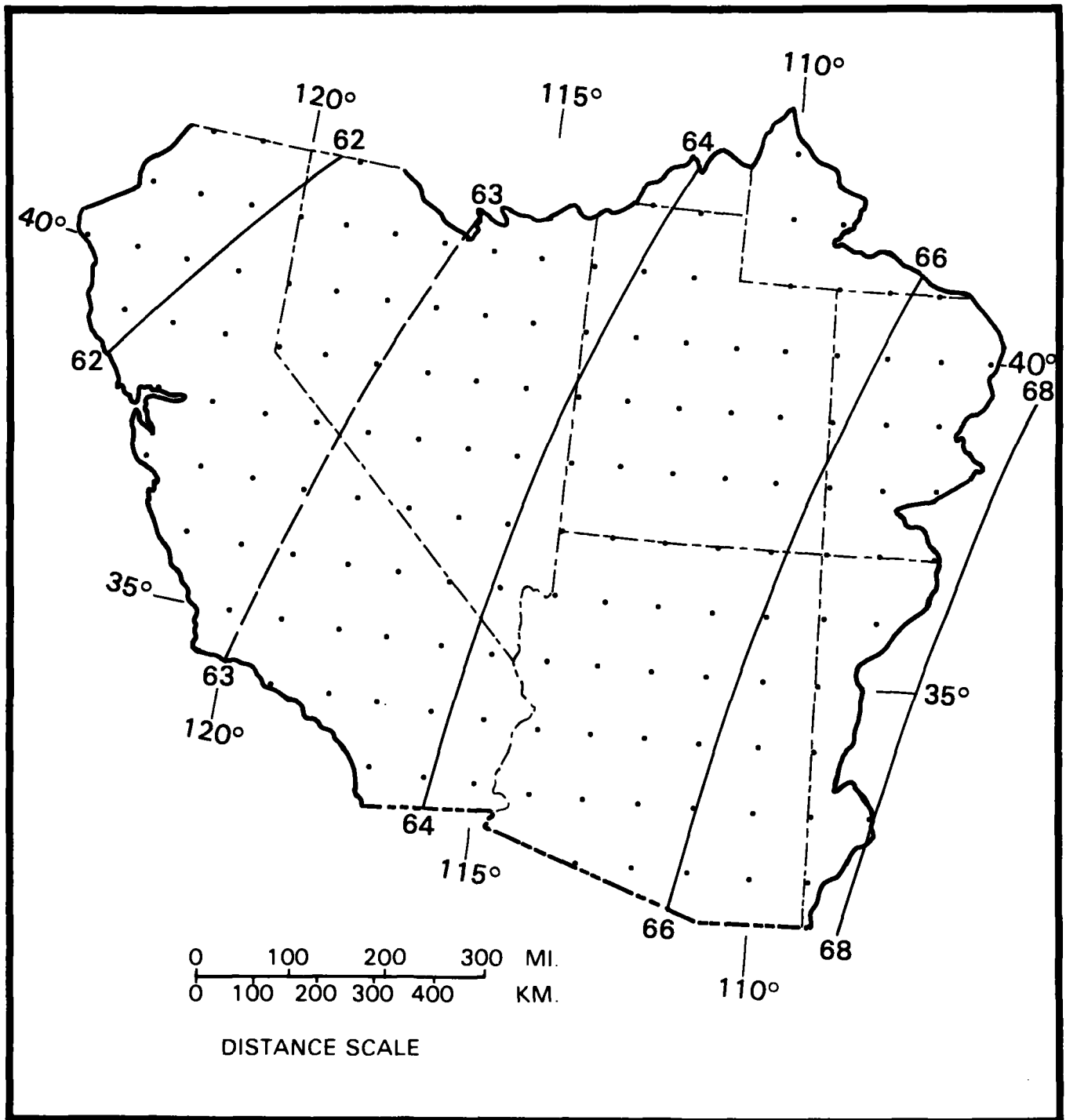
Figure 4.18.--1000-mb 12-hr persisting local storm dew point for mid-May.
