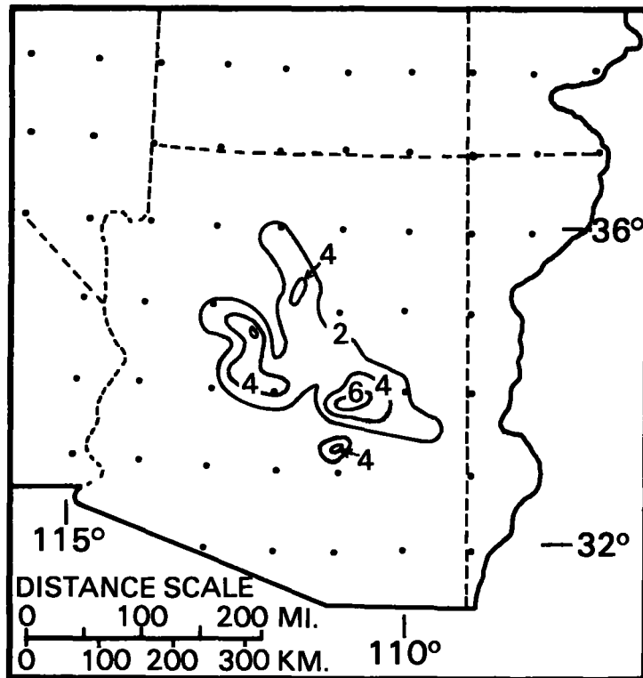
Figure 2.31.--Generalized isohyetal map for the storm of January 25-30, 1916.
