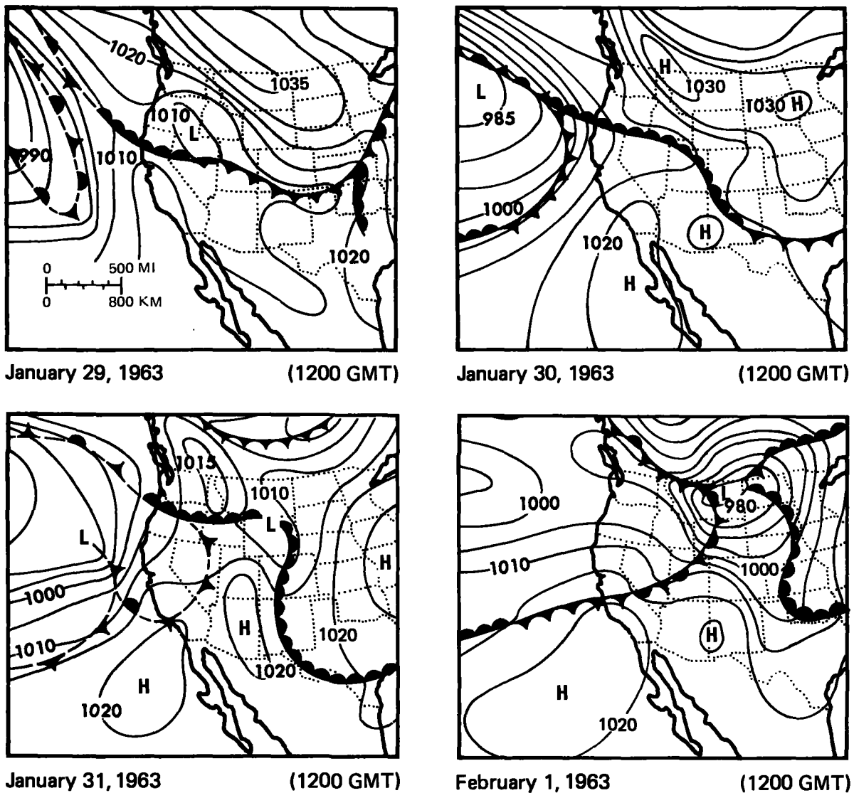
Figure 2.38. Surface weather maps for January 29 to February 1, 1963.
