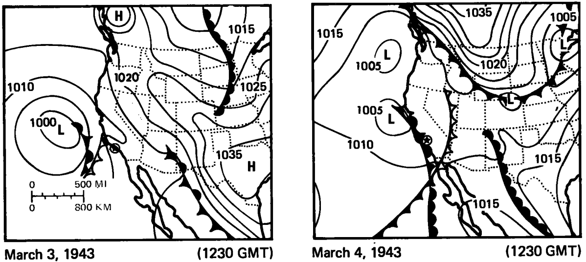
Figure 3.40.--Surface weather maps for March 3-4, 1943.
