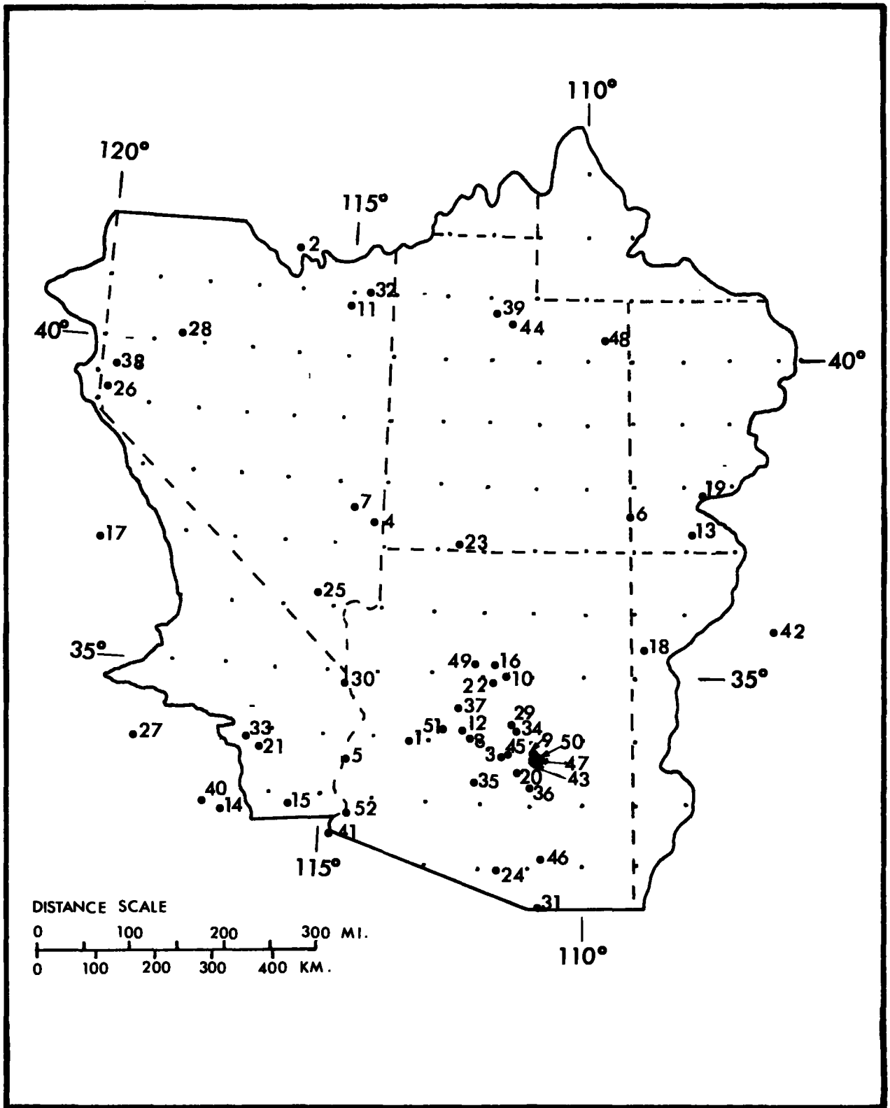
Figure 2.1.--Index map of Colorado River and Great Basin Drainages showing places referred to in chapter 2. Stations identified in table 2.1.
