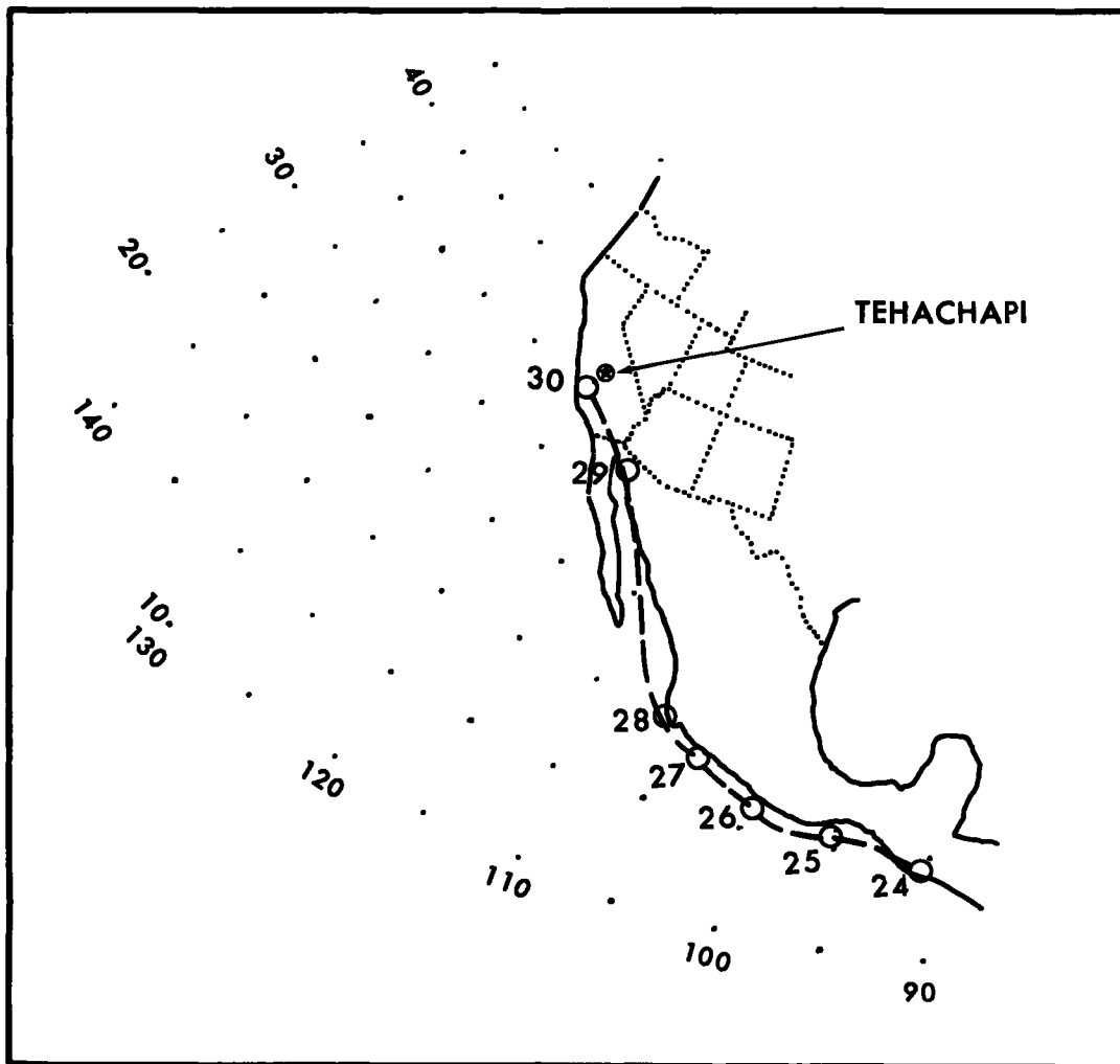
Figure 3.36.--Storm track for tropical cyclone that was important for the September 30, 1932 storm at Tehachapi, Calif.
