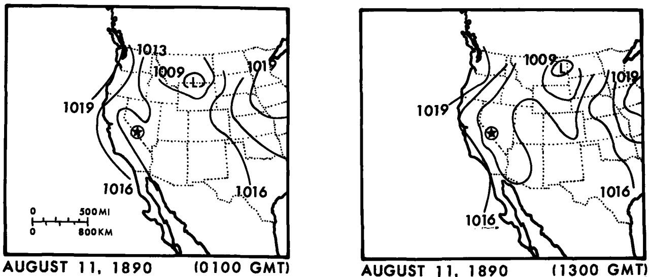
Figure 3.19.--Surface weather maps for August 11, 1890.
