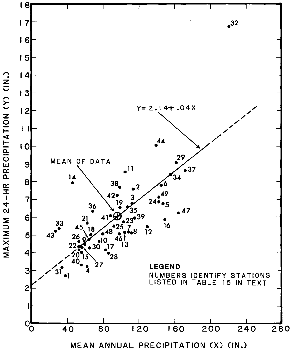
Figure 21.—Maximum observed 24-hr precipitation vs. mean annual precipitation for southeast Alaska.
