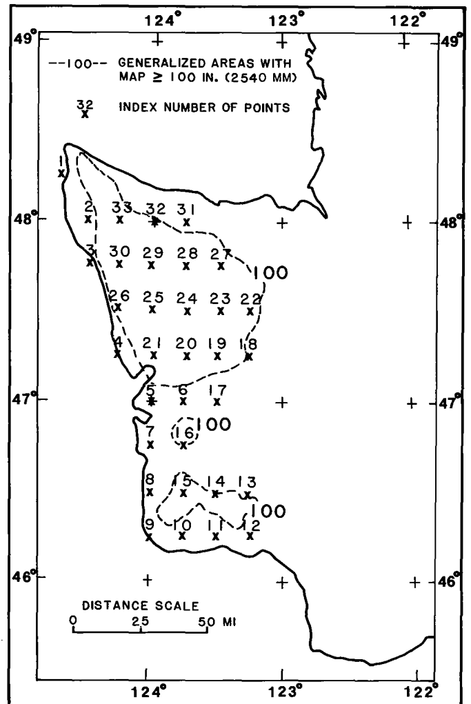
Figure 14.—Location of western Washington points used for probable maximum precipitation vs. mean annual precipitation relation.
