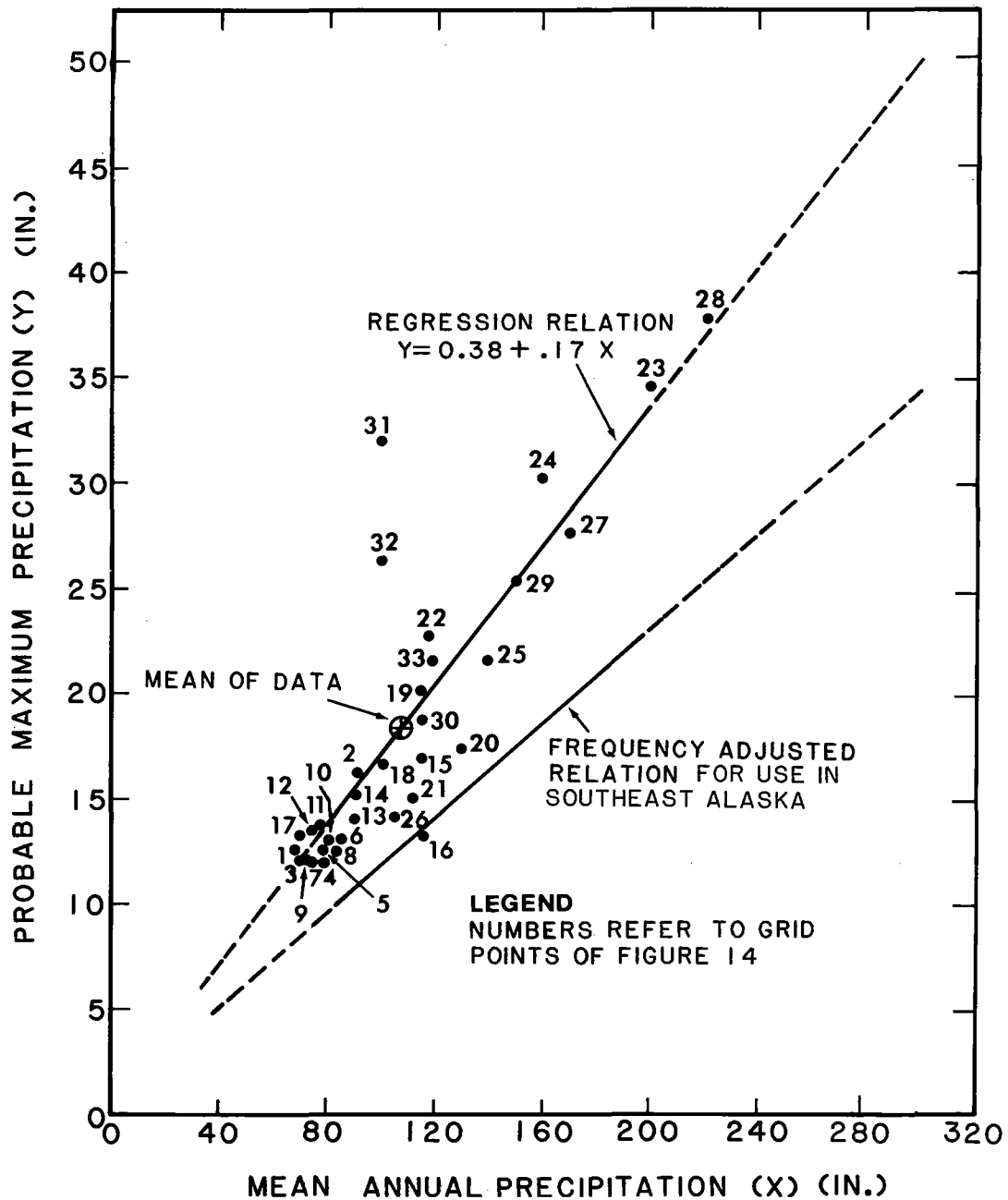
Figure 15.—24-hr 10-mi 2 probable maximum precipitation vs. mean annual precipitation from western Washington data.
