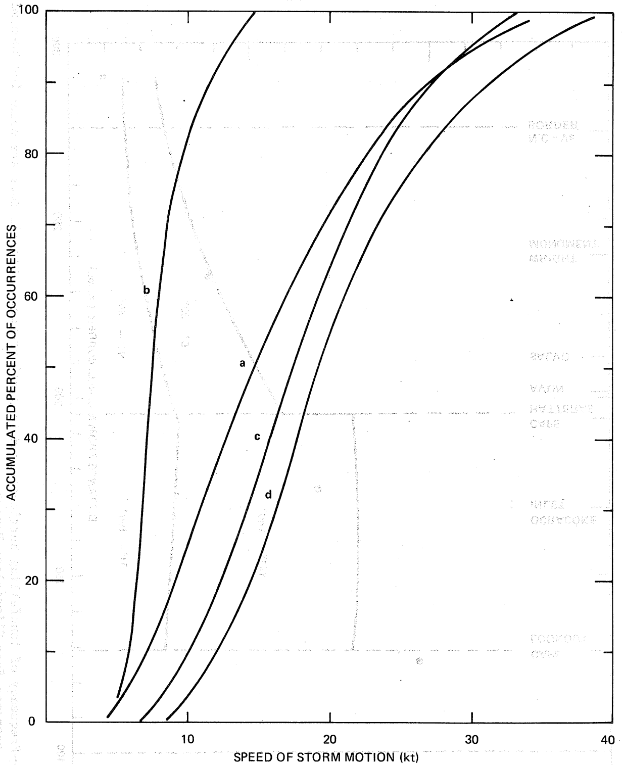
Figure 6.--Probability distributions of speed of storm motion adapted for Wright Monument, N.C., for (a) landfalling storms from the southeast quadrant and exiting storms, (b) landfalling storms from the northeast quadrant, (c) inland storms, and (d) alongshore storms.
