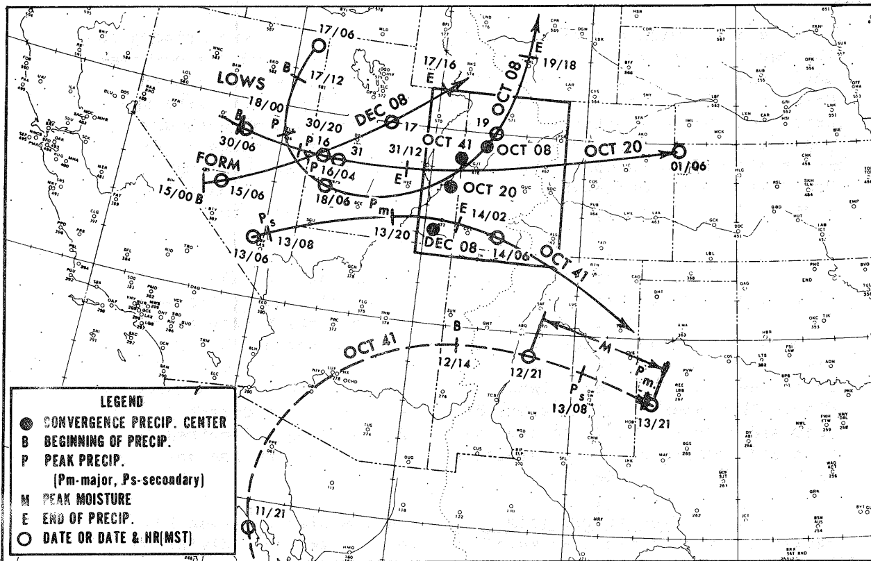
Figure 4-4 Tracks of 700-mb moisture (---) and 500-mb Lows (—) in HL-C type storms. Month and year are shown for tracks and convergence precipitation centers.
