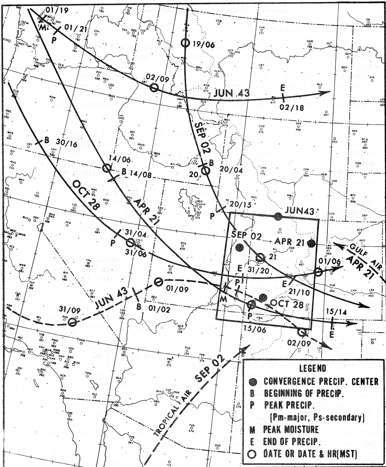
Figure 4-1. Tracks of 700-mb moisture (---) and 500-mb Lows (—) in HBL type storms. Month and year are shown for tracks and convergence precipitation centers.
