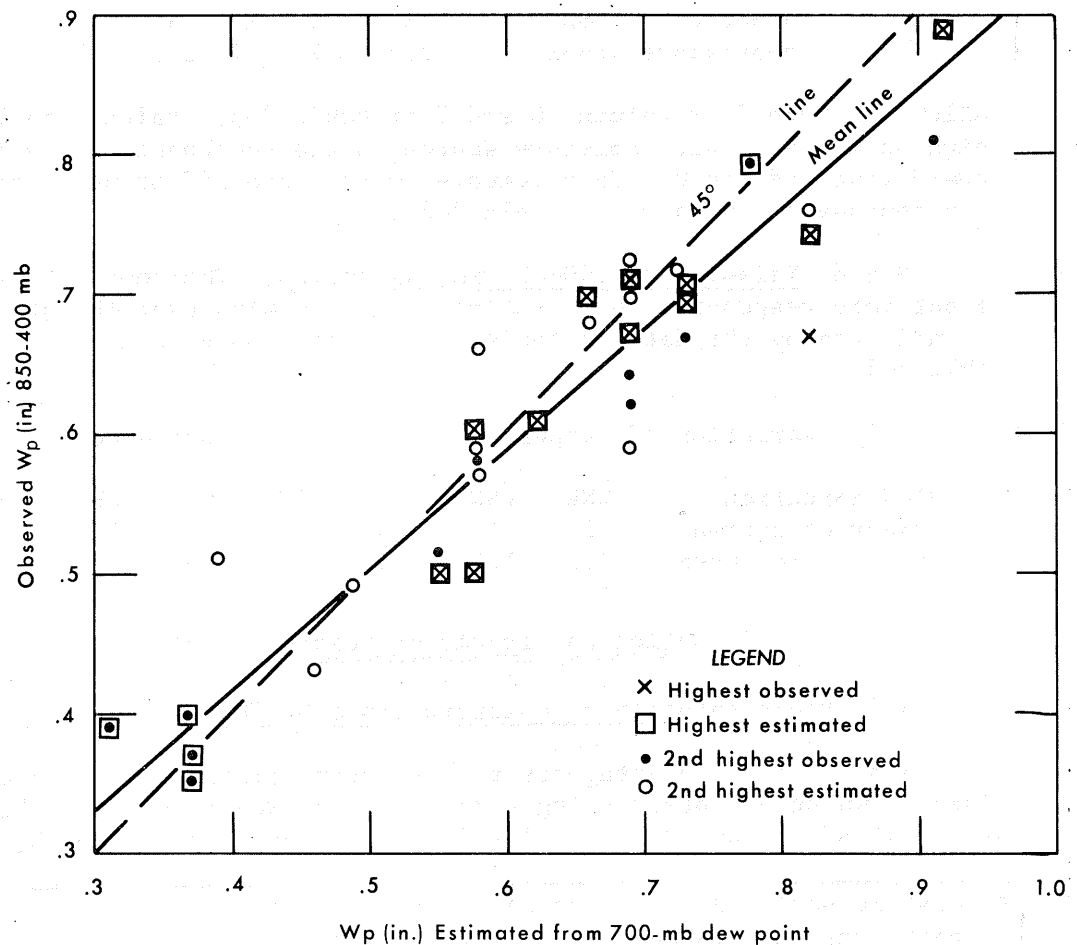
Figure 3-6. Relation between observed 850- to 400-mb precipitable water at Grand Junction and that estimated from 700-mb dew point assuming a moist adiabatic lapse rate. Data are from qualifying and near-qualifying storms 1949 to 1965.
