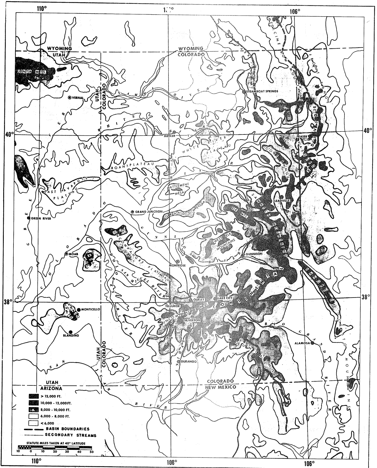
Figure 1-1. Topographic map of western Colorado and eastern Utah.
