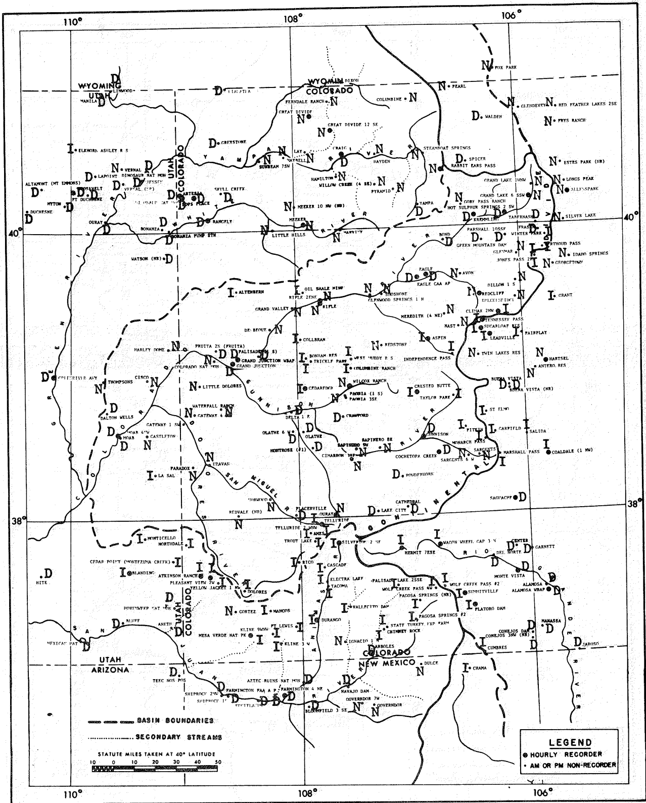
Figure 5-8. Local terrain effects on precipitation for southerly 500-mb winds. Letters indicate effects, observed in storms or estimated, to be depletion (D), no effect (N), or increase (I).
