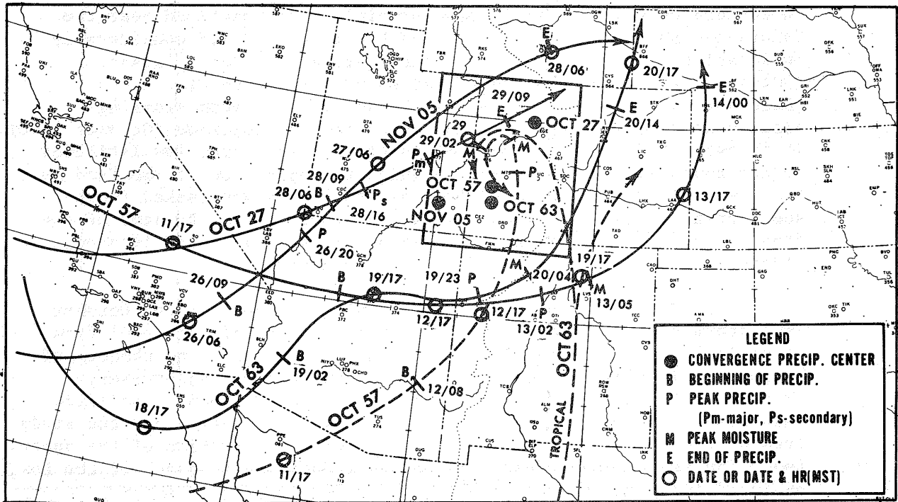
Figure 4-5a. Tracks of 700-mb moisture (---) and 500-mb Lows (—) in C-West type storms. Month and year are shown for tracks and convergence precipitation centers.
