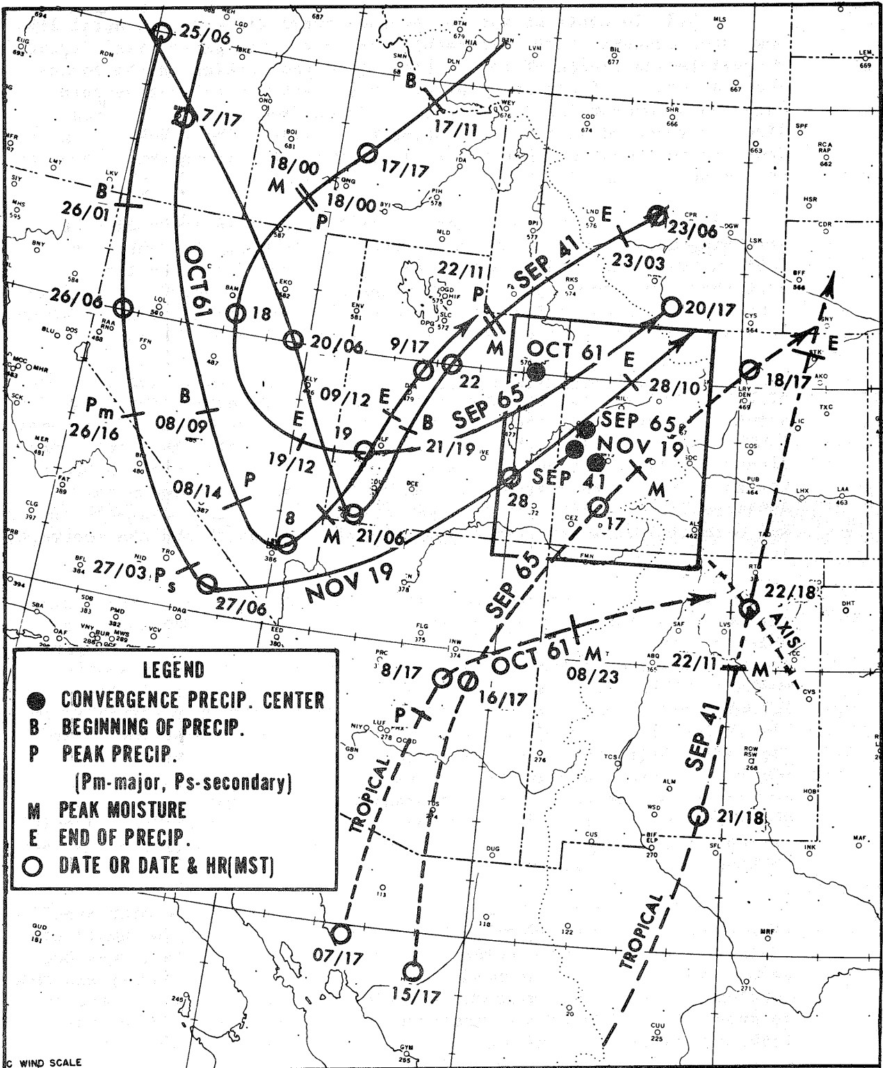
Figure 4-2. Tracks of 700-mb moisture (---) and 500-mb Lows (—) in HBL-C type storms. Month and year are shown for tracks and convergence precipitation centers.
