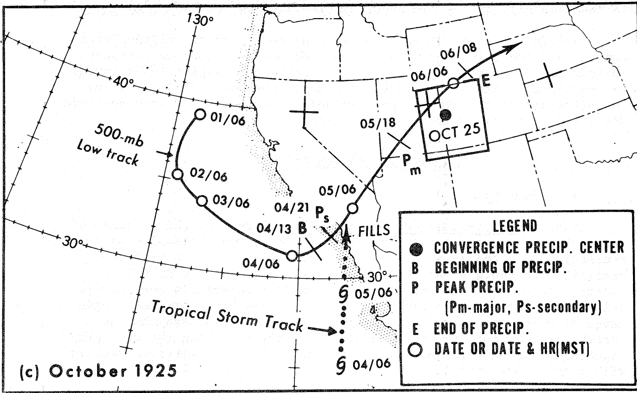
Figure 4-8. Tracks of tropical storms and positions of auxiliary troughs (---) and/or Low tracks (—) at 500 mbs.
