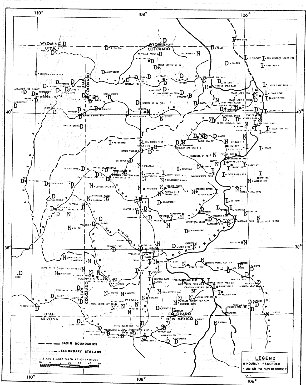
Figure 5-7. Local terrain effects on precipitation for southeasterly 500-mb winds. Letters indicate effects, observed in storms or estimated, to be depletion (D), no effect (N), or increase (I).
