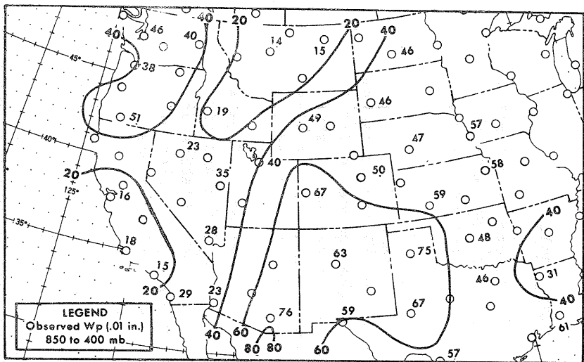
Figure 3-7. Comparison of precipitation water observed in the 850-to 400-mb layer, 1700MST October 8, 1961 with that estimated from 700-mb dew point, assuming saturation.
