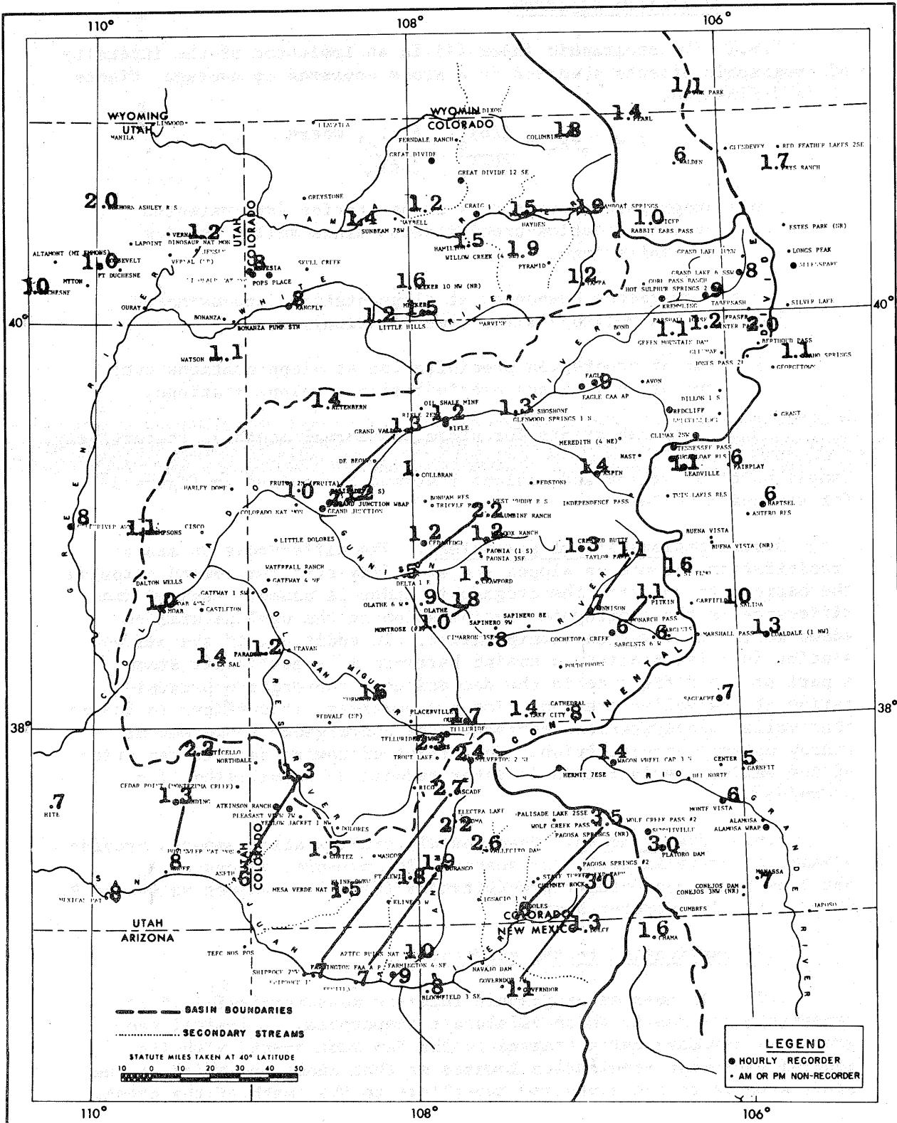
Figure 5-1. Mean October precipitation (in.). Lines connect preferred station pairs for determining orographic indices.
