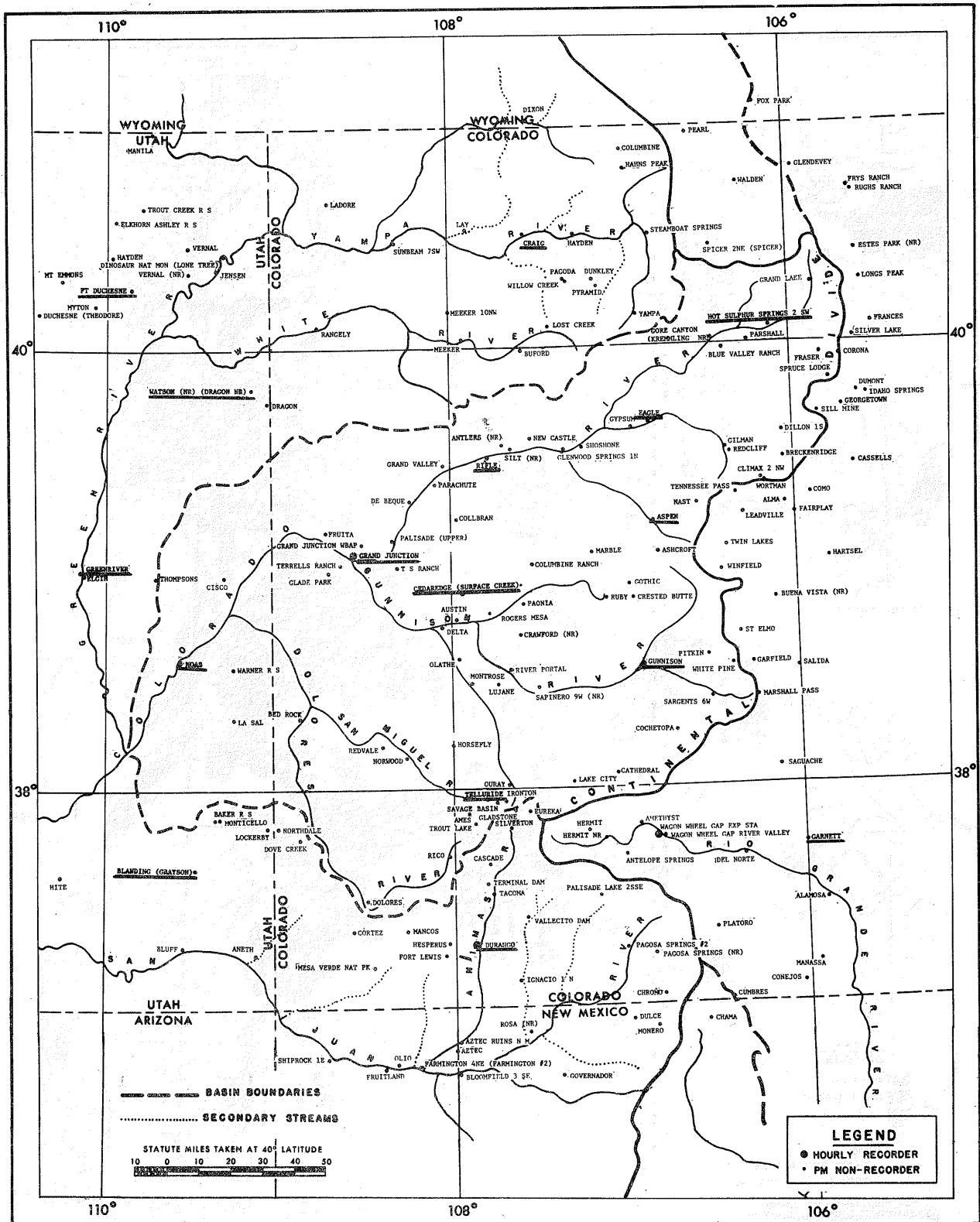
Figure 1-2. Map of precipitation stations in the study area for the period 1899 to 1932. (Key stations for selection of qualifying storms are underlined.)
