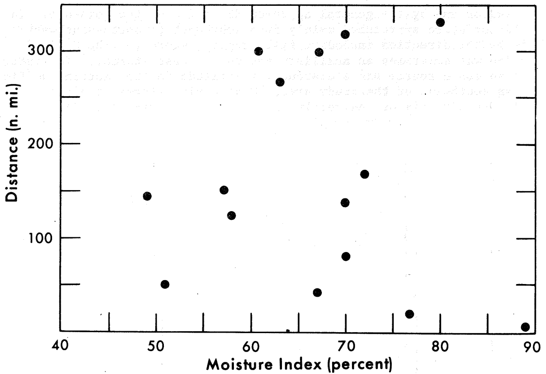
Figure 3-10. Comparison of storm moisture index with shortest distance (n.m.) from the precipitation center to the track of the moisture pool.
