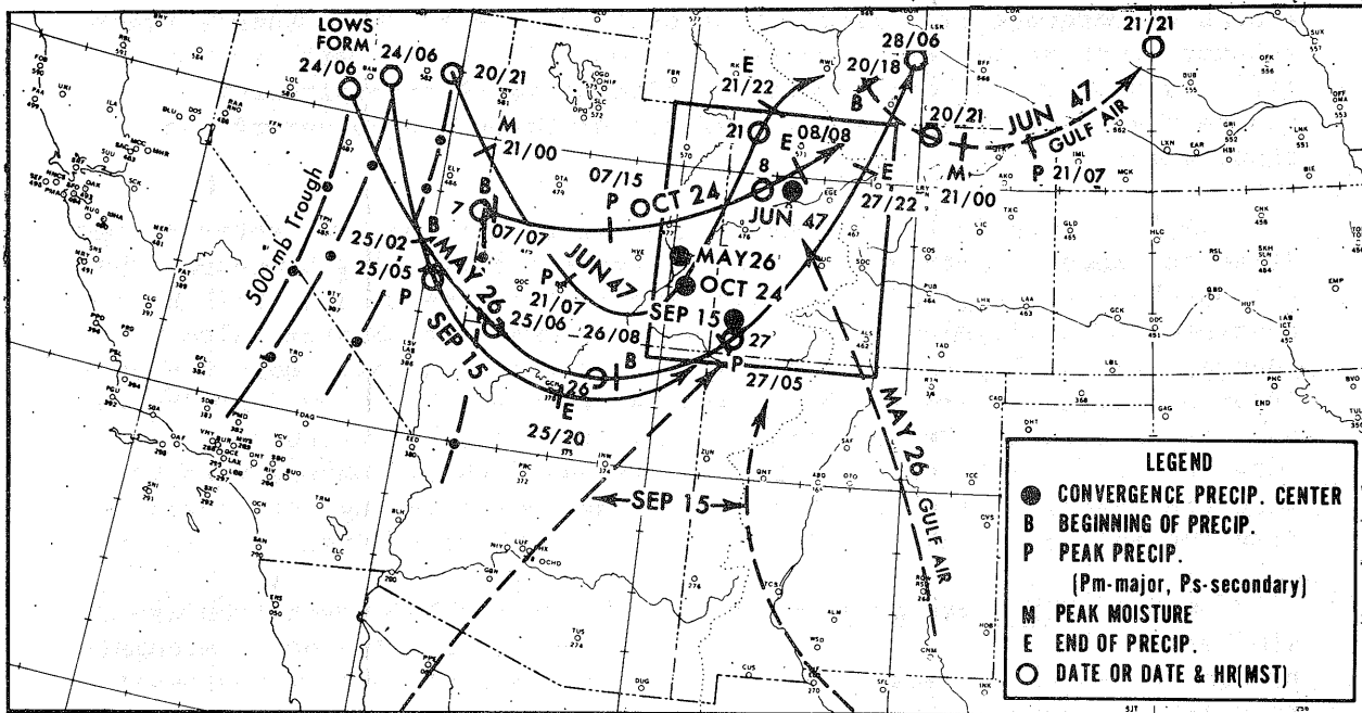
Figure 4-3. Tracks of 700-mb moisture (---) and 500-mb Lows (—) in HBT-C type storms. Troughs are shown by (—●—) on date Low forms. Month and year are shown for tracks and convergence precipitation centers.
