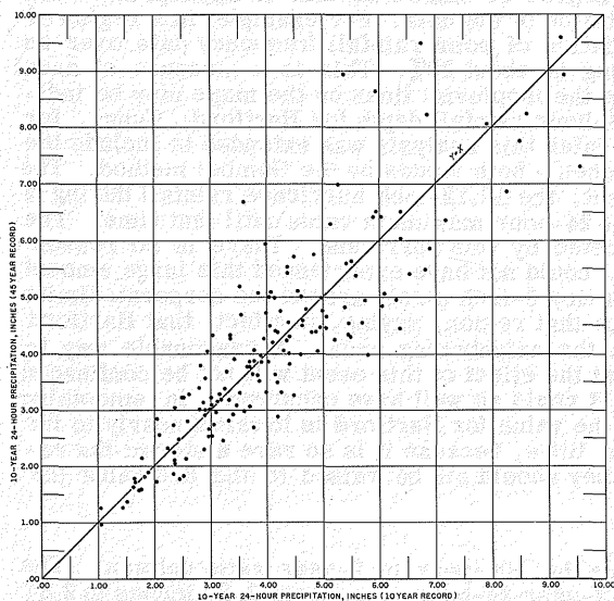
FIGURE 4. COMPARISON OF 10-YEAR 24-HOUR PRECIPITATION BASED ON 10 YEAR AND 45 YEAR RECORDS. AVERAGE DIFFERENCE IS APPROXIMATELY 15 %
