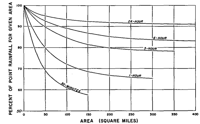
FIGURE 15.—Area-depth curves.
