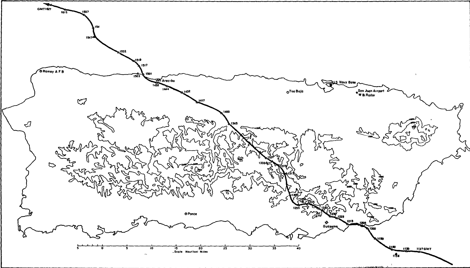
FIGURE 2-5.—Track of hurricane Betsy across Puerto Rico, August 12, 1956 (after Colón)
