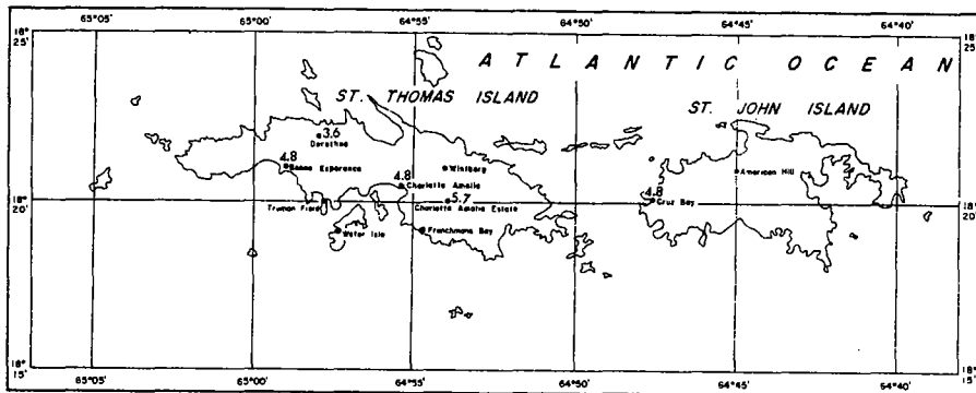
FIGURE 4-81.—25-yr. 3-hr. rainfall for Virgin Islands (in.).
