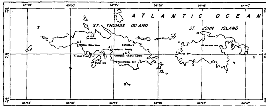
FIGURE 4-85.—2-yr. 6-hr. rainfall for Virgin Islands (in.).
