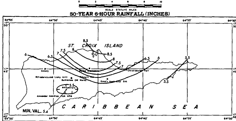
FIGURE 4-89.—50-yr. 6-hr. rainfall for Virgin Islands (in.).
