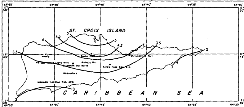
FIGURE 4-69.—100-yr. 1-hr. rainfall for Virgin Islands (in.).
