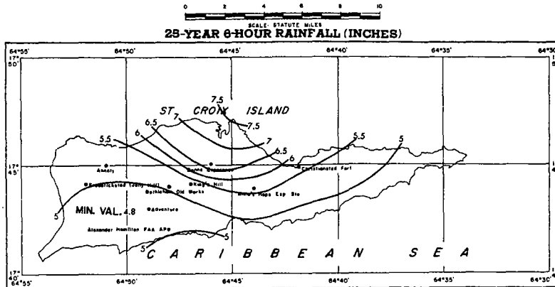
FIGURE 4-88.—25-yr. 6-hr. rainfall for Virgin Islands (in.)
