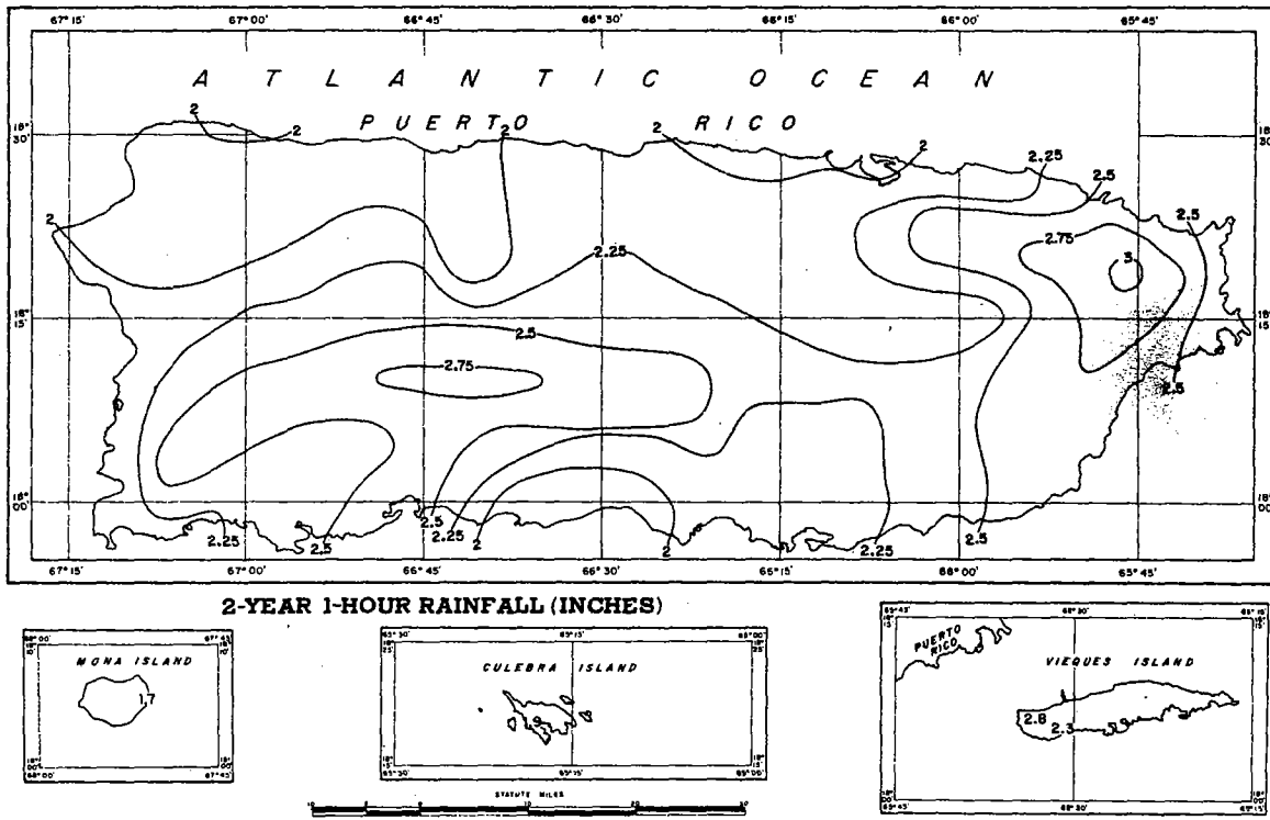
FIGURE 4-15.—2-yr. 1-hr. rainfall for Puerto Rico (in.).
