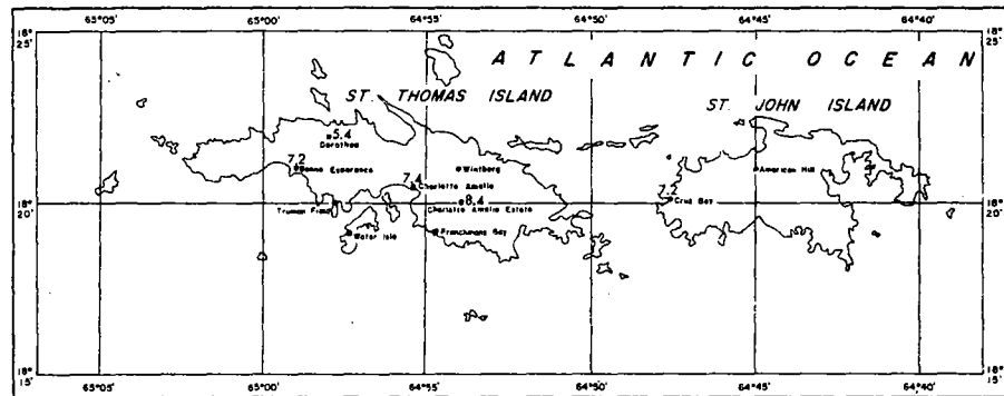
FIGURE 4-89.—50-yr. 6-hr. rainfall for Virgin Islands (in.).
