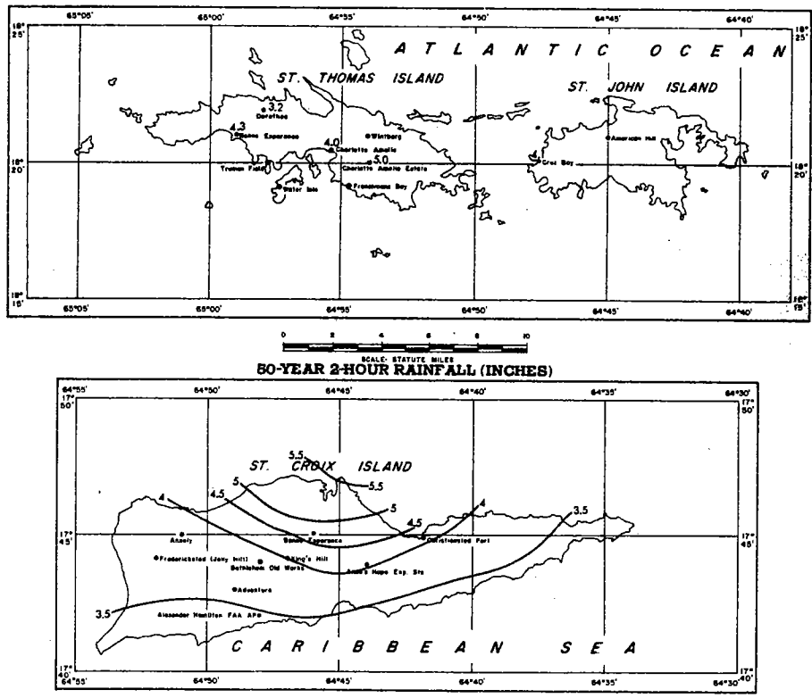
FIGURE 4-75.—50-yr. 2-hr. rainfall for Virgin Islands (in.).
