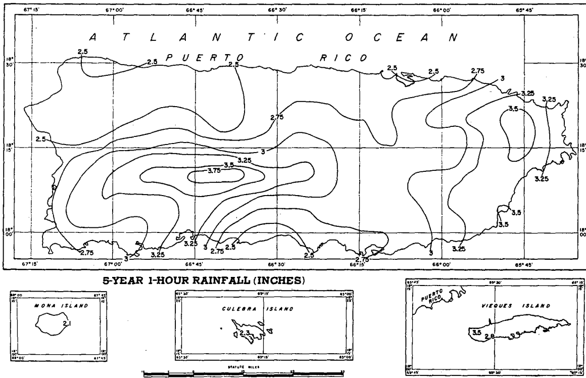
FIGURE 4-16.—5-yr. 1-hr. rainfall for Puerto Rico (in.).
