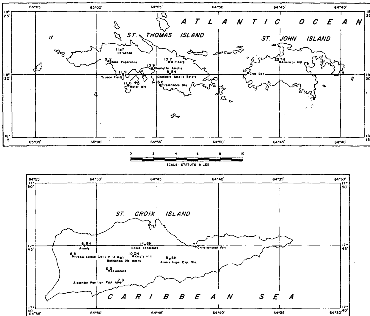
FIGURE 1-2.—Adjusted maximum observed 24-hr. rainfalls (in.) for Virgin Islands. The letter “H” indicates that the rainfall was associated with a hurricane
