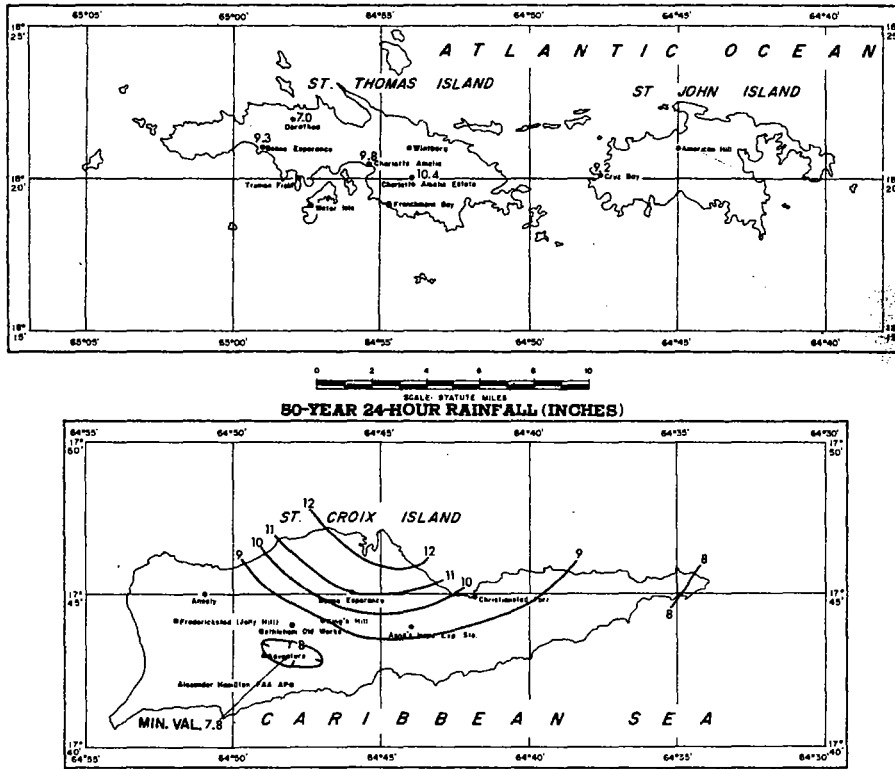
FIGURE 4-103.—50-yr. 24-hr. rainfall for Virgin Islands (in.).
