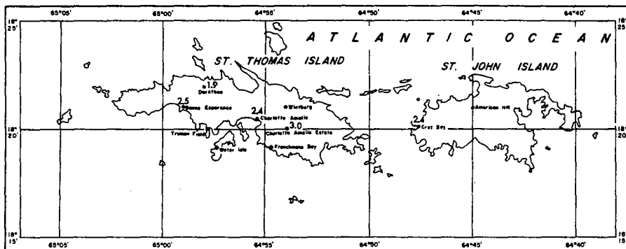
SCALE, STATUTE MILES 25-YEAR 30-MINUTE RAINFALL (INCHES)
