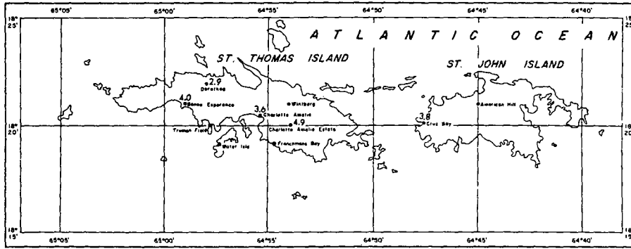
100-YEAR 1-HOUR RAINFALL (INCHES)
