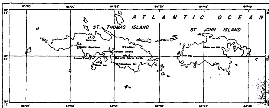
100-YEAR 3-HOUR RAINFALL (INCHES)
