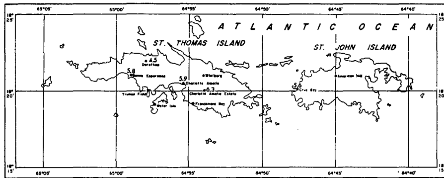
FIGURE 4-93.—5-yr. 12-hr. rainfall for Virgin Islands (in.).
