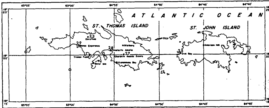
1-YEAR 12-HOUR RAINFALL (INCHES)
