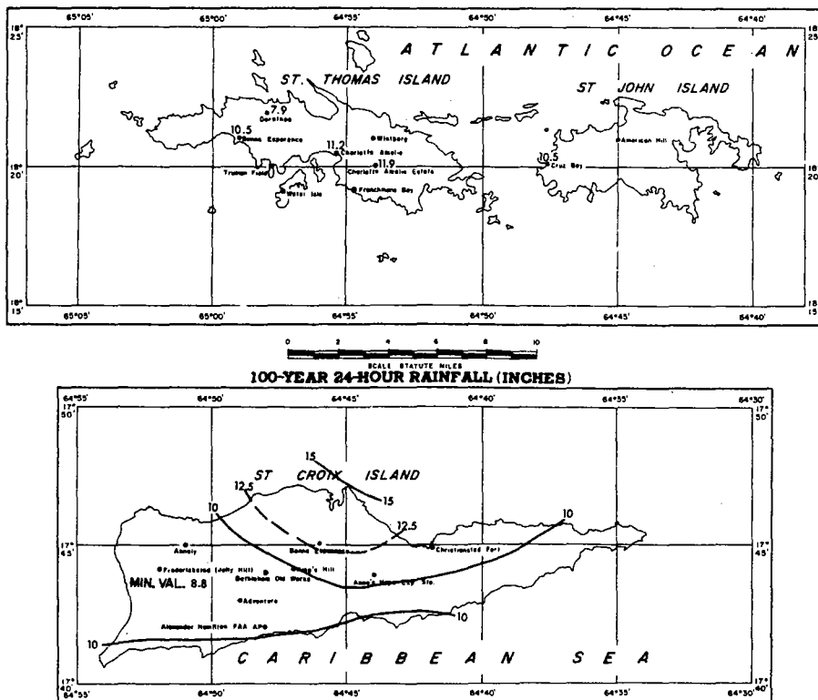
FIGURE 4-104.—100-yr. 24-hr. rainfall for Virgin Islands (in.).
