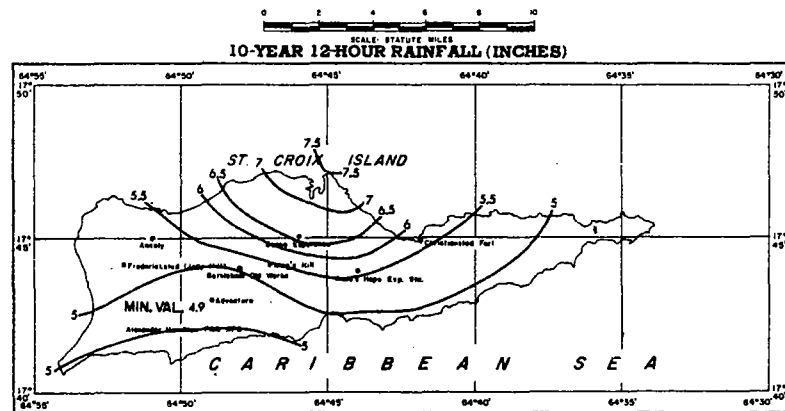
FIGURE 4-94.—10-yr. 12-hr. rainfall for Virgin Islands (in.).
