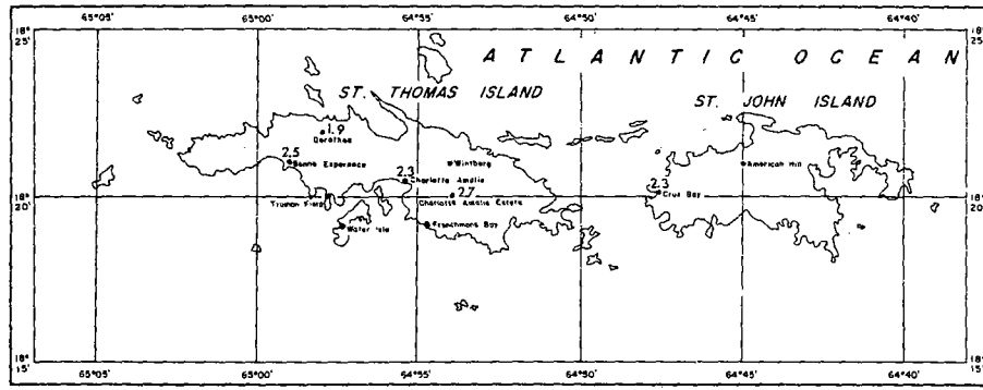
SCALE: STATUTE MILES 5-YEAR 1-HOUR RAINFALL (INCHES)
