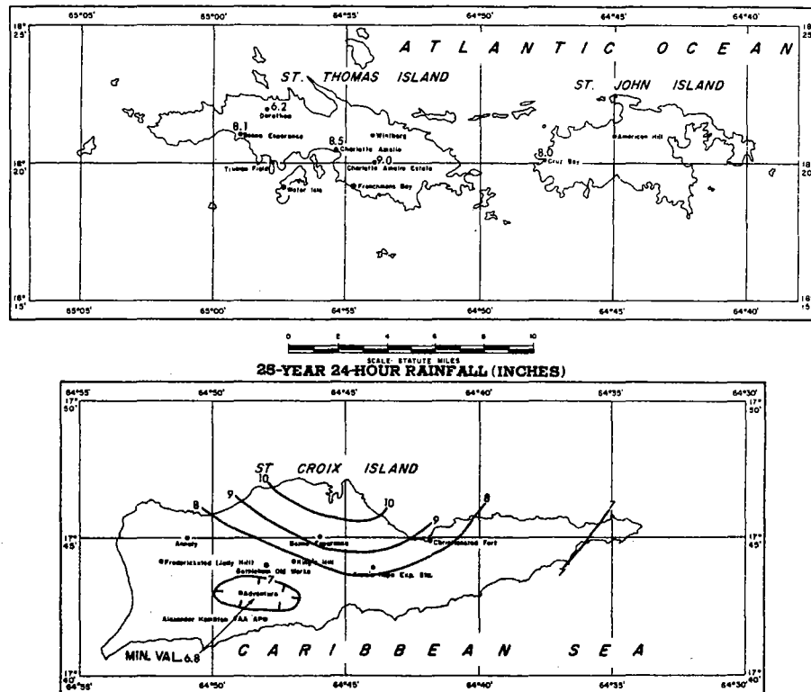
FIGURE 4-102.—25-yr. 24-hr. rainfall for Virgin Islands (in.).
