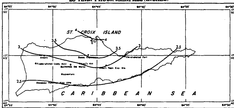
FIGURE 4-67.—25-yr. 1-hr. rainfall for Virgin Islands (in.).
