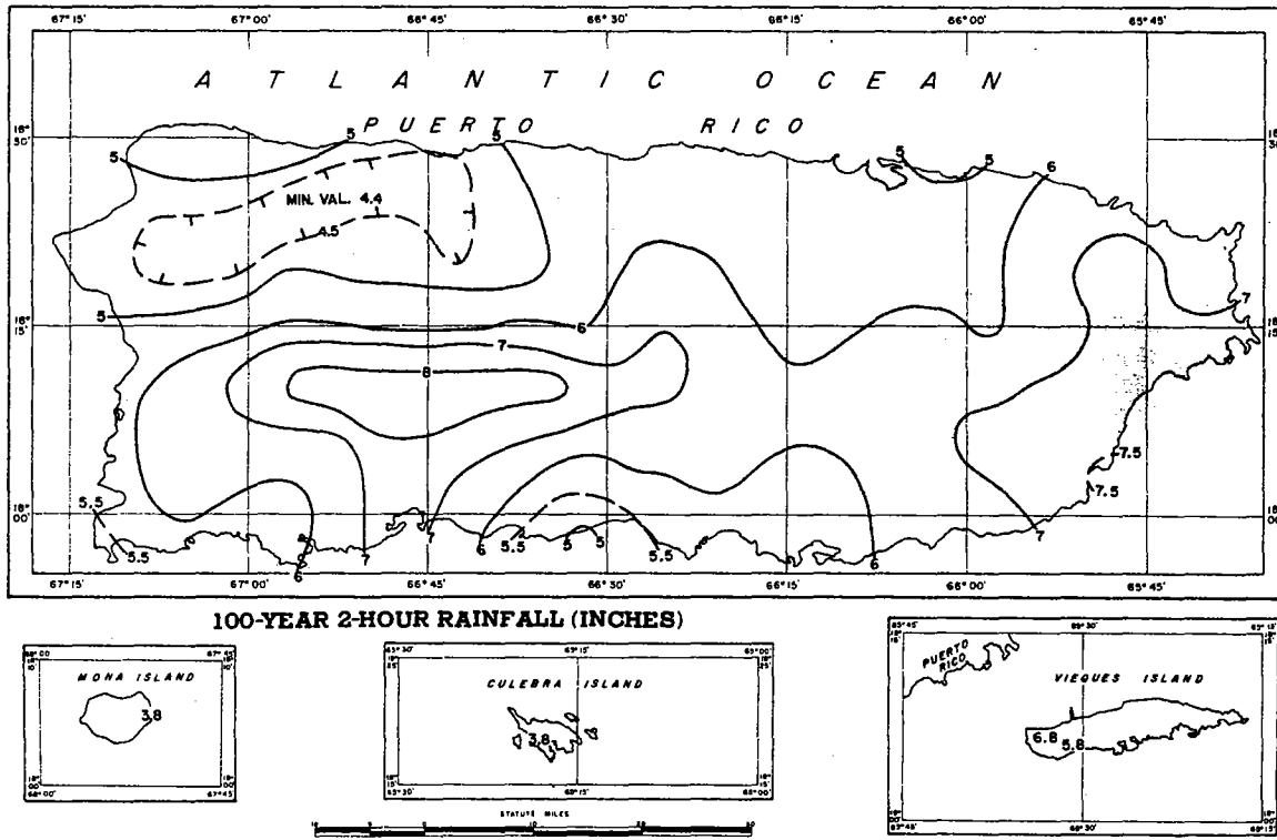
FIGURE 4-27.—100-yr. 2-hr. rainfall for Puerto Rico (in.).
