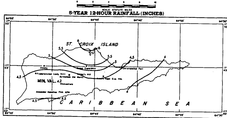
FIGURE 4-93.—5-yr. 12-hr. rainfall for Virgin Islands (in.).
