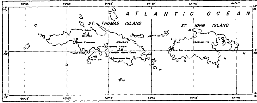
1-YEAR 2-HOUR RAINFALL (INCHES)
