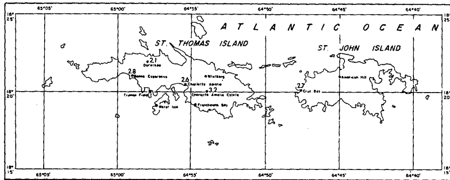
SCALE: STATUTE MILES 10-YEAR 1-HOUR RAINFALL (INCHES)
