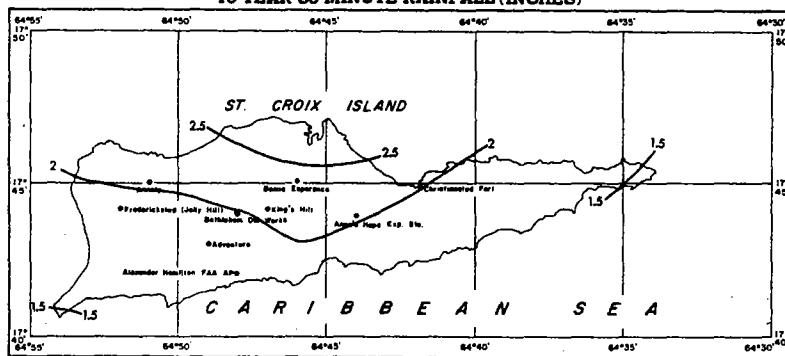
FIGURE 4-59.—10-yr. 30-min. rainfall for Virgin Islands (in.).
