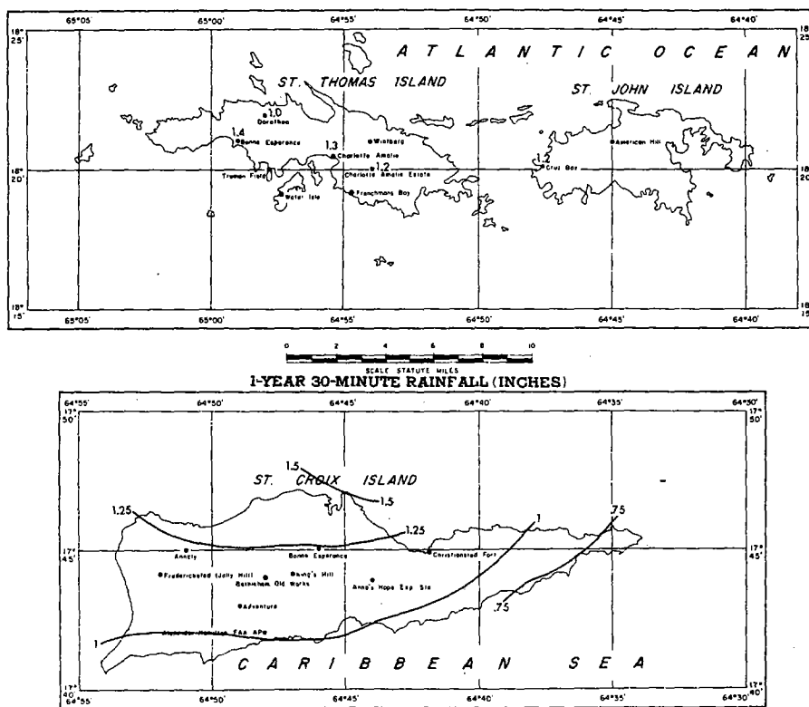
FIGURE 4-56.—1-yr. 30-min. rainfall for Virgin Islands (in.)
