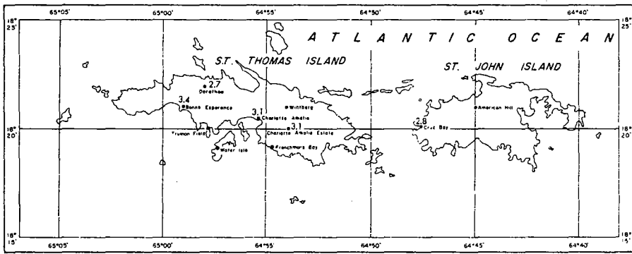
FIGURE 4-97.—100-yr. 12-hr. rainfall for Virgin Islands (in.).
