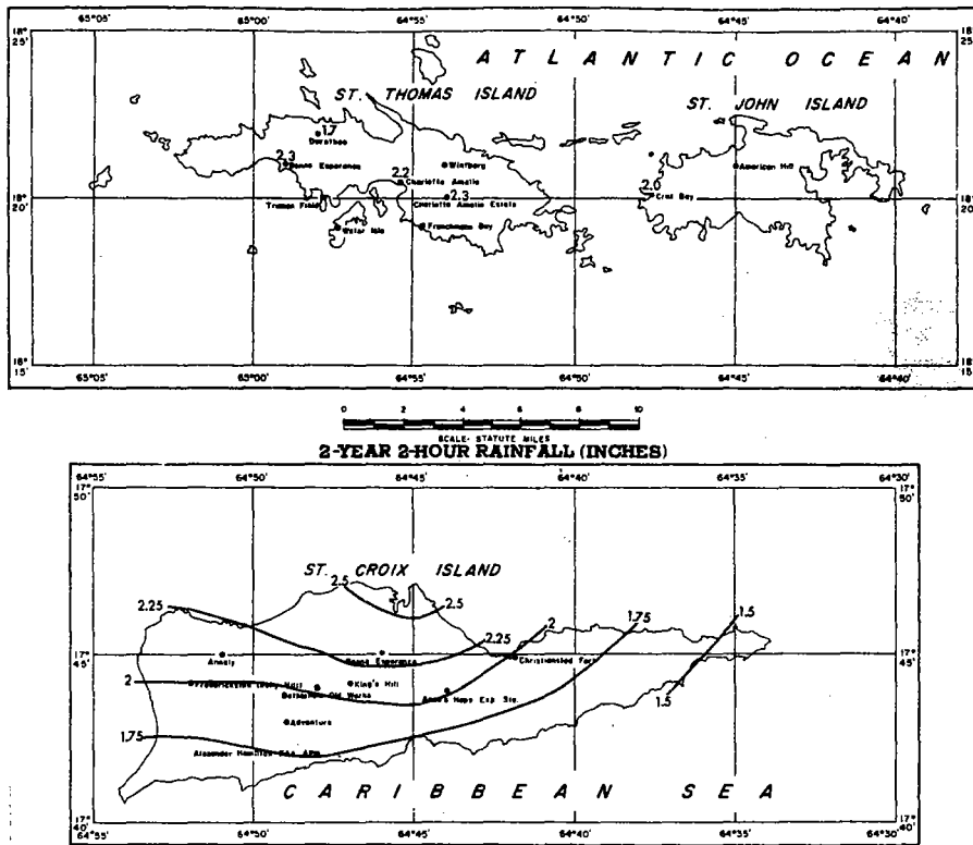
FIGURE 4-71.—2-yr. 2-hr. rainfall for Virgin Islands (in.).
