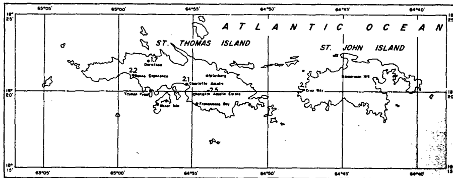
SCALE, STATUTE MILES 10-YEAR 30-MINUTE RAINFALL (INCHES)
