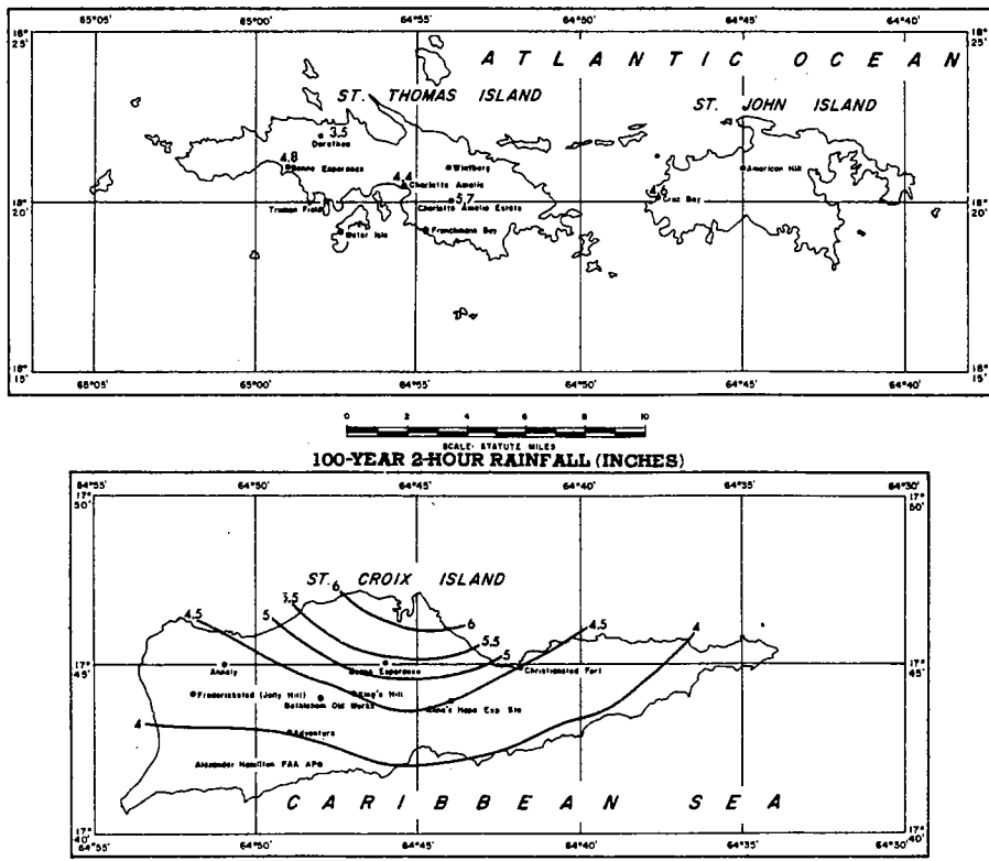
FIGURE 4-76.—100-yr. 2-hr. rainfall for Virgin Islands (in.).
