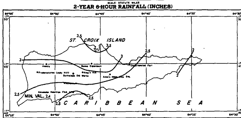
FIGURE 4-85.—2-yr. 6-hr. rainfall for Virgin Islands (in.).
