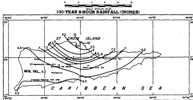
FIGURE 4-90.—100-yr. 6-hr. rainfall for Virgin Islands (in.).
