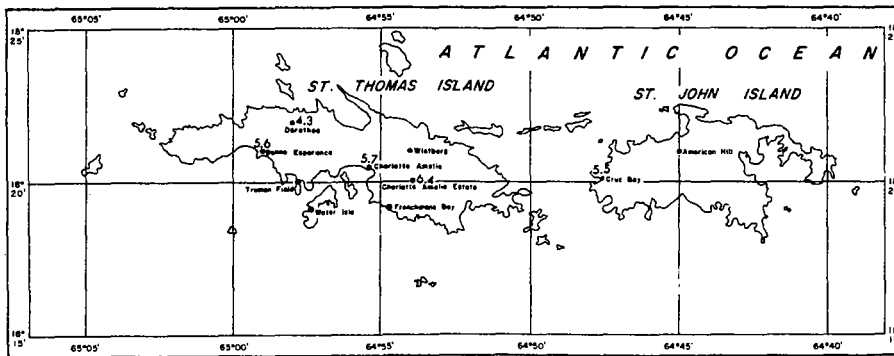
FIGURE 4-87.—10-yr. 6-hr. rainfall for Virgin Islands (in.).
