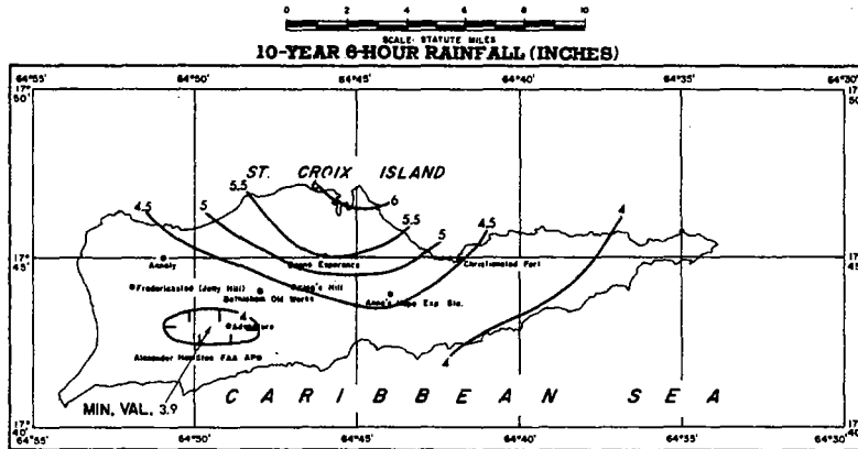
FIGURE 4-87.—10-yr. 6-hr. rainfall for Virgin Islands (in.).
