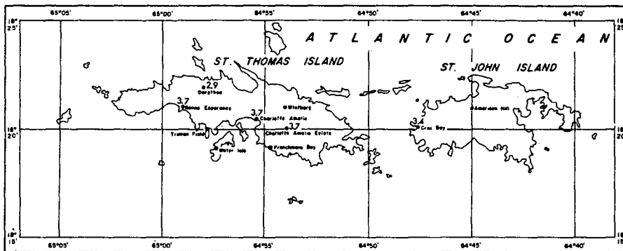
2-YEAR 12-HOUR RAINFALL (INCHES)
