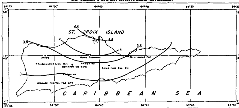
FIGURE 4-68.—50-yr. 1-hr. rainfall for Virgin Islands (in.).
