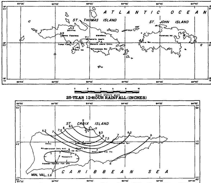
FIGURE 4-95.—25-yr. 12-hr. rainfall for Virgin Islands (in.).
