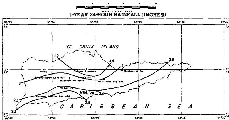
FIGURE 4-98.—1-yr. 24-hr. rainfall for Virgin Islands (in.).
