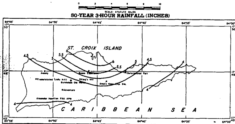
FIGURE 4-82.—50-yr. 3-hr. rainfall for Virgin Islands (in.).
