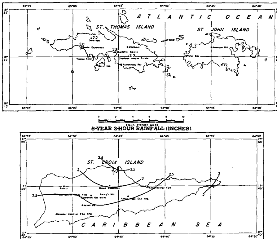
FIGURE 4-72.—5-yr. 2-hr. rainfall for Virgin Islands (in.).
