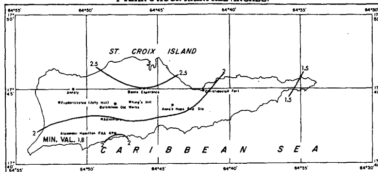
FIGURE 4-84.—1-yr. 6-hr. rainfall for Virgin Islands (in.).
