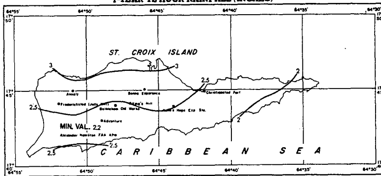
FIGURE 4-91.—1-yr. 12-hr. rainfall for Virgin Islands (in.).
