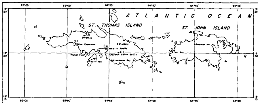
FIGURE 4-79.—5-yr. 3-hr. rainfall for Virgin Islands (in.).
