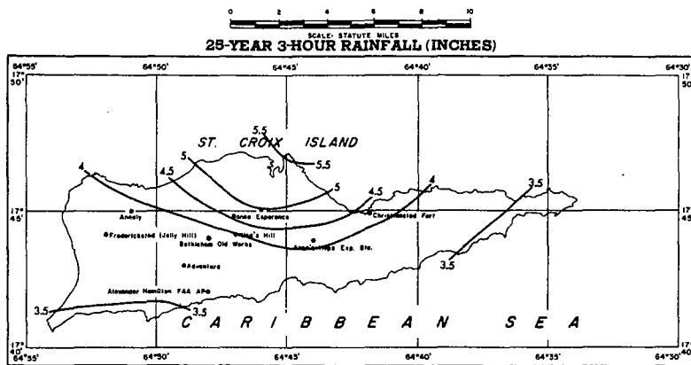
FIGURE 4-81.—25-yr. 3-hr. rainfall for Virgin Islands (in.).
