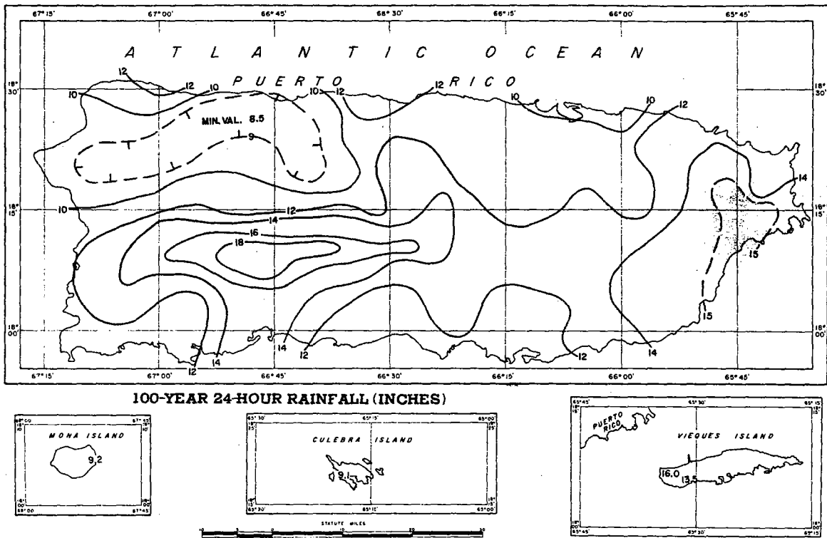
FIGURE 4-55.—100-yr. 24-hr. rainfall for Puerto Rico (in.)
