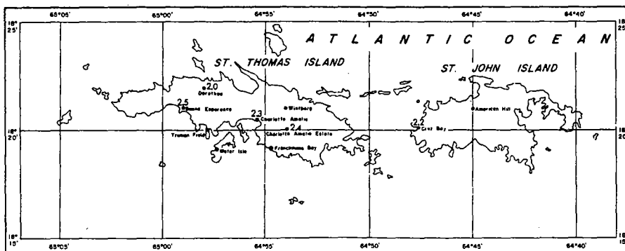
1-YEAR 6-HOUR RAINFALL (INCHES)
