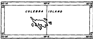
1-YEAR 12-HOUR RAINFALL (INCHES)
