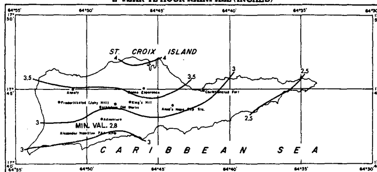
FIGURE 4-92.—2-yr. 12-hr. rainfall for Virgin Islands (in.).
