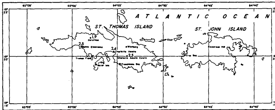
FIGURE 4-77.—1-yr. 3-hr. rainfall for Virgin Islands (in.).
