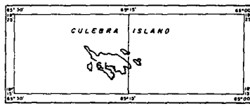
100-YEAR 6-HOUR RAINFALL (INCHES)
