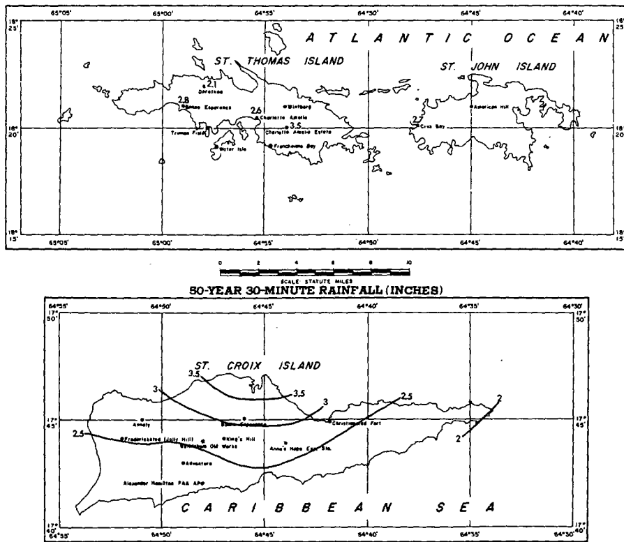
FIGURE 4-61.—50-yr. 30-min. rainfall for Virgin Islands (in.).
