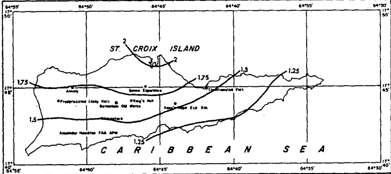
FIGURE 4-70.—1-yr 2-hr rainfall for Virgin Islands (in.).
