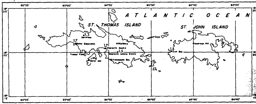
SCALE: STATUTE MILES 1-YEAR 1-HOUR RAINFALL (INCHES)
