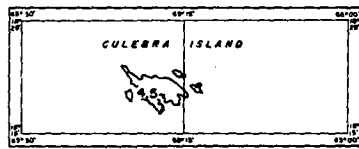
100-YEAR 3-HOUR RAINFALL (INCHES)
