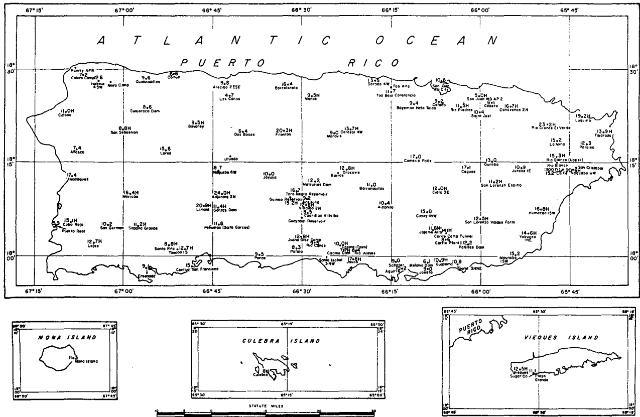
FIGURE 1-1.—Adjusted maximum observed 24-hr. rainfalls (in.) for Puerto Rico. The letter “H” indicates that the rainfall was associated with a hurricane
