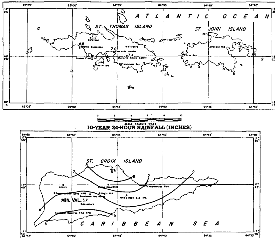
FIGURE 4-101.—10-yr. 24-hr. rainfall for Virgin Islands (in.).
