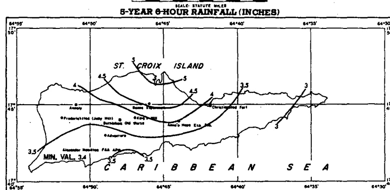
FIGURE 4-86.—5-yr. 6-hr. rainfall for Virgin Islands (in.).
