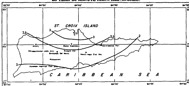
FIGURE 4-60.—25-yr. 30-min. rainfall for Virgin Islands (in.).
