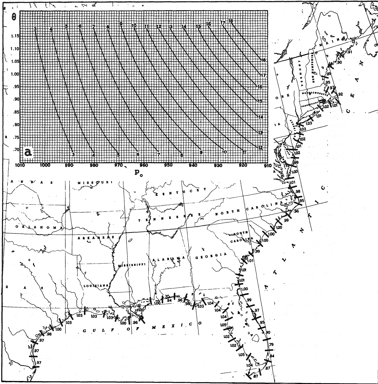
FIGURE 0.2.—A simple hurricane surge prediction model. The slope factor near 1.00, representing the effects of the off-shore depths, is obtained from the map. The expected storm surge is given by the curved lines at the intersection of the slope factor and the central pressure. There is a \frac{2}{3} probability that the actual peak surge will not differ from the expected value by more than 2.1 ft.
