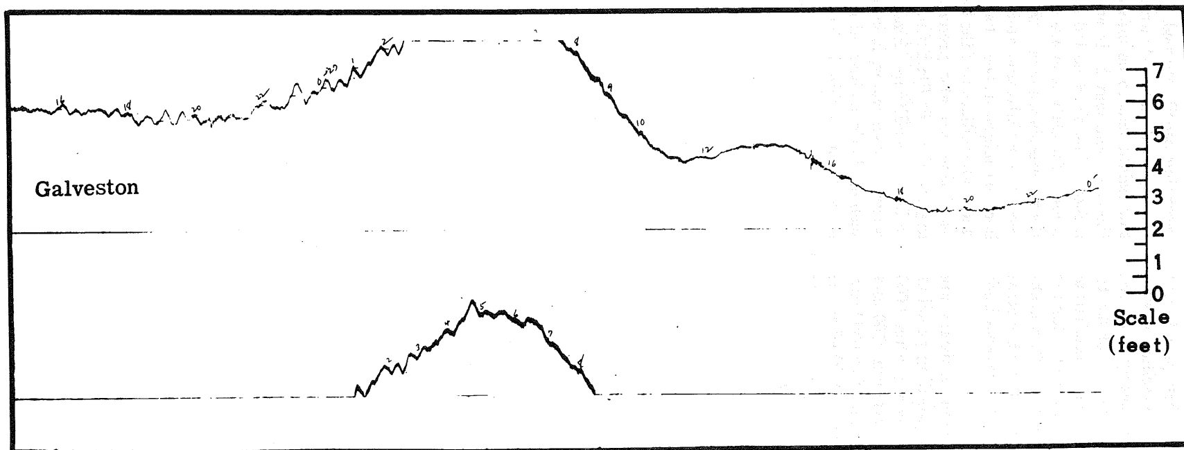
FIGURE 24.6.—Hurricane Audrey 1957, June 26-27. Observed tide records for Galveston, Tex., Coast and Geodetic Survey tide station.
