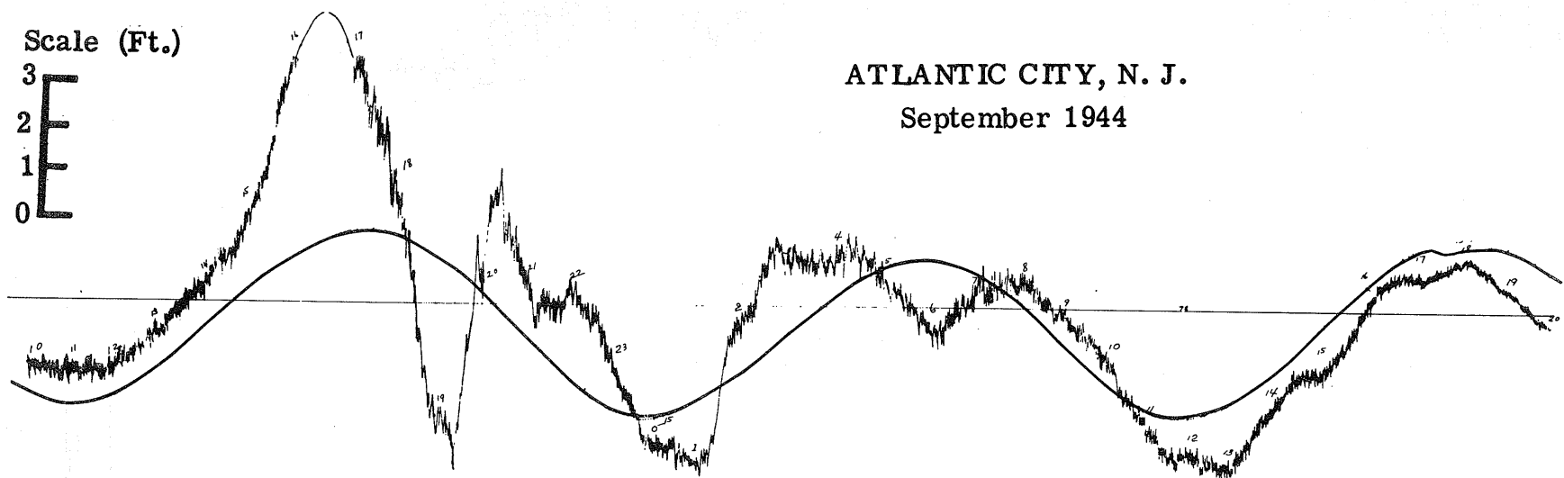
FIGURE 10.4.—Hurricane 1944, September 13–15. Recorded tide traced from original gage record and predicted tide at Coast and Geodetic Survey tide station, Steel Pier, Atlantic City, N.J.
