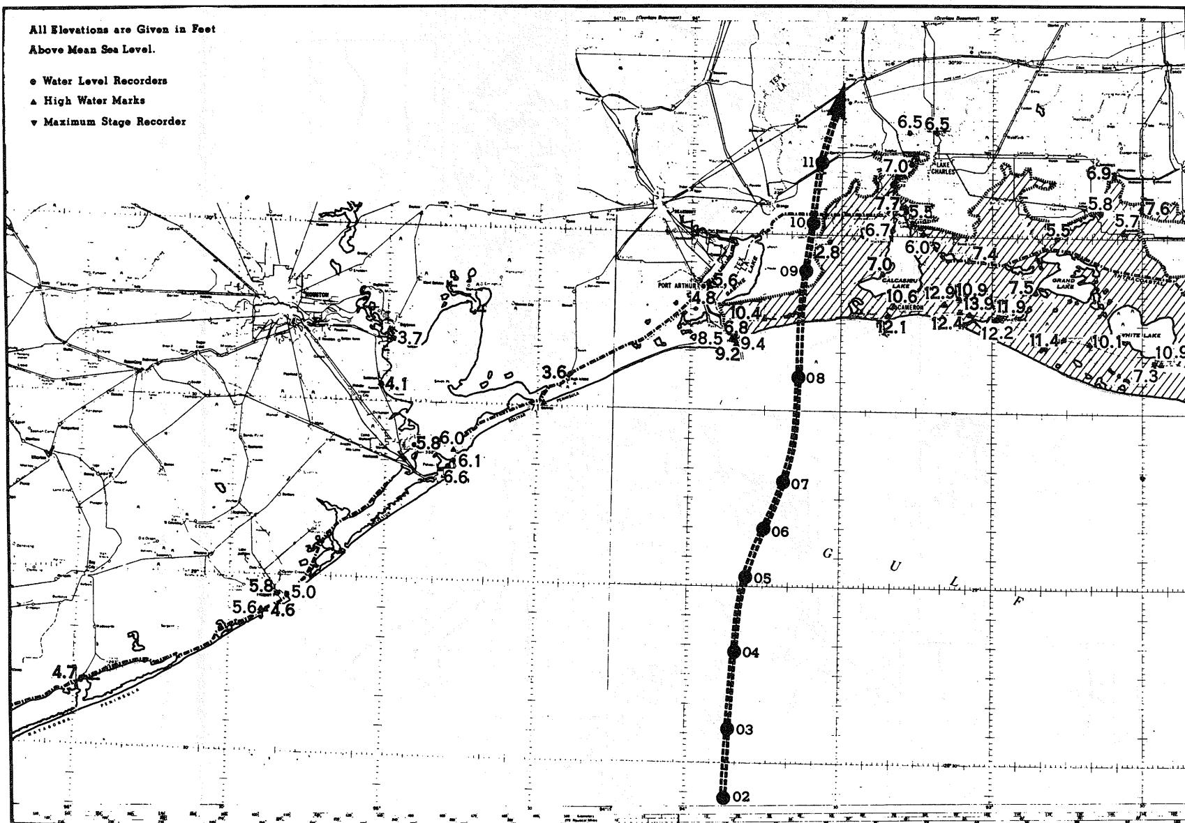
FIGURE 24.4a.—Hurricane Audrey 1957, June 26–27. High water mark chart for Texas and western Louisiana. Hatched area gives limit of inundation in Louisiana.
