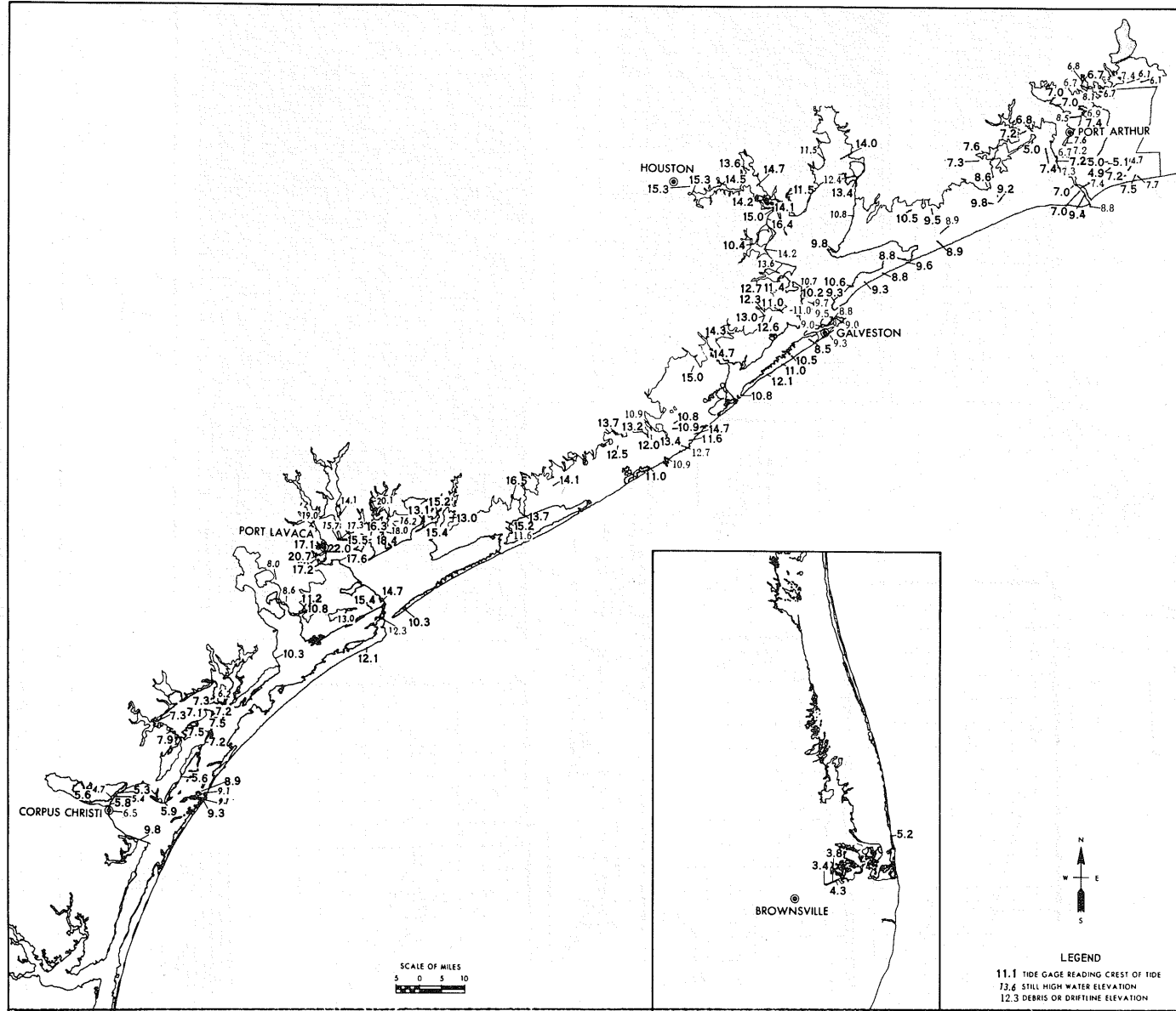
FIGURE 27.3.—Hurricane Carla 1961, September 7-12. High water mark chart for Texas. Shaded area indicates the extent of flooding. (Based on data obtained from the Galveston District of the U.S. Army Corps of Engineers.)
