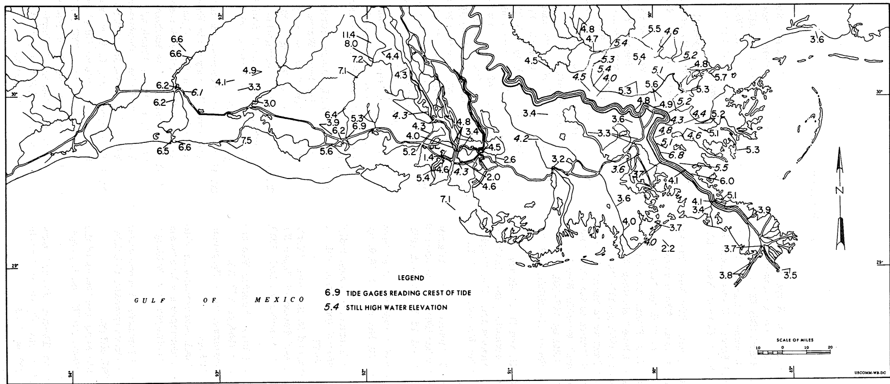
FIGURE 27.4.—Hurricane Carla 1961, September 7–12. High water mark chart for southern Louisiana. (Based on data obtained from the New Orleans District of the U.S. Army Corps of Engineers.)
