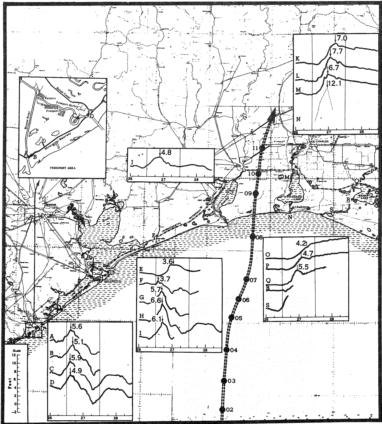
FIGURE 24.3a.—Hurricane Audrey 1957, June 26–27. Observed tides, Texas and western Louisiana. Insert map of Freeport, Tex.
