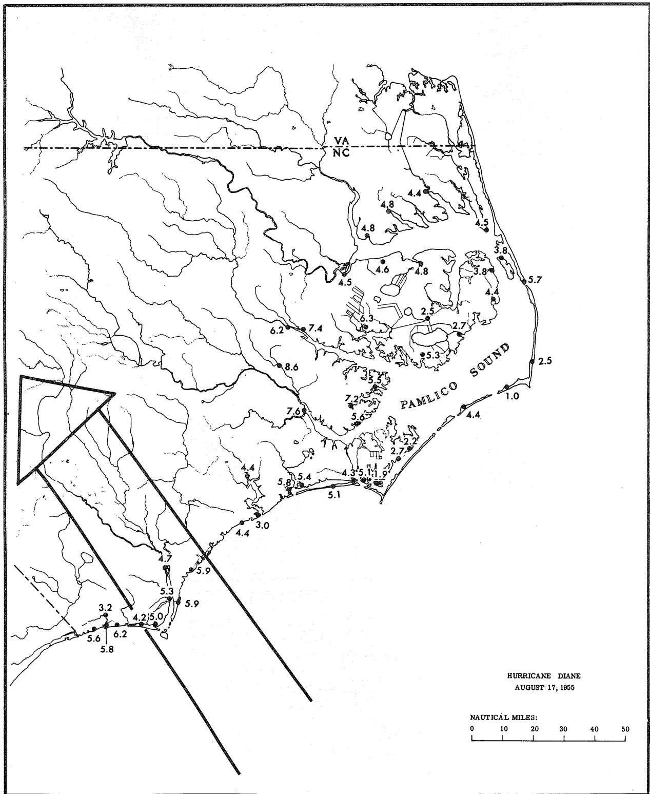
FIGURE 21.2.—Hurricane Diane 1955, August 16-19. High water chart for North Carolina. (Based on data obtained from the Wilmington District of the U.S. Army Corps of Engineers.)
