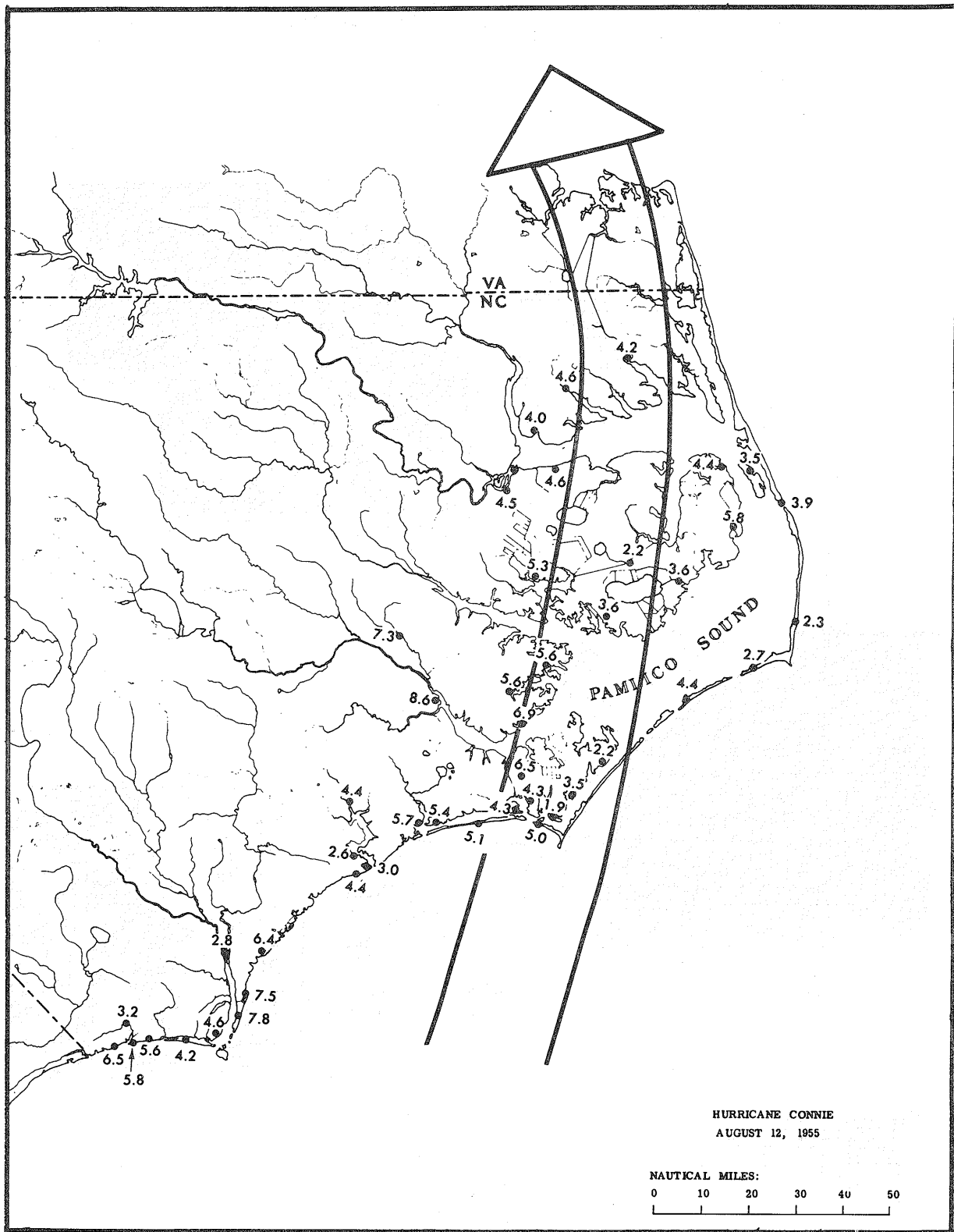
FIGURE 20.3.—Hurricane Connie 1955, August 11–13. High water mark chart for North Carolina. (Based on data obtained from the Wilmington District of the U.S. Army Corps of Engineers.)
