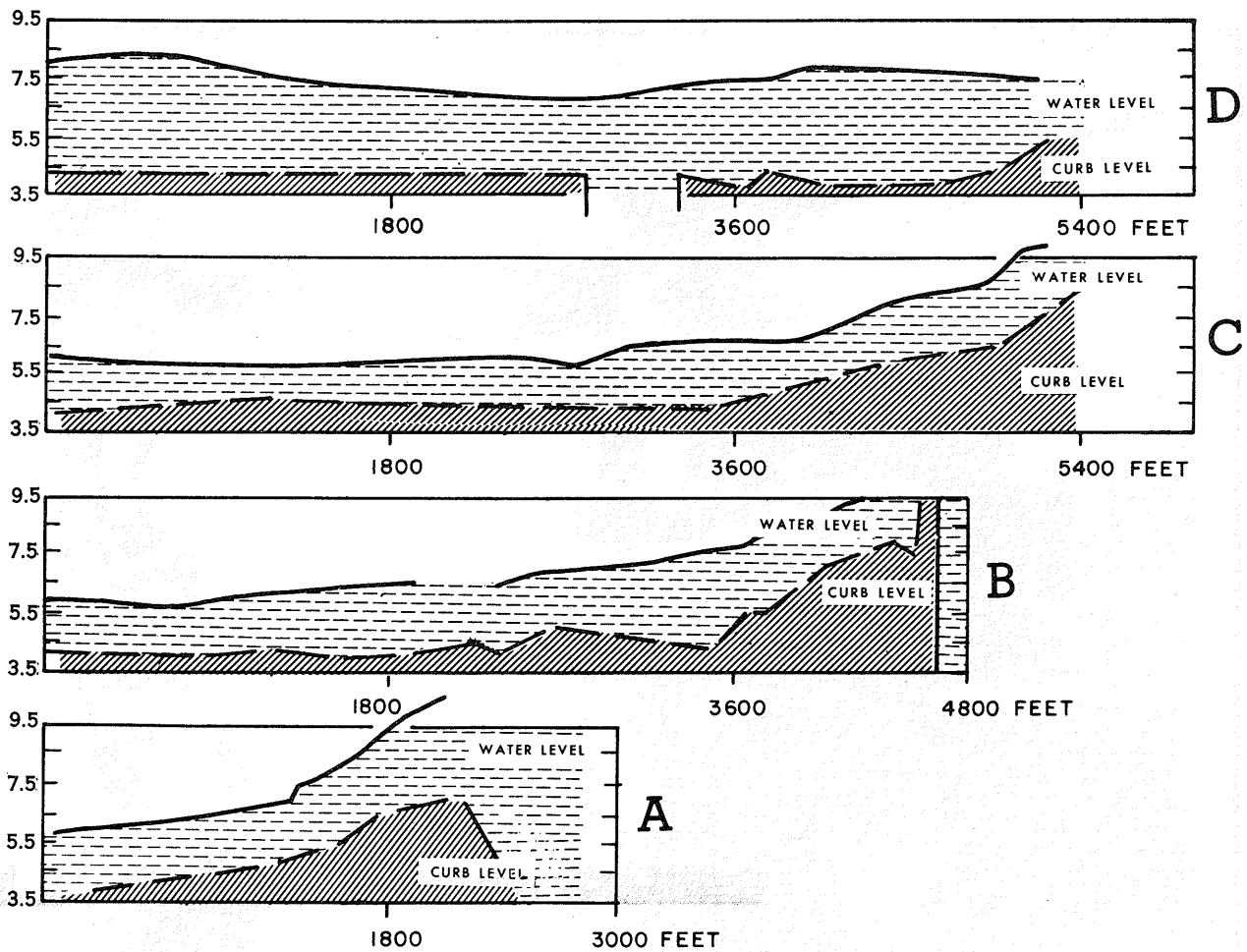
FIGURE 1.5.—Hurricane 1926, September 17-22. High water mark cross sections of Miami Beach at locations A, B, C, D marked on figure 4.
