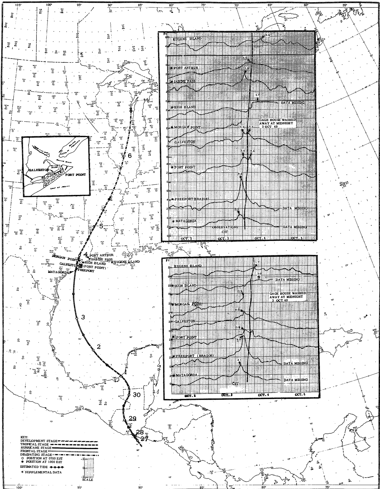
FIGURE 14.2.—Hurricane 1949, October 3-4. Storm surge (upper panel) and tide observations chart (hourly values only). Insert map for Galveston, Tex.
