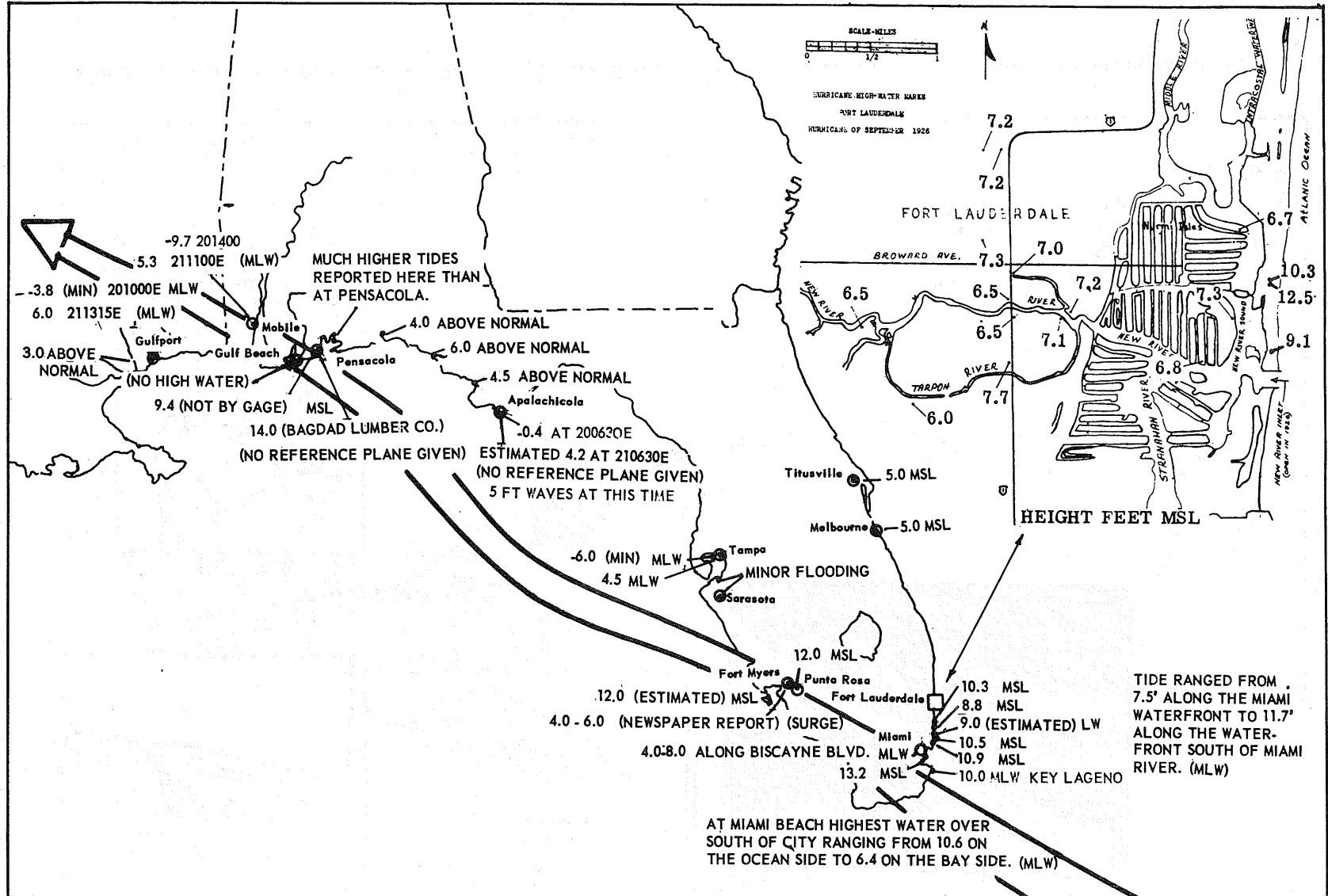
FIGURE 1.3.—Hurricane 1926, September 17–22. Summary of high water marks.
