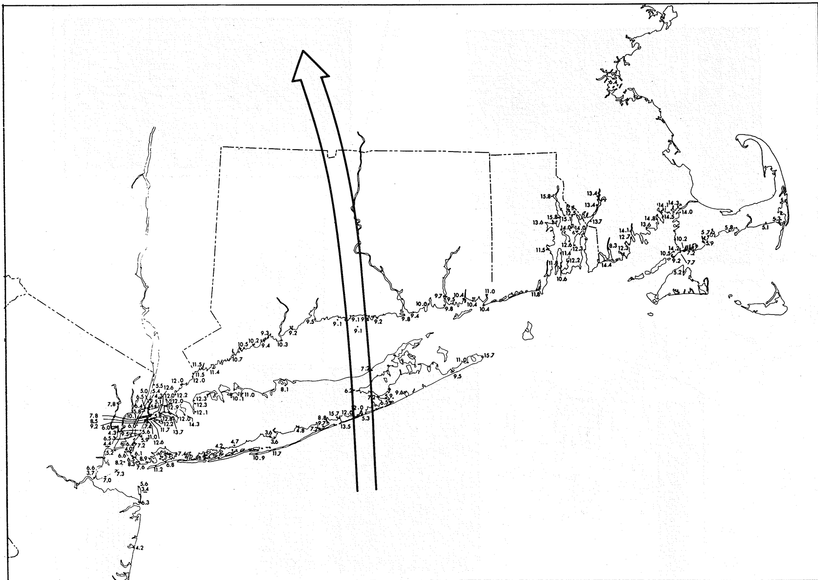
FIGURE 8.3.—Hurricane 1938, September 21–22. High water marks, New York and New England area. (Based on data obtained from New England Division and New York District of the U.S. Army Corps of Engineers and the Woods Hole Oceanographic Institution.)
