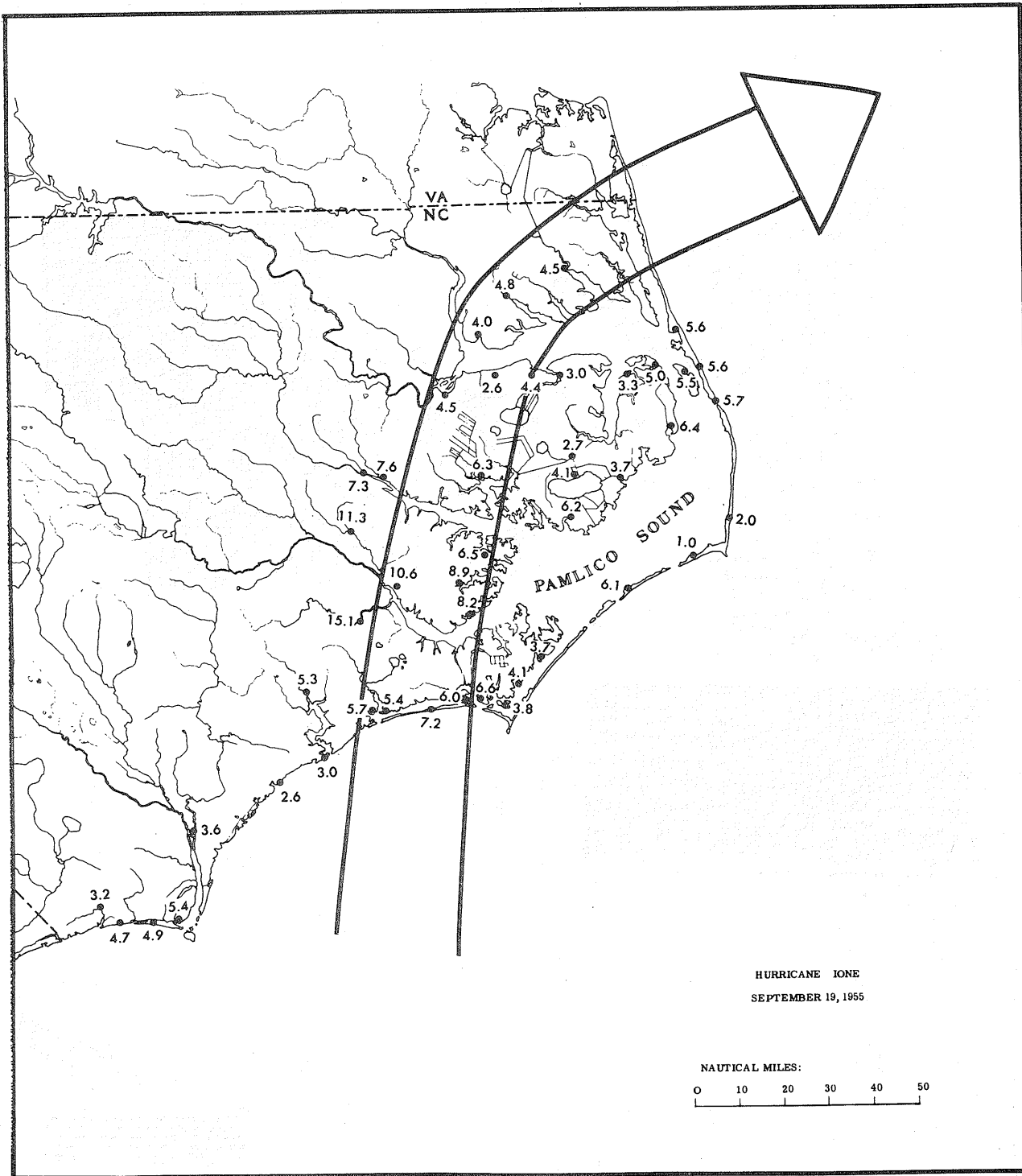
FIGURE 22.3.—Hurricane Ione 1955, September 18–20. High water mark chart of North Carolina. (Based on data obtained from the Wilmington District of the U.S. Army Corps of Engineers.)
