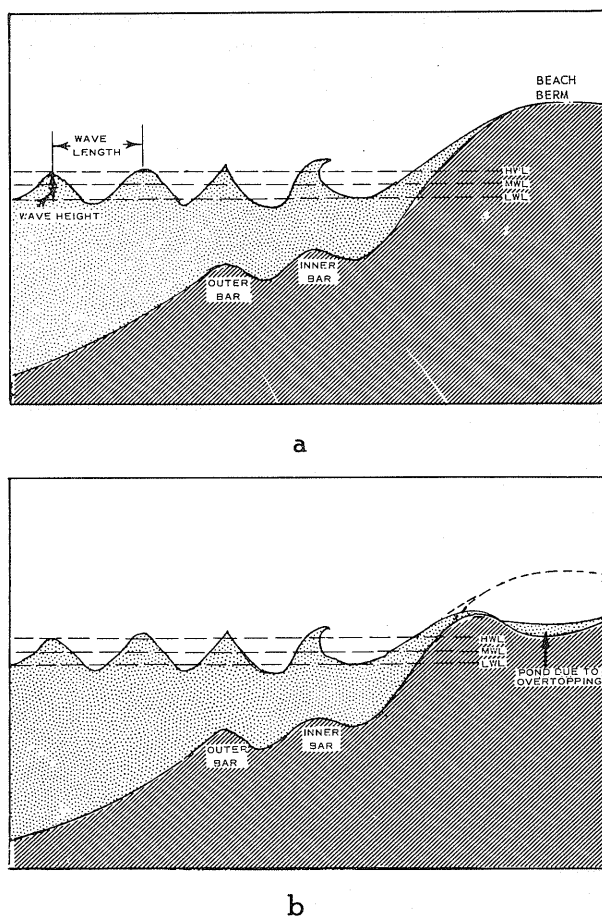
FIGURE 0.1.—Schematic diagram illustrating (a) the effect of wave run-up on a beach and (b) wave overtopping and ponding. The dashed line in (b) shows the profile appearing in (a).
