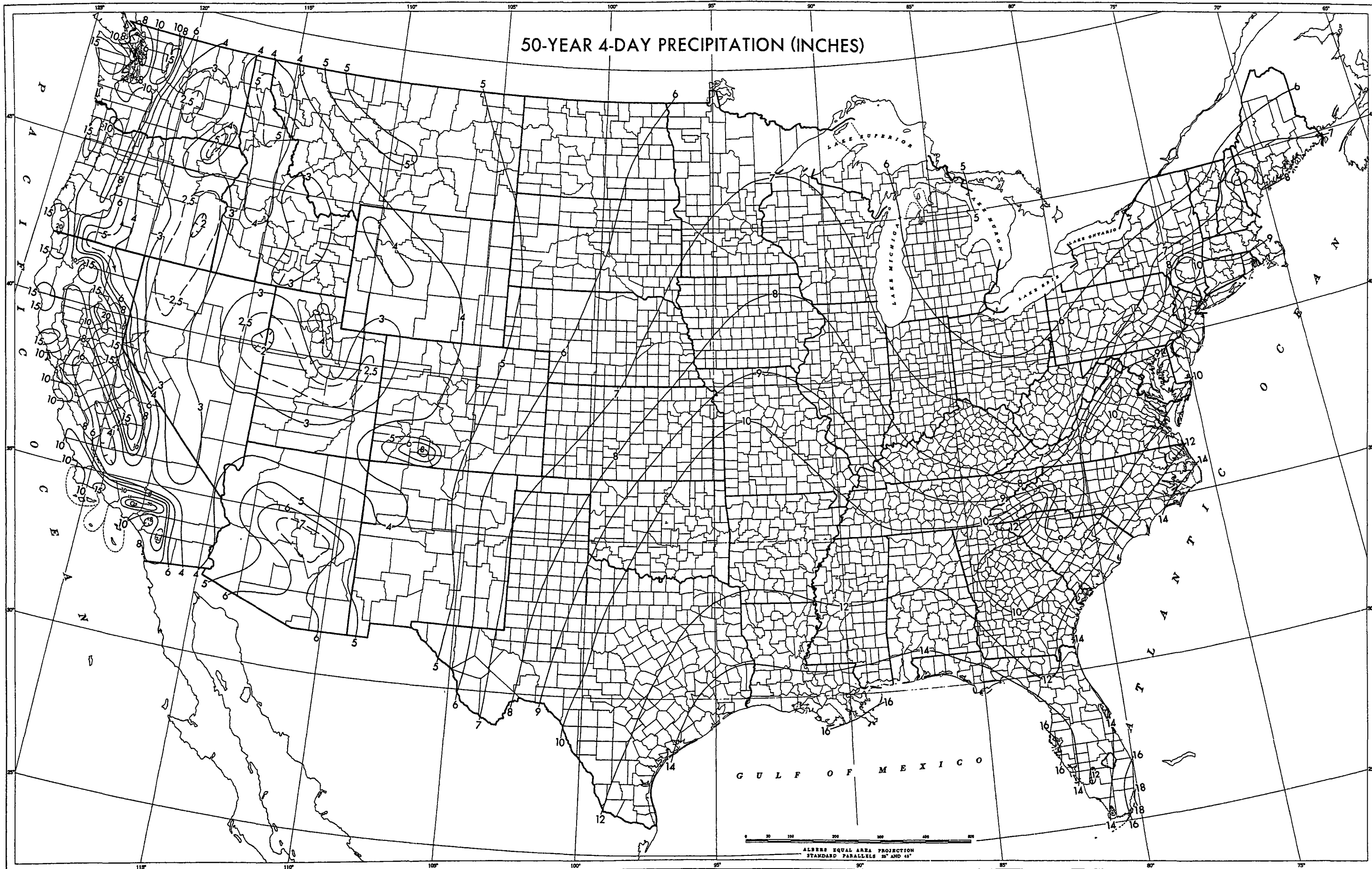
FIGURE 22.—50-year 4-day precipitation (in.).
