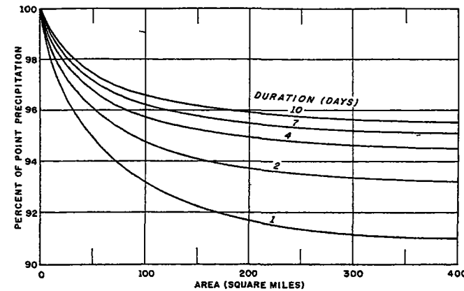
FIGURE 10.—Depth-area curves.
