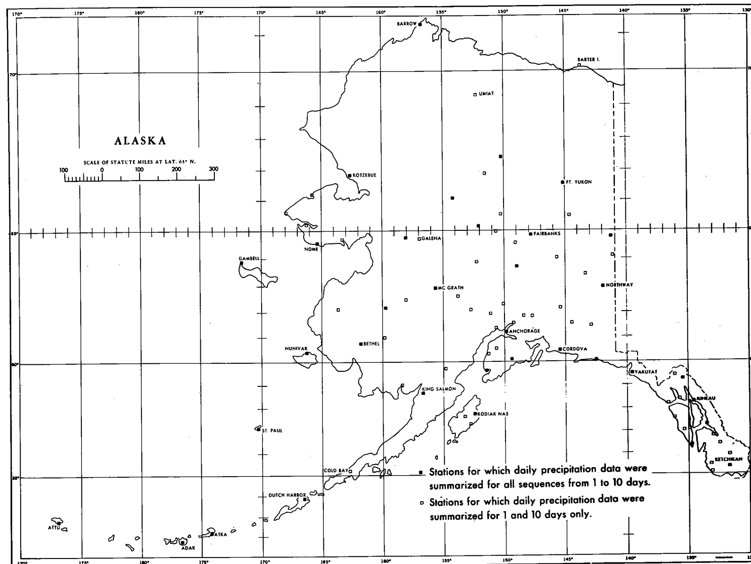
FIGURE 1.—Precipitation stations.
