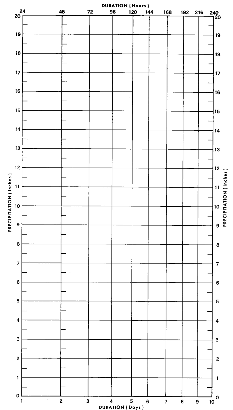
FIGURE 2.—Duration-interpolation diagram.
