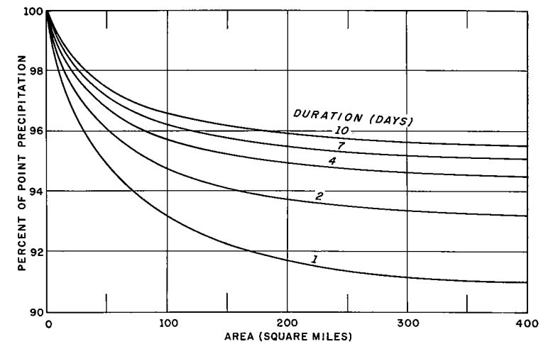
FIGURE 10.—Depth-area curves.
