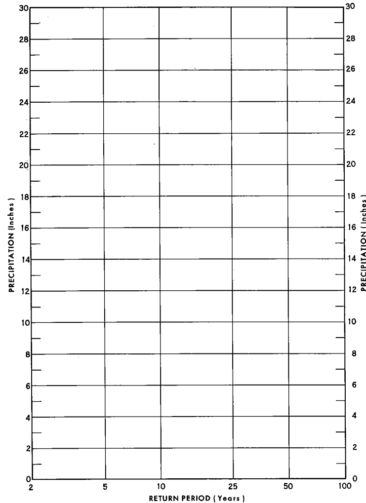
FIGURE 3.—Return-period—interpolation diagram.
