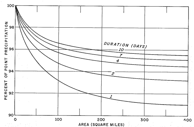
FIGURE 10.—Depth-area curves.
