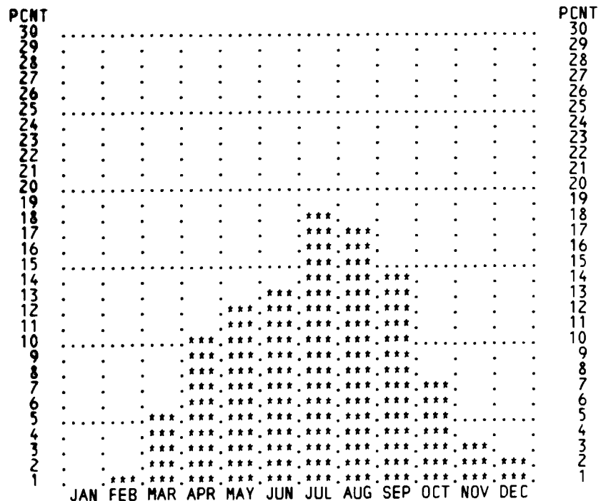
FIGURE III- 8 MONTHLY DISTRIBUTION (BY PERCENT) OF 2-HR STORMS - CLASS III
