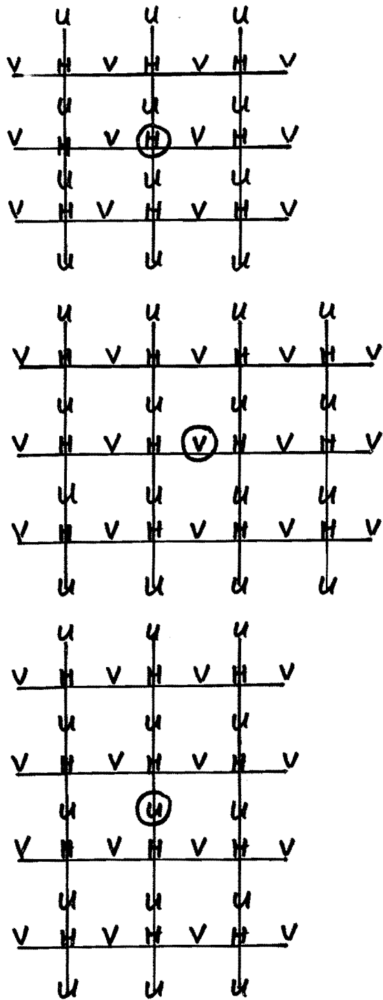
Figure H.1.--Neighboring data points needed to make one complete Lax-Wendroff time step for the central variable enclosed in a circle. The symbols H, U, V represent the full time step variables (H, H \theta , H q ), H u , and H v .
