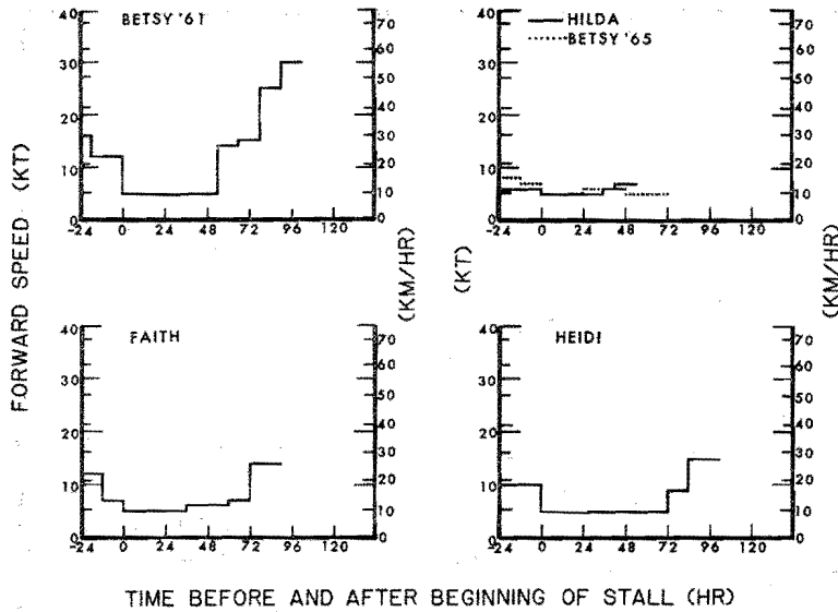
Figure 16.8a.--Variation of forward speed (T) with time for selected stalling hurricanes. Time = 0 indicates the beginning of stall (T < 5 kt, 9 km/hr)
