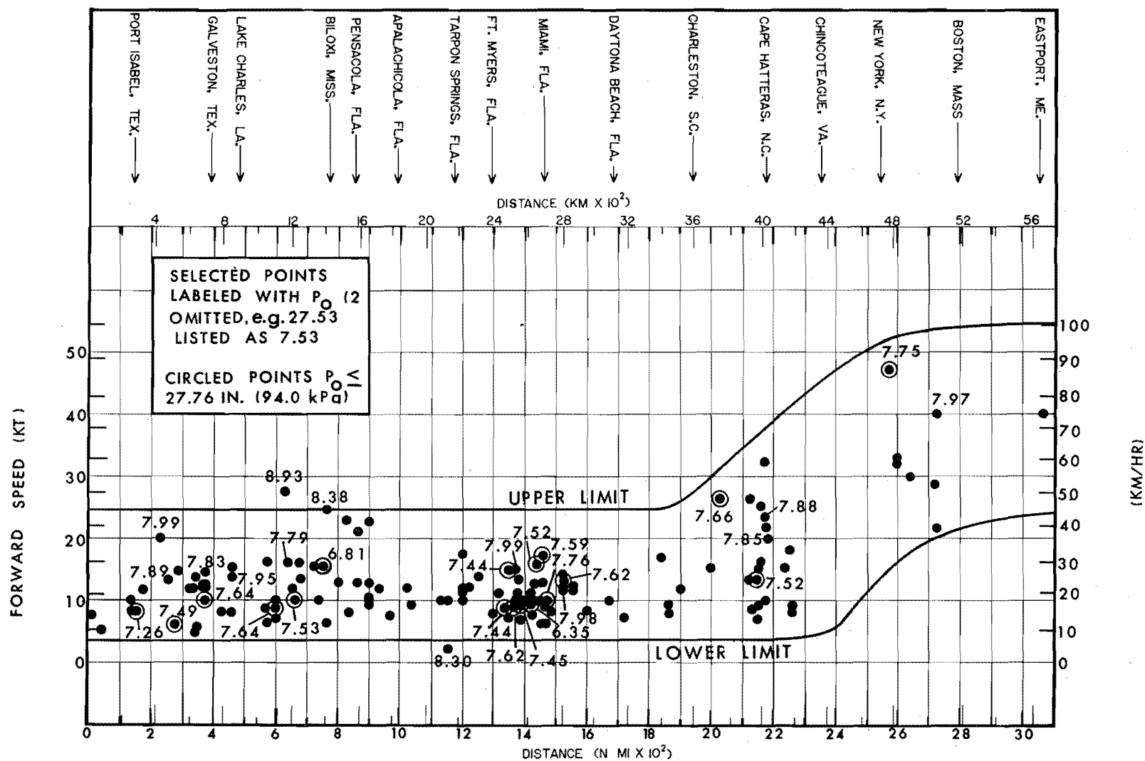
Figure 10.3.--Adopted SPH upper and lower limits of T . Data is from tables 4.1 to 4.4. All data points falling outside the two curves are labeled with lowest central pressure ( p_0 ). All circled data points falling inside the two curves are labeled with lowest p_0 . Other data points (except those between mileposts 1300 and 1500) are labeled with lowest p_0 if this p_0 is \leq 28.00 in. (94.8 kPa).
