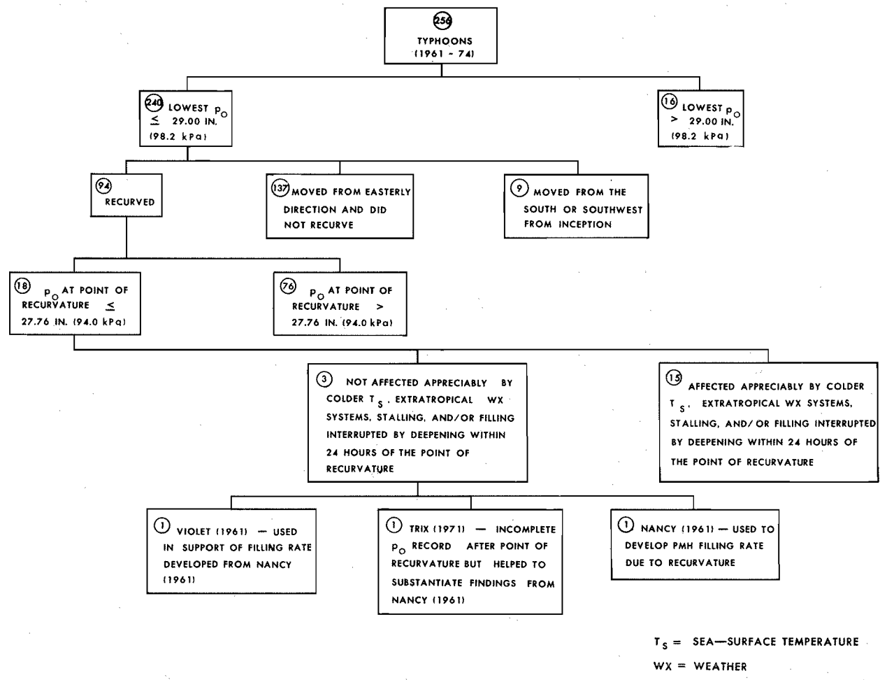
Figure 8.9.--Schematic summary of typhoons used for guidance on filling rate of PMH after recurvature over the northeast gulf coast.
