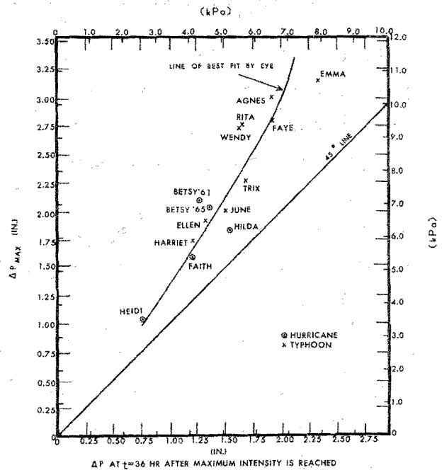
Figure 16.5b.--Same as figure 16.5a except abscissa refers to time 36 hours later.
