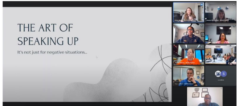
NWS Nashville Meteorologist in Charge, Krissy Hurley, delivering the keynote address on “Speaking Up When Something is Wrong” at the 2022 Southern Region Women’s Conference
