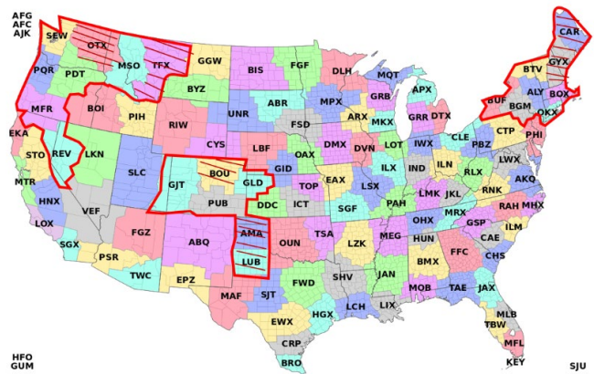
Map depicting the three exercise pods, with Hazard Services sites denoted by hatching
