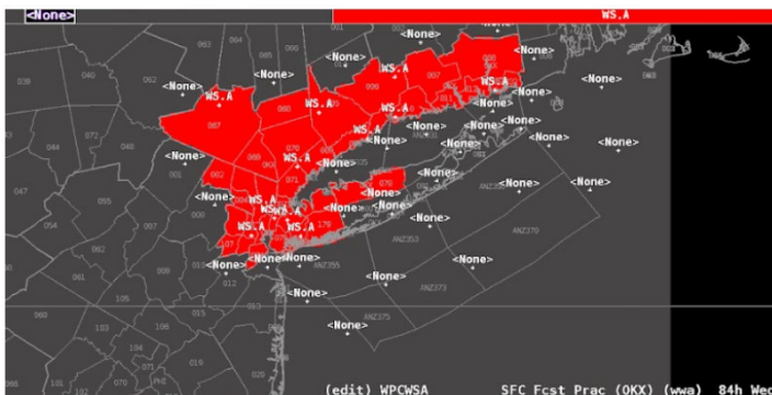
A test proposed Watch within WFO OKX's forecast area
