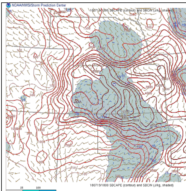
Figure A5 - Surface-based CAPE (J/kg) shown in red contours and Convective Inhibition (J/kg) shown in shading and dashed blue contours at 100 PM. Image from SPC.
