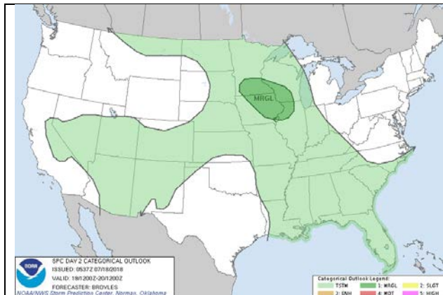
Figure 6a – Day 2 SPC Outlook issued 1237 am July 18, 2018
