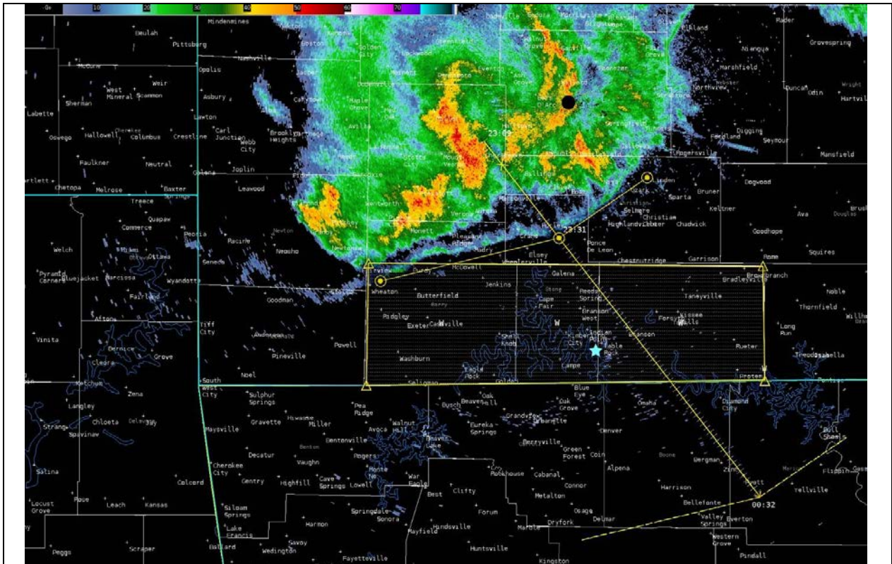
Figure 20: Example 2 of Warngen mock-up using 3 vertices for SVR #243.
