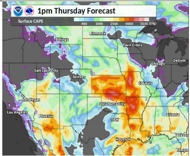
Figure 4: 6-hr forecast of NAM surface-based CAPE valid at 100 pm on July 19, 2018.
