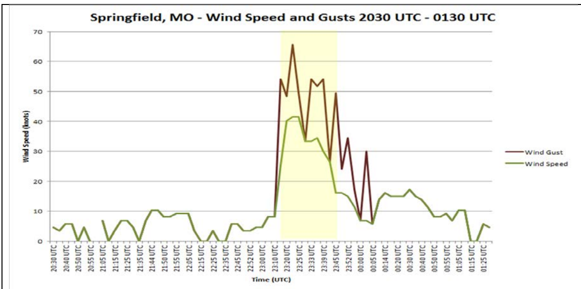
Figure A17 - Wind speed sustained (green line) and gusts (maroon line) in knots at the Springfield, MO ASOS between 2030 UTC (330 PM) and 0125 UTC (825 PM). Yellow shading highlights 30-minute period which had regular gusts of 49 knots or greater.
