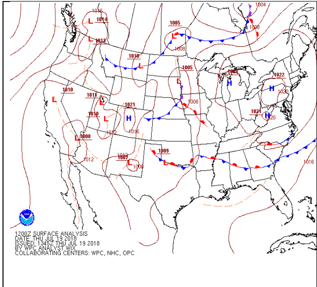
Figure 3 - Surface map valid at 700 am, July 19, 2018.
