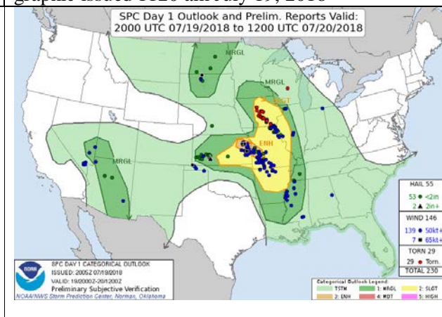
Figure 7d – SPC Day 1 outlook issued 3 pm July 19, 2018 with preliminary verification reports.
