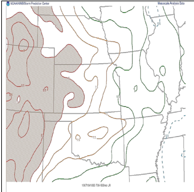
Figure A3 - 700-500 mb Lapse Rates at (C/km) at 100 PM. Image from SPC.
