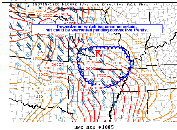
Figure 7c – SPC MCD #1085 issued 216 pm July 19, 2018
