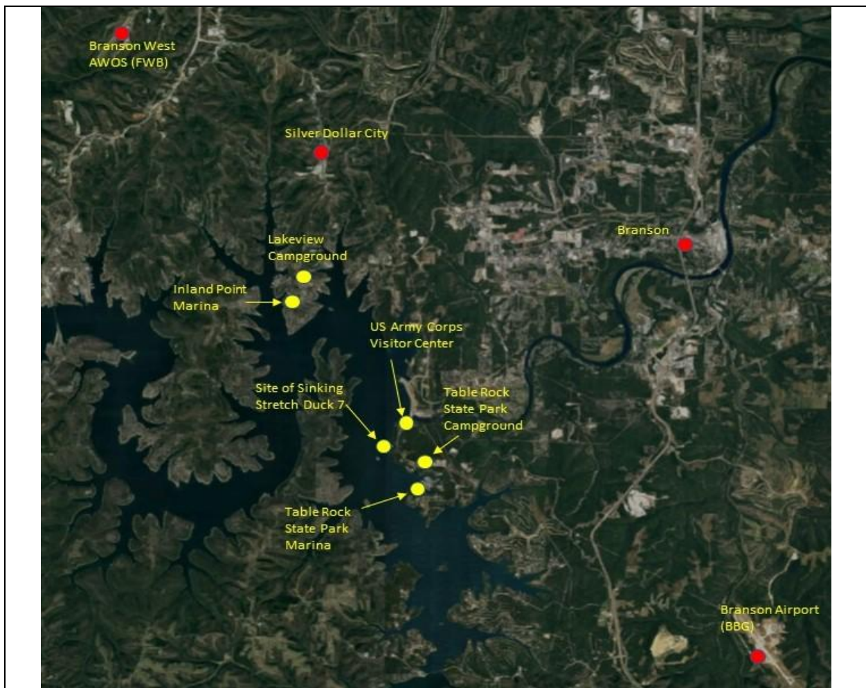
Figure 18: Map of pertinent locations around Table Rock Lake. Not shown – Stockton SP, MO State Highway Patrol Marine and Communication Units.
