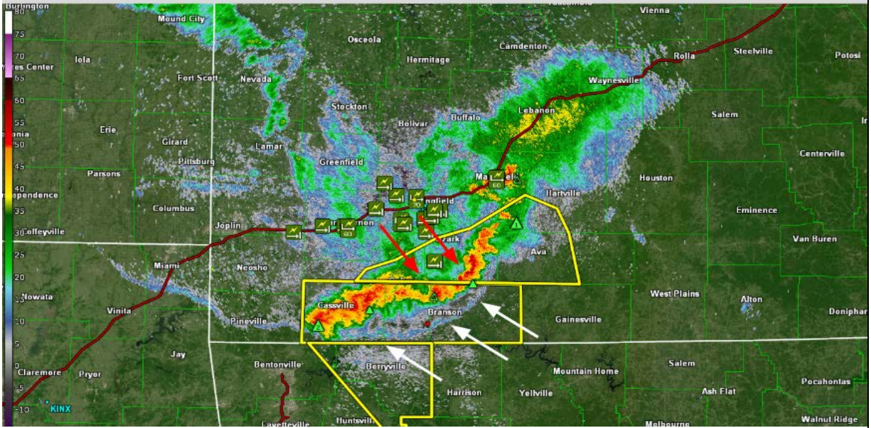
Figure A16 - 0.5 degree reflectivity image from Springfield WSR-88D at 701 PM. Red arrows indicate rear inflow notches and white arrows show the leading edge of the outflow. Yellow polygons are NWS Severe Thunderstorm Warnings. Small red square in the lower center part of the image marks the location of the Table Rock Lake State Park Marina.
