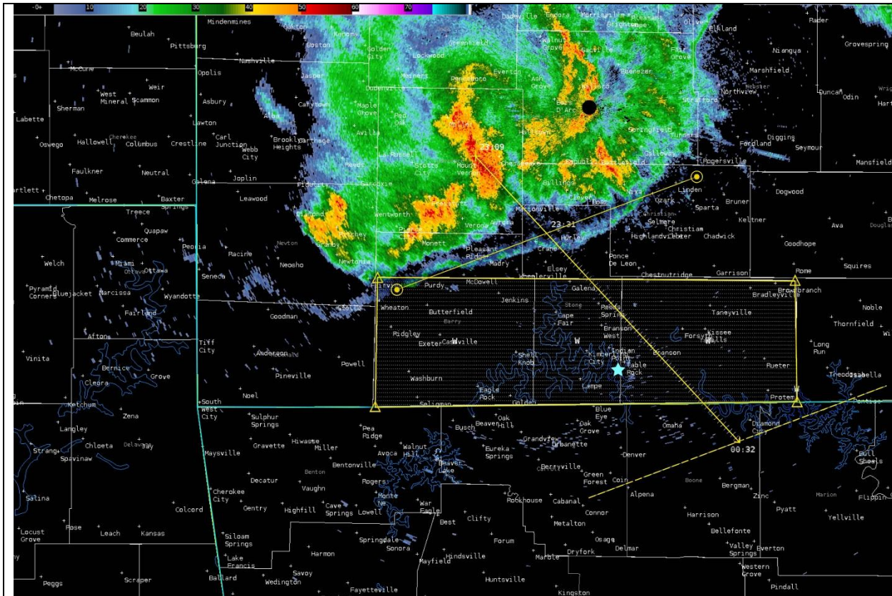
Figure 19: Example 1 of Warngen mock-up using exact vertices and storm motion used in real-time for SVR #243
