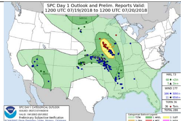
Figure 6b – SPC Day 1 outlook issued 1237 am July 19, 2018 with preliminary verification reports.
