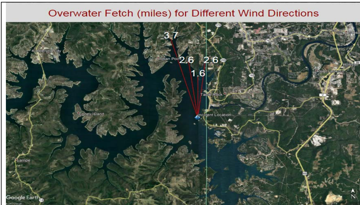
Figure A19 - Image of Table Rock Lake showing different fetch lengths (miles) for different wind directions from the north arm of the lake down to near the Table Rock Lake State Park marina.
