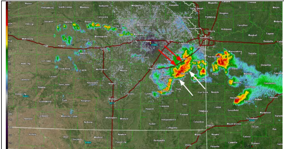
Figure A7 - 0.5 degree reflectivity image from Topeka WSR-88D at 405 PM. Red arrows indicate rear inflow notches and white arrows show the leading edge of the outflow and tight low-level reflectivity gradient. Small red square in the lower right marks the location of the Table Rock Lake State Park Marina.
