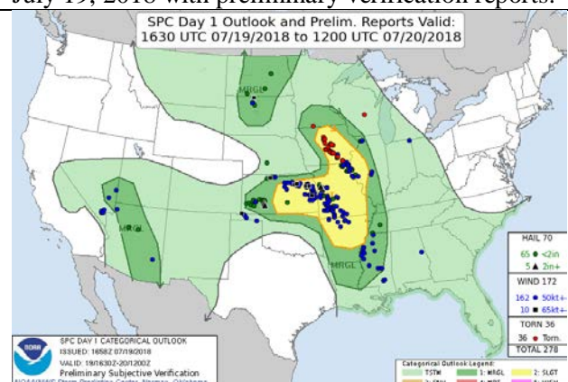
Figure 6d – SPC Day 1 outlook issued 1159 am July 19, 2018 with preliminary verification reports.
