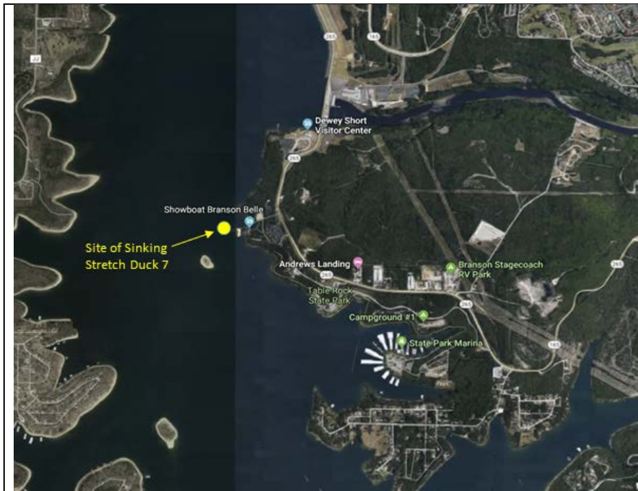
Figure 1: Map of region around Table Rock State Park, Table Rock Marina, Branson Belle Showboat Dock, and location of Stretch Duck 7 sinking.
