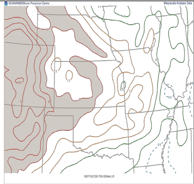
Figure A4 - 700-500 mb Lapse Rates at (C/km) at 500 PM. Image from SPC.
