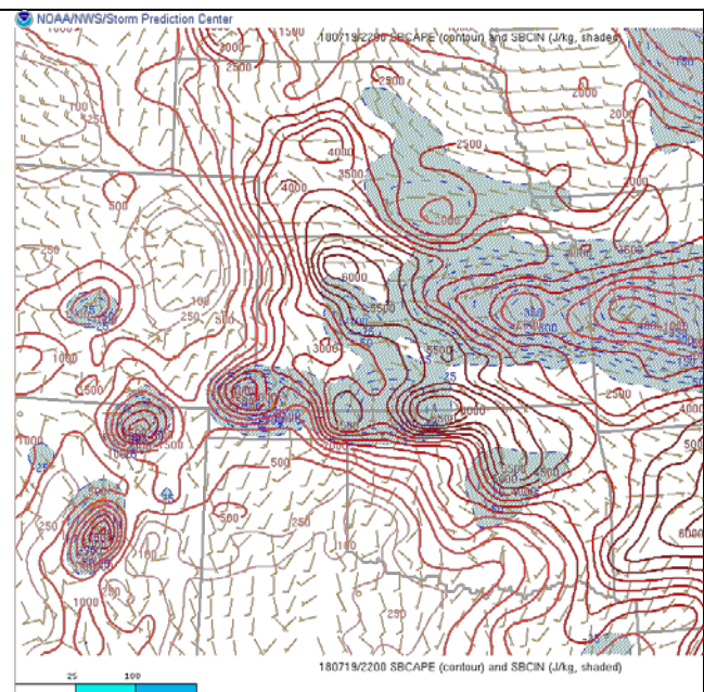
Figure A6 - Surface-based CAPE (J/kg) shown in red contours and Convective Inhibition (J/kg) shown in shading and dashed blue contours at 500 PM. Image from SPC.
