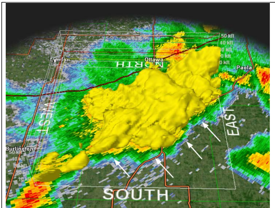
Figure A8 - Volumetric reflectivity image from Topeka WSR-88D at 405 PM. Image highlights 40 dBZ surface. White arrows show the leading edge of the outflow.
