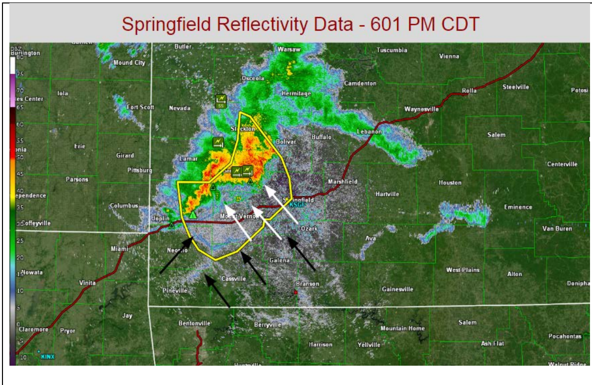
Figure A11 - 0.5 degree reflectivity image from Springfield WSR-88D at 601 PM. White arrows show the leading edge of the outflow associated with the derecho and black arrows identify location of remnant outflow from earlier convection. Yellow polygon is a NWS Severe Thunderstorm Warning. Small red square in the lower center part of the image marks the location of the Table Rock Lake State Park Marina.
