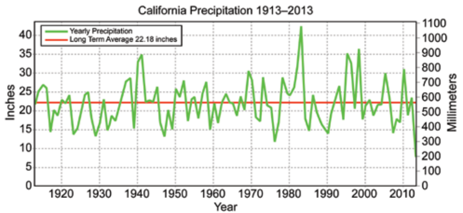
Total average calendar year precipitation for California from 1913 through 2013 (green line) and long term average (red line).
