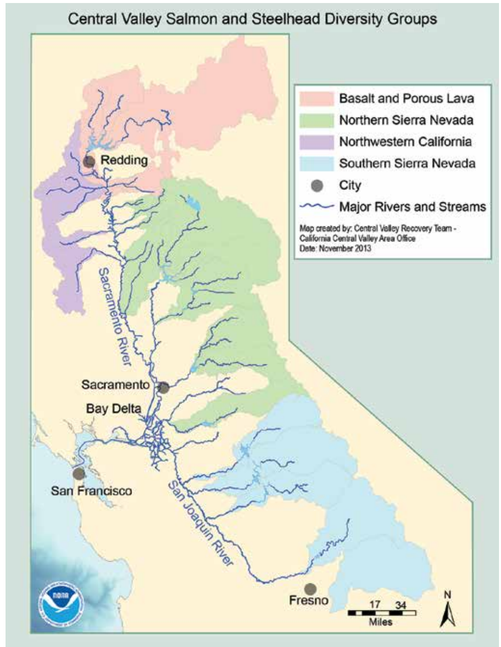
Location of key salmon watersheds in the Central Valley of California.
