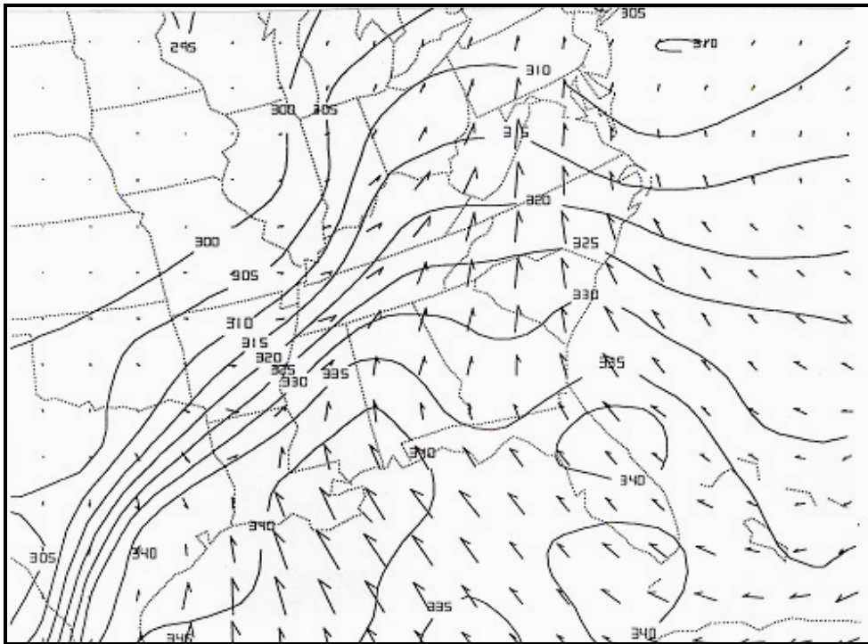
Fig. 6. NGM initial field of equivalent potential temperature ( \theta\text{-e} ) and moisture transport vectors on the 295 K isentropic surface, valid 1200 UTC (7 a.m. EST), March 27, 1994. \theta\text{-e} contoured every 5 K.
