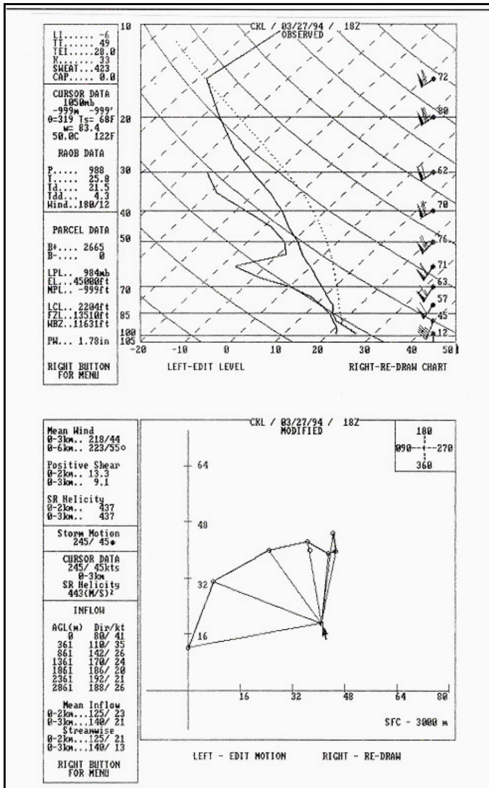
Fig. 10. Special upper-air sounding for Centreville, Alabama (CKL), valid 1800 UTC (1 p.m. EST), March 27, 1994. The Skew-T (top) depicts a CAPE value of 2665 J kg -1 . The hodograph (bottom) indicates 0-3 km SRH of 443 m 2 s 2 , based on an observed storm motion of 245/45.
