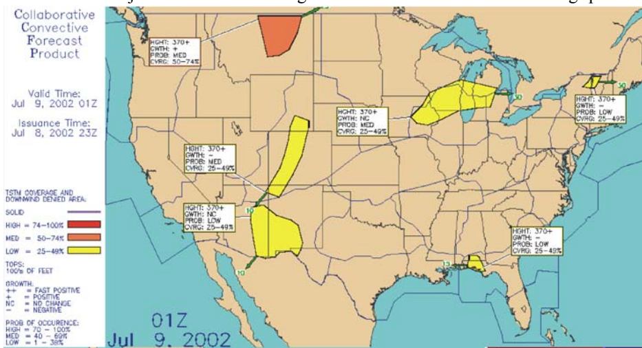
Figure 2. The CCFP forecast graphic for thunderstorms displays areas in which severe weather may impact the efficient and safe flow of air traffic. The forecasts are issued by the Aviation Weather Center and are the result of consultation between meteorologists in the Center Weather Service Units and major airlines.
