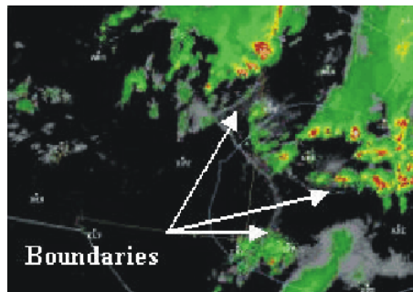
Figure 4 Boundaries produce by cold air outflow from thunderstorms.
