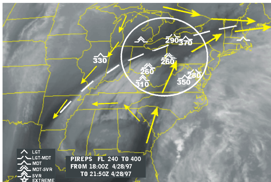
Figure 2. GOES WV image of a deformation zone (white dashed line) associated with a large scale low pressure system on 28 April 1997. Jet streams are shown by large arrows. Smaller arrows indicate direction of weaker flow. Circle indicates the likely region of strongest CAT. Note the pronounced dark zone shown along the deformation zone and jet stream.
