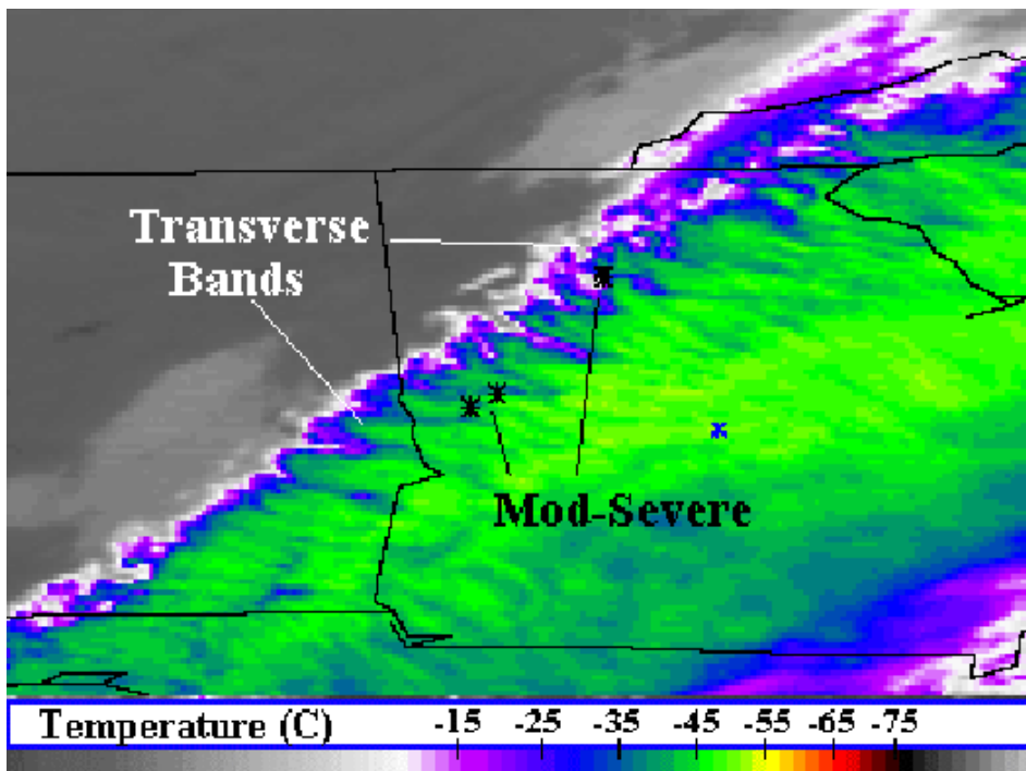
Figure 1. GOES IR image showing well-defined transverse cirrus bands along a strong jet stream and frontal cloud system on 24 November 1995. Turbulence reports were from large jet aircraft between FL200 - FL300.
