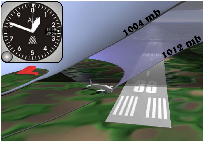
Figure 8a The 1012 mb (29.88 in Hg) pressure surface is at Wittman Field in Oshkosh, WI. For landing, the altimeter setting provided was 29.88 in. Hg. and the altimeter reads the field elevation of 808 ft. MSL. The pilot and friends leave the altimeter set at 29.88 and take in the fabulous AirVenture.
