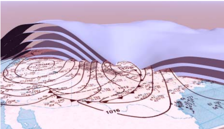
Figure 6. Pressure “surfaces” intersect the weather map at the respective isobars. If you take off where the air pressure is 1008 mb (29.77 inches) your altimeter will give altitude relative to that pressure surface. As the pressure surface changes altitude, your actual height above ground will change even though your altimeter is rock steady.
