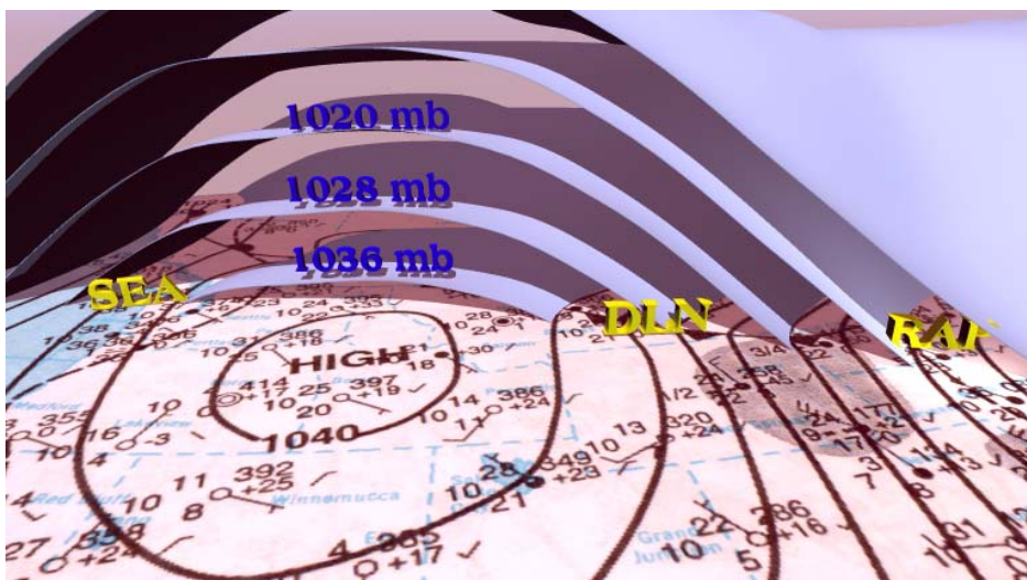
Figure 7. On a flight from Seattle, WA (SEA) to Rapid City, SD (RAP) the altimeter is set to local conditions prior to take off, and it follows the 1036 mb pressure surface. If not reset to local altimeter settings en route, the altimeter would lead you into lower altitudes or even into the terrain without warning. By resetting the altimeter regularly, you ensure that you are following the correct pressure surface.
