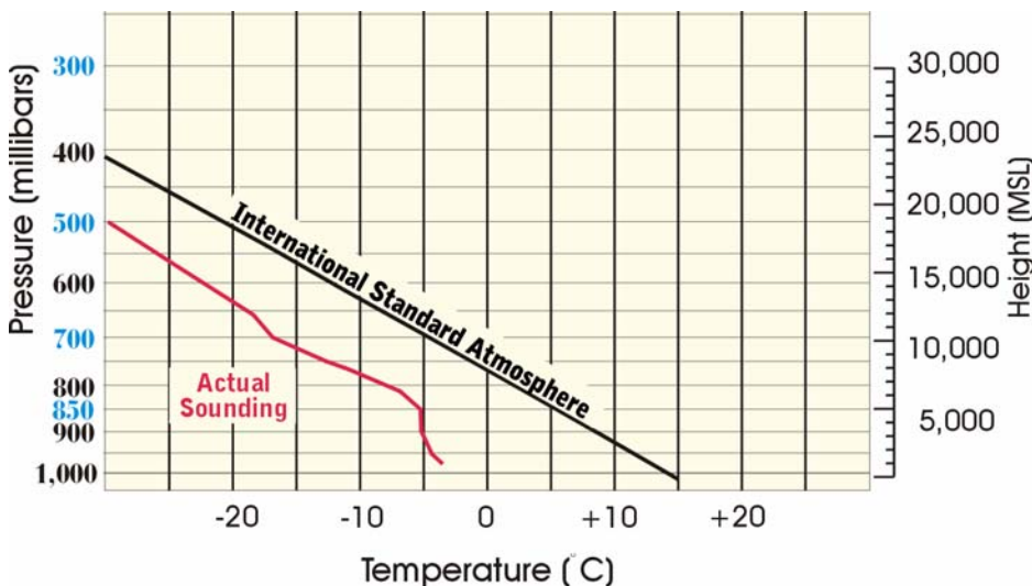
Figure 5. The International Standard Atmosphere (ISA) is an average, uniform distribution of pressure, temperature, and density. Actual conditions on any given day as measured by balloon soundings are often different. When differences are large, altimeter errors increase because pressure surfaces move to different levels vertically.
