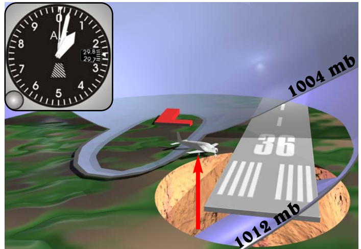
Figure 8b During the day, the low pressure center arrives with the 1004 mb (29.65 in Hg) pressure surface. At the end of a long day and without changing the setting in the Kollsman window, the altimeter now reads 230 ft MSL higher . The pressure has fallen 8 mb (0.23 in Hg). The altimeter reads 230 feet higher because the 1012 mb pressure surface is “below” the field.
