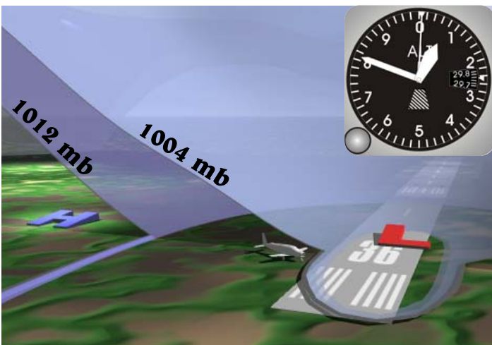
Figure 9a A high pressure ridge is approaching. The current altimeter setting, 1004 mb (29.65 in Hg) is the pressure surface at the ASOS site. The indicated altitude is 808 ft. MSL, and the Kollsman window is set at 29.65.
