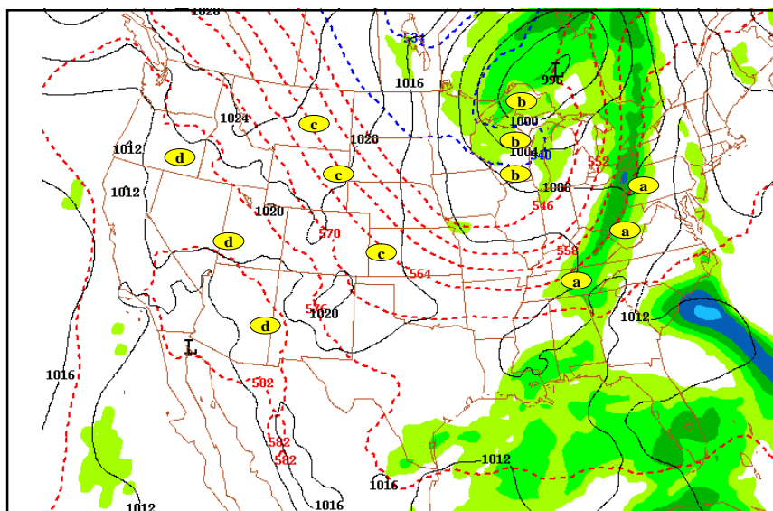
Figure 3: NWS Surface chart: Solid black lines are isobars or lines of equal pressure are the contour lines that help place frontal boundaries (western Pennsylvania). The dash lines are lines of thickness which help delineate different airmasses (western Pennsylvania and southwest through Kentucky). The blue line to the north (Wisconsin) is the 540 line and is used widely to delineate rain versus snow. The shaded green is depicting areas of precipitation.
