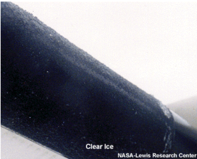
Figure 3: Clear ice
