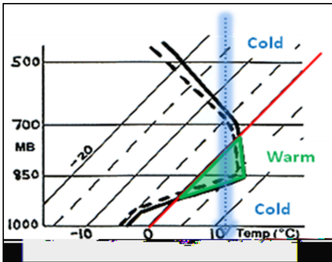
Figure 6: Freezing rain
