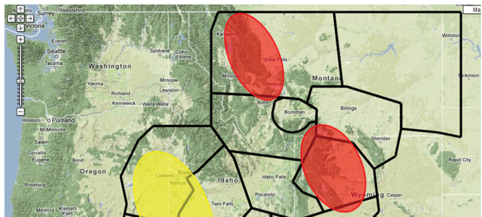
Map highlighting ZLC Airspace. Primary mountain wave activity areas are shaded in red, with a secondary region in yellow.
