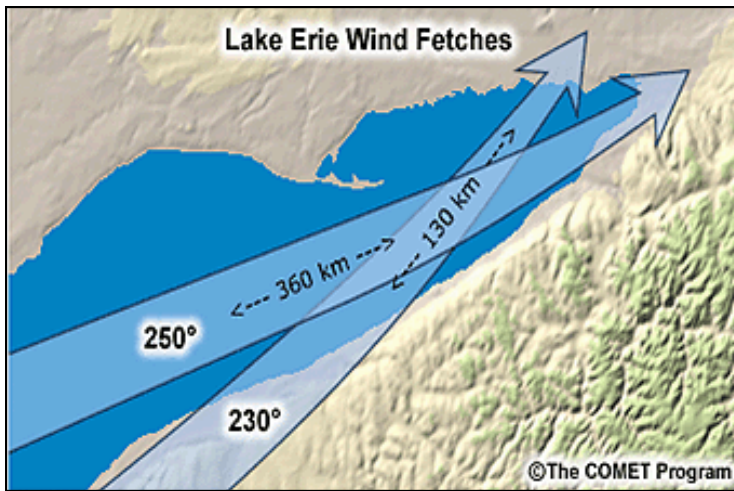
Figure 6: Lake Erie wind fetches
