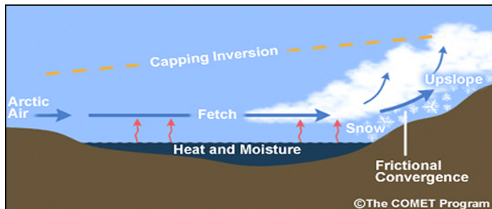
Figure 5: Quick look at lake effect weather
