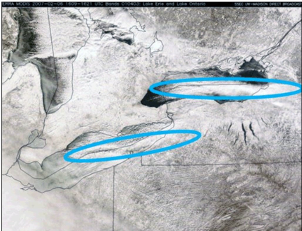
Figure 10: West winds producing intense single band of lake effect snow over Upstate New York
