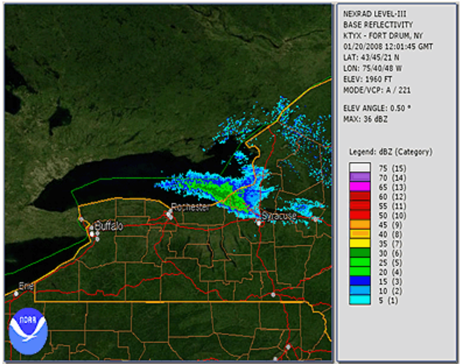
Figure 14: Single band of lake-effect snow in Upstate New York.
