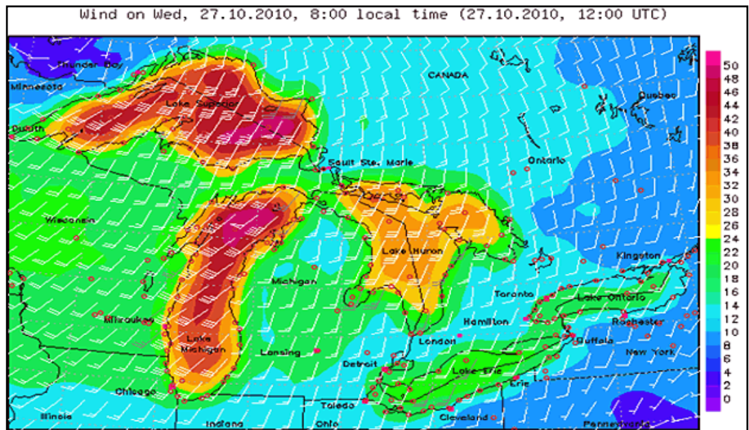
Figure 25: Example of how reduced friction over the lakes and an unstable atmosphere can combine to produce much stronger winds over the Great Lakes.
