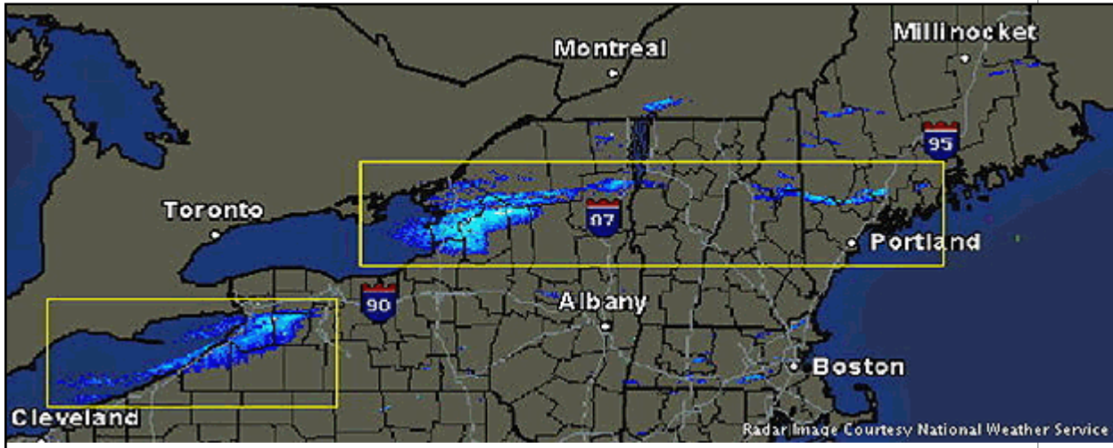
Figure 11: Two, intense (2"-4" per hour) single lake-effect snow bands
