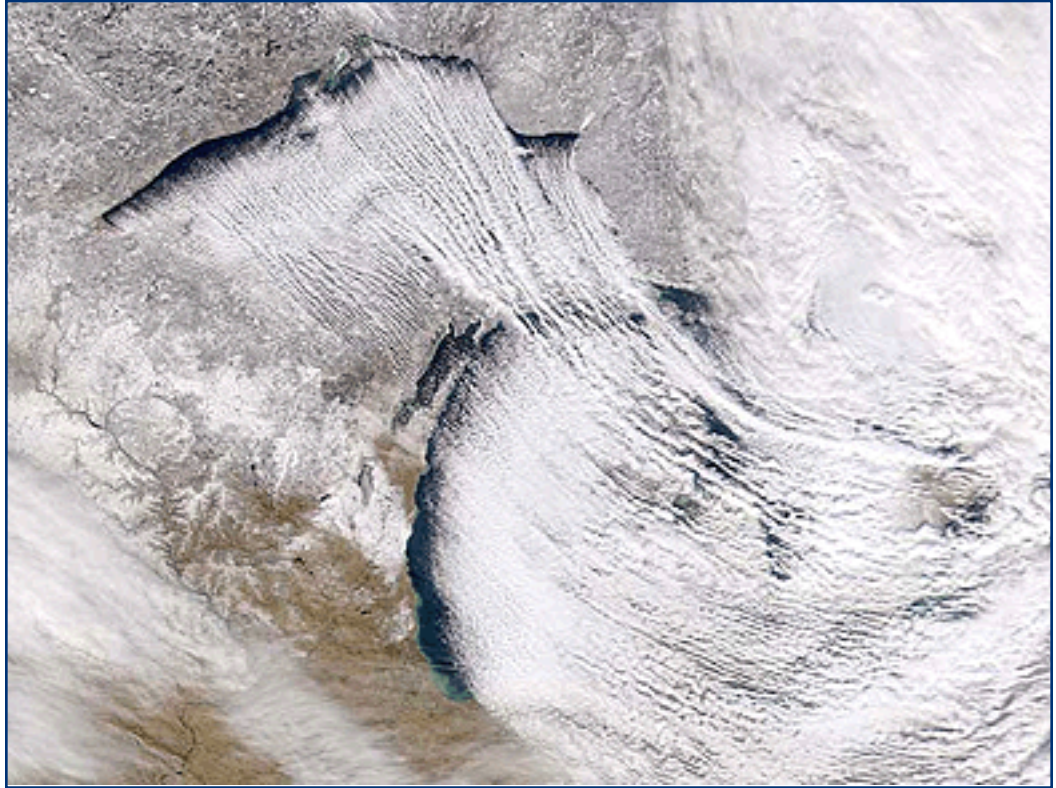
Figure 9: Northwest winds producing multiple bands of lake effect in Michigan and Wisconsin
