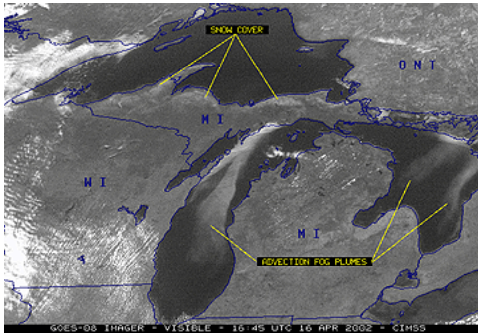
Figure 21: Satellite picture showing advection fog over lakes
