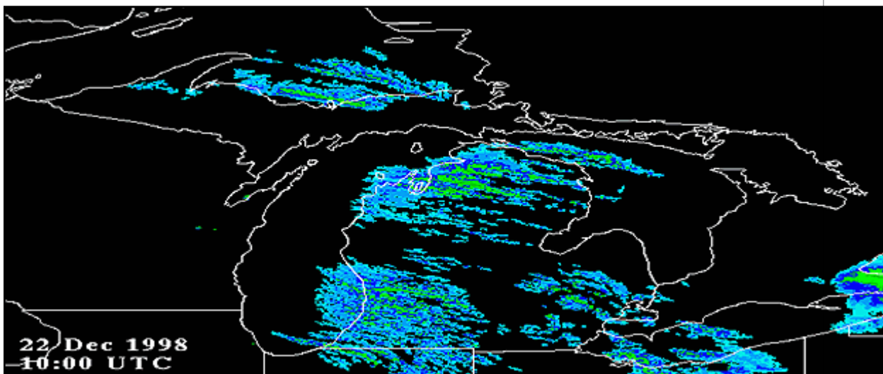
Figure 12: Multiple bands of lake effect snow
