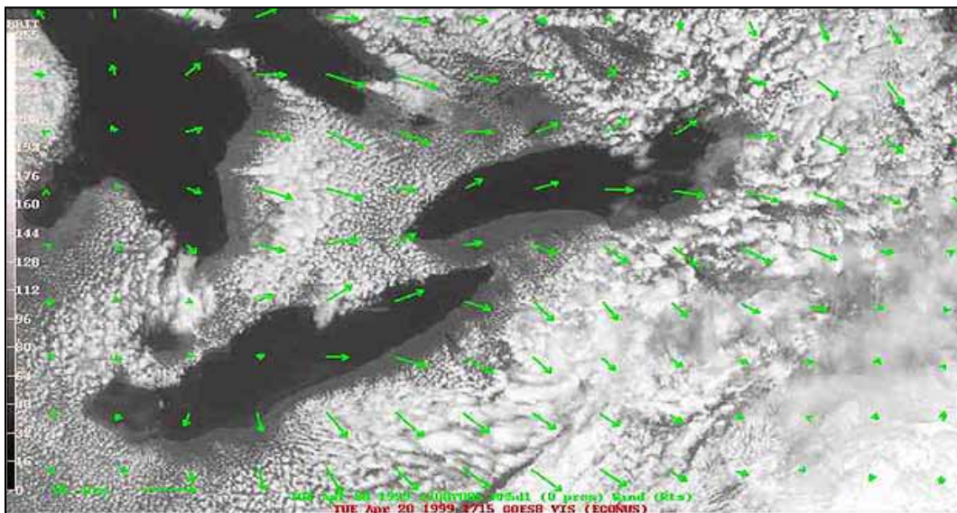
Figure 28: Satellite view of eastern Great Lakes.
