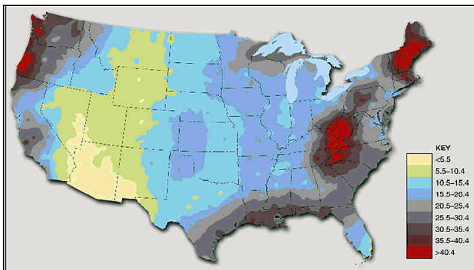
Figure 15: Number of days with dense fog: visibility less than ¼ mile
