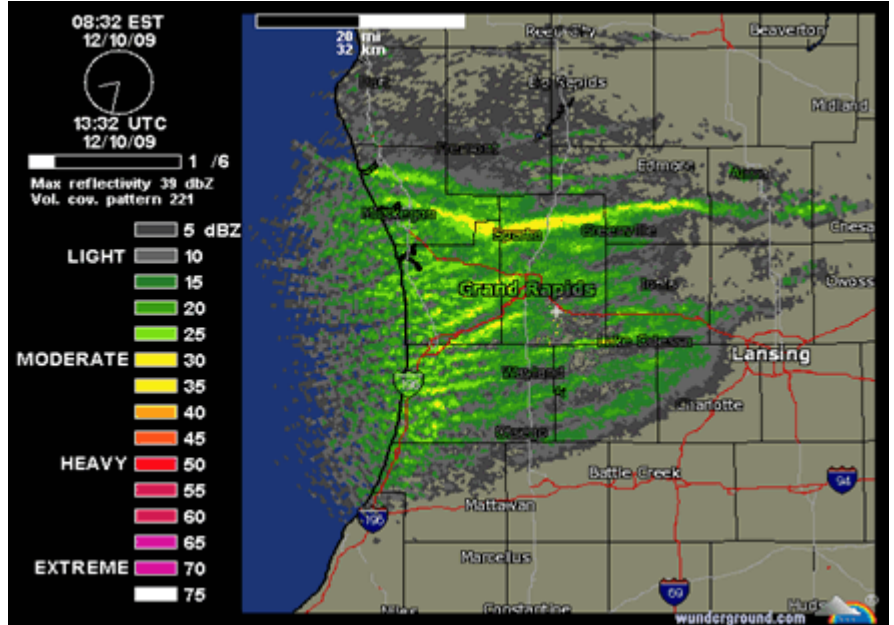
Figure 13: Multiple bands of lake-effect snow
