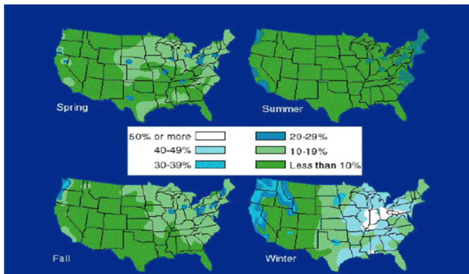
Figure 16: Probability of Instrument Meteorological Conditions
