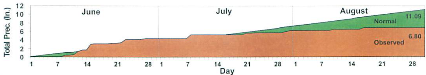
Summer 1998 Daily Cumulative Precipitation at DCA
