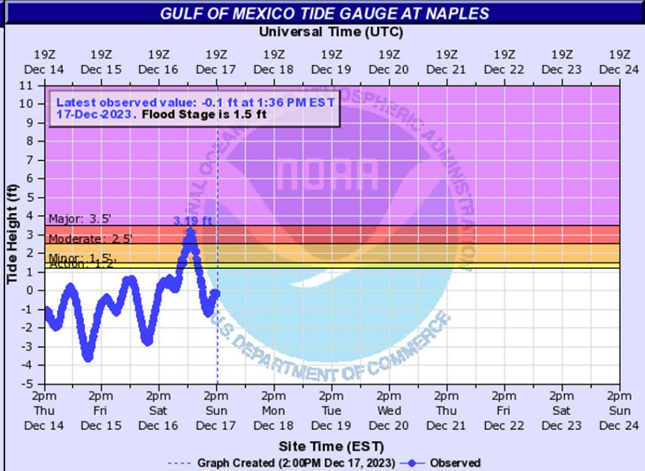
NPSF1(plotting HMIRG) "Gage 0" Datum: n/a
