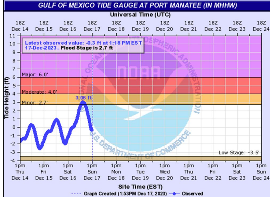
PMAF1(plotting HMIRG) "Gage 0" Datum: n/a
