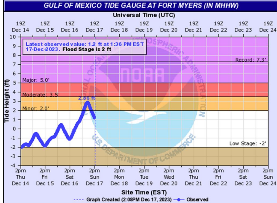
FMRF1(plotting HMIRG) "Gage 0" Datum: n/a
