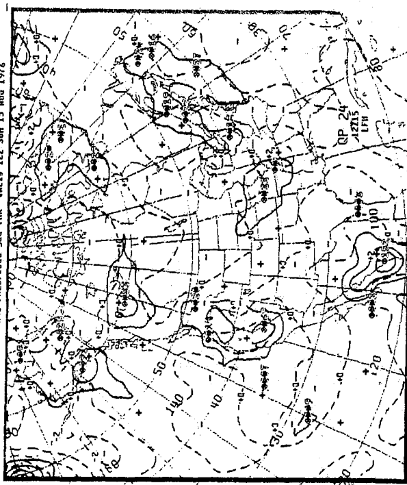
700 HEIGHT/VEL AND VORTICITY - RP 24 M086 .. 24HR ECST HEIGHTS/VORTICITY VALID 12Z SUN 15 AUG 1976
