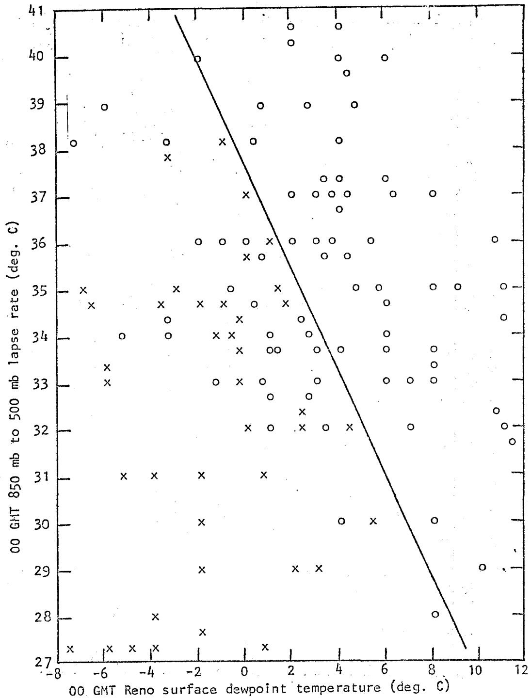
Figure 9 Distribution of observed Sierra cumulonimbus days (o) and Sierra days with no convection (x) as functions of Reno surface dewpoint and 850-mb to 500-mb lapse rate.
